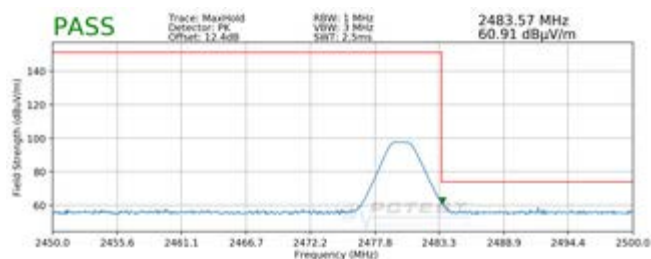
Plot 7-52. Radiated Restricted Upper Band Edge Measurement (Peak) (2 Mbps)
