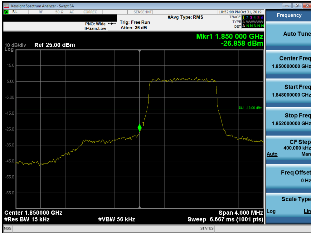
Plot 7-243. Lower Band Edge Plot (Band 25/2 - 1.4MHz QPSK - Full RB Configuration)
