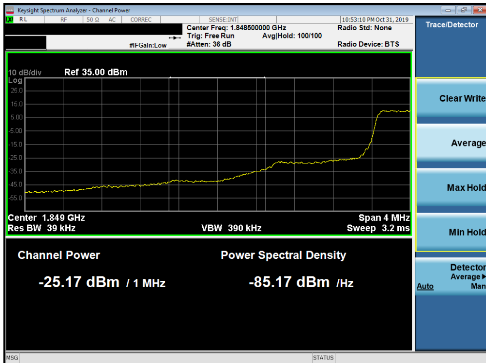
Plot 7-244. Lower Extended Band Edge Plot (Band 25/2 - 1.4MHz QPSK - Full RB Configuration)
