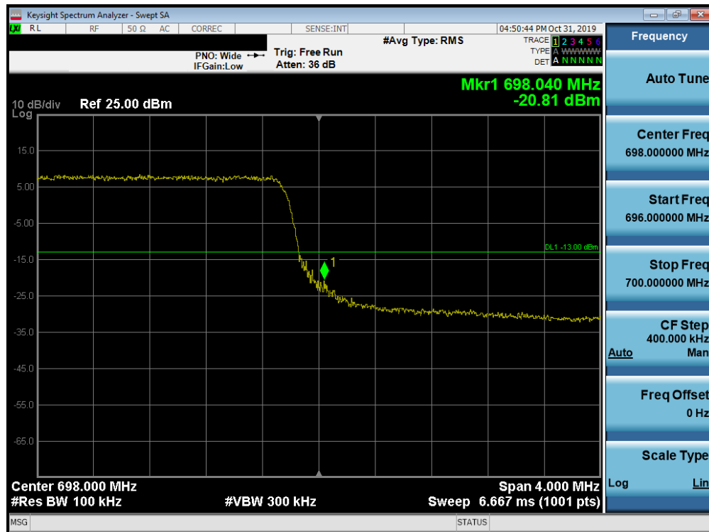
Plot 7-173. Upper Band Edge Plot (Band 71 - 5.0MHz QPSK - Full RB Configuration)
