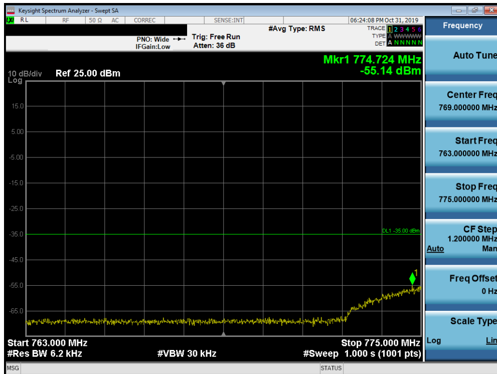
Plot 7-190. Lower Emission Mask Plot (Band 13 - 5.0MHz QPSK - Full RB Configuration)
