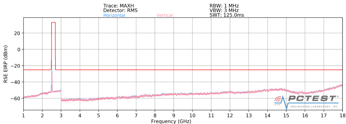
Plot 7-367. Radiated Spurious Plot 1GHz - 18GHz (Band 41 PC3)
