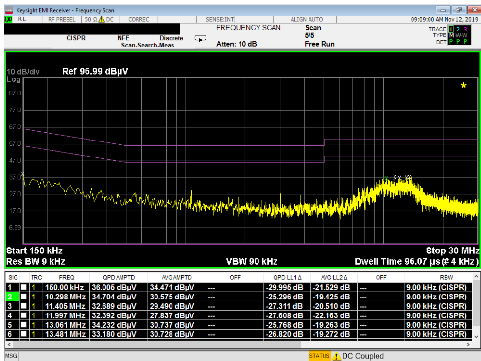
Plot 7-40. Line Conducted Plot with 802.11b (N)
