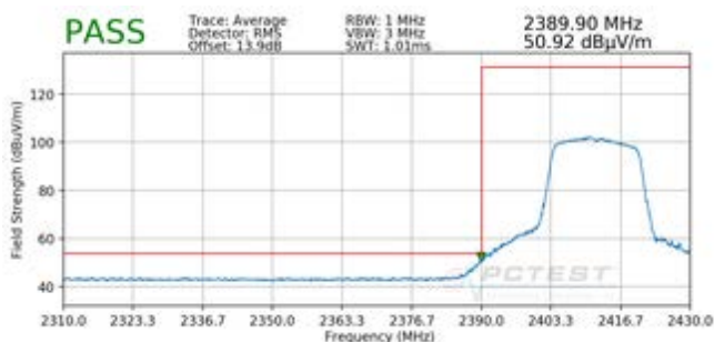
Plot 7-35. Radiated Restricted Lower Band Edge Measurement (Average)
