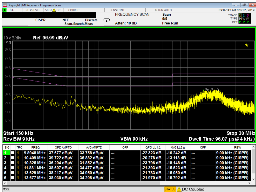
Plot 7-39. Line Conducted Plot with 802.11b (L1)
