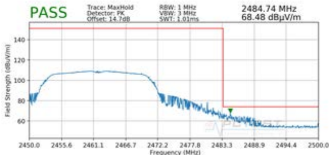
Plot 7-38. Radiated Restricted Upper Band Edge Measurement (Peak)
