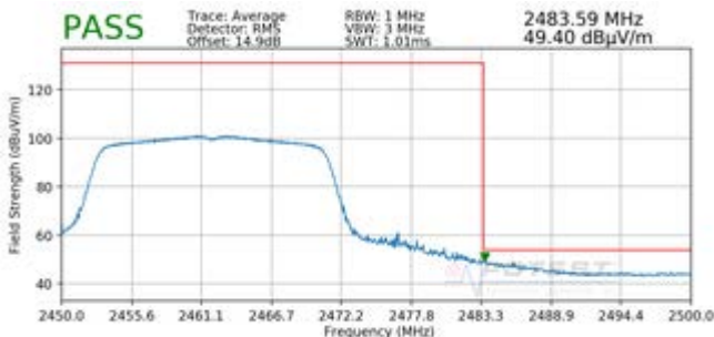
Plot 7-37. Radiated Restricted Upper Band Edge Measurement (Average)
