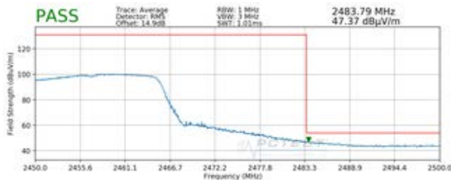
Plot 7-9. Radiated Restricted Upper Band Edge Measurement (Average)
