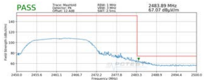
Plot 7-12. Radiated Restricted Upper Band Edge Measurement (Peak)
