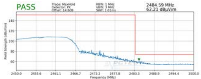
Plot 7-10. Radiated Restricted Upper Band Edge Measurement (Peak)
