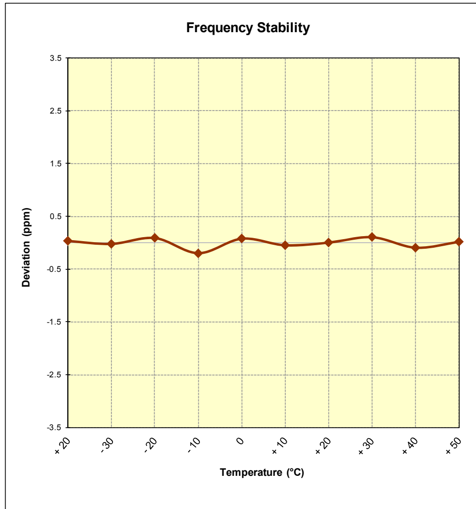
Figure 7-10. Frequency Stability Graph (Band 2)
