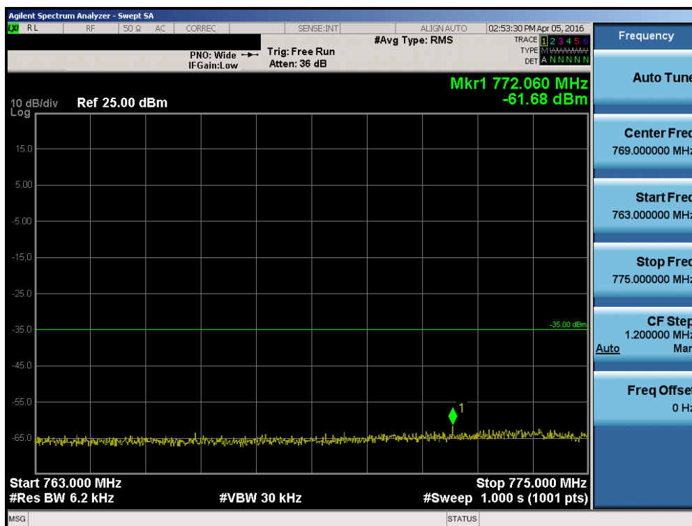
Plot 7-61. Lower Emission Mask Edge Plot (Band 13 – 10.0MHz QPSK – RB Size 50)
