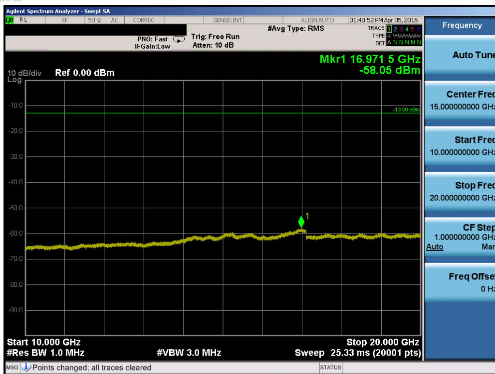
Plot 7-43. Conducted Spurious Plot (Band 4 – 20.0MHz QPSK – RB Size 1, RB Offset 0 – Mid Channel)
