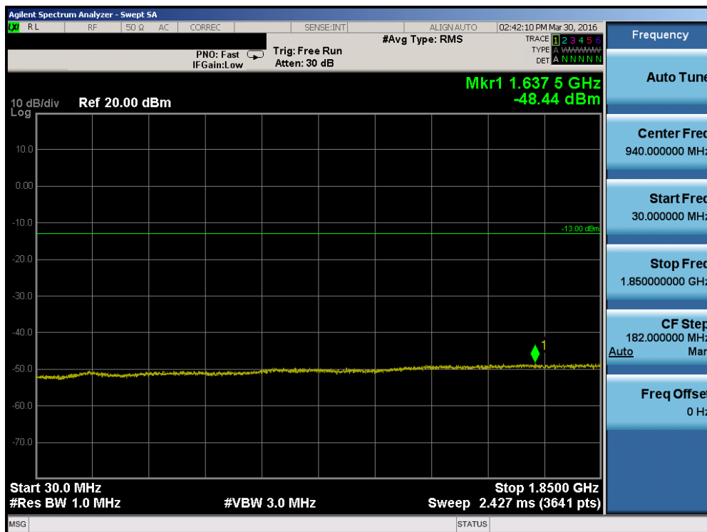
Plot 7-50. Conducted Spurious Plot (Band 2 – 20.0MHz QPSK – RB Size 1, RB Offset 0 – Mid Channel)
