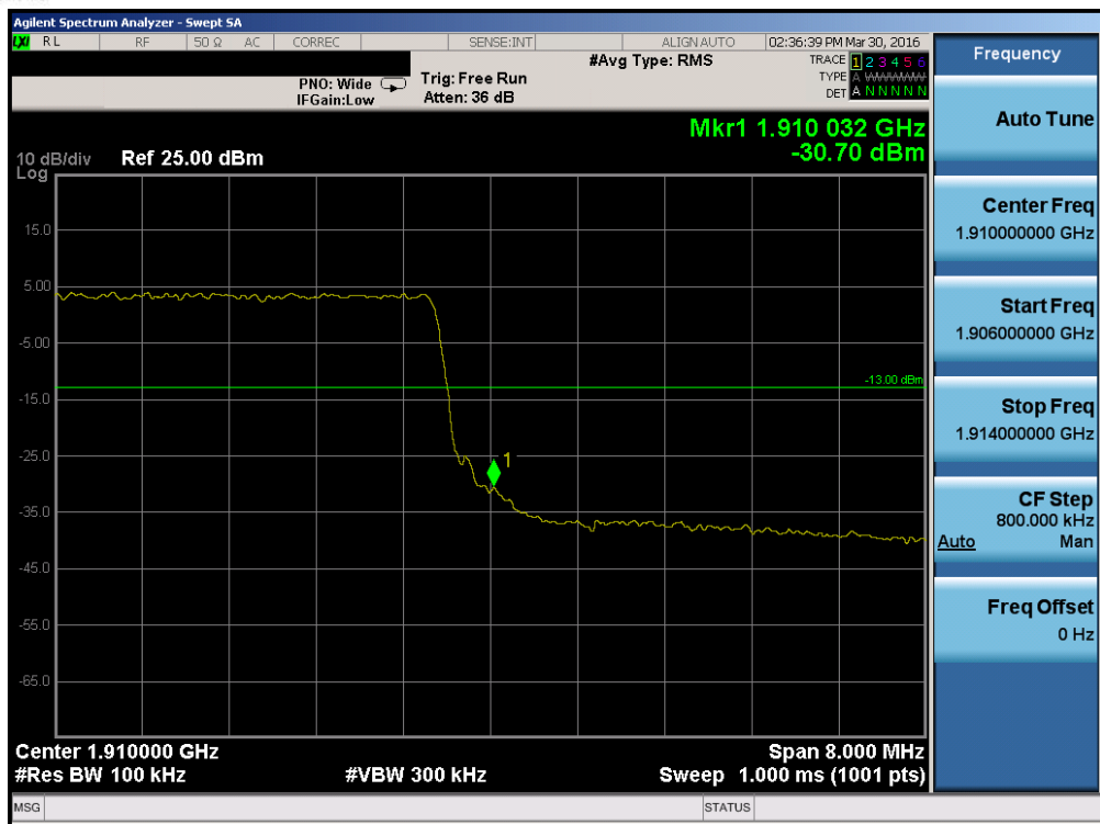
Plot 7-102. Upper Band Edge Plot (Band 2 – 10.0MHz QPSK – RB Size 50)
