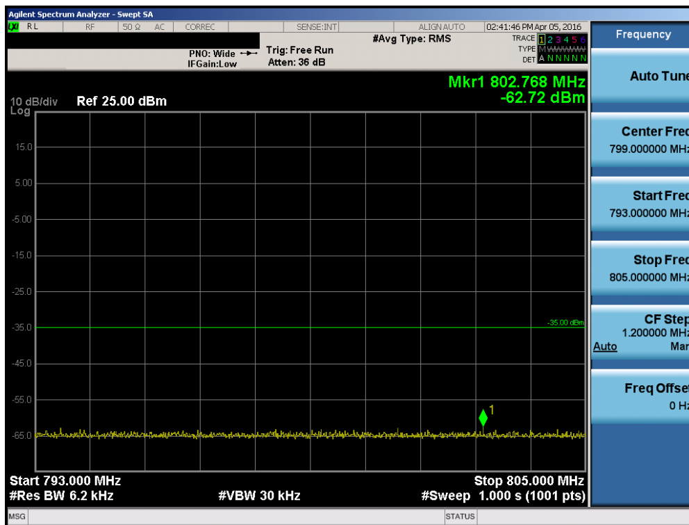
Plot 7-59. Upper Emission Mask Edge Plot (Band 13 – 5.0MHz QPSK – RB Size 25)
