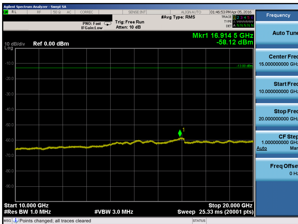
Plot 7-46. Conducted Spurious Plot (Band 4 – 20.0MHz QPSK – RB Size 1, RB Offset 0 – High Channel)
