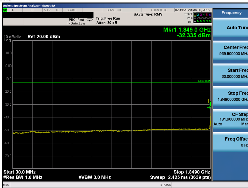
Plot 7-47. Conducted Spurious Plot (Band 2 – 20.0MHz QPSK – RB Size 1, RB Offset 0– Low Channel)
