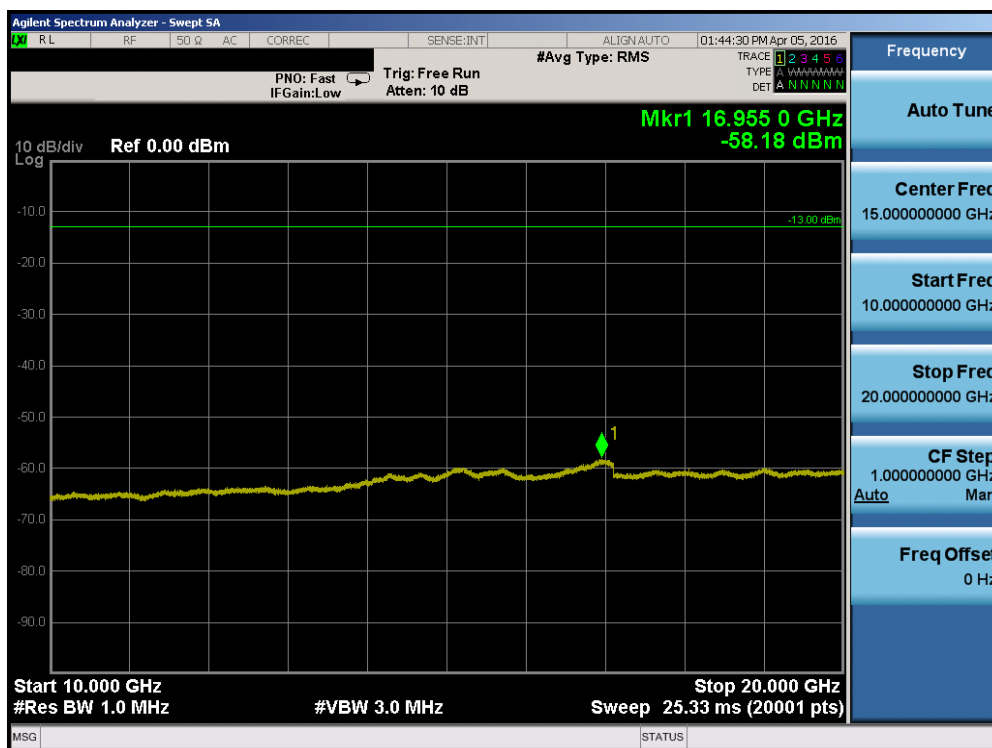
Plot 7-40. Conducted Spurious Plot (Band 4 – 20.0MHz QPSK – RB Size 1, RB Offset 0 – Low Channel)
