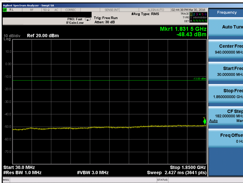
Plot 7-53. Conducted Spurious Plot (Band 2 – 20.0MHz QPSK – RB Size 1, RB Offset 0 – High Channel)
