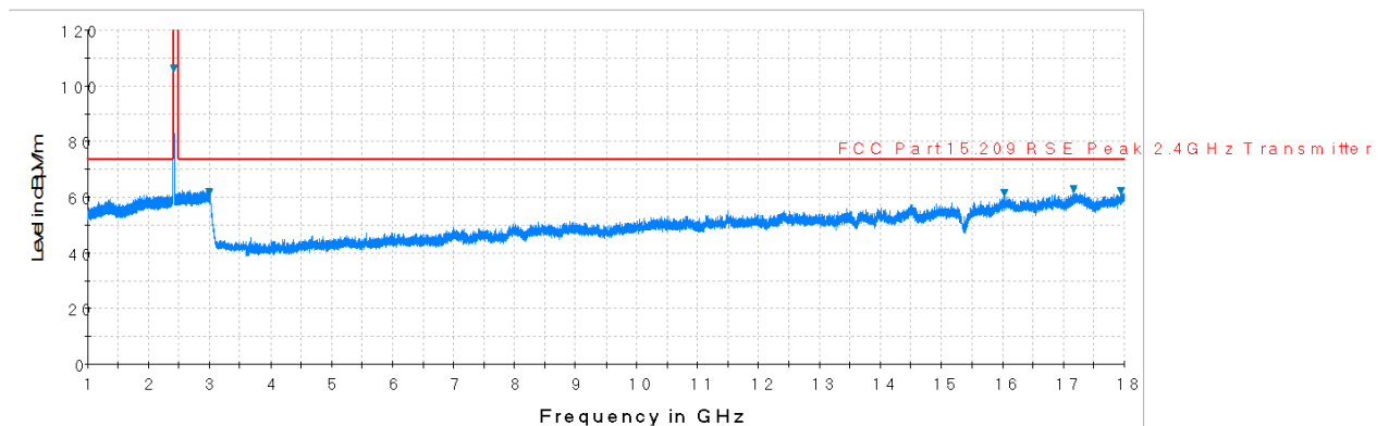
Plot 7-36. Radiated Spurious Plot above 1GHz (802.11b – Ch. 1, Ant. Pol. V)
