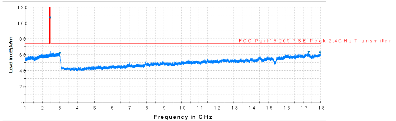
Plot 7-38. Radiated Spurious Plot above 1GHz (802.11b – Ch. 6, Ant. Pol. V)
