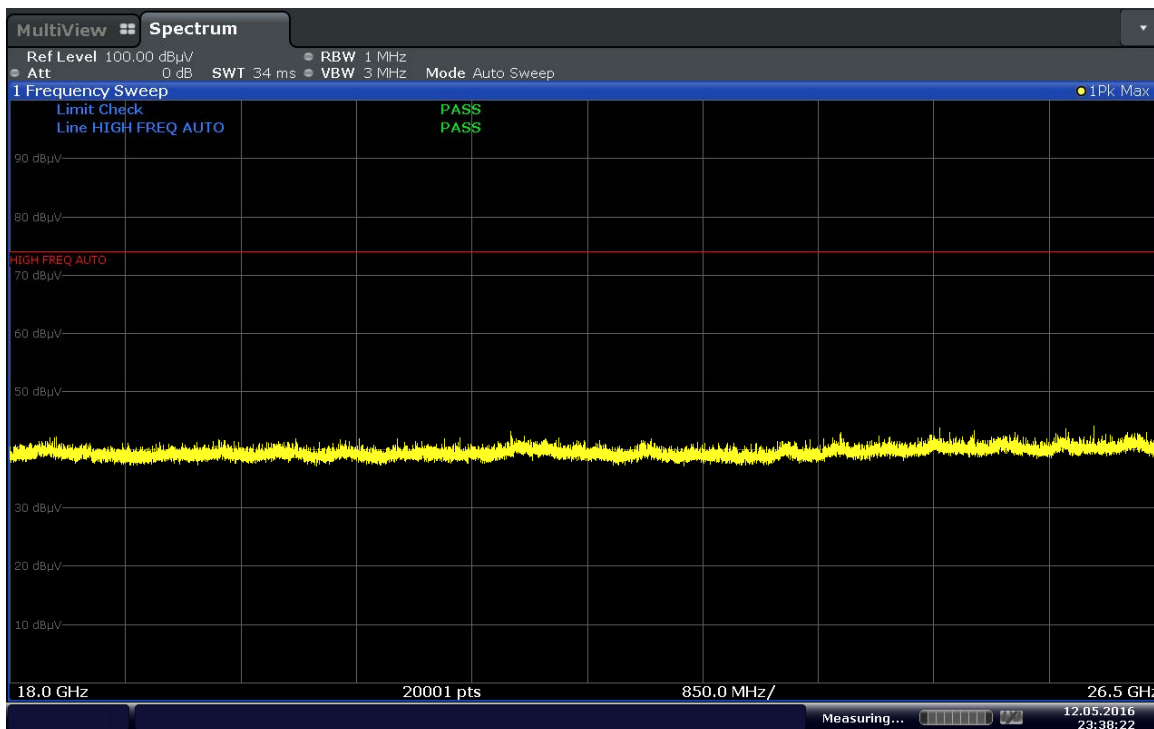
Plot 7-42. Radiated Spurious Plot above 18GHz (Pol. V)
