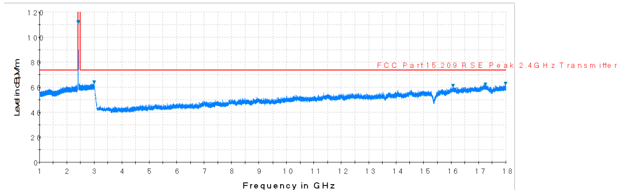
Plot 7-35. Radiated Spurious Plot above 1GHz (802.11b – Ch. 1, Ant. Pol. H)
