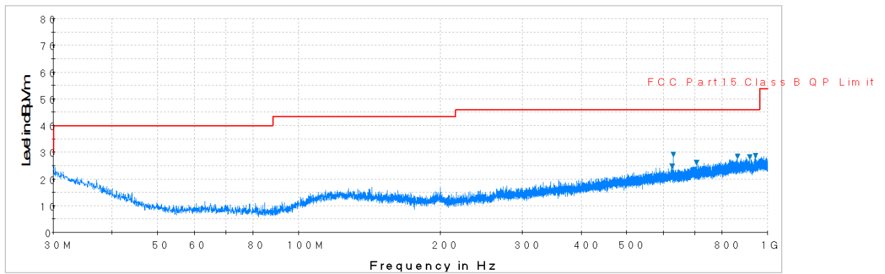
Plot 7-52. Radiated Spurious Plot below 1GHz (Pol. V)
