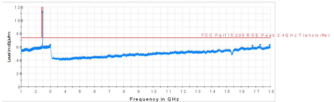
Plot 7-39. Radiated Spurious Plot above 1GHz (802.11b – Ch. 11, Ant. Pol. H)
