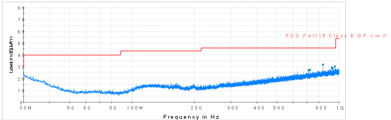
Plot 7-51. Radiated Spurious Plot below 1GHz (Pol. H)
