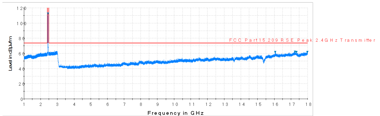
Plot 7-37. Radiated Spurious Plot above 1GHz (802.11b – Ch. 6, Ant. Pol. H)
