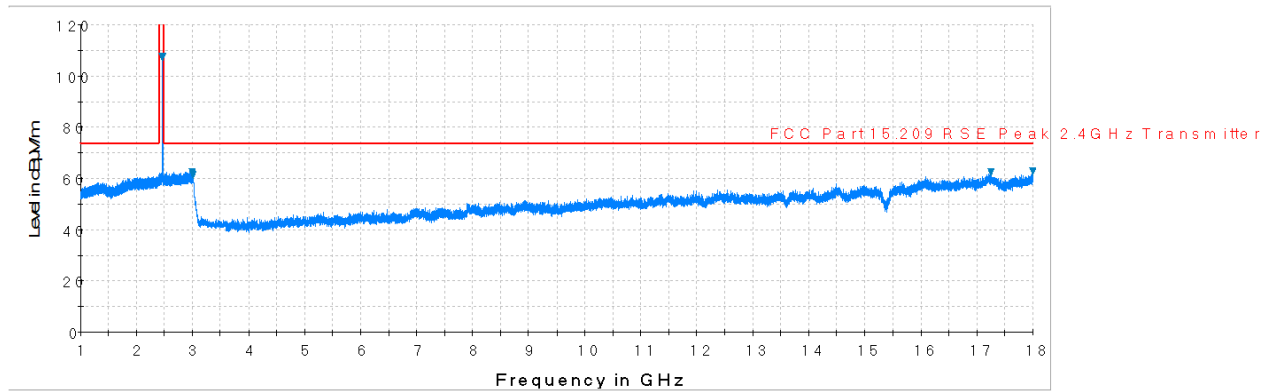
Plot 7-40. Radiated Spurious Plot above 1GHz (802.11b – Ch. 11, Ant. Pol. V)
