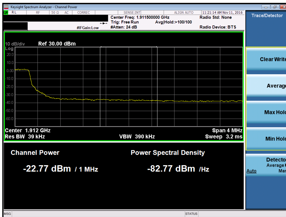
Plot 7-140. Upper Extended Band Edge Plot (Band 2 – 5.0MHz QPSK – RB Size 25)
