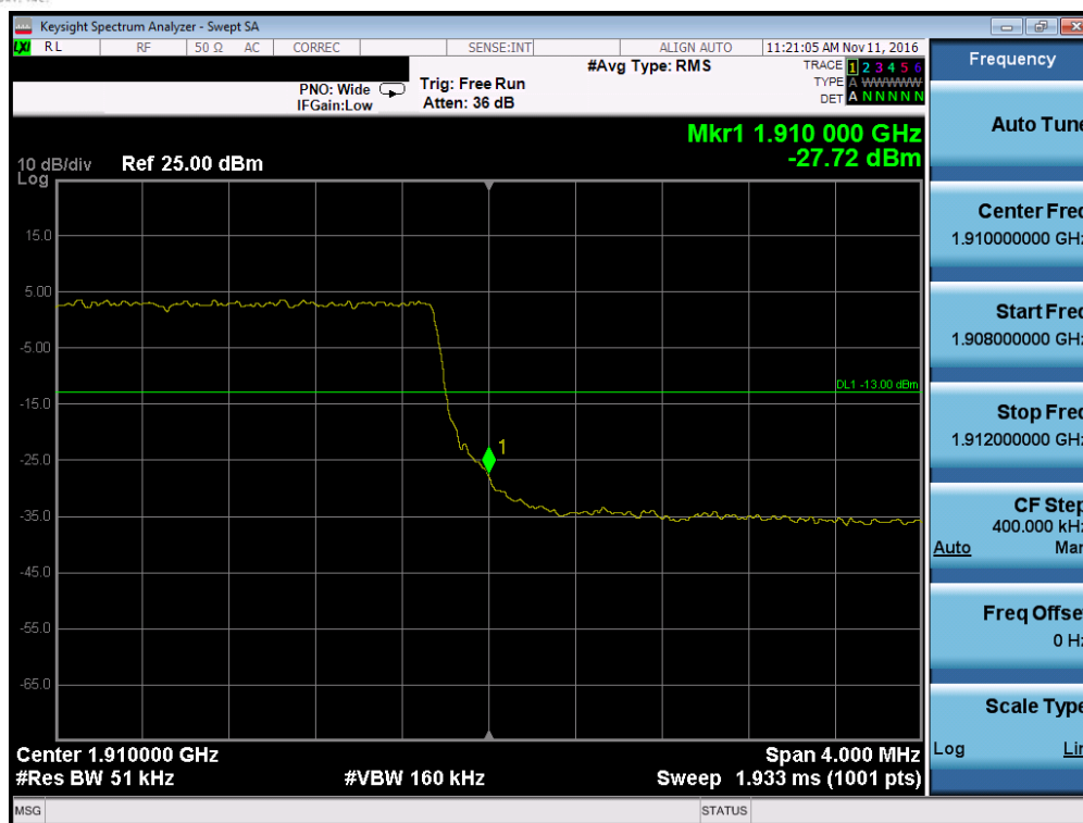
Plot 7-139. Upper Band Edge Plot (Band 2 – 5.0MHz QPSK – RB Size 25)
