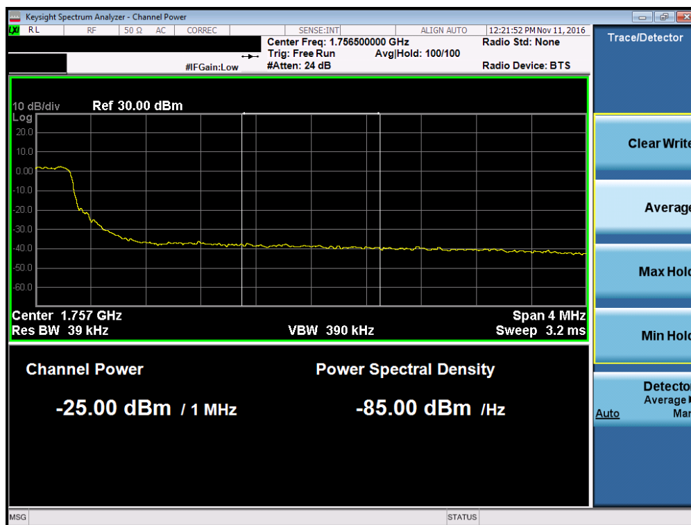
Plot 7-116. Upper Extended Band Edge Plot (Band 4 – 5.0MHz QPSK – RB Size 25)
