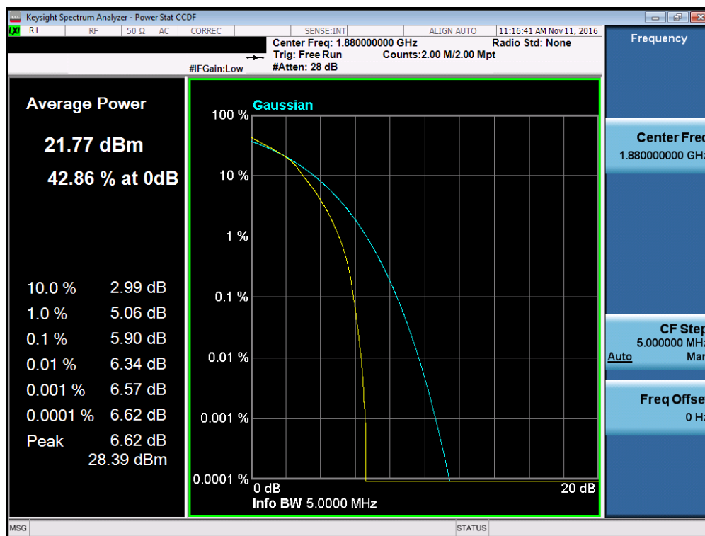
Plot 7-158. PAR Plot (Band 2 – 5.0MHz 16-QAM – RB Size 25)
