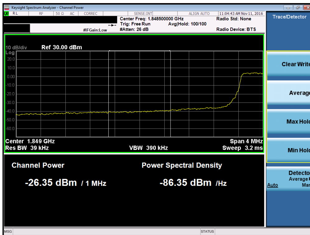
Plot 7-134. Lower Extended Band Edge Plot (Band 2 – 3.0MHz QPSK – RB Size 15)
