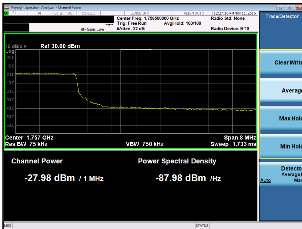
Plot 7-120. Upper Extended Band Edge Plot (Band 4 – 10.0MHz QPSK – RB Size 50)
