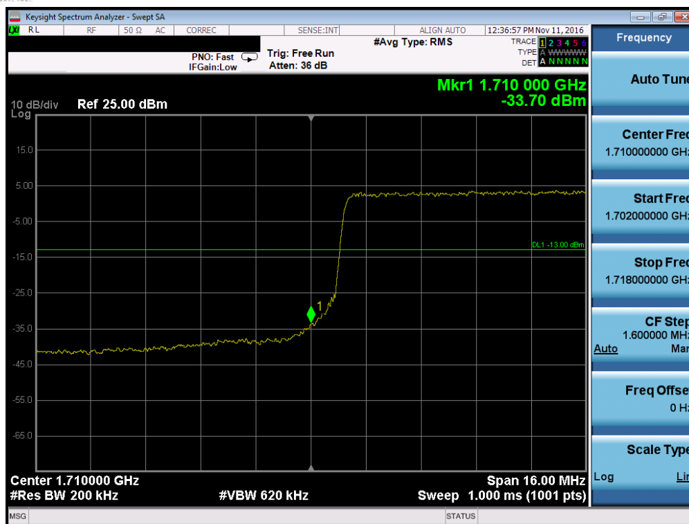
Plot 7-125. Lower Band Edge Plot (Band 4 – 20.0MHz QPSK – RB Size 100)
