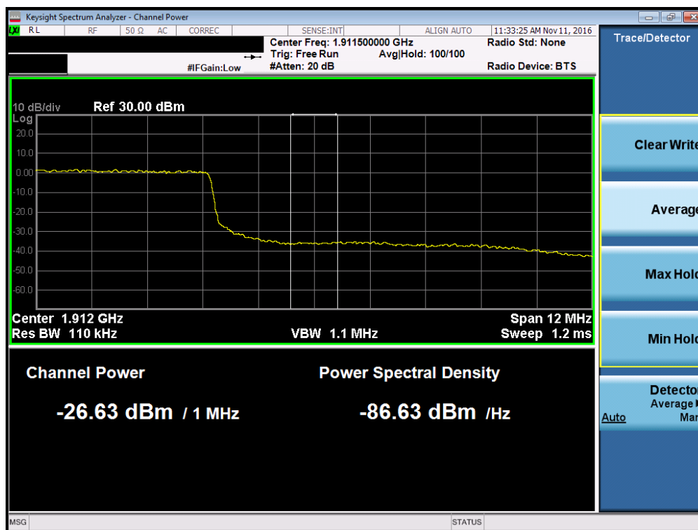
Plot 7-148. Upper Extended Band Edge Plot (Band 2 – 15.0MHz QPSK – RB Size 75)
