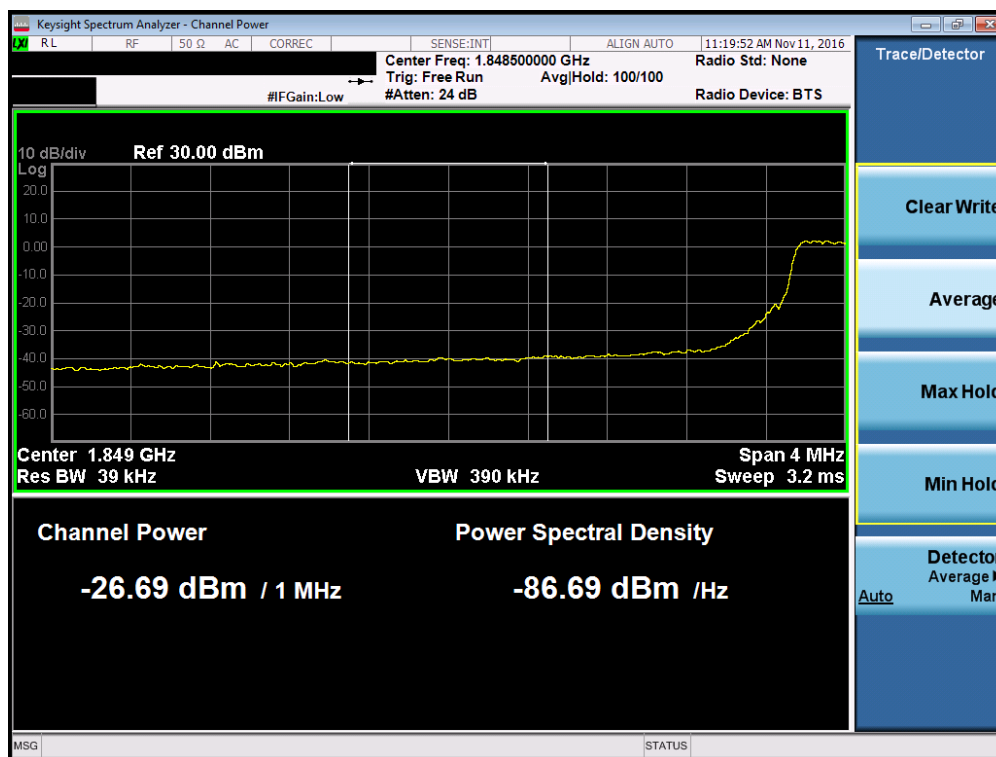
Plot 7-138. Lower Extended Band Edge Plot (Band 2 – 5.0MHz QPSK – RB Size 25)
