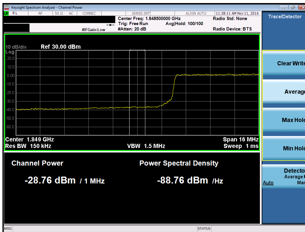
Plot 7-150. Lower Extended Band Edge Plot (Band 2 – 20.0MHz QPSK – RB Size 100)
