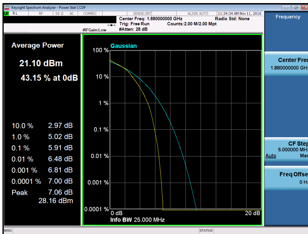
Plot 7-164. PAR Plot (Band 2 – 20.0MHz 16-QAM – RB Size 100)
