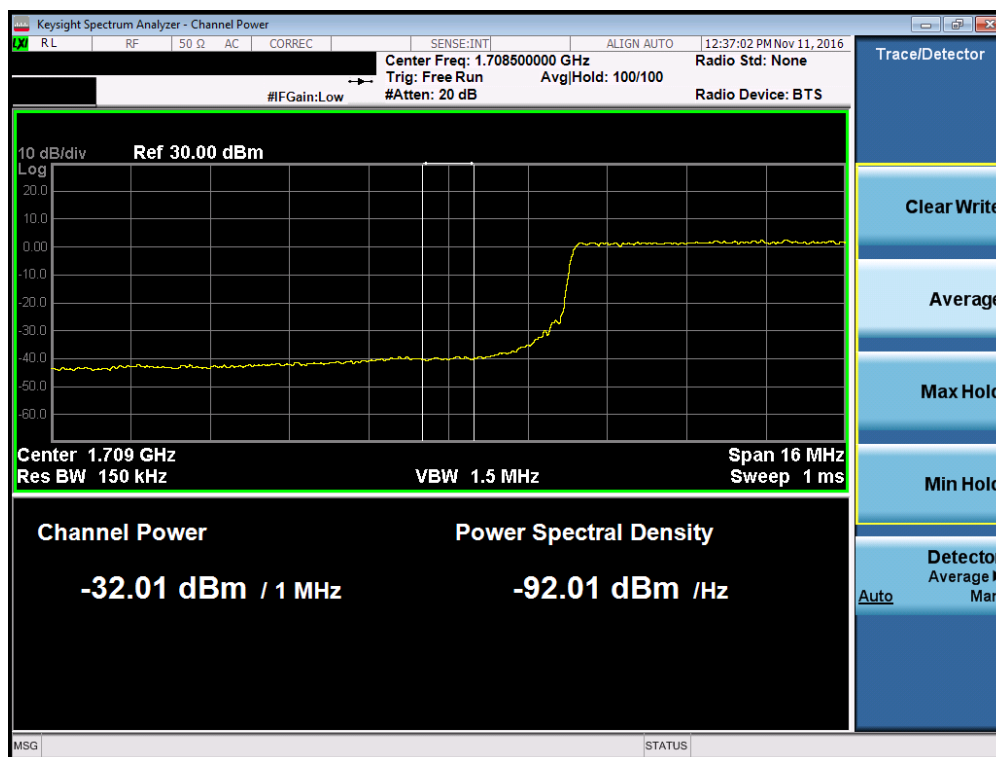
Plot 7-126. Lower Extended Band Edge Plot (Band 4 – 20.0MHz QPSK – RB Size 100)
