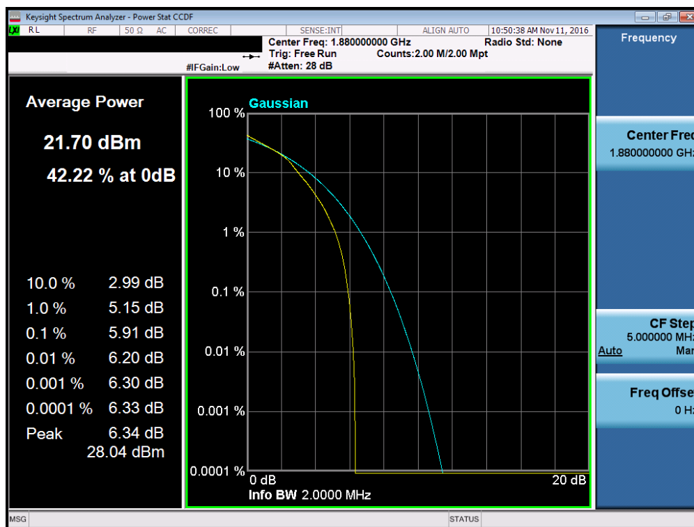
Plot 7-154. PAR Plot (Band 2 – 1.4MHz 16-QAM – RB Size 6)
