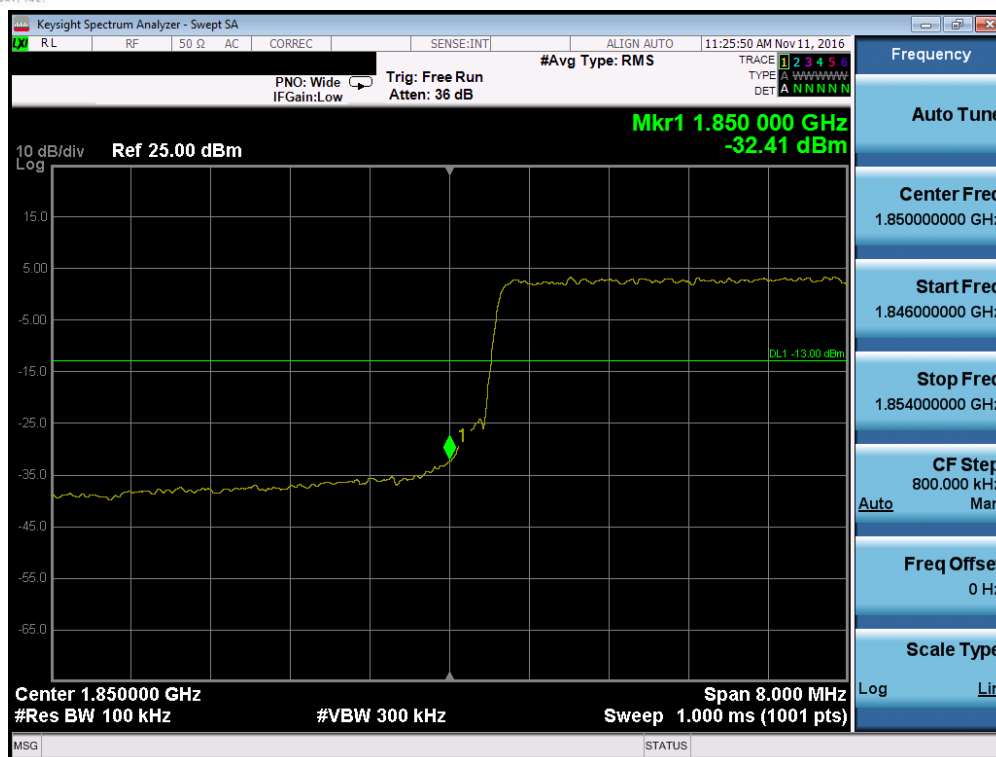
Plot 7-141. Lower Band Edge Plot (Band 2 – 10.0MHz QPSK – RB Size 50)
