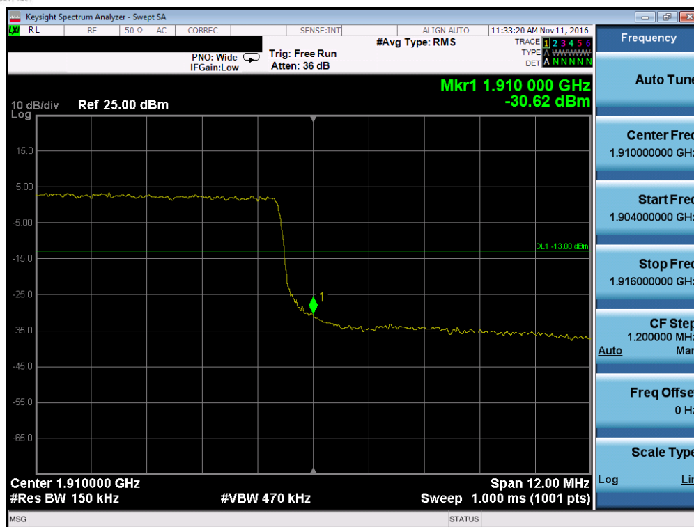
Plot 7-147. Upper Band Edge Plot (Band 2 – 15.0MHz QPSK – RB Size 75)
