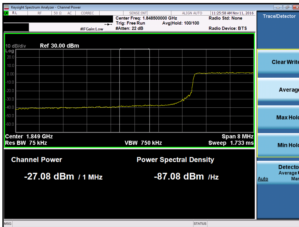
Plot 7-142. Lower Extended Band Edge Plot (Band 2 – 10.0MHz QPSK – RB Size 50)
