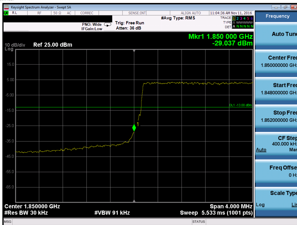
Plot 7-133. Lower Band Edge Plot (Band 2 – 3.0MHz QPSK – RB Size 15)
