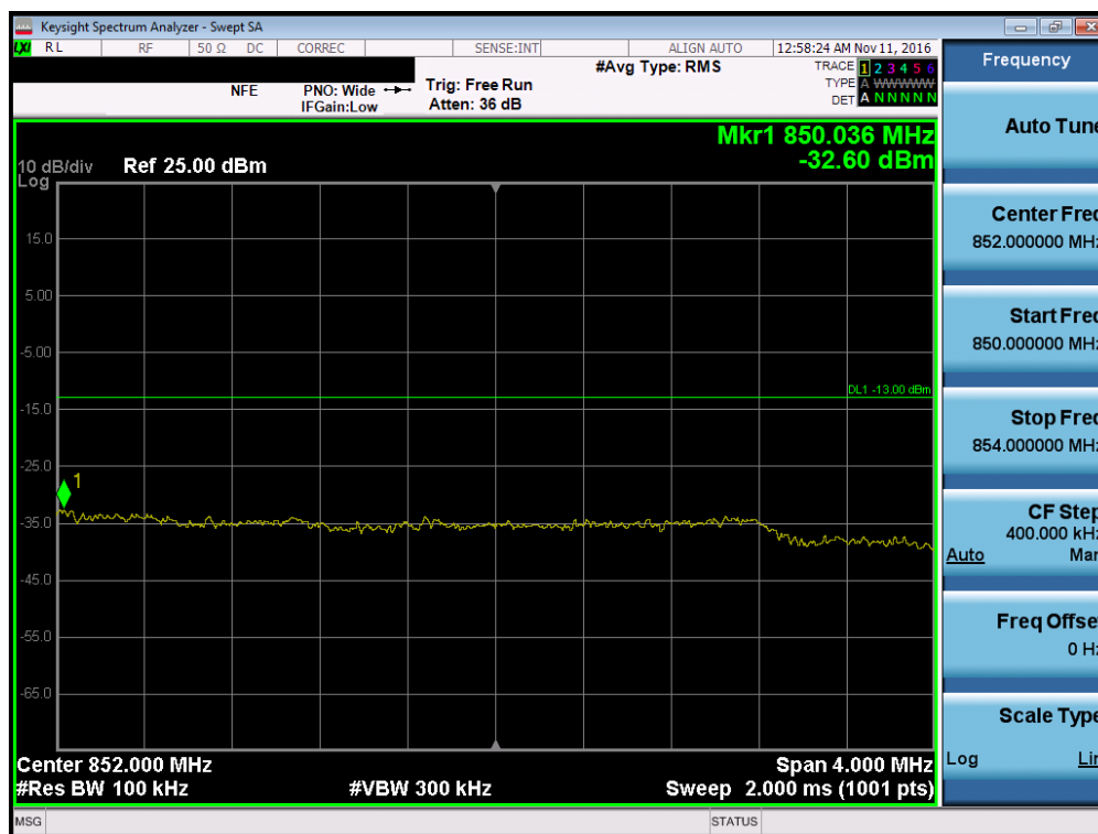
Plot 7-102. Upper Extended Band Edge Plot (Band 5 - 5.0MHz QPSK - RB Size 25)
