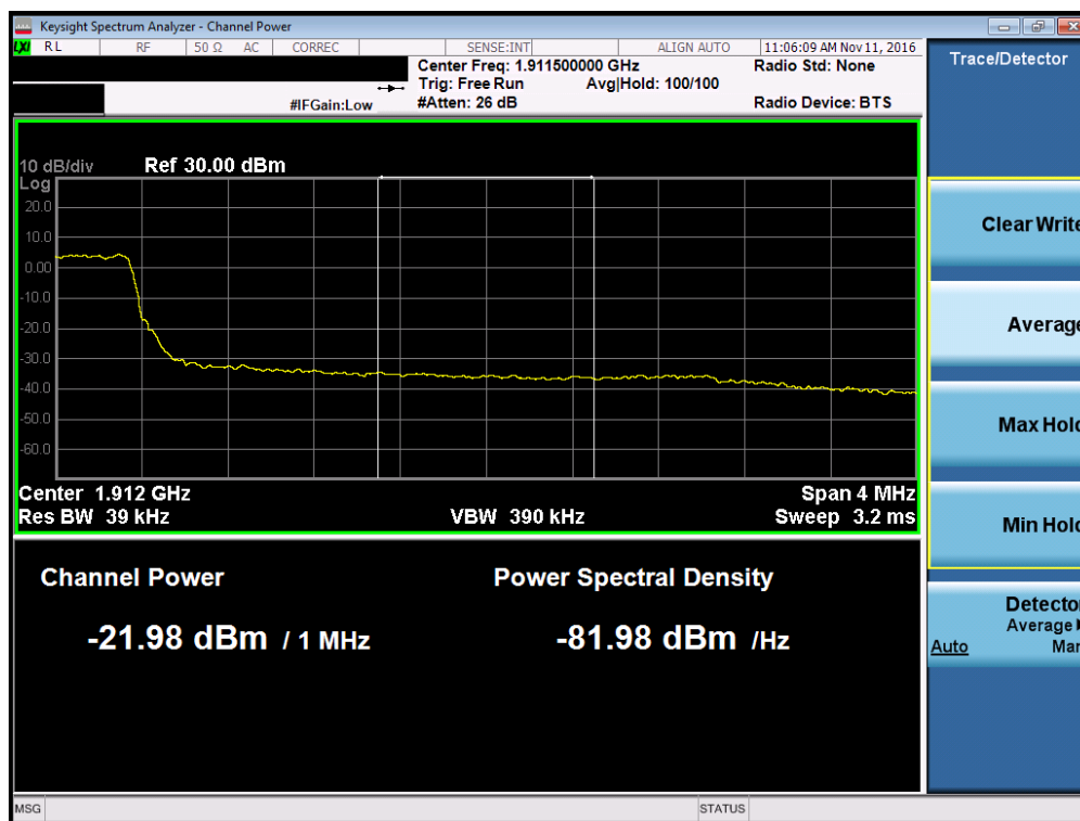
Plot 7-136. Upper Extended Band Edge Plot (Band 2 – 3.0MHz QPSK – RB Size 15)
