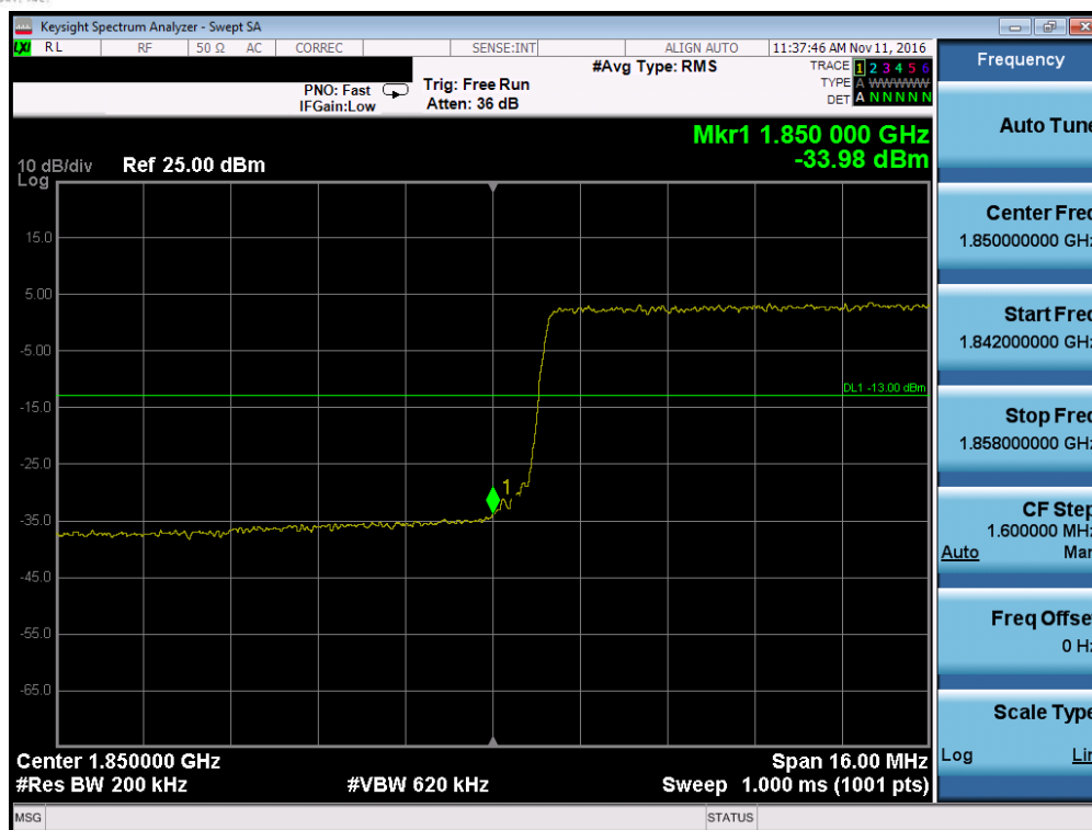
Plot 7-149. Lower Band Edge Plot (Band 2 – 20.0MHz QPSK – RB Size 100)
