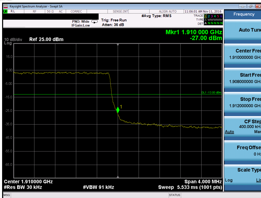
Plot 7-135. Upper Band Edge Plot (Band 2 – 3.0MHz QPSK – RB Size 15)
