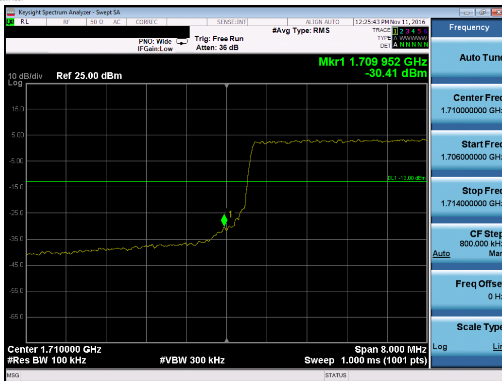
Plot 7-117. Lower Band Edge Plot (Band 4 – 10.0MHz QPSK – RB Size 50)
