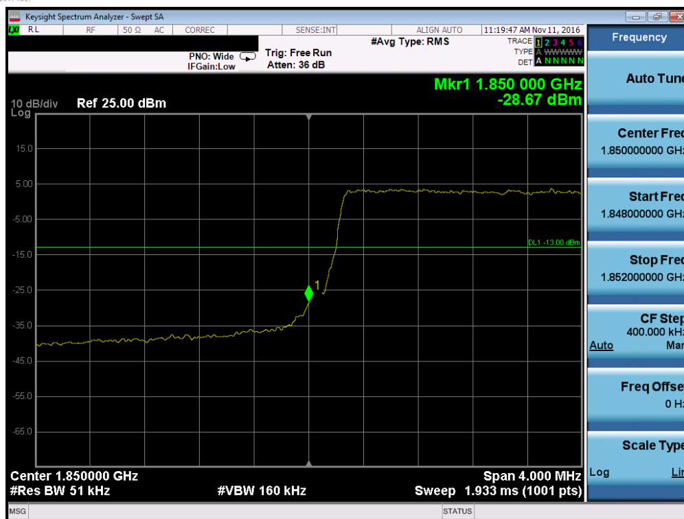
Plot 7-137. Lower Band Edge Plot (Band 2 – 5.0MHz QPSK – RB Size 25)
