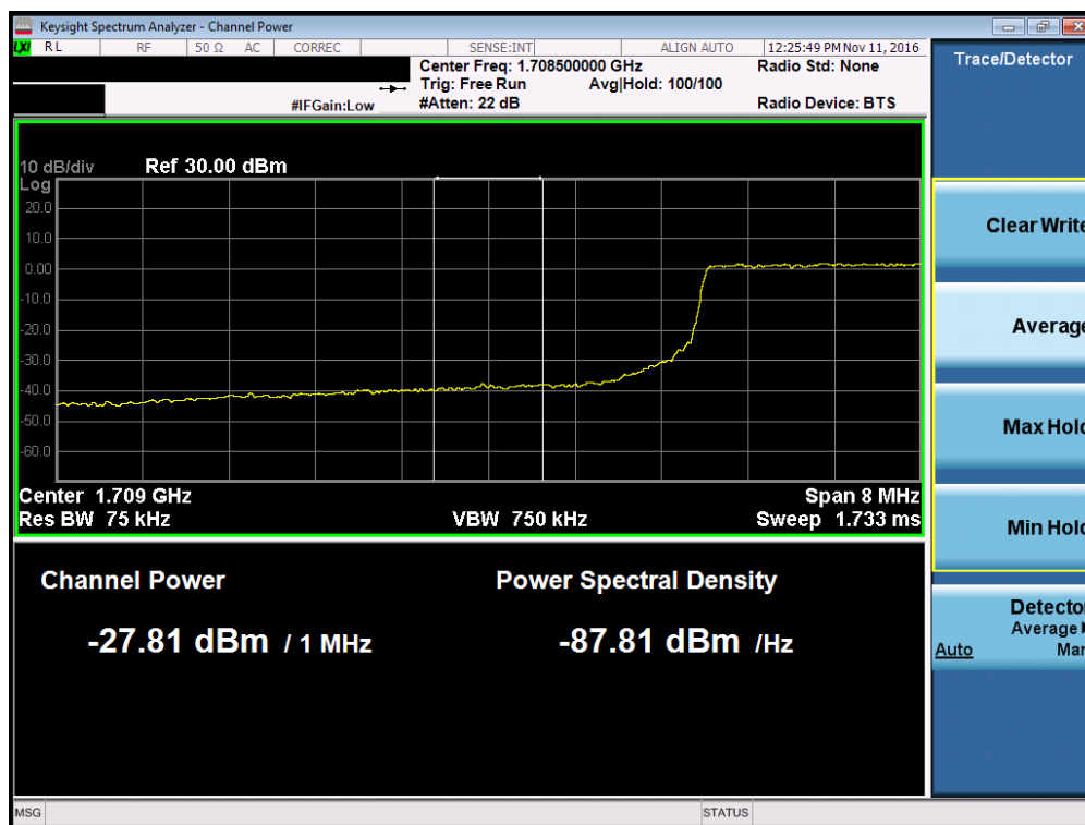
Plot 7-118. Lower Extended Band Edge Plot (Band 4 – 10.0MHz QPSK – RB Size 50)
