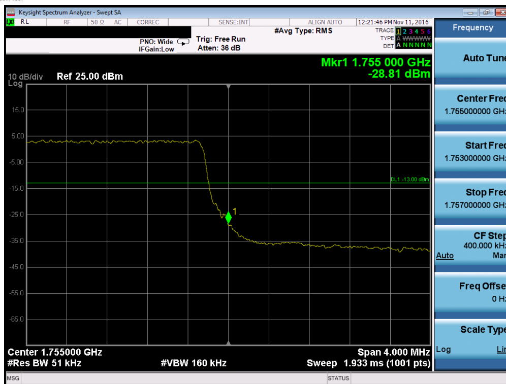
Plot 7-115. Upper Band Edge Plot (Band 4 – 5.0MHz QPSK – RB Size 25)
