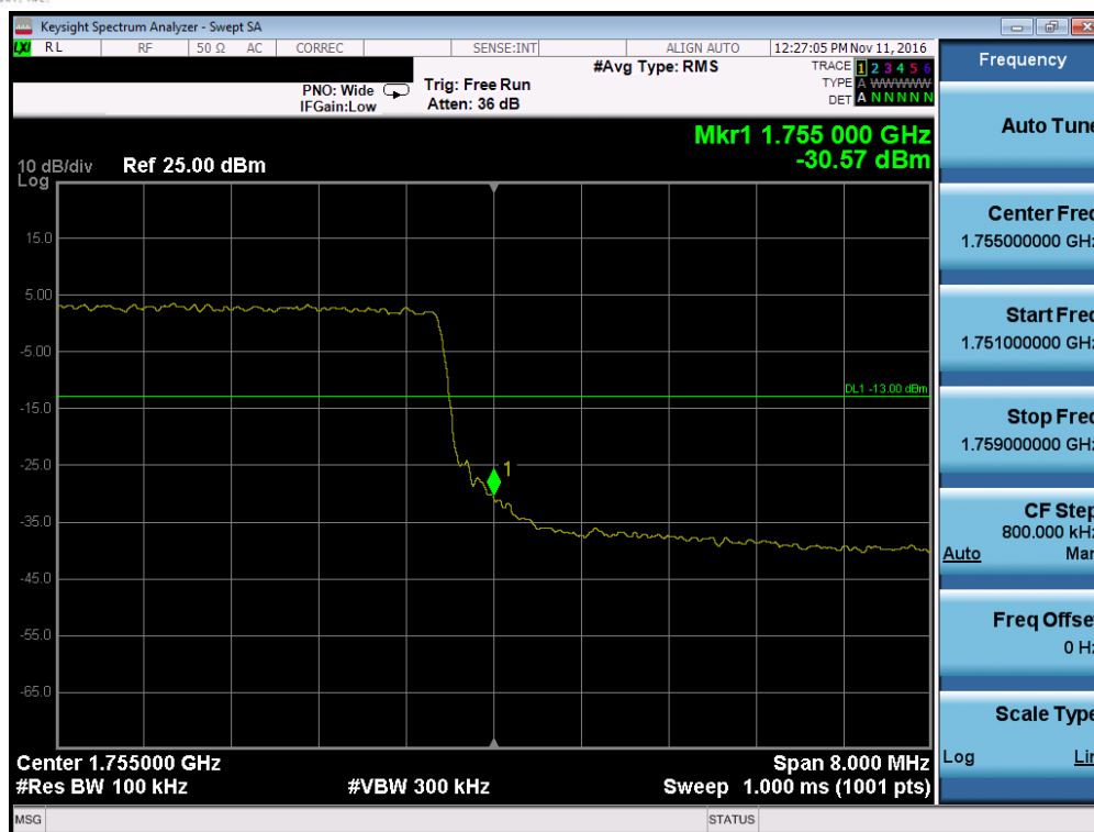
Plot 7-119. Upper Band Edge Plot (Band 4 – 10.0MHz QPSK – RB Size 50)
