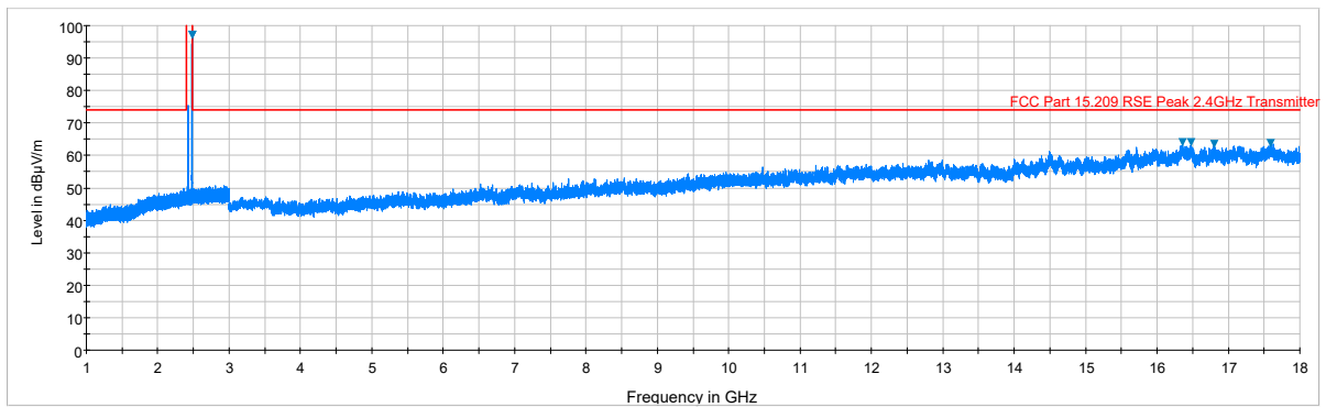
Plot 7-46. Radiated Spurious Plot above 1GHz (BT – Ch. 78, Ant. Pol. H)
