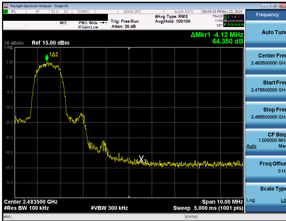
Plot 7-29. Band Edge Plot (Bluetooth with Hopping Disabled, 3 Mbps – Ch. 78)
