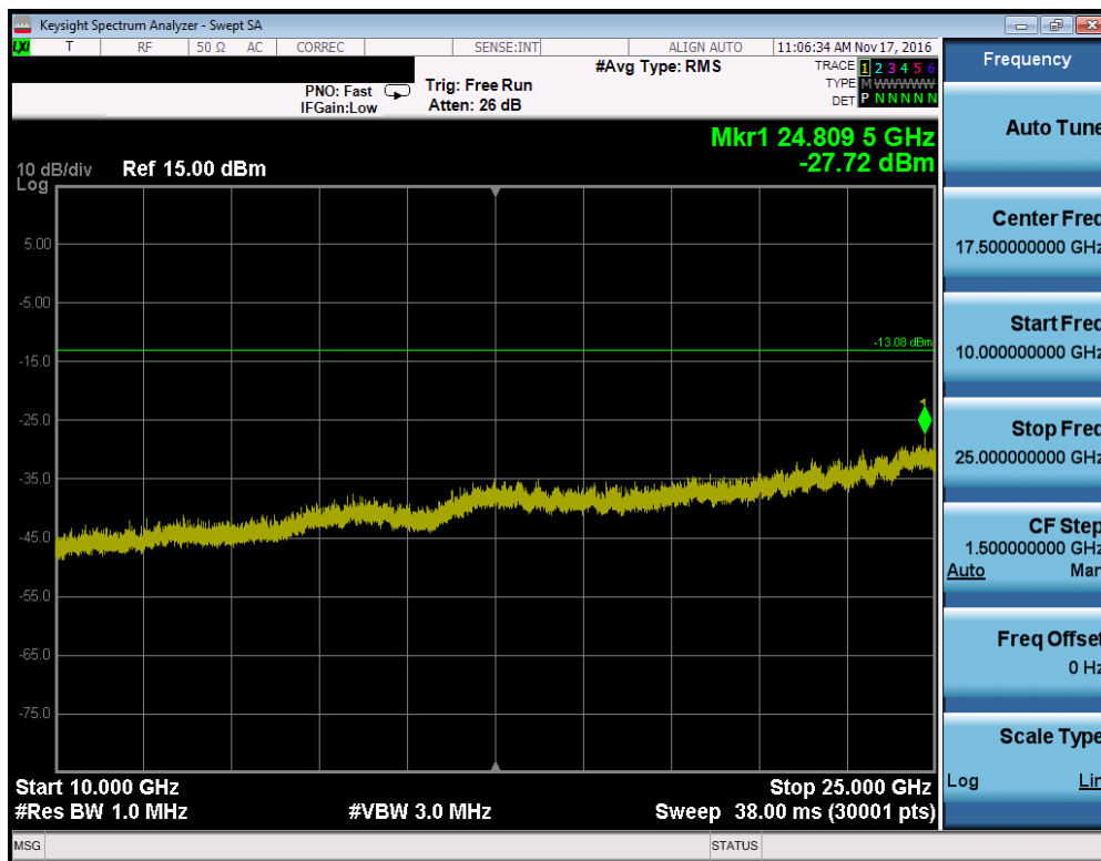
Plot 7-37. Conducted Spurious Plot (Bluetooth, 3Mbps – Ch. 0)
