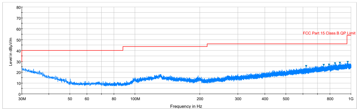
Plot 7-53. Radiated Spurious Plot below 1GHz (Pol. V)
