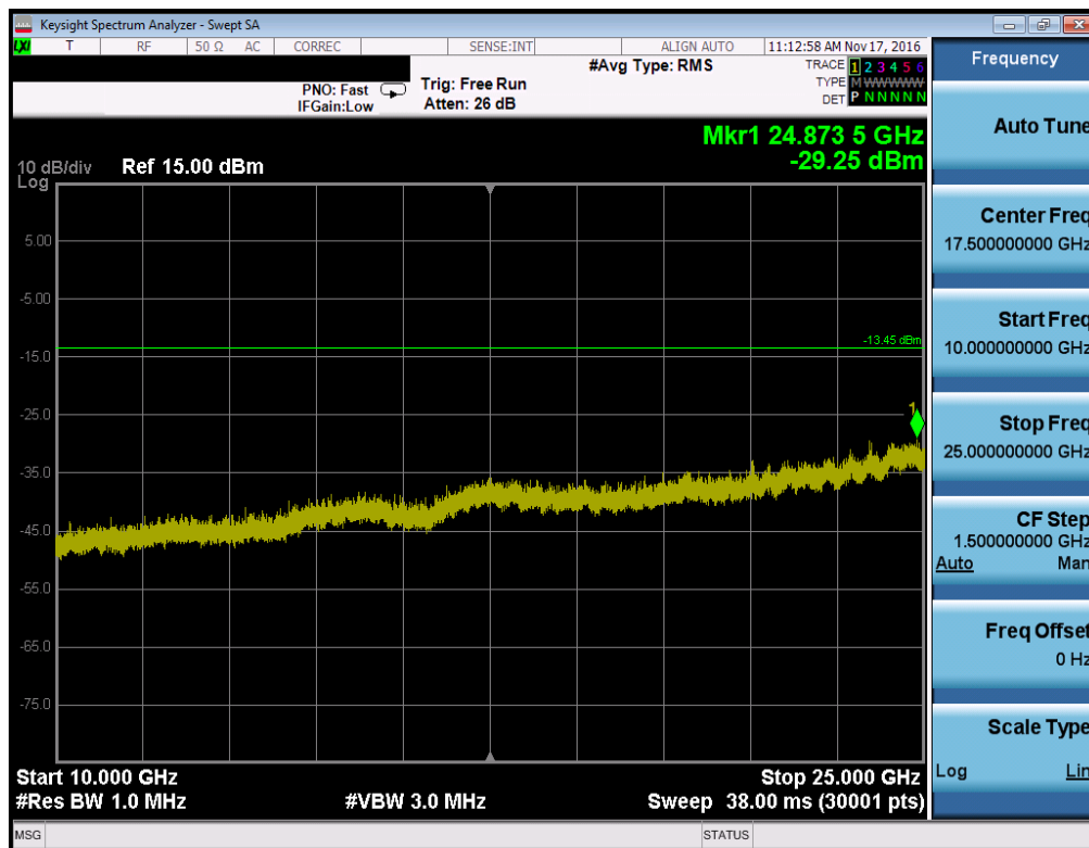
Plot 7-41. Conducted Spurious Plot (Bluetooth, 3Mbps – Ch. 78)
