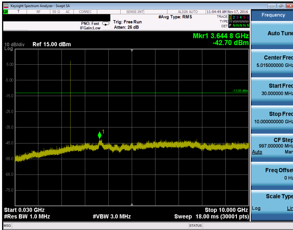
Plot 7-36. Conducted Spurious Plot (Bluetooth, 3Mbps – Ch. 0)
