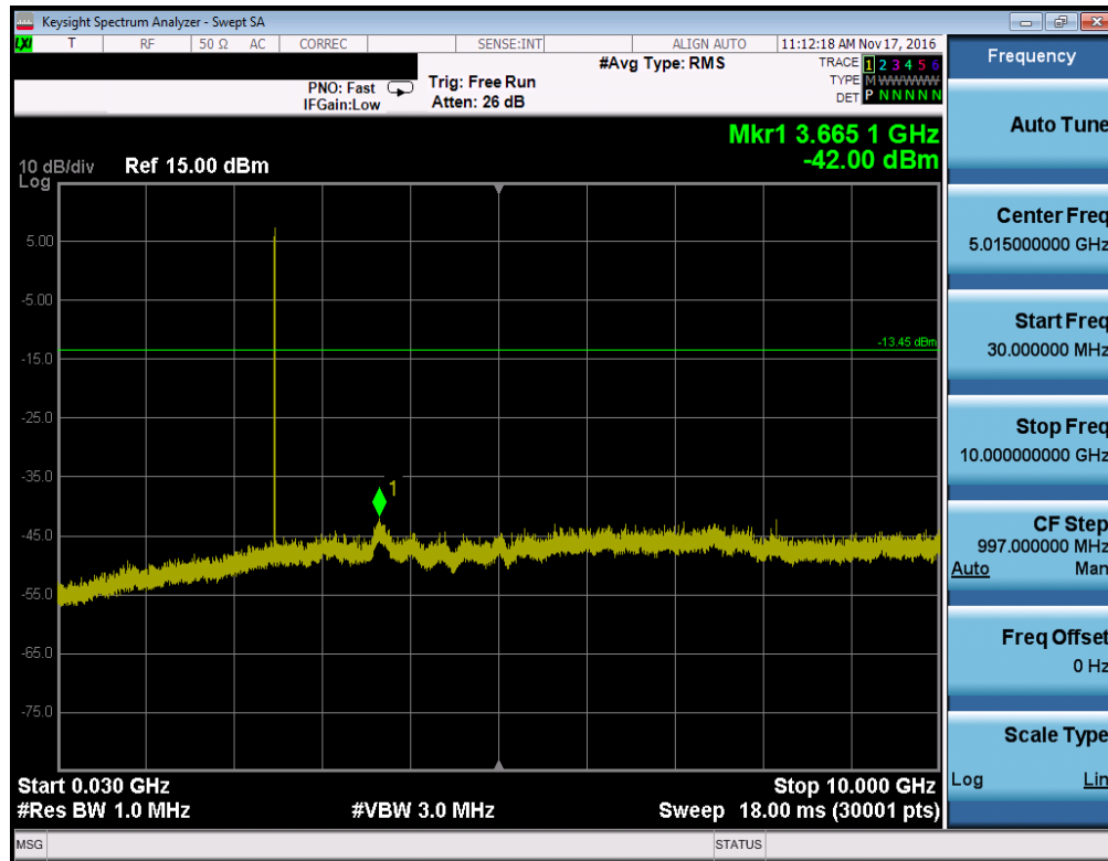
Plot 7-40. Conducted Spurious Plot (Bluetooth, 3Mbps – Ch. 78)
