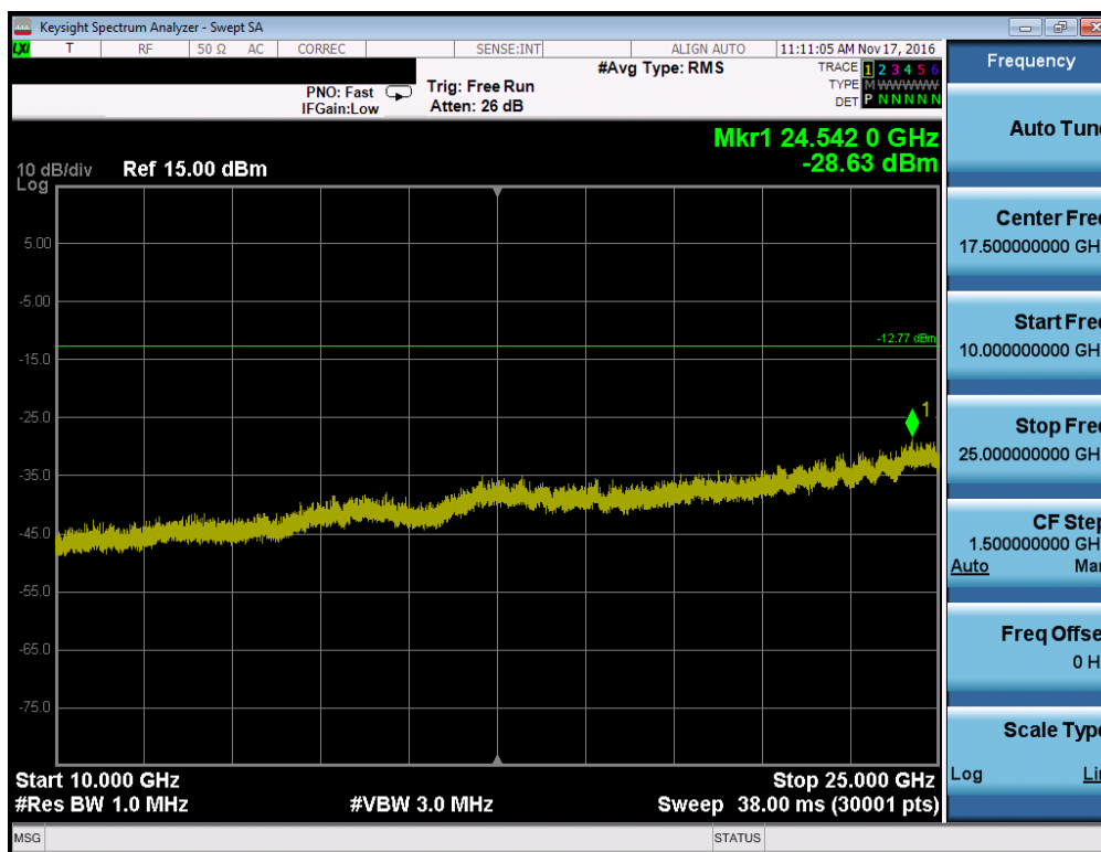
Plot 7-39. Conducted Spurious Plot (Bluetooth, 3Mbps – Ch. 39)
