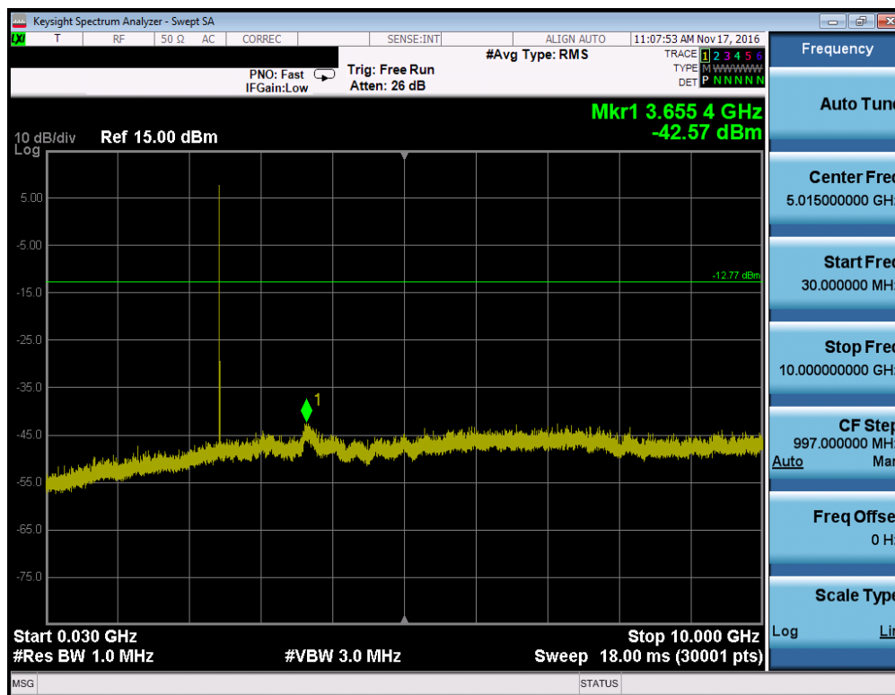
Plot 7-38. Conducted Spurious Plot (Bluetooth, 3Mbps – Ch. 39)
