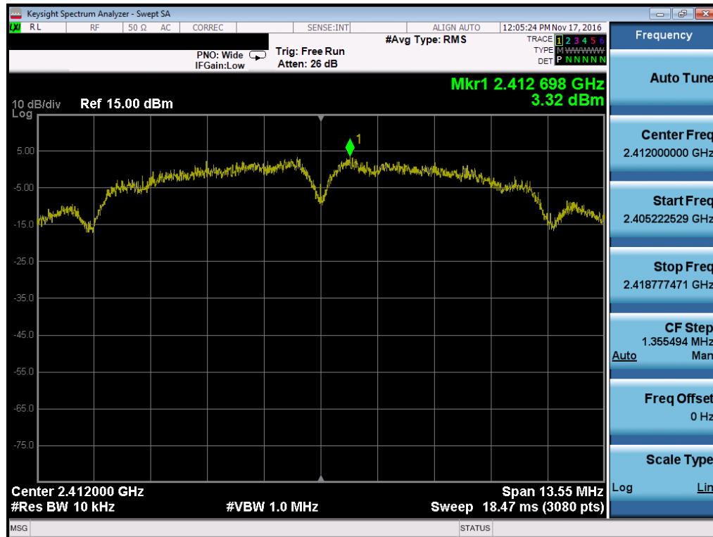
Plot 7-10. Power Spectral Density Plot (802.11b – Ch. 1)
