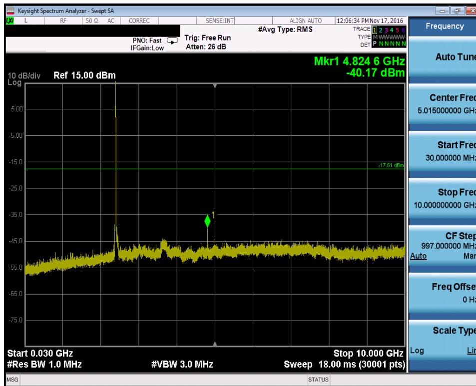
Plot 7-25. Conducted Spurious Plot (802.11b – Ch. 1)
