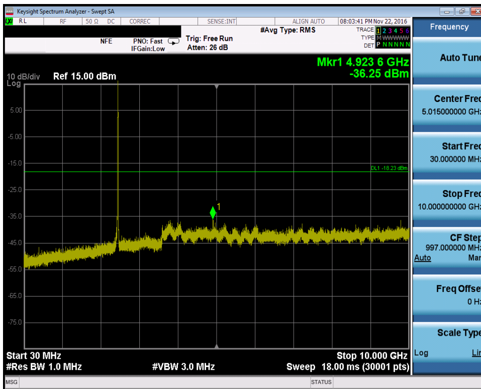
Plot 7-29. Conducted Spurious Plot (802.11b – Ch. 11)
