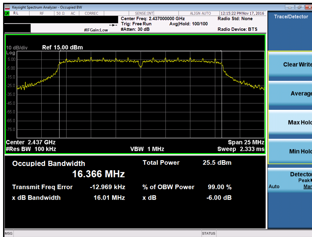
Plot 7-5. 6dB Bandwidth Plot (802.11g – Ch. 6)
