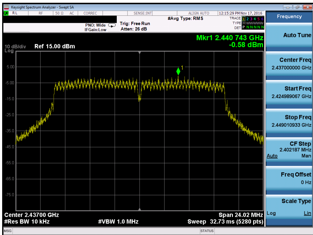
Plot 7-14. Power Spectral Density Plot (802.11g – Ch. 6)
