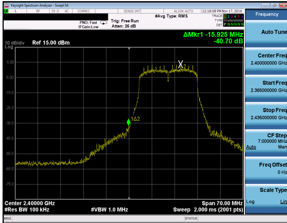
Plot 7-23. Band Edge Plot (802.11n (2.4GHz) – Ch. 1)
