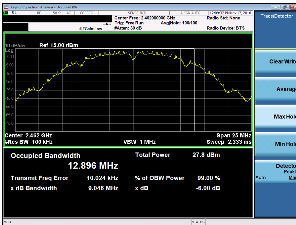
Plot 7-3. 6dB Bandwidth Plot (802.11b – Ch. 11)
