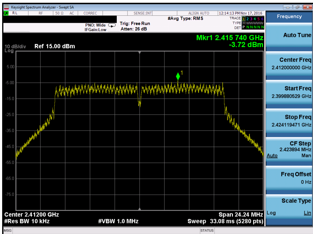
Plot 7-13. Power Spectral Density Plot (802.11g – Ch. 1)
