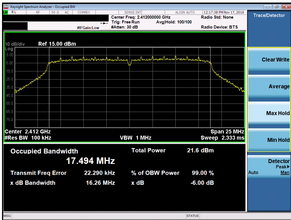
Plot 7-7. 6dB Bandwidth Plot (802.11n (2.4GHz) – Ch. 1)
