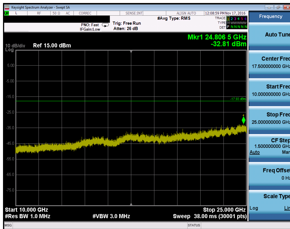
Plot 7-28. Conducted Spurious Plot (802.11b – Ch. 6)
