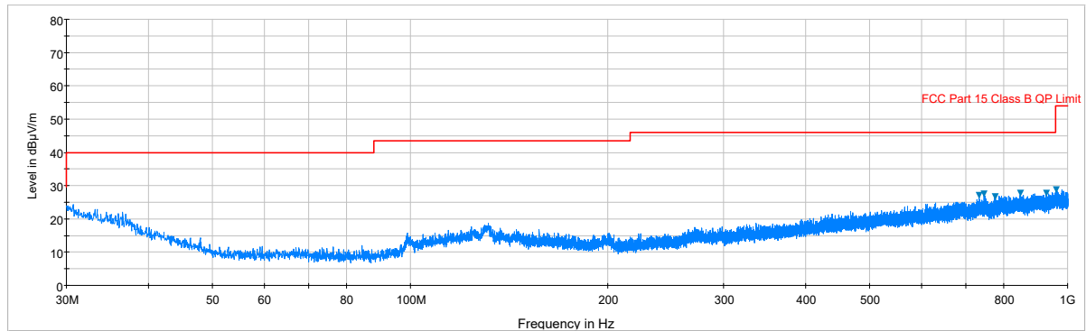
Plot 7-43. Radiated Spurious Plot below 1GHz (Pol. H)
