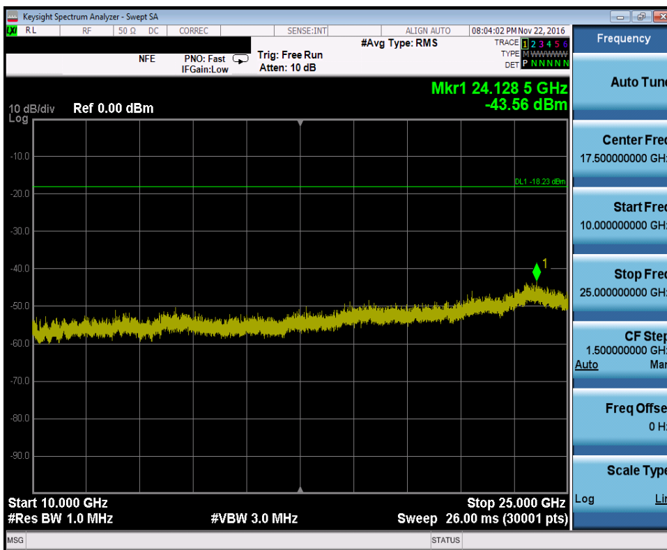
Plot 7-30. Conducted Spurious Plot (802.11b – Ch. 11)
