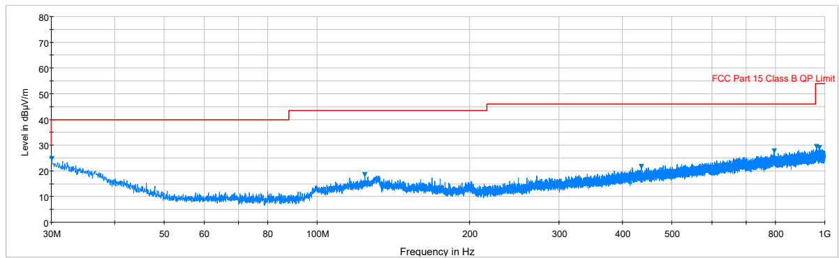
Plot 7-44. Radiated Spurious Plot below 1GHz (Pol. V)
