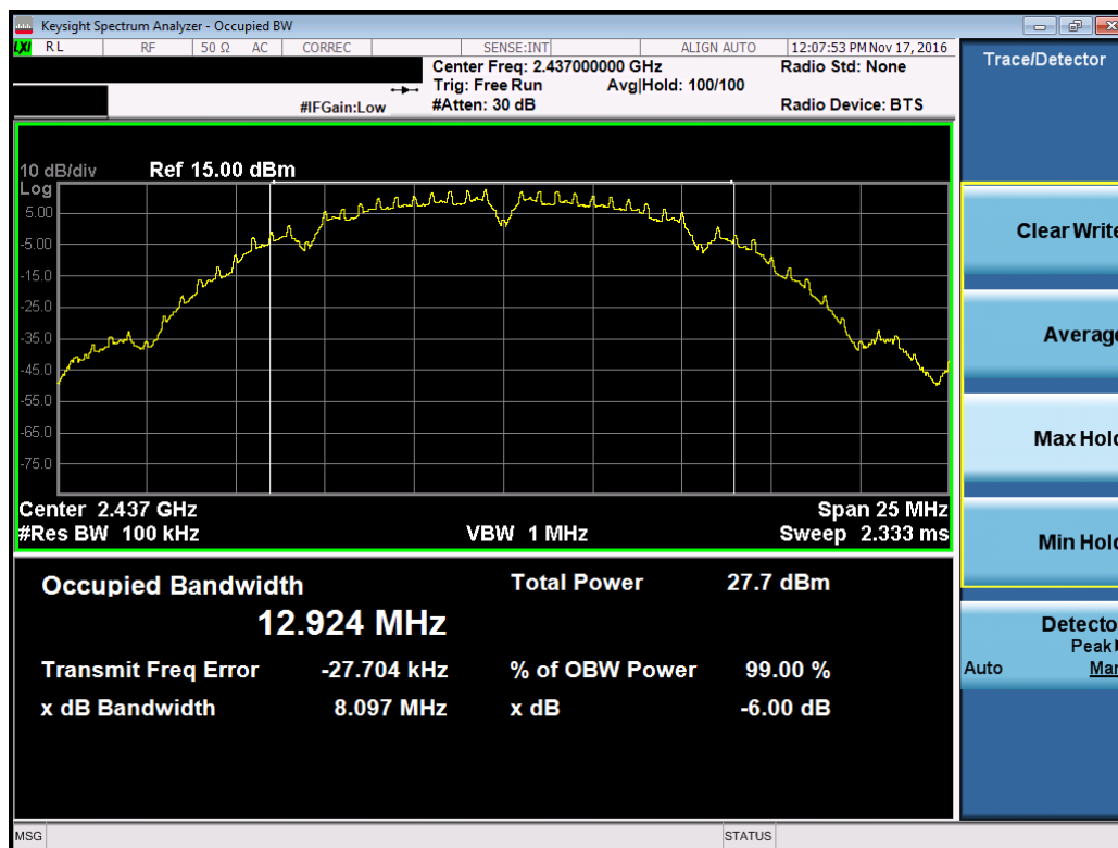
Plot 7-2. 6dB Bandwidth Plot (802.11b – Ch. 6)
