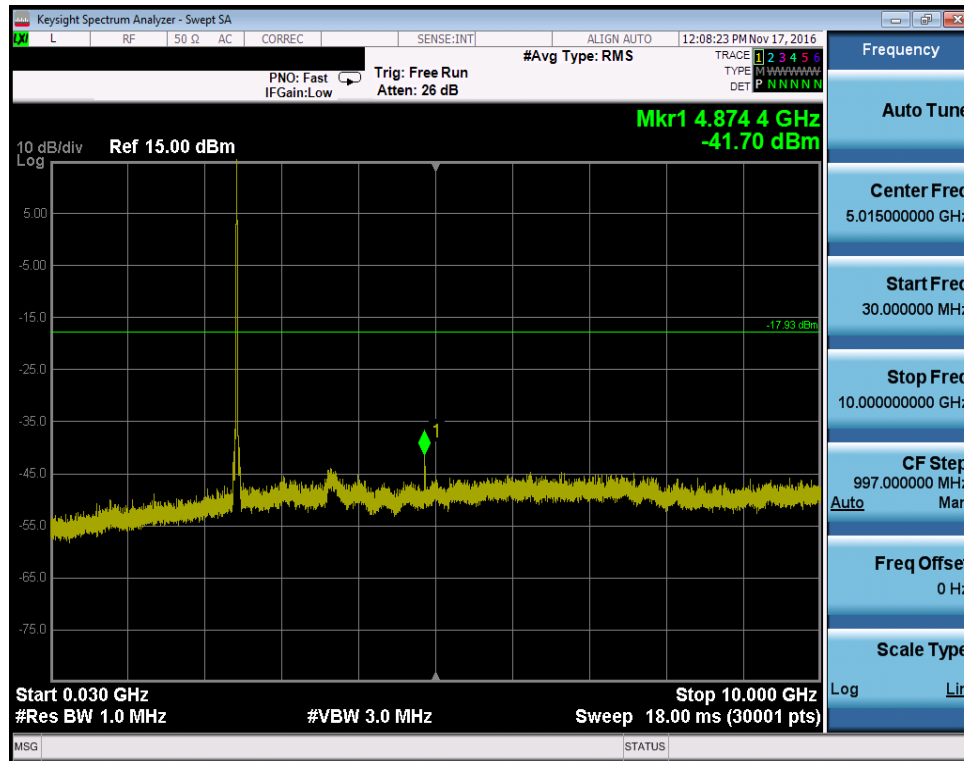
Plot 7-27. Conducted Spurious Plot (802.11b – Ch. 6)
