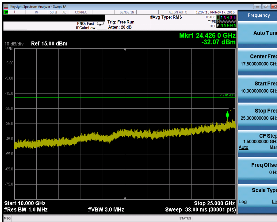
Plot 7-26. Conducted Spurious Plot (802.11b – Ch. 1)
