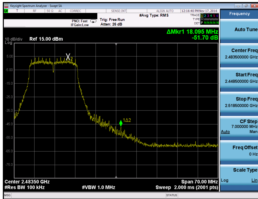
Plot 7-22. Band Edge Plot (802.11g - Ch. 11)
