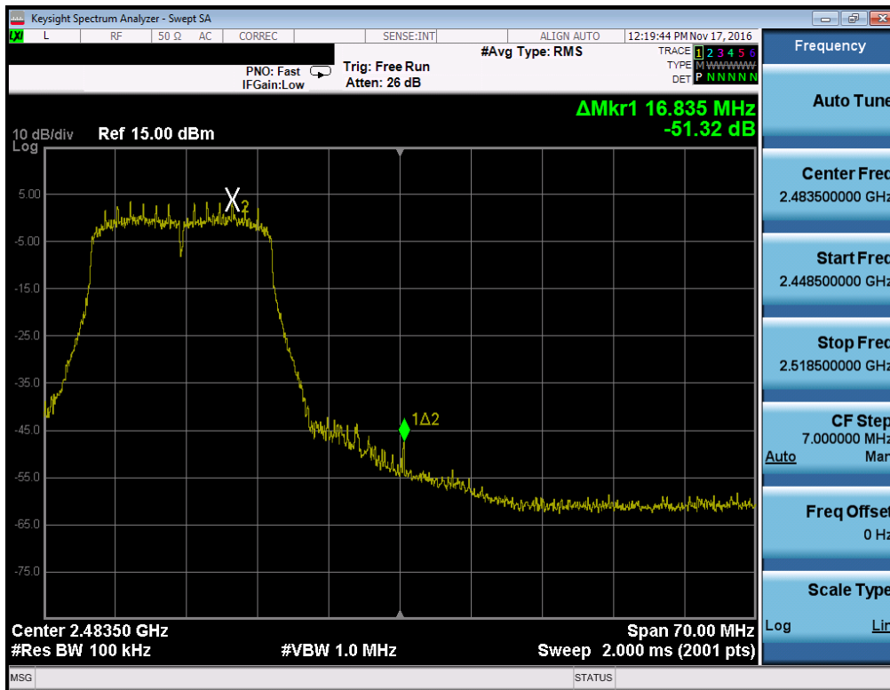
Plot 7-24. Band Edge Plot (802.11n (2.4GHz) – Ch. 11)
