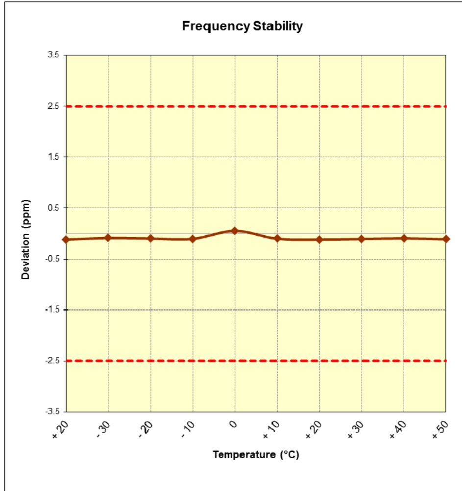
Figure 7-9. Frequency Stability Graph (PCS CDMA Mode – Ch. 600)
