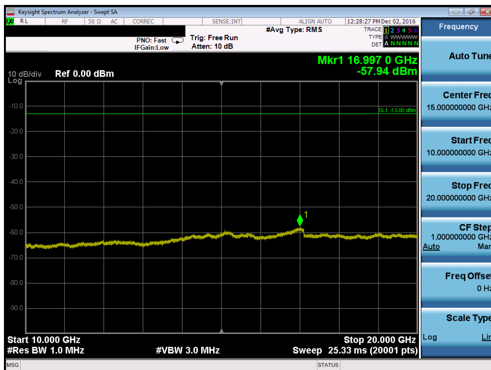
Plot 7-35. Conducted Spurious Plot (Band 4 – 20.0MHz QPSK – RB Size 1, RB Offset 0 – Low Channel)
