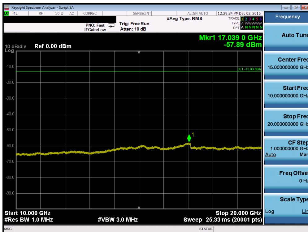
Plot 7-41. Conducted Spurious Plot (Band 4 – 20.0MHz QPSK – RB Size 1, RB Offset 0 – High Channel)
