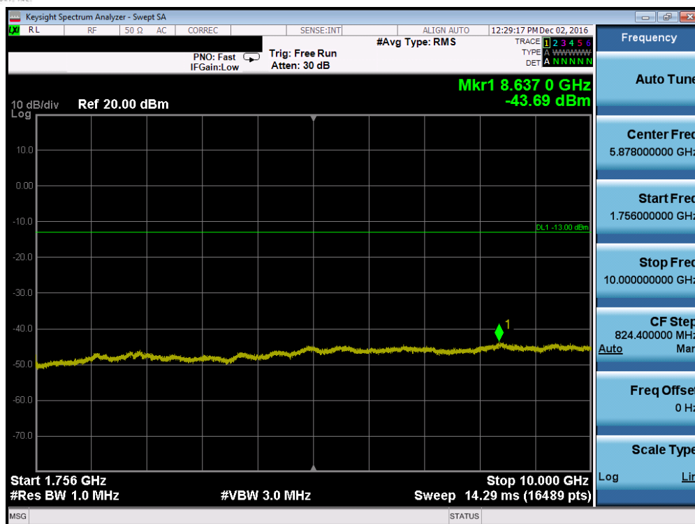
Plot 7-40. Conducted Spurious Plot (Band 4 – 20.0MHz QPSK – RB Size 1, RB Offset 0 – High Channel)
