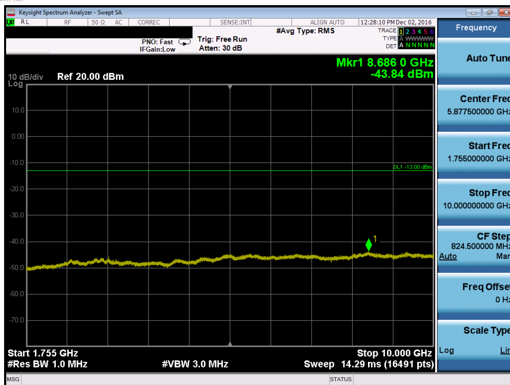
Plot 7-34. Conducted Spurious Plot (Band 4 – 20.0MHz QPSK – RB Size 1, RB Offset 0 – Low Channel)
