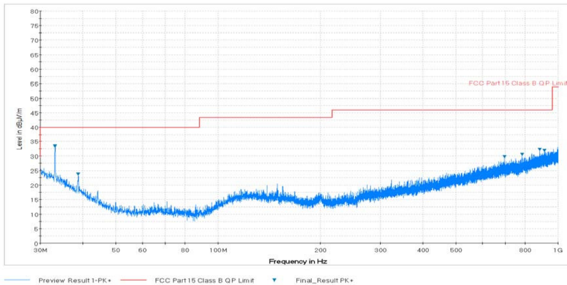
Plot 7-53. Radiated Spurious Plot below 1GHz (Pol. V)
