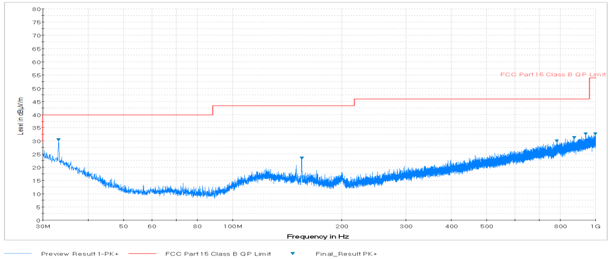
Plot 7-43. Radiated Spurious Plot below 1GHz (Pol. H)
