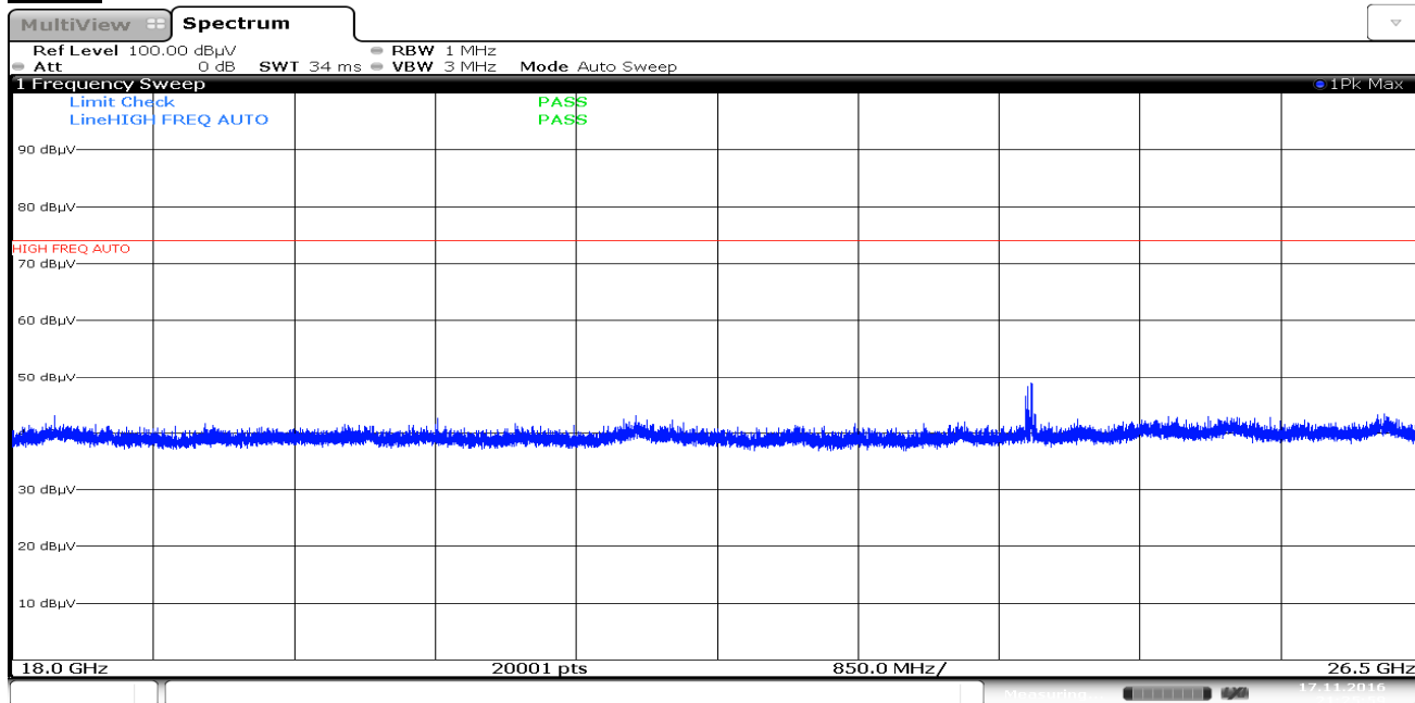
Plot 7-37. Radiated Spurious Plot above 18GHz (Pol. H)
