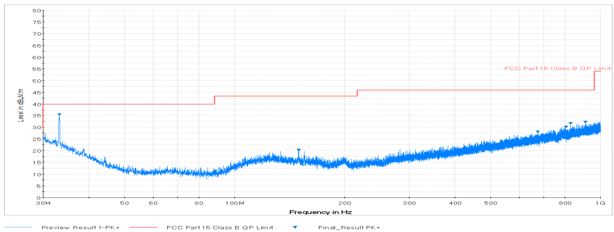
Plot 7-44. Radiated Spurious Plot below 1GHz (Pol. V)
