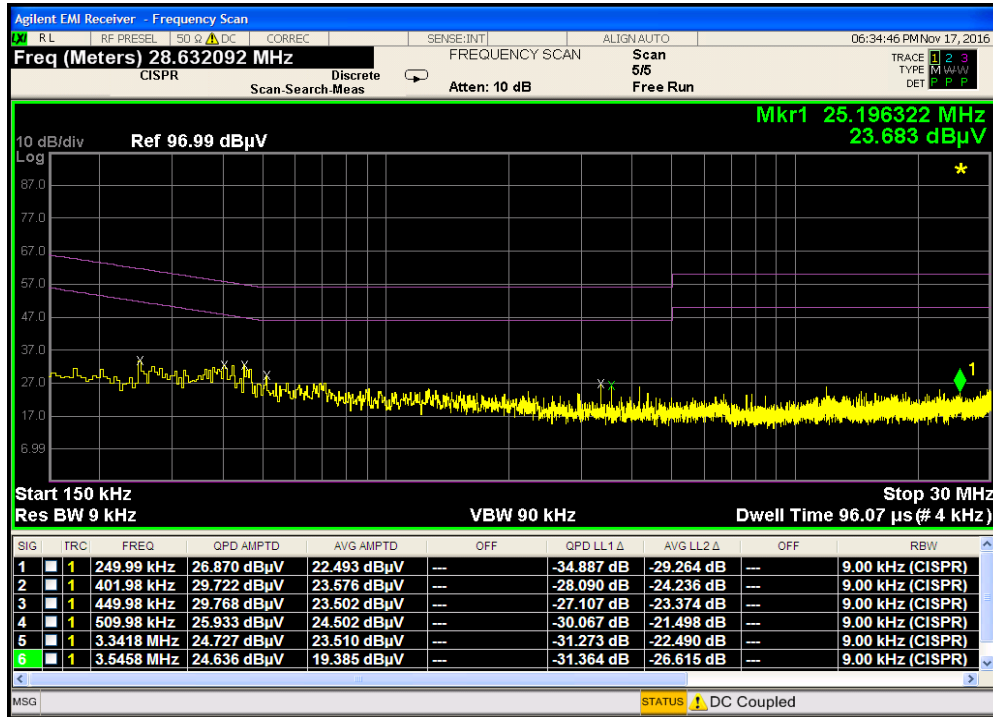
Plot 7-45. Line Conducted Plot with 802.11b (L1)
