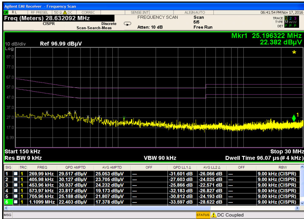
Plot 7-46. Line Conducted Plot with 802.11b (N)
