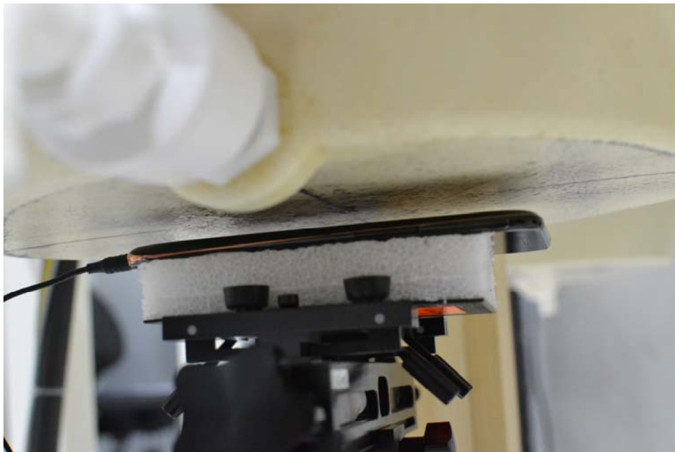
SAR Test Setup Photo 6 – Back Side at 1.0 cm with headphones
