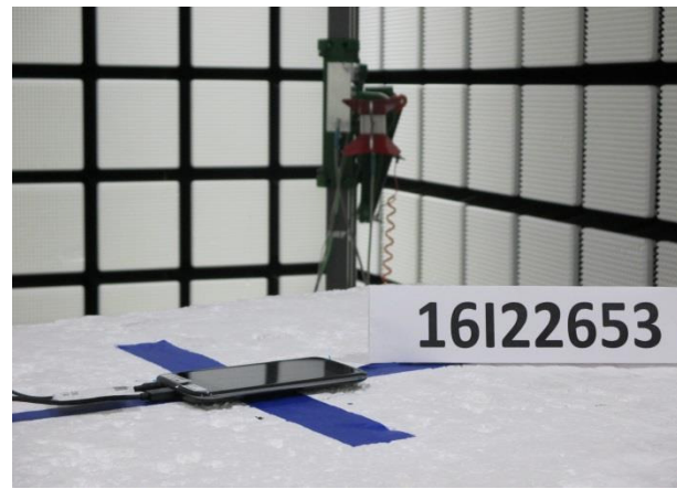
X-AXIS POSITION
