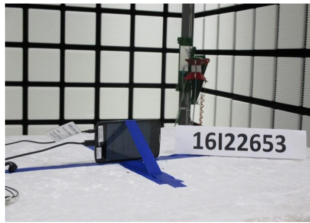
Y-AXIS POSITION
