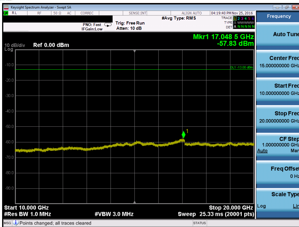
Plot 7-73. Conducted Spurious Plot (Band 2 – 3.0MHz QPSK – RB Size 1, RB Offset 0 – Mid Channel)
