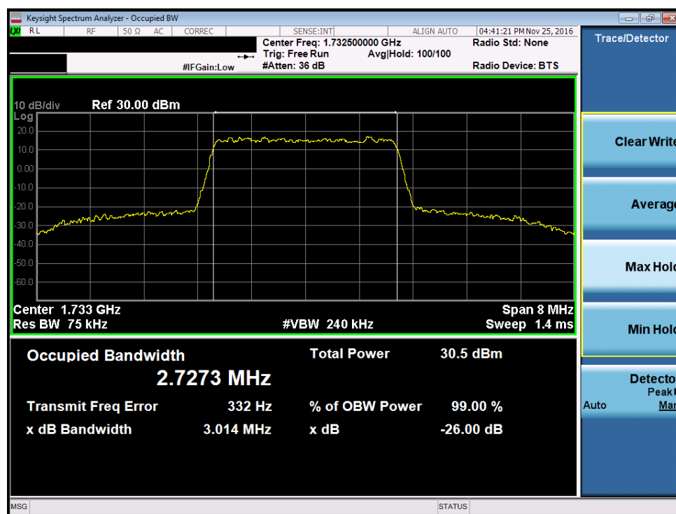
Plot 7-20. Occupied Bandwidth Plot (Band 4 – 3.0MHz QPSK – RB Size 15)
