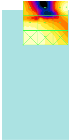
Figure 10-1 Sample E-field Scan Overlay (T-Coil Centered scan area pictured. See Test Setup Photographs for actual WD overlay and Acoustic Centered scan area.)
