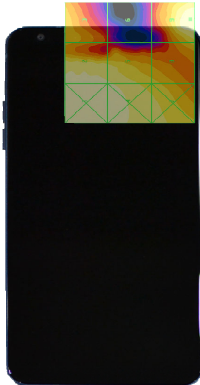
Figure 17-4 E-Field WD Scan overlay (T-Coil Centered scan area pictured)
