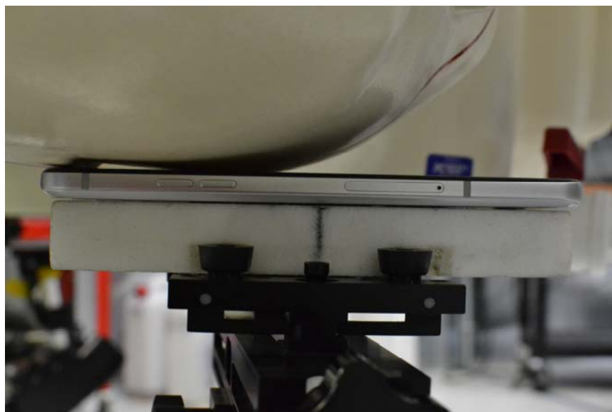
SAR Test Setup Photo 1 – Right Cheek
