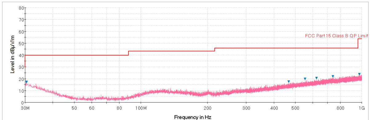
Plot 7-11. Radiated Spurious Plot below 1GHz (Pol. H)
