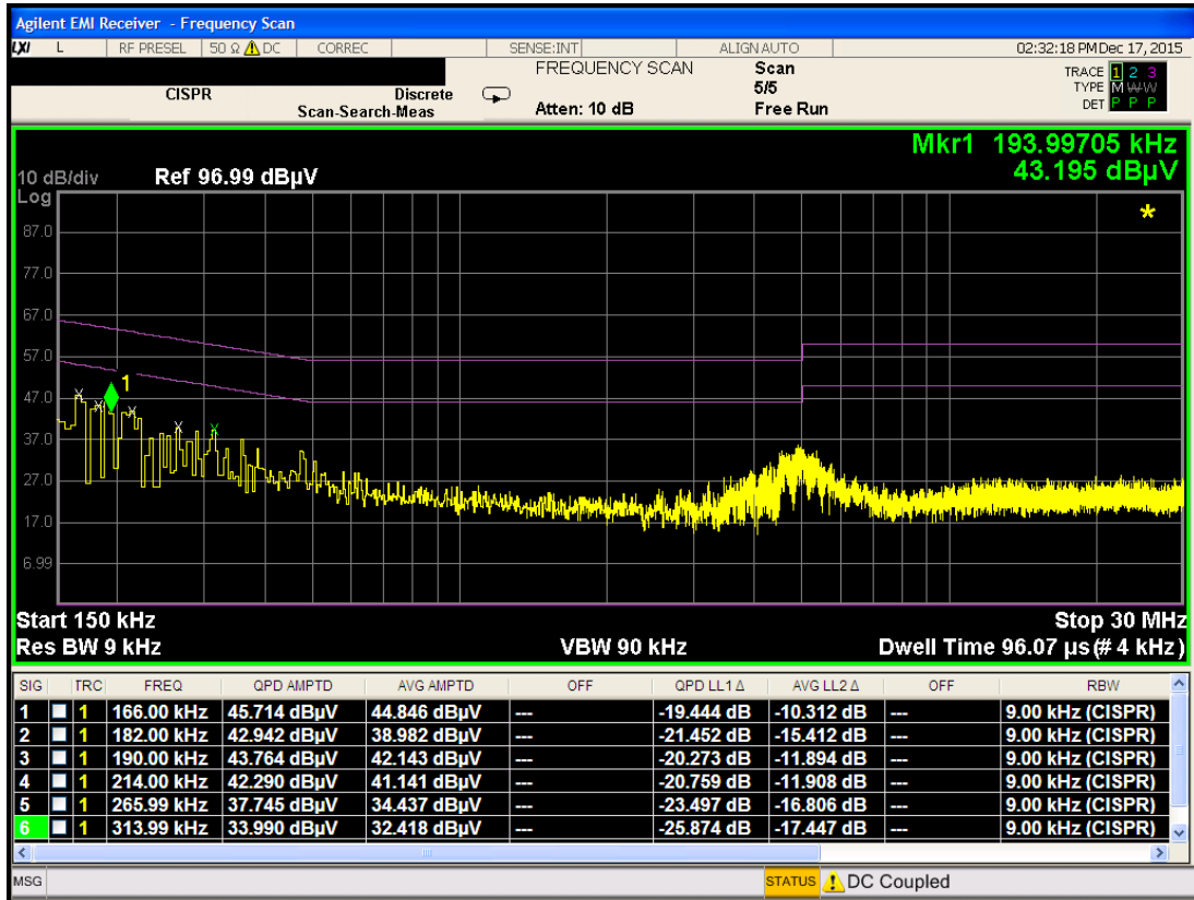
Plot 7-46. Line Conducted Plot with 802.11b (N)
