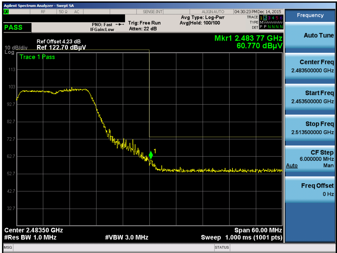
Plot 7-42. Radiated Restricted Upper Band Edge Measurement (Peak)
