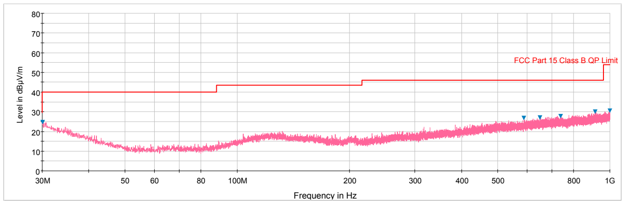
Plot 7-44. Radiated Spurious Plot below 1GHz (Pol. V)
