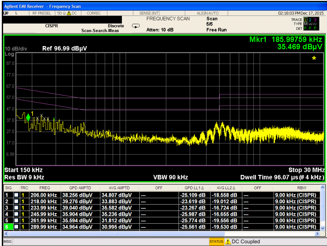
Plot 7-45. Line Conducted Plot with 802.11b (L1)
