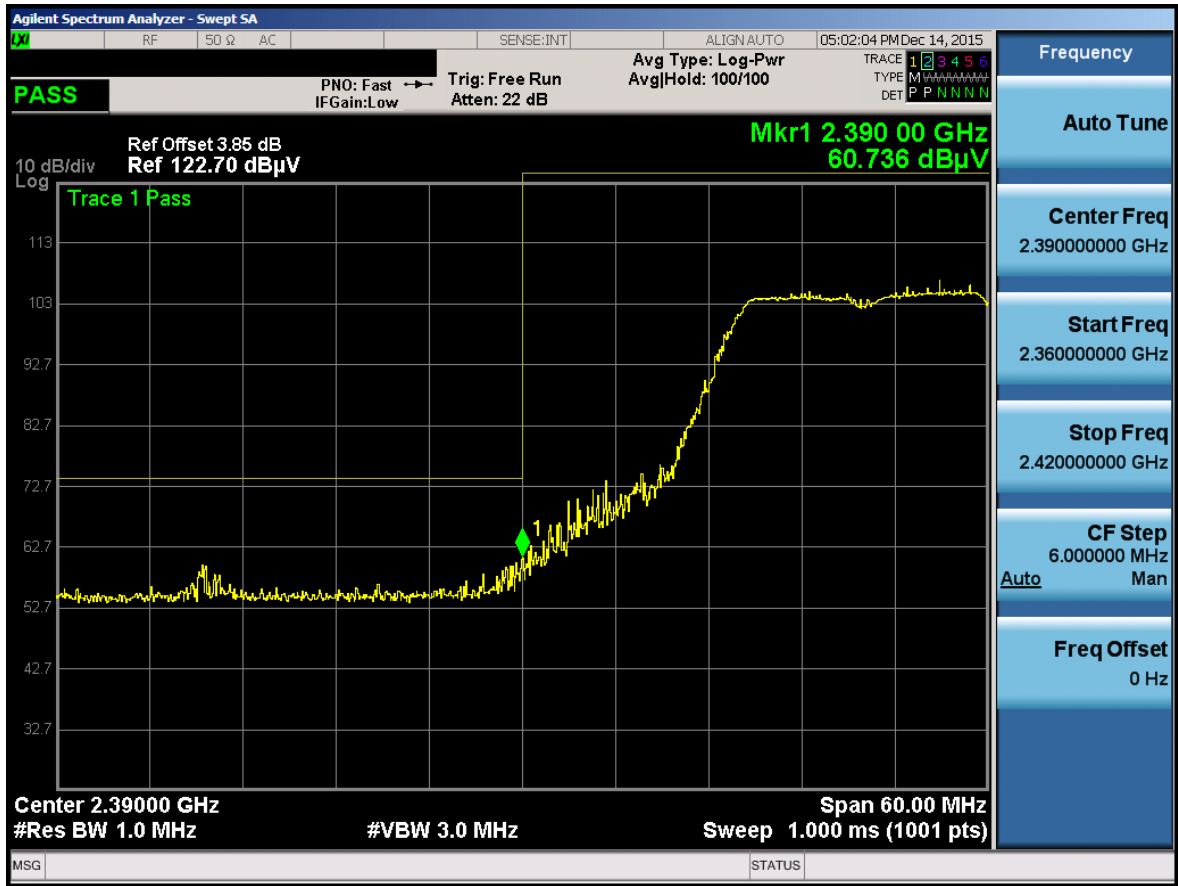
Plot 7-40. Radiated Restricted Lower Band Edge Measurement (Peak)
