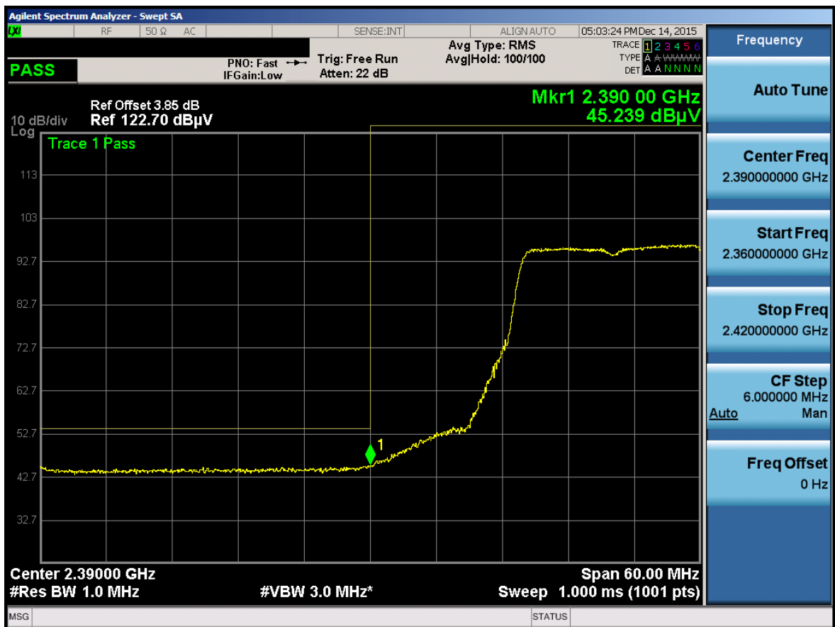
Plot 7-39. Radiated Restricted Lower Band Edge Measurement (Average)
