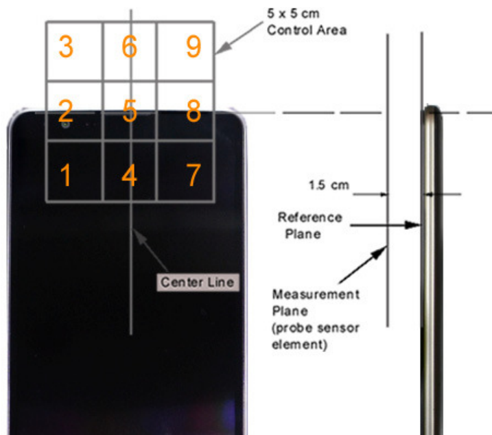
Figure 18-3 5x5 Scan grid above WD (Acoustic Centered Scan Pictured)
