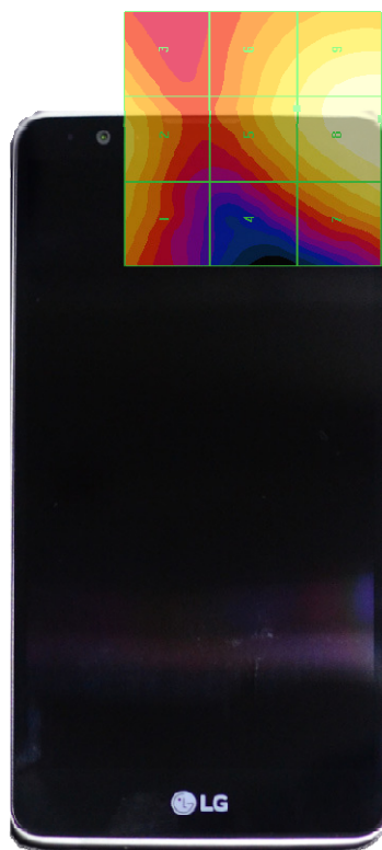
Figure 18-4 E-Field WD Scan overlay (T-Coil Centered Scan Pictured)
