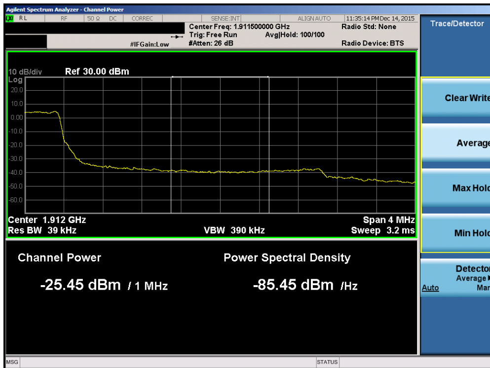
Plot 7-95. Upper Extended Band Edge Plot (Band 2 – 3.0MHz QPSK – RB Size 15)
