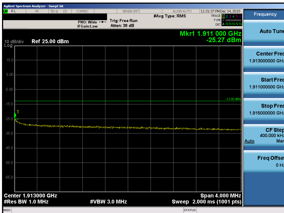
Plot 7-103. Upper Extended Band Edge Plot (Band 2 – 10.0MHz QPSK – RB Size 50)
