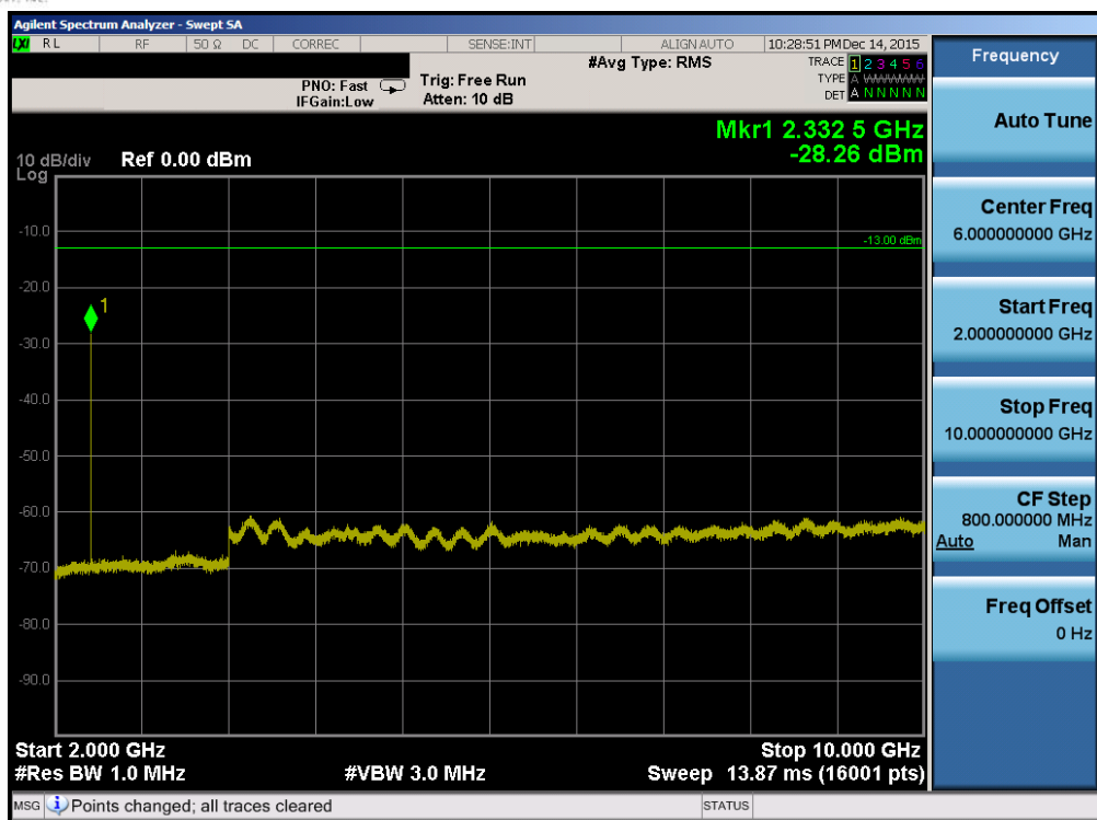
Plot 7-31. Conducted Spurious Plot (Band 13 – 5.0MHz QPSK – RB Size 1, RB Offset 0 – Low Channel)
