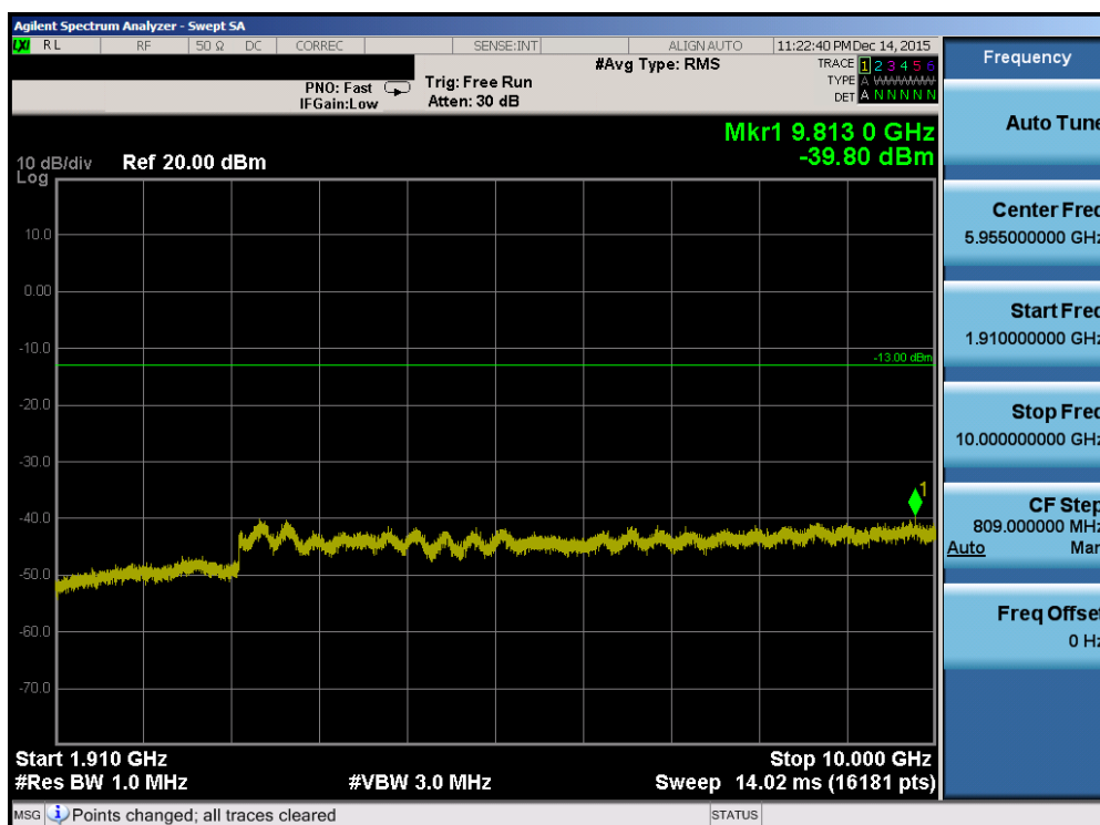
Plot 7-48. Conducted Spurious Plot (Band 2 – 5.0MHz QPSK – RB Size 1, RB Offset 0 – Low Channel)
