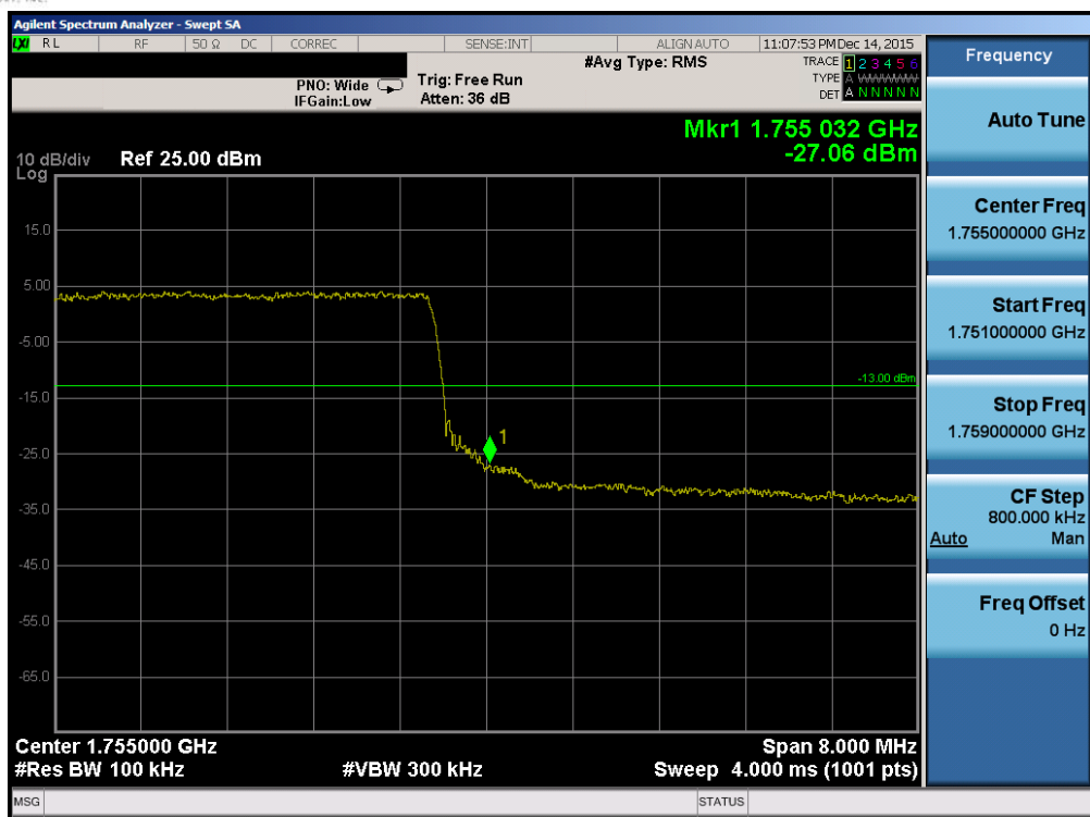
Plot 7-78. Upper Band Edge Plot (Band 4 – 10.0MHz QPSK – RB Size 50)
