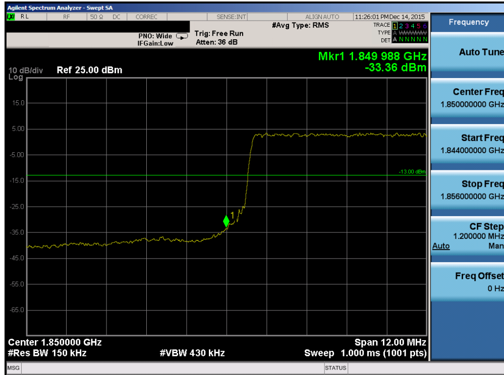
Plot 7-104. Lower Band Edge Plot (Band 2 – 15.0MHz QPSK – RB Size 75)
