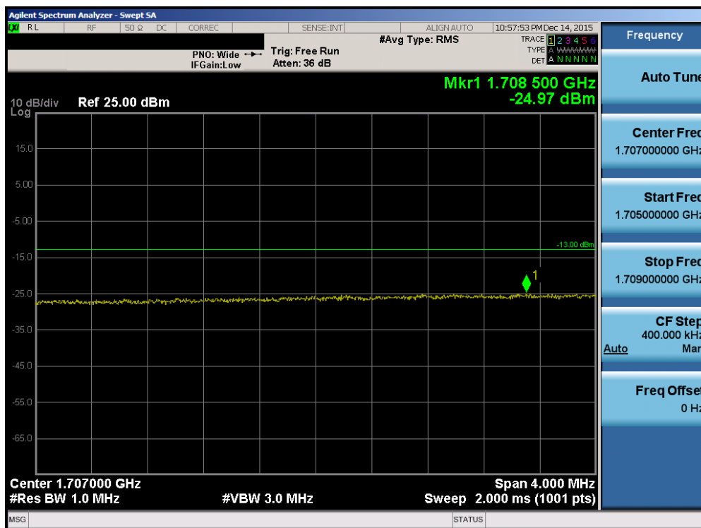
Plot 7-85. Lower Extended Band Edge Plot (Band 4 – 20.0MHz QPSK – RB Size 100)
