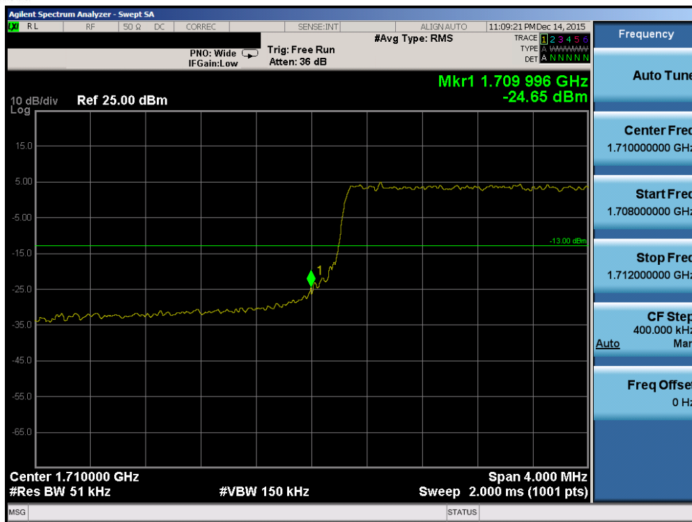
Plot 7-72. Lower Band Edge Plot (Band 4 – 5.0MHz QPSK – RB Size 25)
