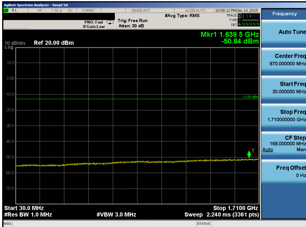
Plot 7-44. Conducted Spurious Plot (Band 4 – 3.0MHz QPSK – RB Size 1, RB Offset 0 – High Channel)
