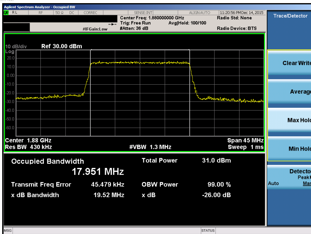
Plot 7-27. Occupied Bandwidth Plot (Band 2 – 20.0MHz QPSK – RB Size 100)
