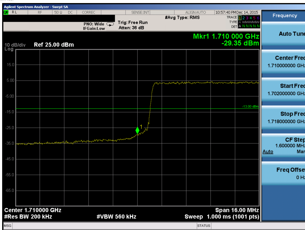
Plot 7-84. Lower Band Edge Plot (Band 4 – 20.0MHz QPSK – RB Size 100)
