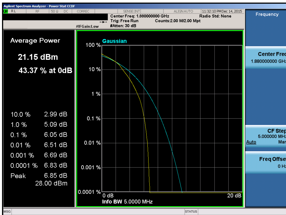
Plot 7-117. PAR Plot (Band 2 – 5.0MHz 16-QAM – RB Size 25)
