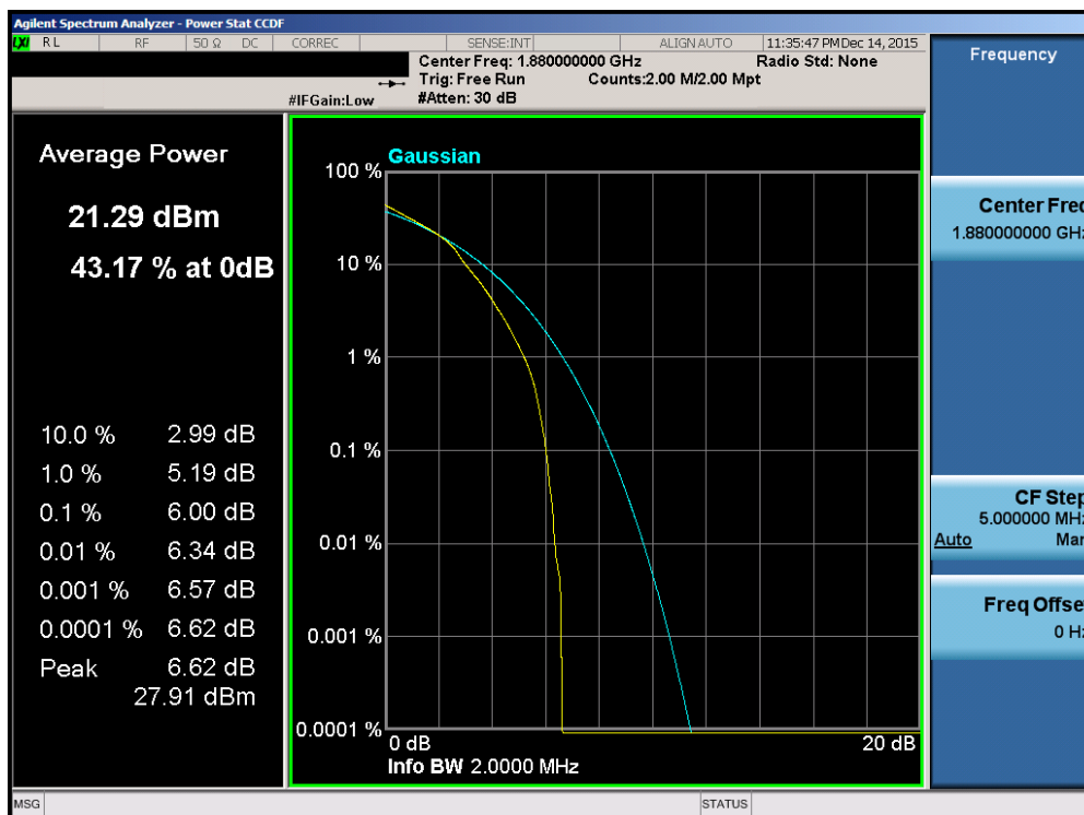
Plot 7-113. PAR Plot (Band 2 – 1.4MHz 16-QAM – RB Size 6)
