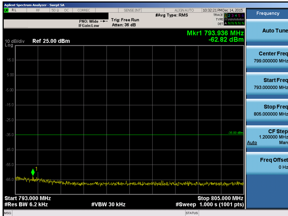
Plot 7-59. Upper Emission Mask Edge Plot (Band 13 – 5.0MHz QPSK – RB Size 25)
