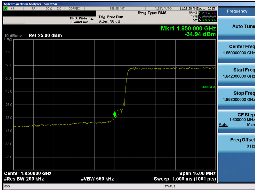
Plot 7-108. Lower Band Edge Plot (Band 2 – 20.0MHz QPSK – RB Size 100)
