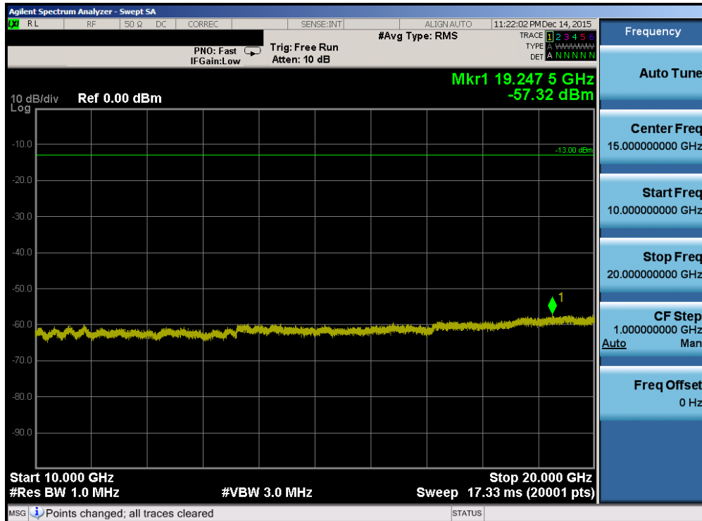
Plot 7-52. Conducted Spurious Plot (Band 2 – 5.0MHz QPSK – RB Size 1, RB Offset 0 – Mid Channel)
