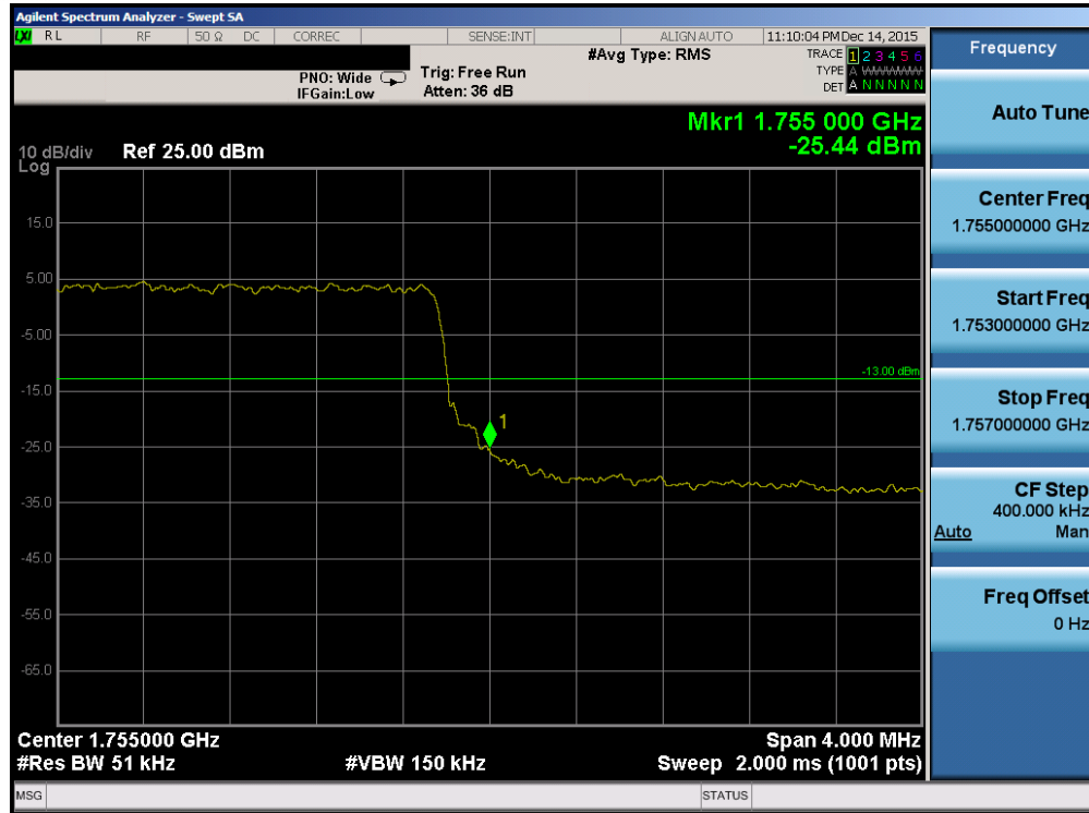
Plot 7-74. Upper Band Edge Plot (Band 4 – 5.0MHz QPSK – RB Size 25)
