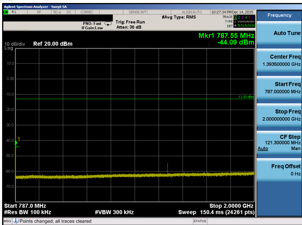
Plot 7-33. Conducted Spurious Plot (Band 13 – 5.0MHz QPSK – RB Size 1, RB Offset 0 – Mid Channel)
