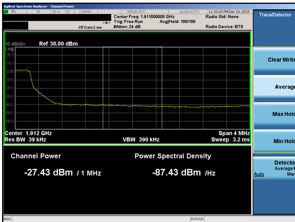
Plot 7-99. Upper Extended Band Edge Plot (Band 2 – 5.0MHz QPSK – RB Size 25)
