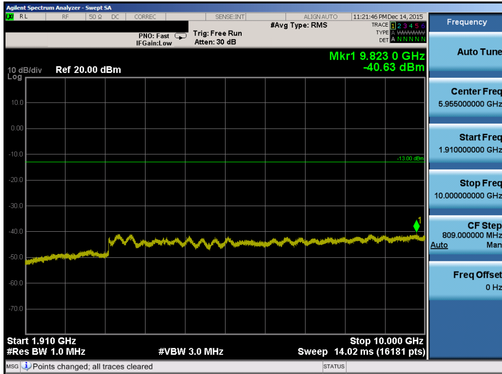
Plot 7-51. Conducted Spurious Plot (Band 2 – 5.0MHz QPSK – RB Size 1, RB Offset 0 – Mid Channel)
