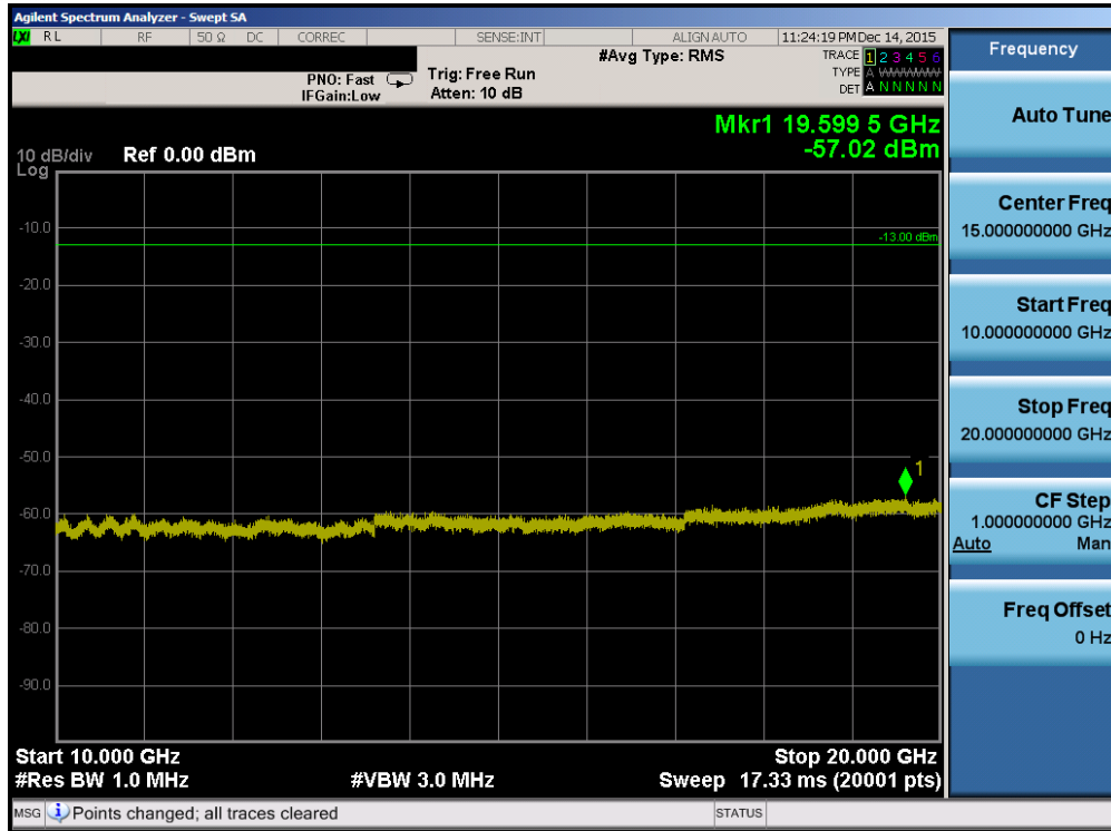
Plot 7-55. Conducted Spurious Plot (Band 2 – 5.0MHz QPSK – RB Size 1, RB Offset 0 – High Channel)
