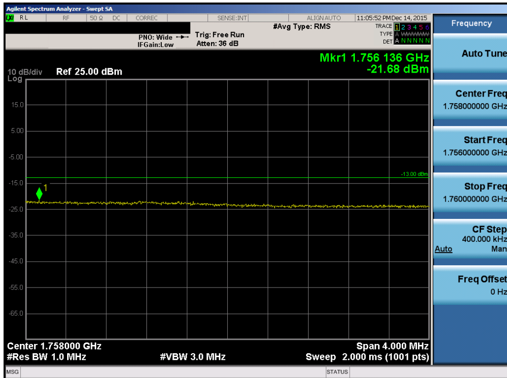
Plot 7-83. Upper Extended Band Edge Plot (Band 4 – 15.0MHz QPSK – RB Size 75)
