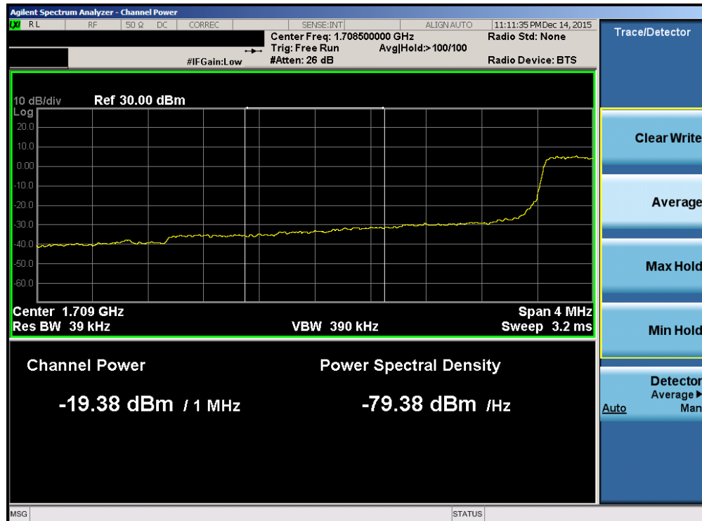
Plot 7-69. Lower Extended Band Edge Plot (Band 4 – 3.0MHz QPSK – RB Size 15)
