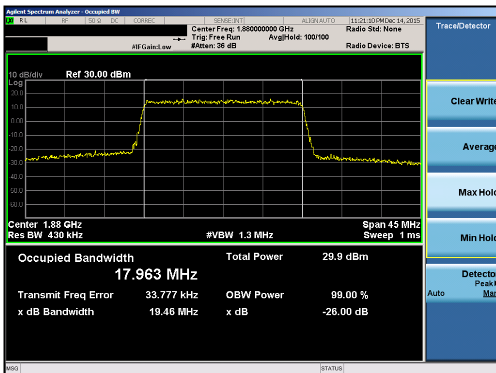
Plot 7-28. Occupied Bandwidth Plot (Band 2 – 20.0MHz 16-QAM – RB Size 100)
