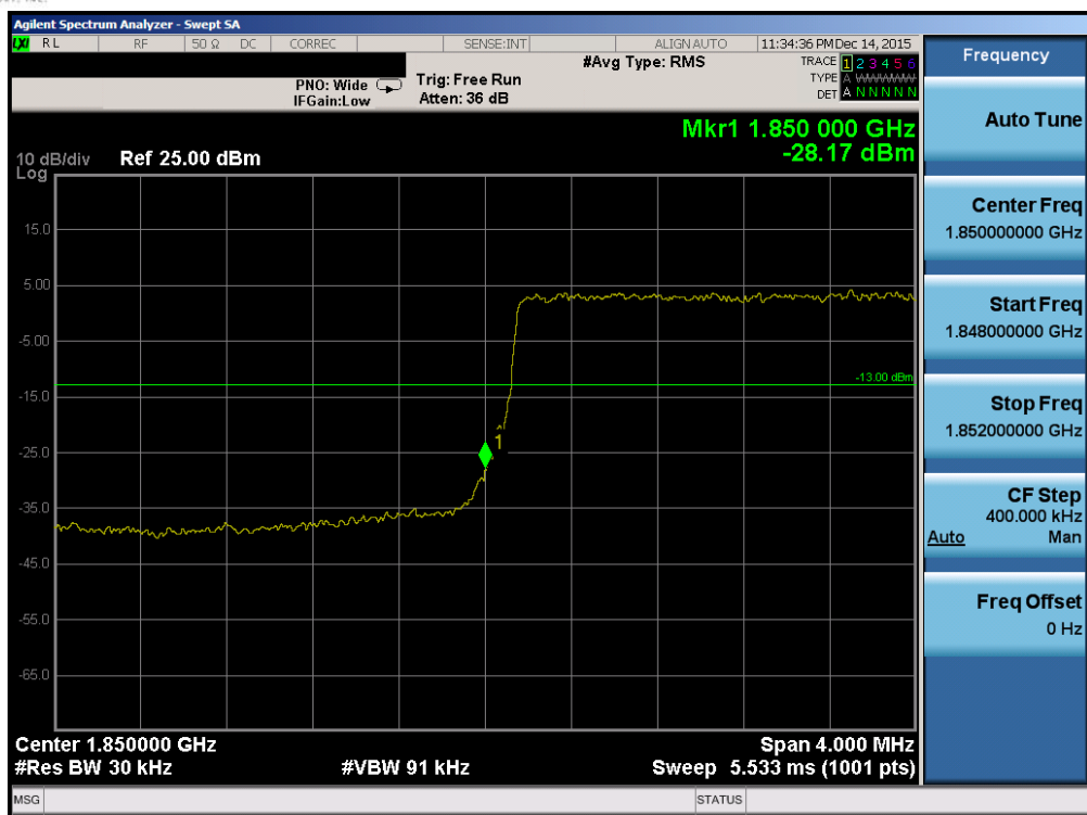
Plot 7-92. Lower Band Edge Plot (Band 2 – 3.0MHz QPSK – RB Size 15)
