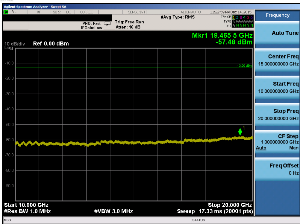
Plot 7-49. Conducted Spurious Plot (Band 2 – 5.0MHz QPSK – RB Size 1, RB Offset 0 – Low Channel)
