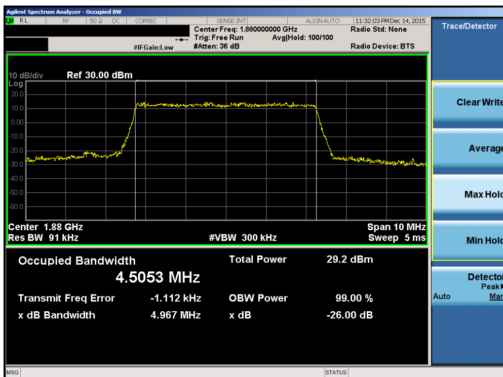
Plot 7-22. Occupied Bandwidth Plot (Band 2 – 5.0MHz 16-QAM – RB Size 25)
