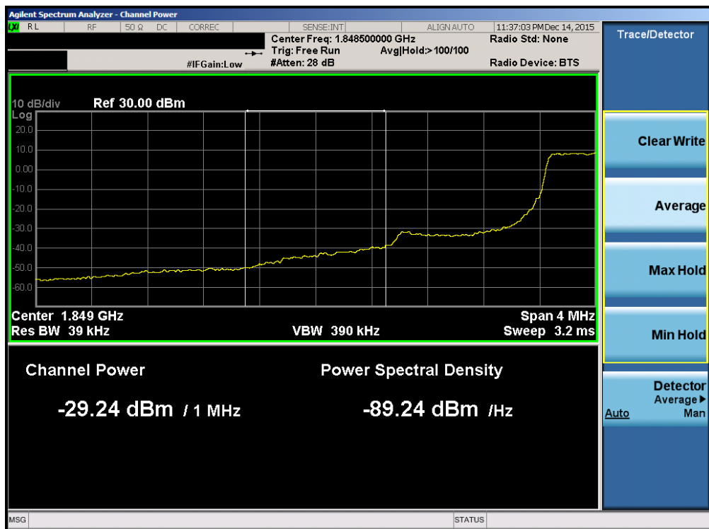
Plot 7-89. Lower Extended Band Edge Plot (Band 2 – 1.4MHz QPSK – RB Size 6)
