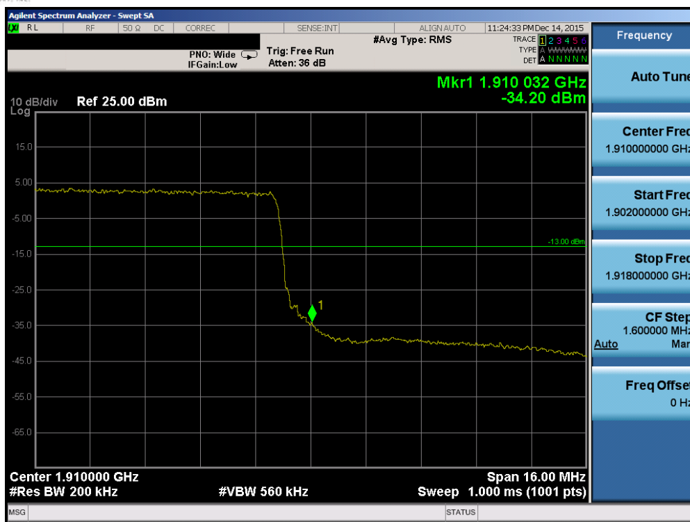
Plot 7-110. Upper Band Edge Plot (Band 2 – 20.0MHz QPSK – RB Size 100)
