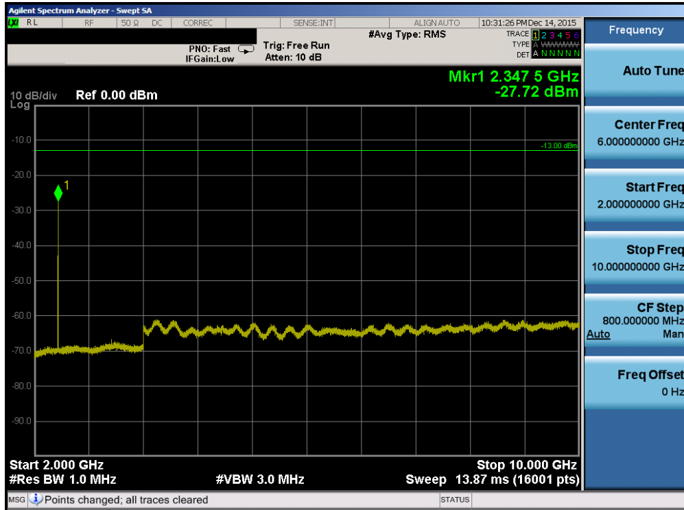
Plot 7-37. Conducted Spurious Plot (Band 13 – 5.0MHz QPSK – RB Size 1, RB Offset 0 – High Channel)
