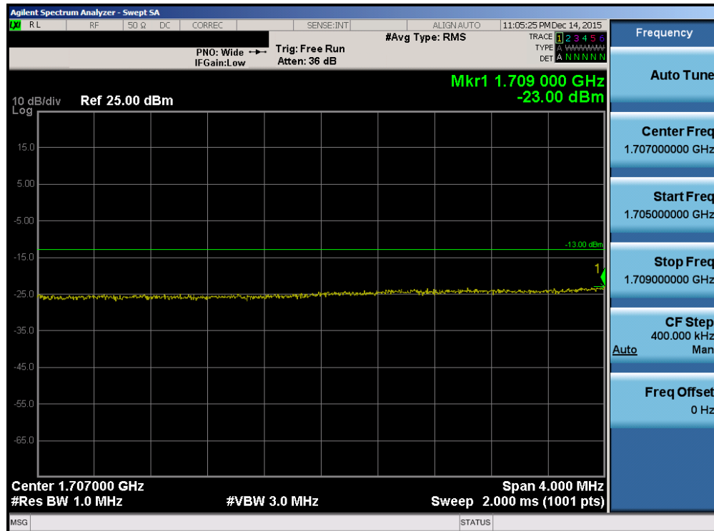
Plot 7-81. Lower Extended Band Edge Plot (Band 4 – 15.0MHz QPSK – RB Size 75)
