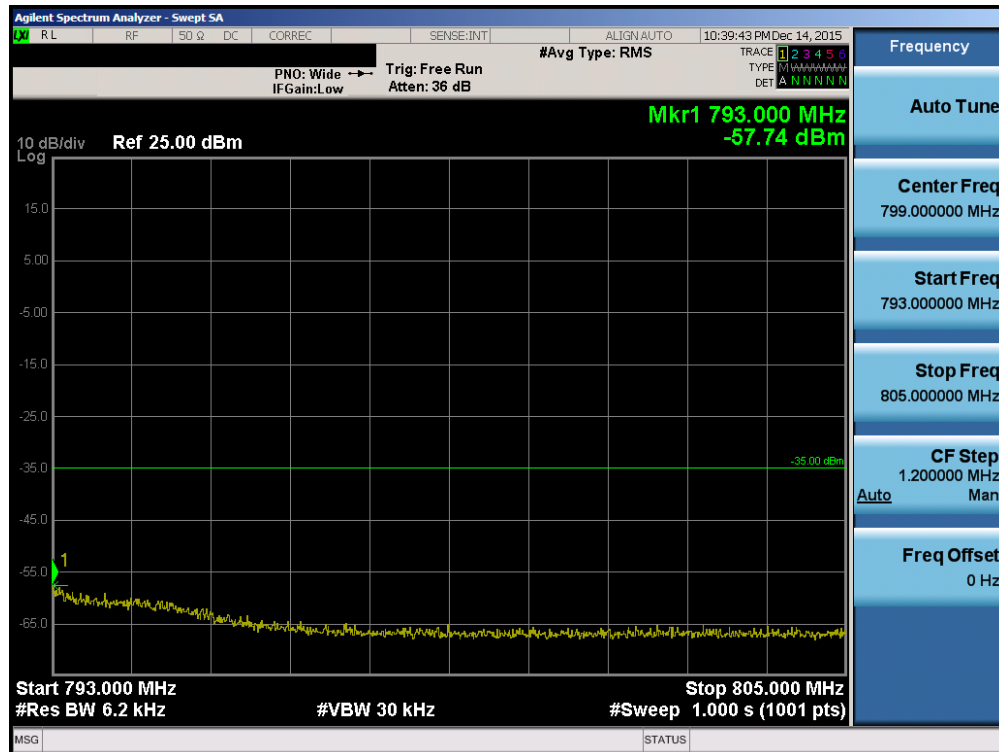
Plot 7-63. Upper Emission Mask Edge Plot (Band 13 – 10.0MHz QPSK – RB Size 50)
