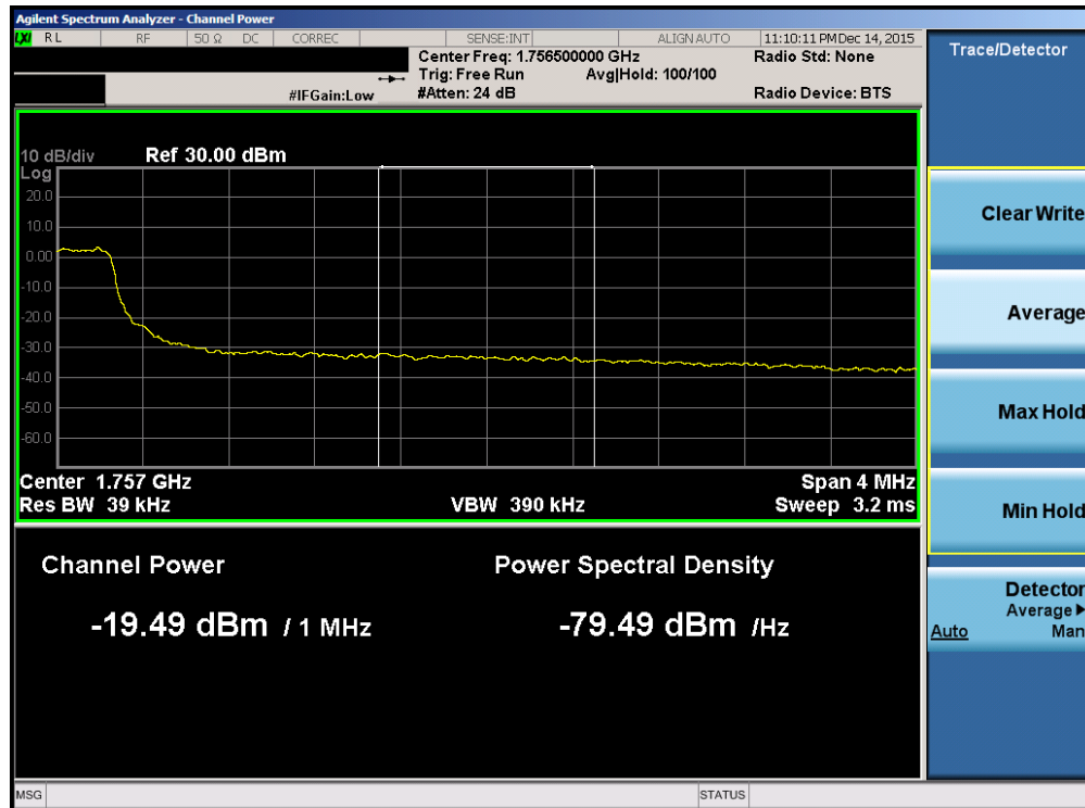
Plot 7-75. Upper Extended Band Edge Plot (Band 4 – 5.0MHz QPSK – RB Size 25)
