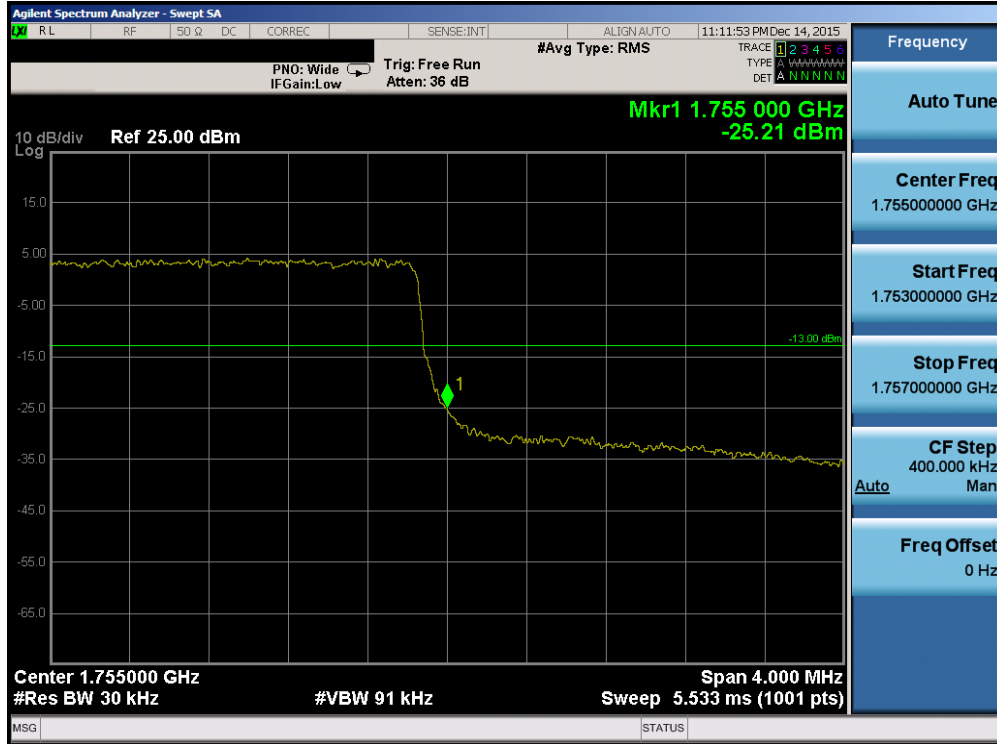
Plot 7-70. Upper Band Edge Plot (Band 4 – 3.0MHz QPSK – RB Size 15)
