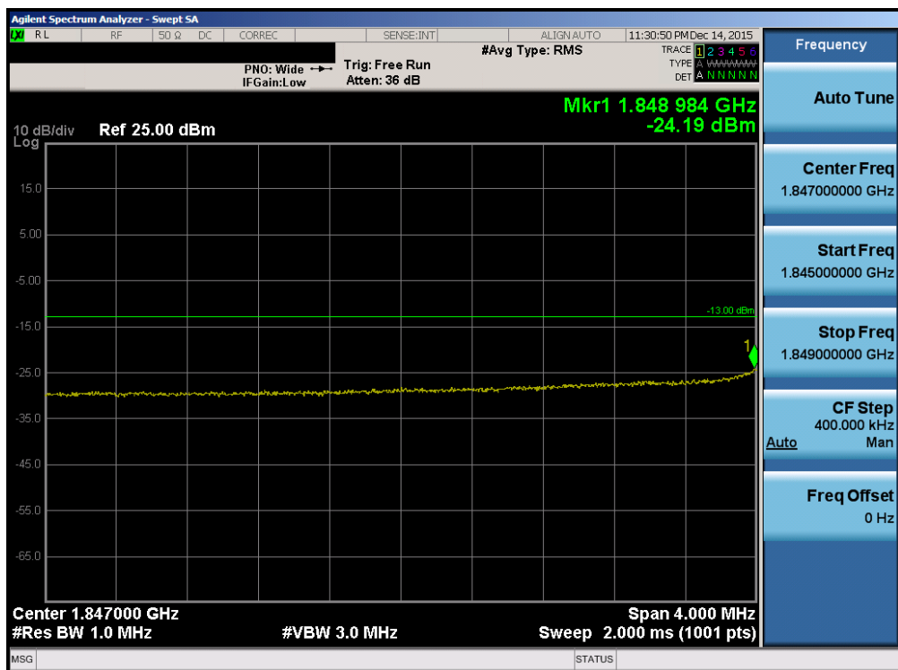
Plot 7-101. Lower Extended Band Edge Plot (Band 2 – 10.0MHz QPSK – RB Size 50)
