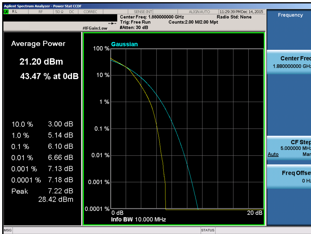
Plot 7-119. PAR Plot (Band 2 – 10.0MHz 16-QAM – RB Size 50)
