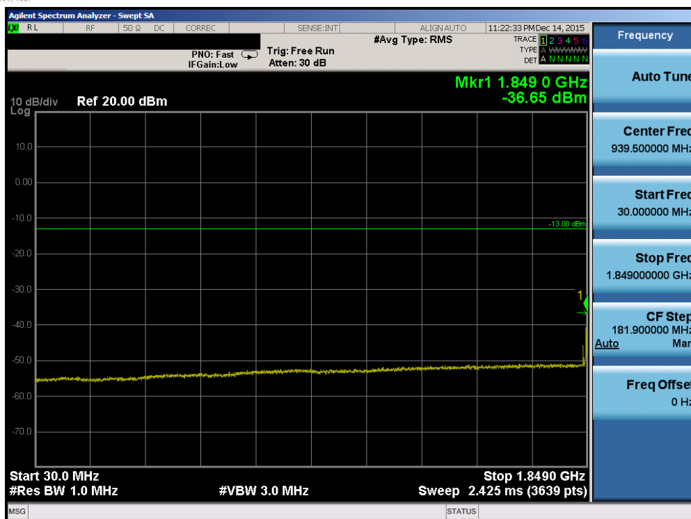
Plot 7-47. Conducted Spurious Plot (Band 2 – 5.0MHz QPSK – RB Size 1, RB Offset 0 – Low Channel)
