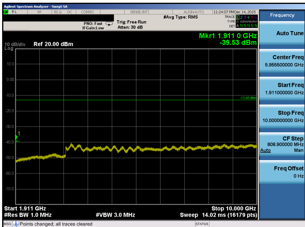
Plot 7-54. Conducted Spurious Plot (Band 2 – 5.0MHz QPSK – RB Size 1, RB Offset 0 – High Channel)
