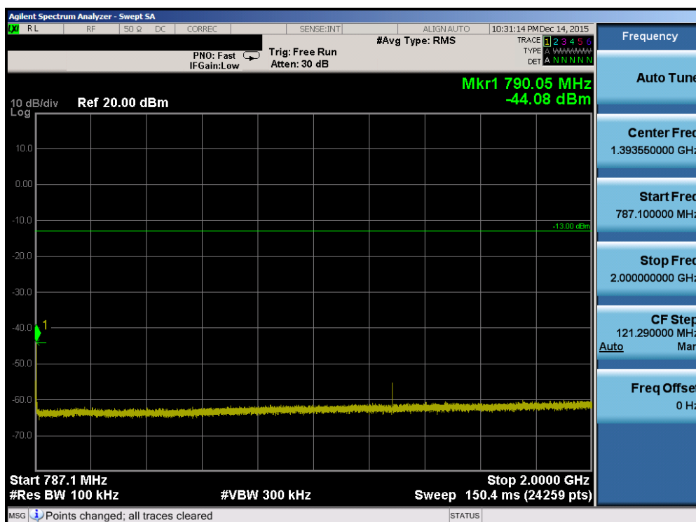
Plot 7-36. Conducted Spurious Plot (Band 13 – 5.0MHz QPSK – RB Size 1, RB Offset 0 – High Channel)
