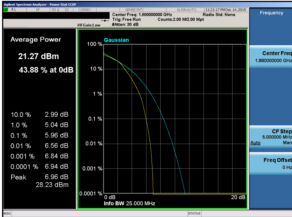
Plot 7-123. PAR Plot (Band 2 – 20.0MHz 16-QAM – RB Size 100)
