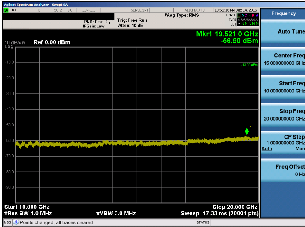
Plot 7-43. Conducted Spurious Plot (Band 4 – 3.0MHz QPSK – RB Size 1, RB Offset 0 – Mid Channel)
