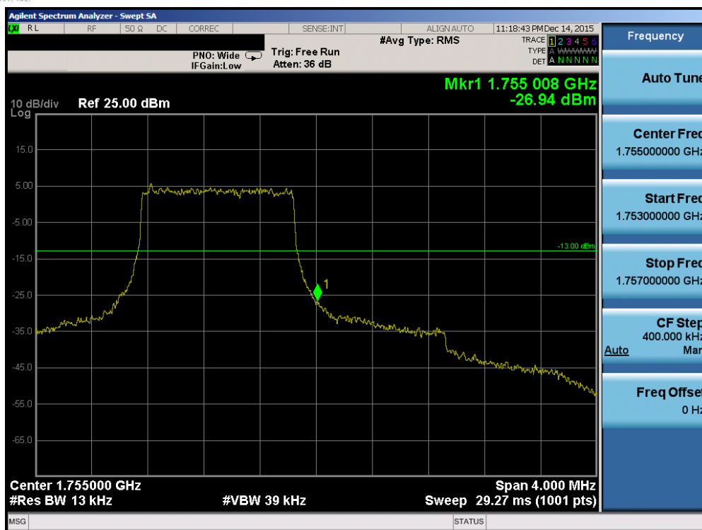
Plot 7-66. Upper Band Edge Plot (Band 4 – 1.4MHz QPSK – RB Size 6)
