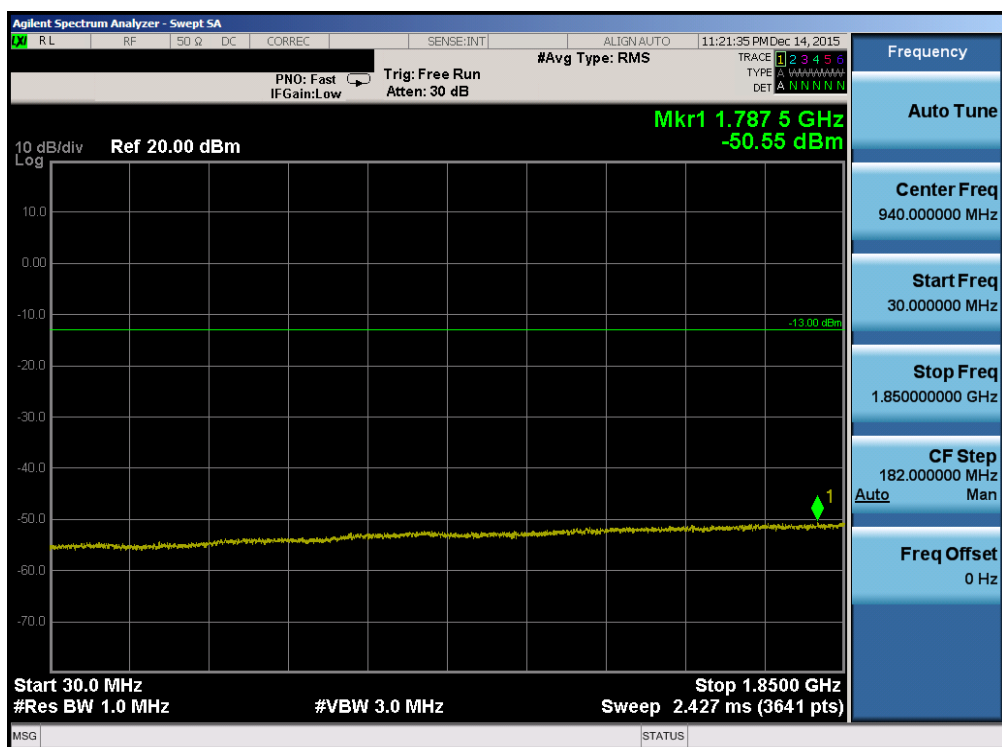
Plot 7-50. Conducted Spurious Plot (Band 2 – 5.0MHz QPSK – RB Size 1, RB Offset 0 – Mid Channel)
