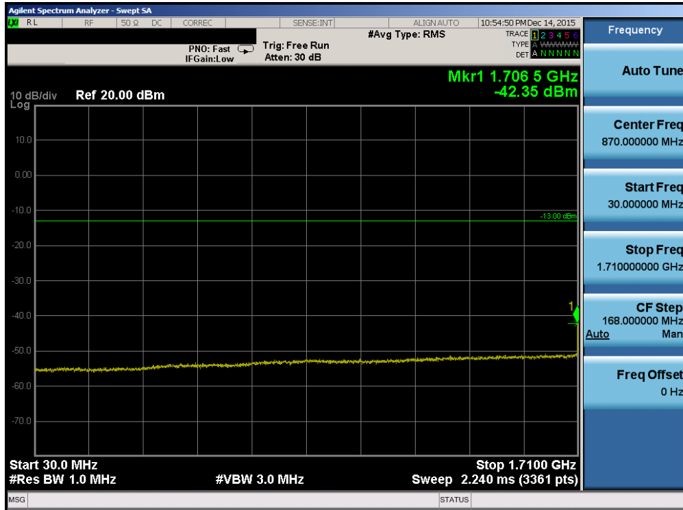
Plot 7-41. Conducted Spurious Plot (Band 4 – 3.0MHz QPSK – RB Size 1, RB Offset 0 – Mid Channel)
