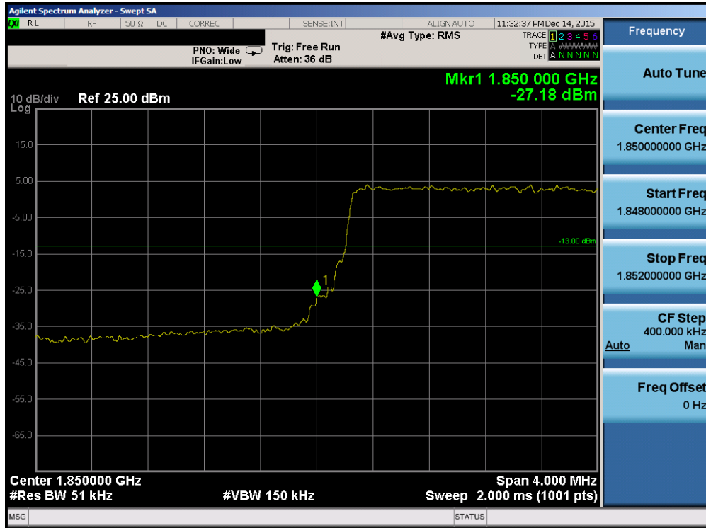
Plot 7-96. Lower Band Edge Plot (Band 2 – 5.0MHz QPSK – RB Size 25)
