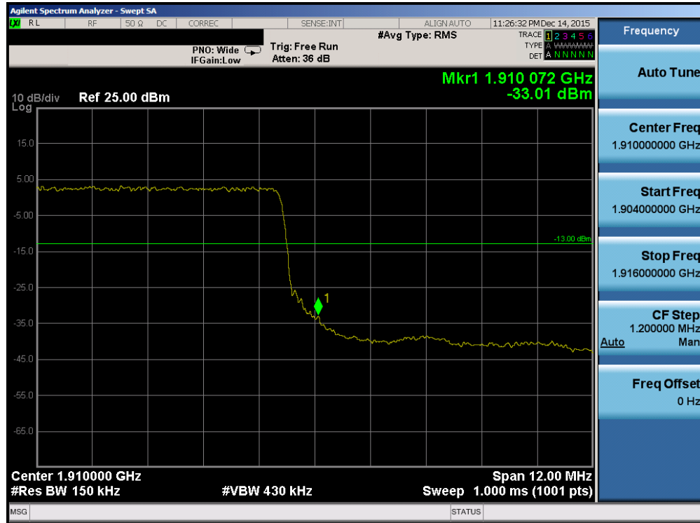
Plot 7-106. Upper Band Edge Plot (Band 2 – 15.0MHz QPSK – RB Size 75)
