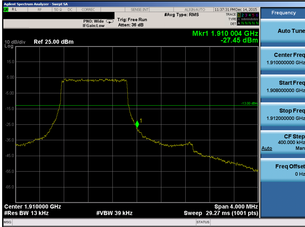
Plot 7-90. Upper Band Edge Plot (Band 2 – 1.4MHz QPSK – RB Size 6)
