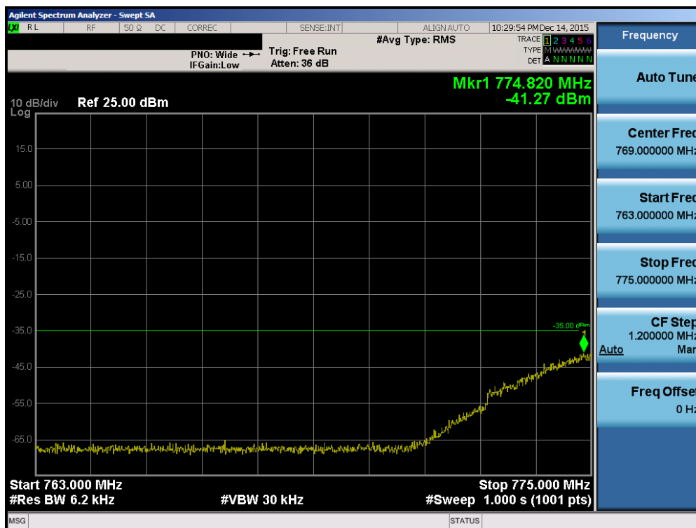
Plot 7-57. Lower Emission Mask Edge Plot (Band 13 – 5.0MHz QPSK – RB Size 25)
