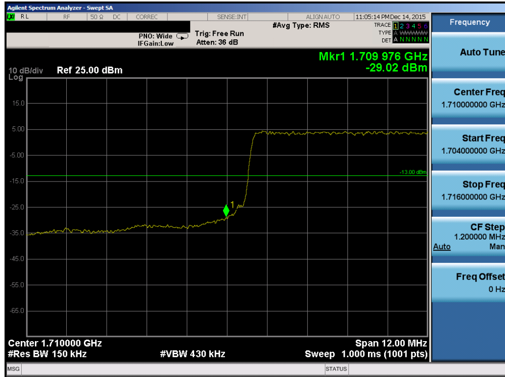
Plot 7-80. Lower Band Edge Plot (Band 4 – 15.0MHz QPSK – RB Size 75)
