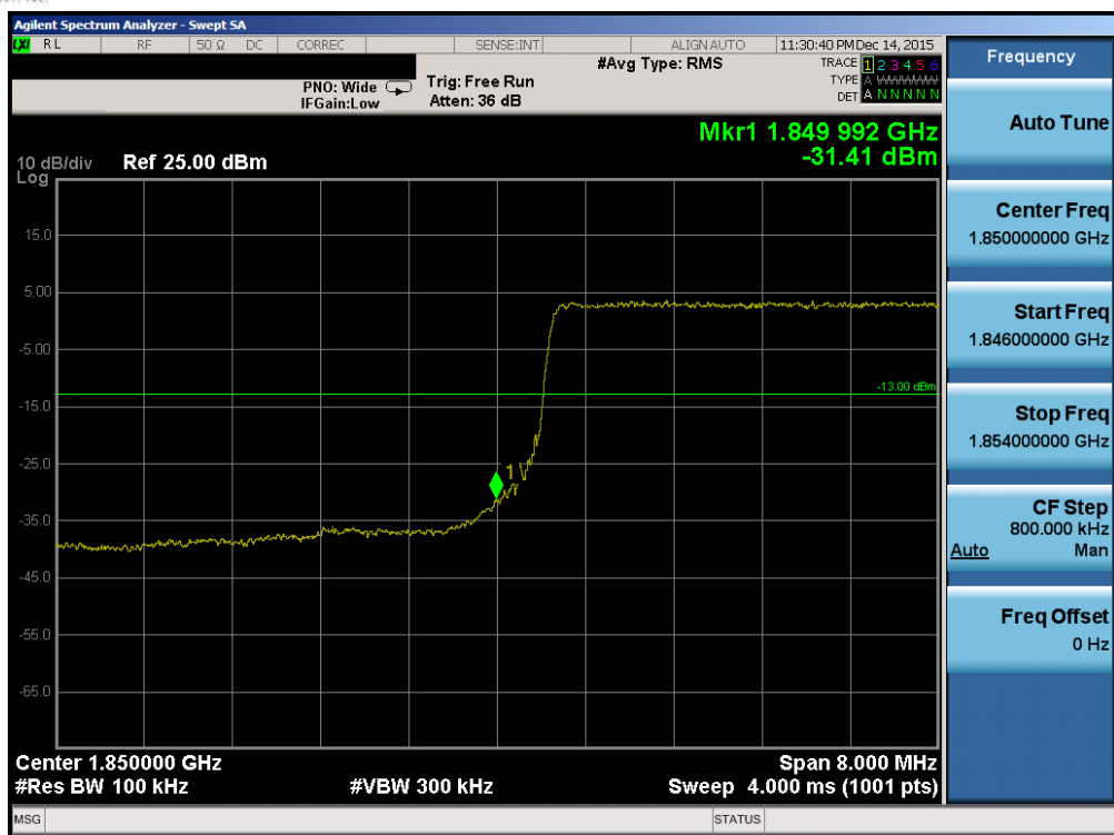
Plot 7-100. Lower Band Edge Plot (Band 2 – 10.0MHz QPSK – RB Size 50)
