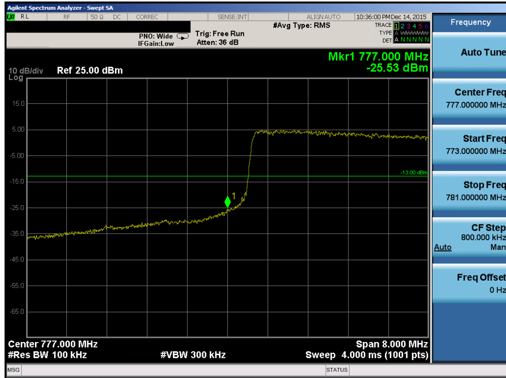
Plot 7-60. Lower Band Edge Plot (Band 13 – 10.0MHz QPSK – RB Size 50)
