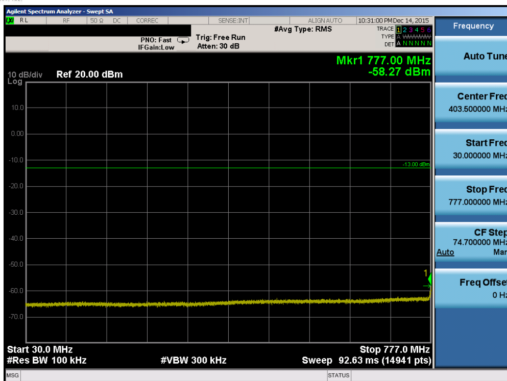
Plot 7-35. Conducted Spurious Plot (Band 13 – 5.0MHz QPSK – RB Size 1, RB Offset 0 – High Channel)
