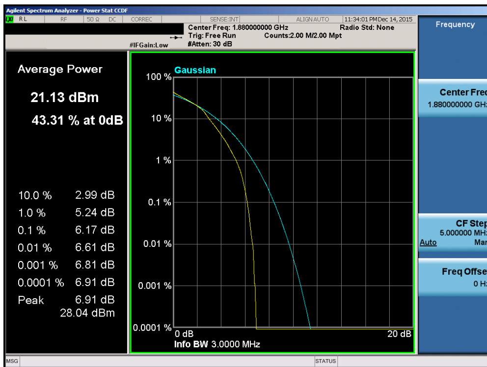
Plot 7-115. PAR Plot (Band 2 – 3.0MHz 16-QAM – RB Size 15)
