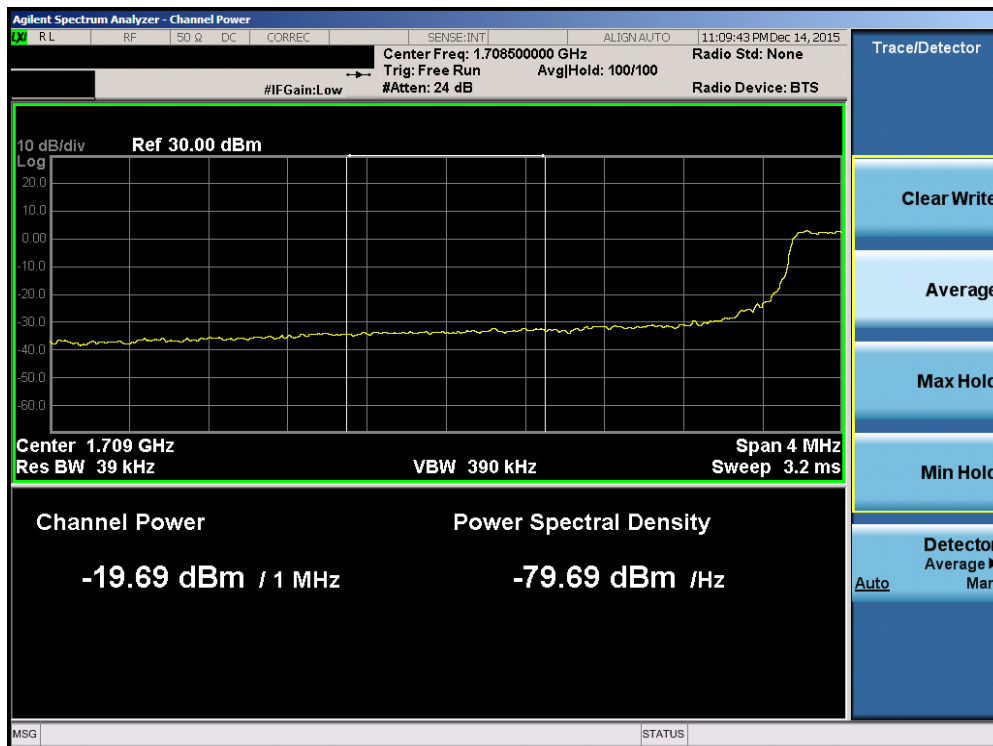
Plot 7-73. Lower Extended Band Edge Plot (Band 4 – 5.0MHz QPSK – RB Size 25)
