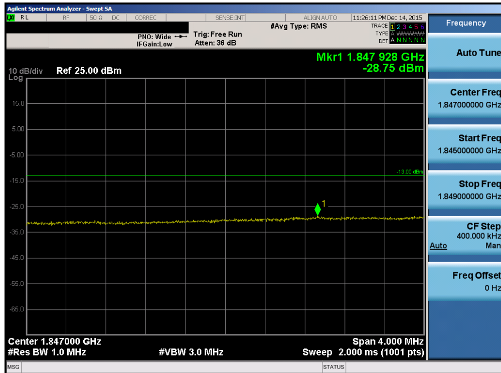
Plot 7-105. Lower Extended Band Edge Plot (Band 2 – 15.0MHz QPSK – RB Size 75)
