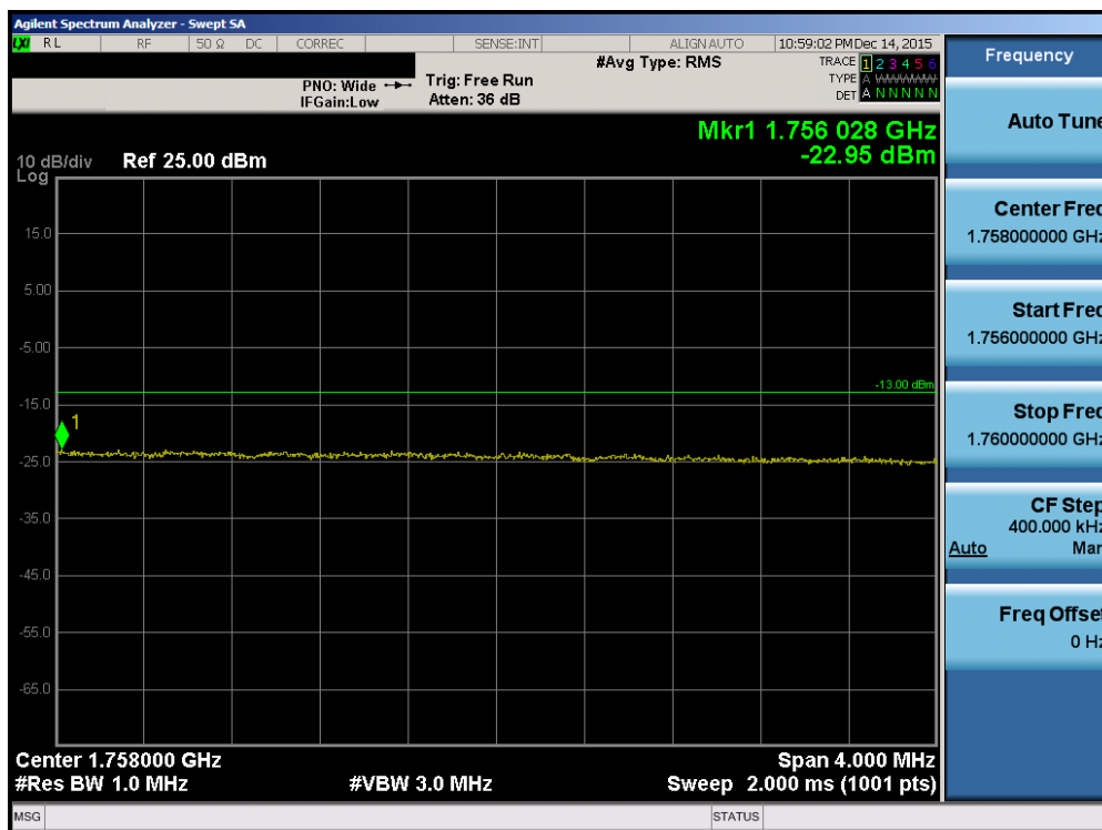
Plot 7-87. Upper Extended Band Edge Plot (Band 4 – 20.0MHz QPSK – RB Size 100)
