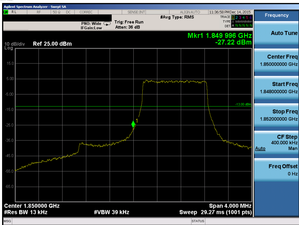
Plot 7-88. Lower Band Edge Plot (Band 2 – 1.4MHz QPSK – RB Size 6)
