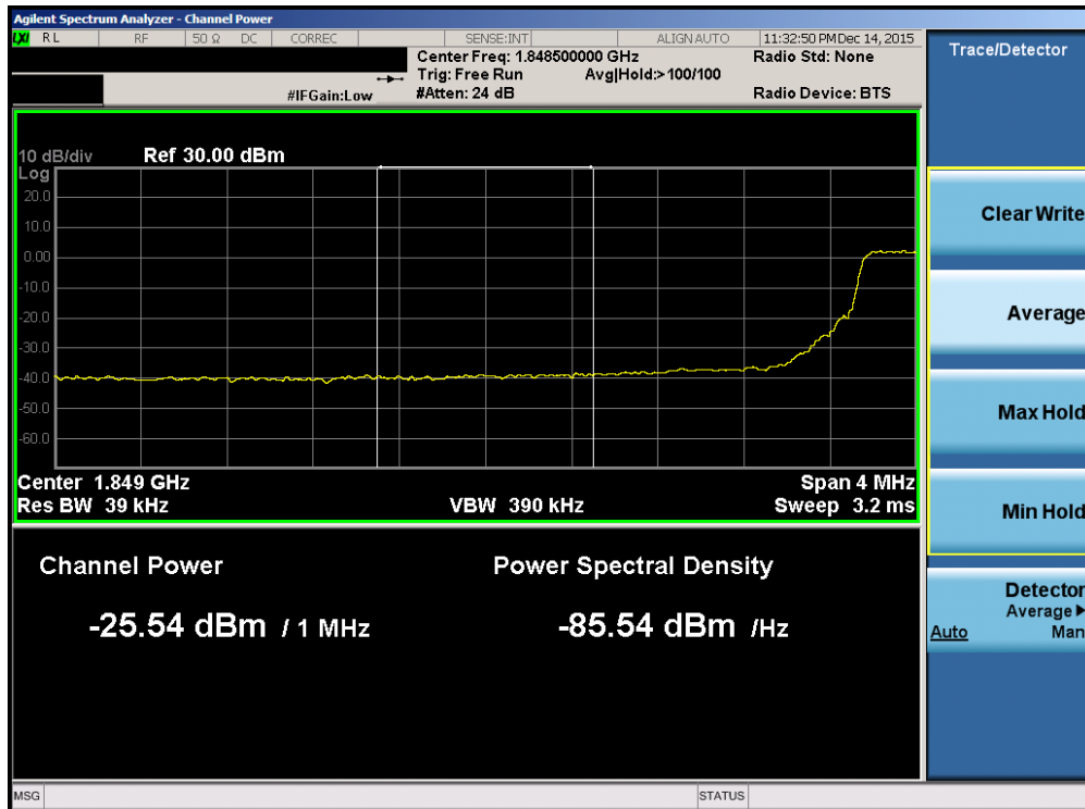
Plot 7-97. Lower Extended Band Edge Plot (Band 2 – 5.0MHz QPSK – RB Size 25)
