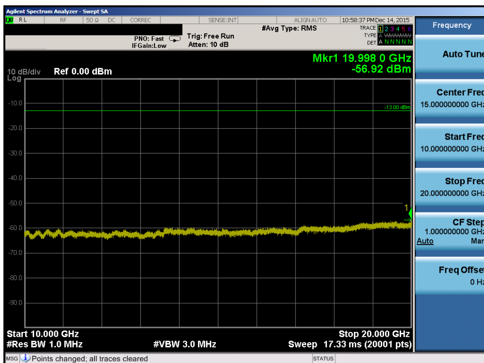
Plot 7-46. Conducted Spurious Plot (Band 4 – 3.0MHz QPSK – RB Size 1, RB Offset 0 – High Channel)
