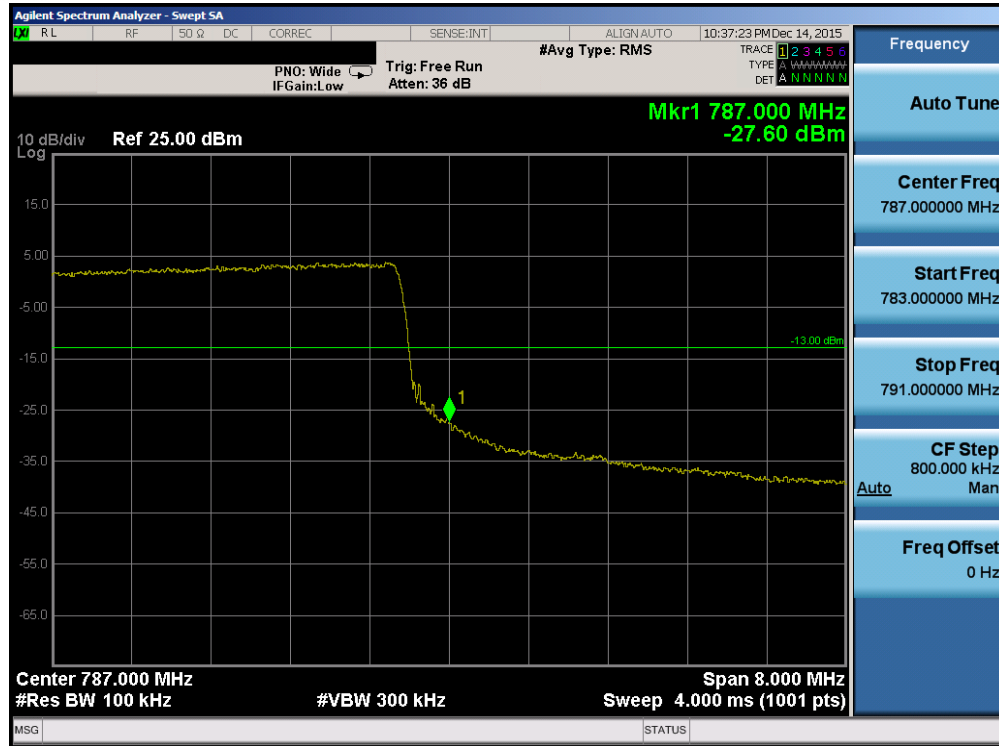
Plot 7-62. Upper Band Edge Plot (Band 13 – 10.0MHz QPSK – RB Size 50)
