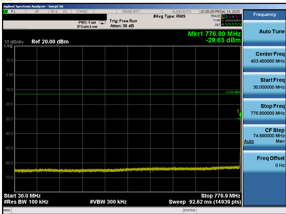
Plot 7-29. Conducted Spurious Plot (Band 13 – 5.0MHz QPSK – RB Size 1, RB Offset 0 – Low Channel)
