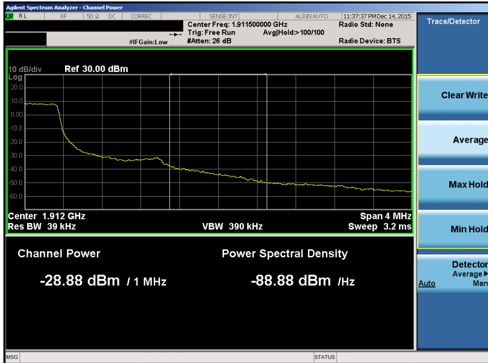
Plot 7-91. Upper Extended Band Edge Plot (Band 2 – 1.4MHz QPSK – RB Size 6)
