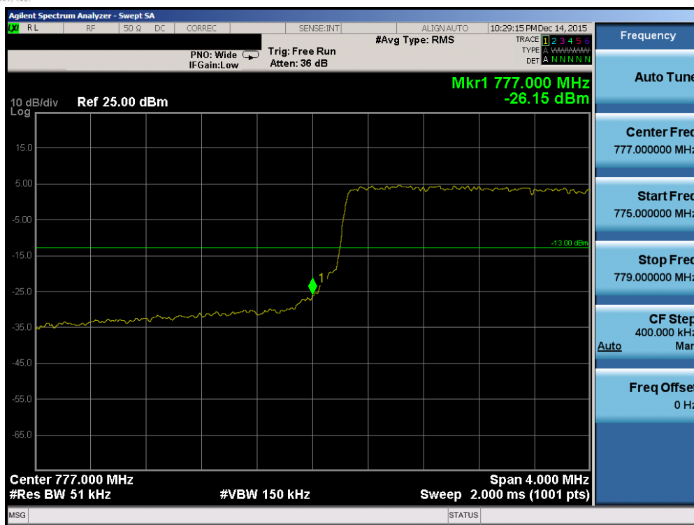
Plot 7-56. Lower Band Edge Plot (Band 13 – 5.0MHz QPSK – RB Size 25)
