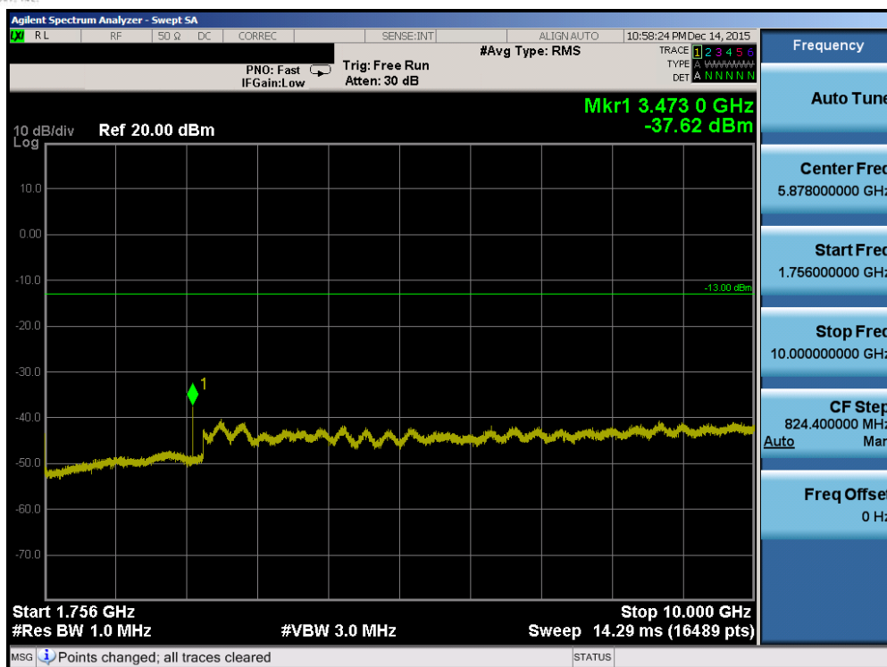
Plot 7-45. Conducted Spurious Plot (Band 4 – 3.0MHz QPSK – RB Size 1, RB Offset 0 – High Channel)
