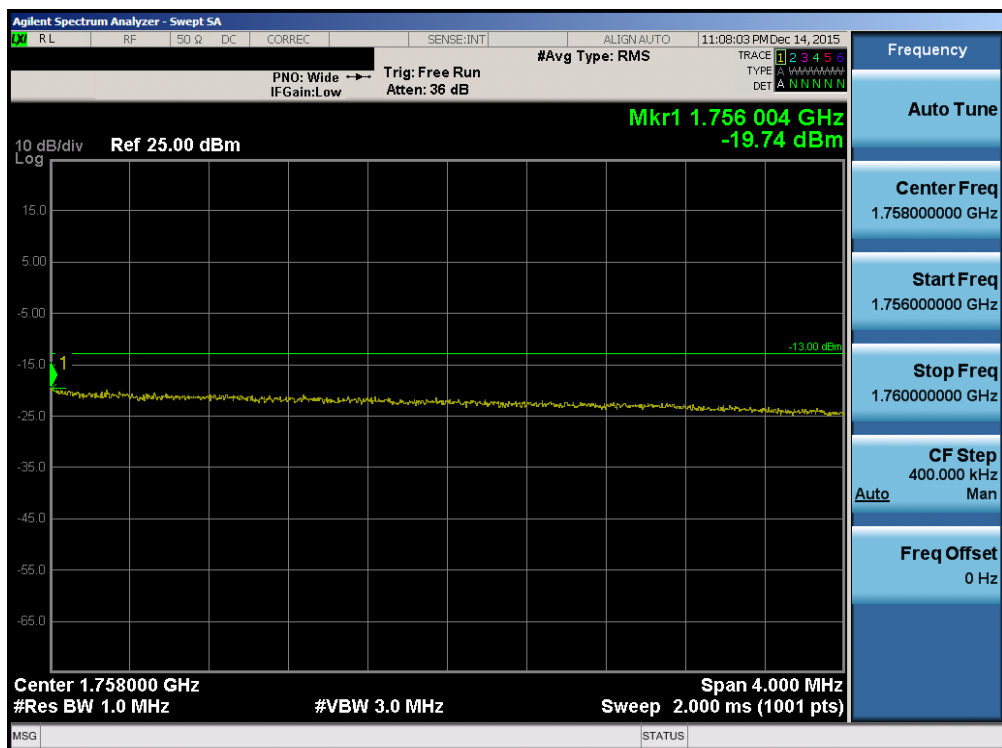
Plot 7-79. Upper Extended Band Edge Plot (Band 4 – 10.0MHz QPSK – RB Size 50)
