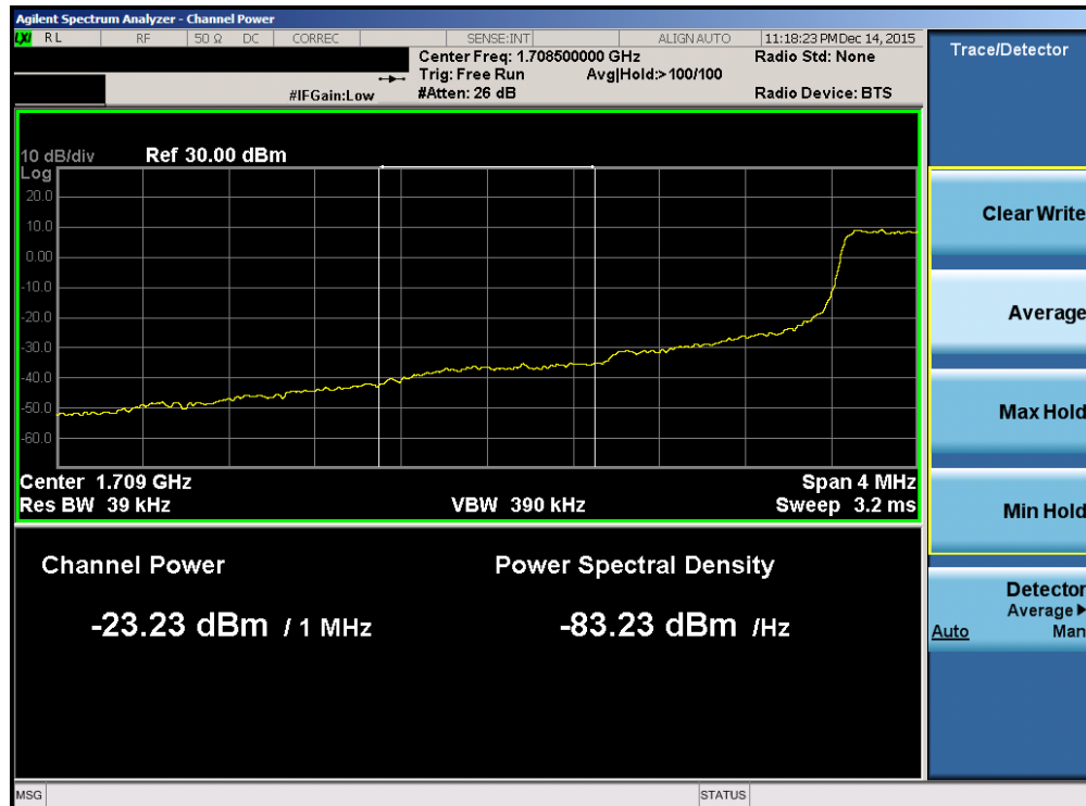
Plot 7-65. Lower Extended Band Edge Plot (Band 4 – 1.4MHz QPSK – RB Size 6)
