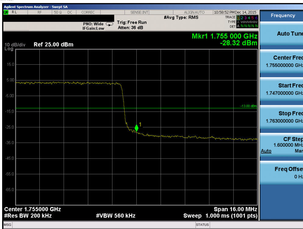
Plot 7-86. Upper Band Edge Plot (Band 4 – 20.0MHz QPSK – RB Size 100)
