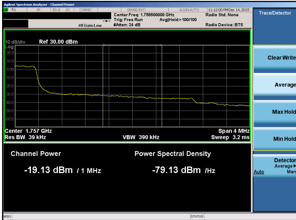
Plot 7-71. Upper Extended Band Edge Plot (Band 4 – 3.0MHz QPSK – RB Size 15)
