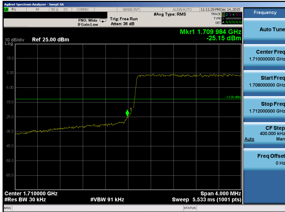
Plot 7-68. Lower Band Edge Plot (Band 4 – 3.0MHz QPSK – RB Size 15)
