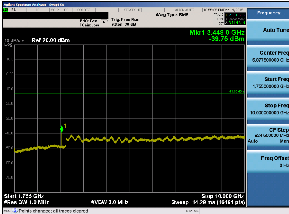
Plot 7-42. Conducted Spurious Plot (Band 4 – 3.0MHz QPSK – RB Size 1, RB Offset 0 – Mid Channel)
