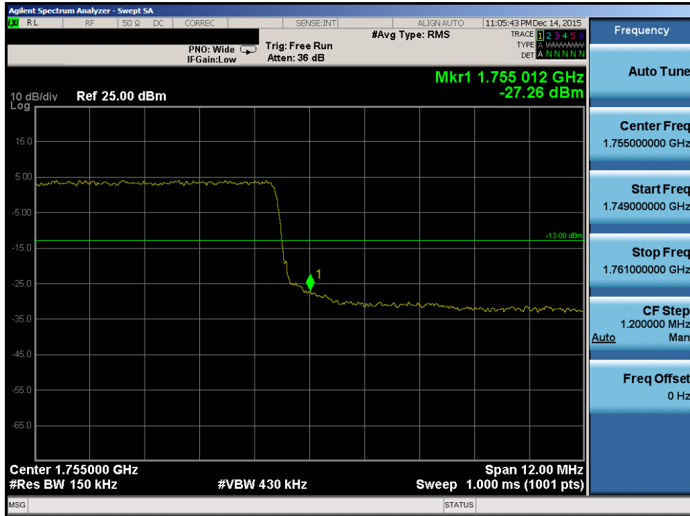
Plot 7-82. Upper Band Edge Plot (Band 4 – 15.0MHz QPSK – RB Size 75)
