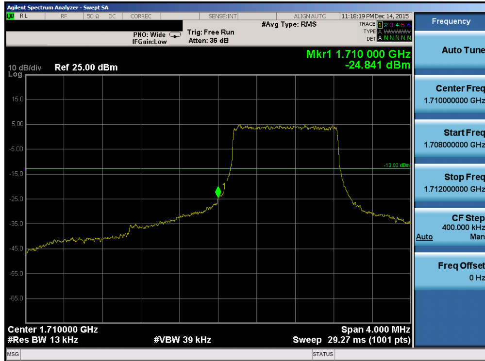
Plot 7-64. Lower Band Edge Plot (Band 4 – 1.4MHz QPSK – RB Size 6)
