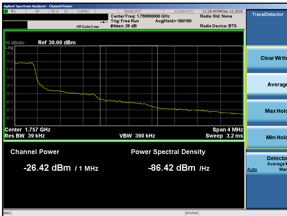
Plot 7-67. Upper Extended Band Edge Plot (Band 4 – 1.4MHz QPSK – RB Size 6)
