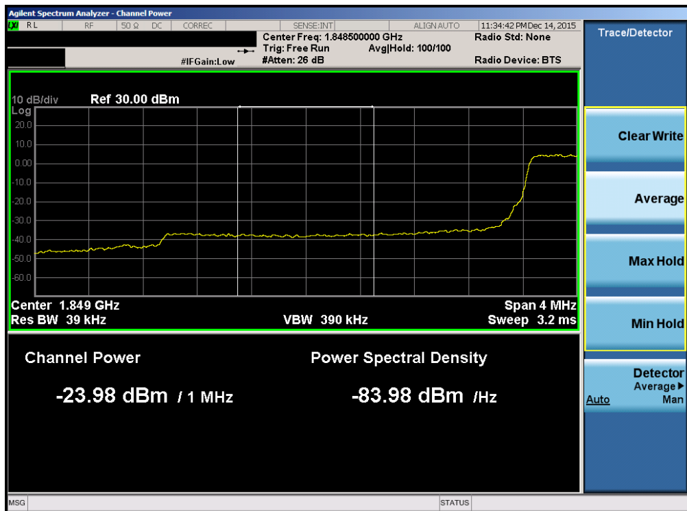
Plot 7-93. Lower Extended Band Edge Plot (Band 2 – 3.0MHz QPSK – RB Size 15)
