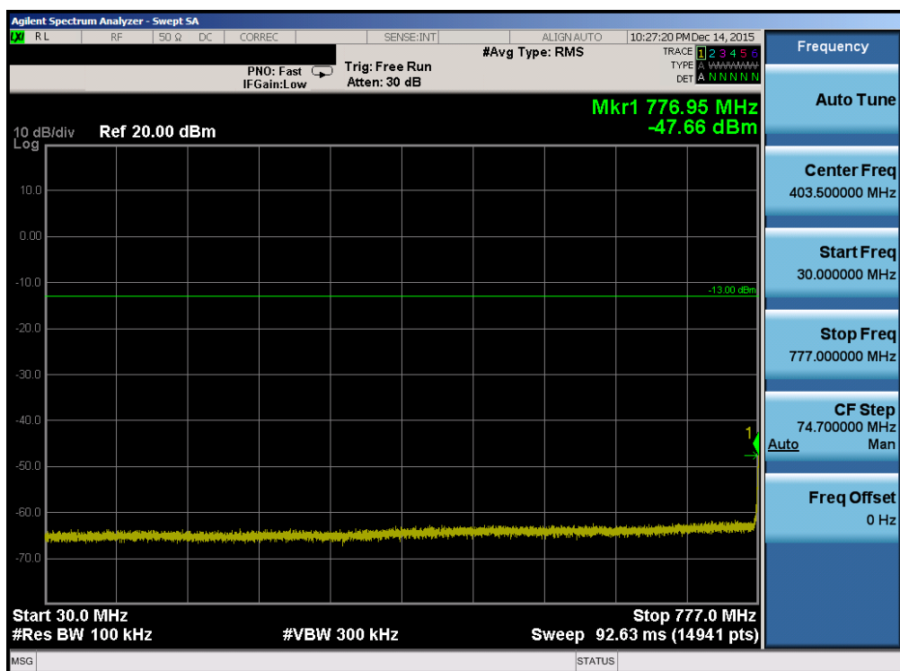
Plot 7-32. Conducted Spurious Plot (Band 13 – 5.0MHz QPSK – RB Size 1, RB Offset 0 – Mid Channel)
