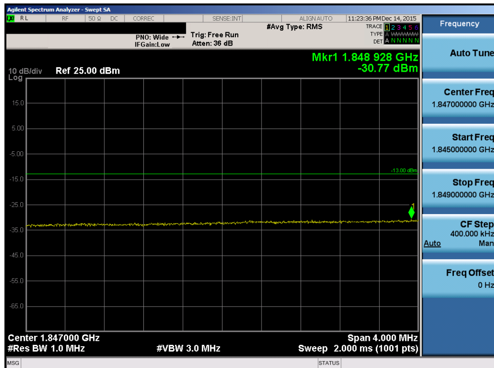
Plot 7-109. Lower Extended Band Edge Plot (Band 2 – 20.0MHz QPSK – RB Size 100)
