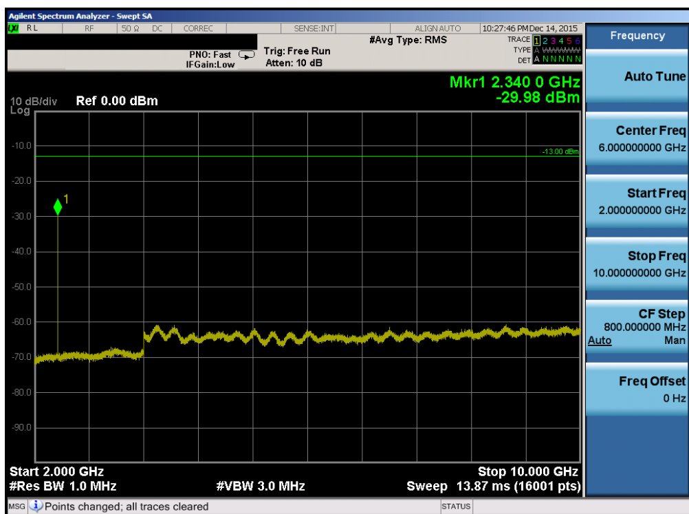
Plot 7-34. Conducted Spurious Plot (Band 13 – 5.0MHz QPSK – RB Size 1, RB Offset 0 – Mid Channel)
