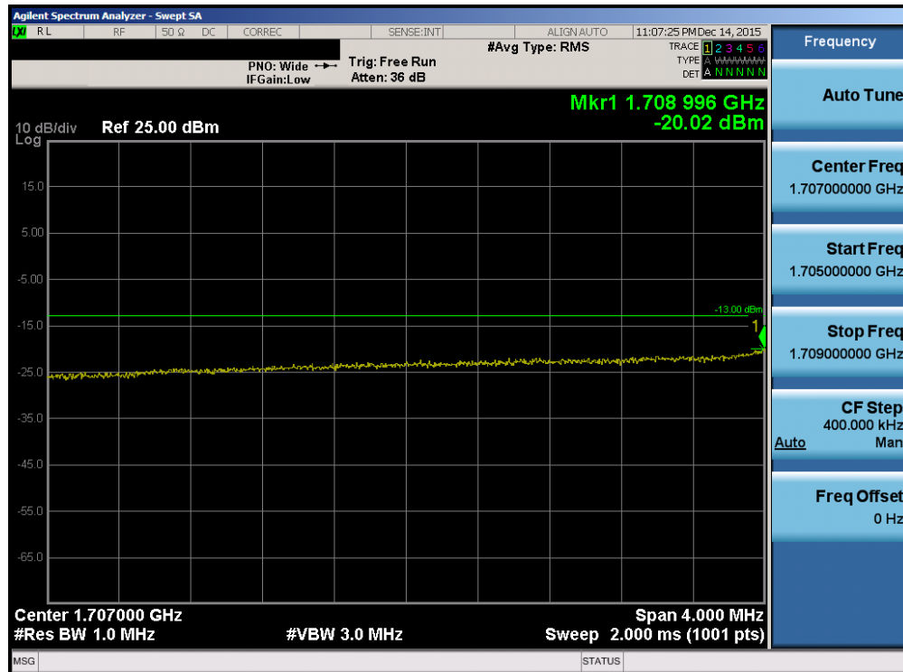
Plot 7-77. Lower Extended Band Edge Plot (Band 4 – 10.0MHz QPSK – RB Size 50)
