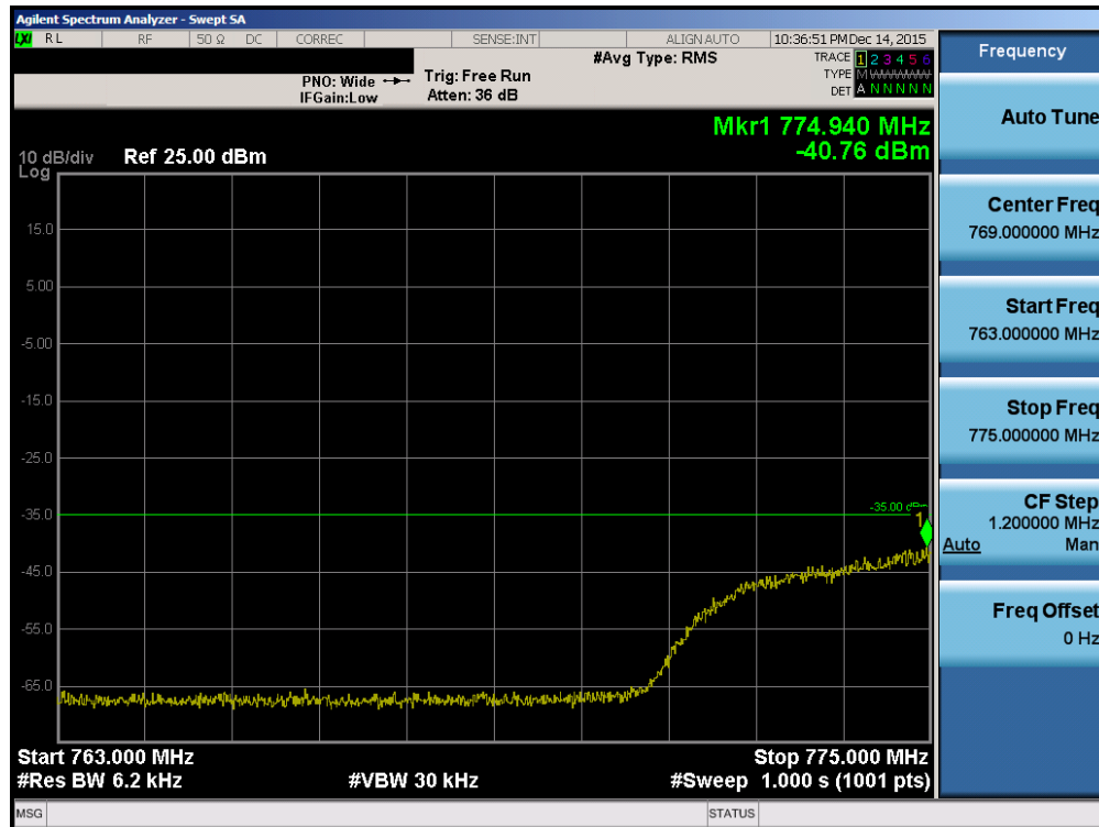
Plot 7-61. Lower Emission Mask Edge Plot (Band 13 – 10.0MHz QPSK – RB Size 50)
