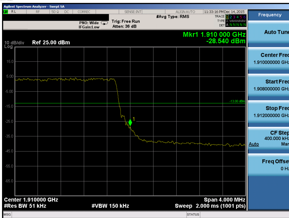
Plot 7-98. Upper Band Edge Plot (Band 2 – 5.0MHz QPSK – RB Size 25)
