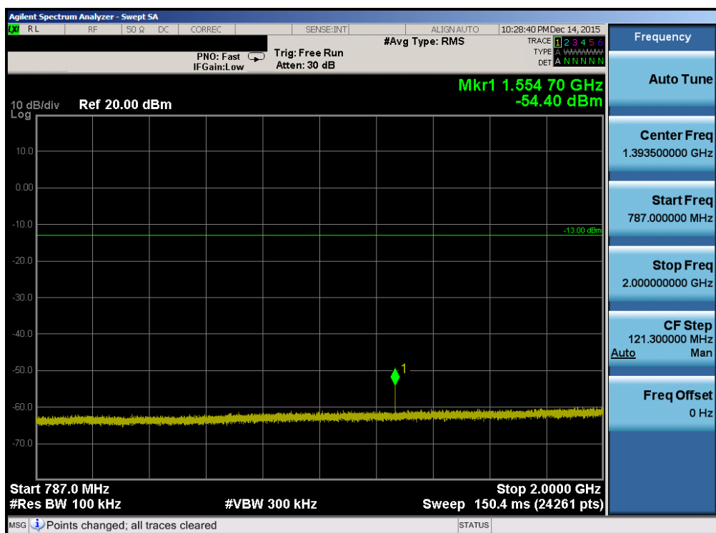
Plot 7-30. Conducted Spurious Plot (Band 13 – 5.0MHz QPSK – RB Size 1, RB Offset 0 – Low Channel)
