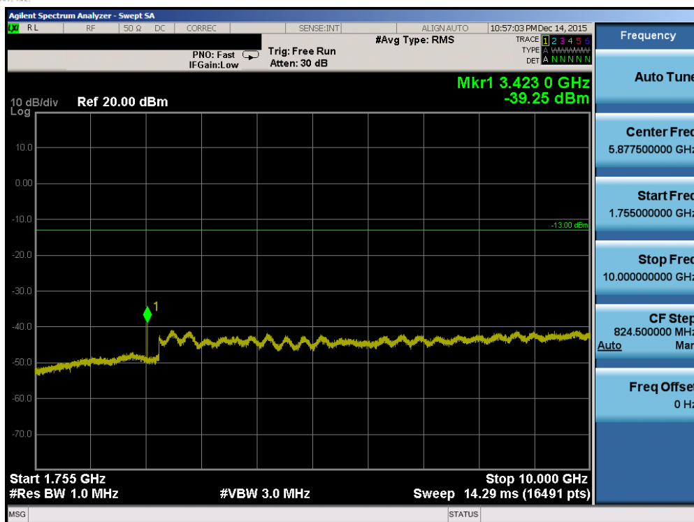
Plot 7-39. Conducted Spurious Plot (Band 4 – 3.0MHz QPSK – RB Size 1, RB Offset 0 – Low Channel)
