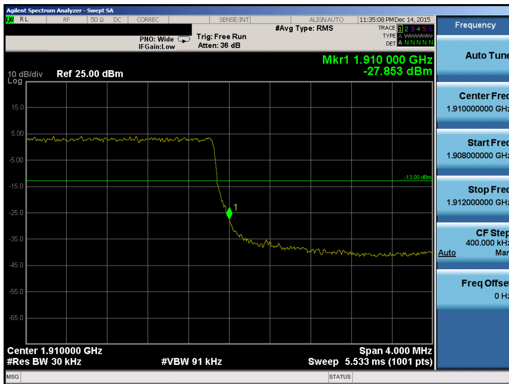
Plot 7-94. Upper Band Edge Plot (Band 2 – 3.0MHz QPSK – RB Size 15)
