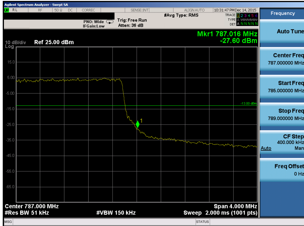
Plot 7-58. Upper Band Edge Plot (Band 13 – 5.0MHz QPSK – RB Size 25)
