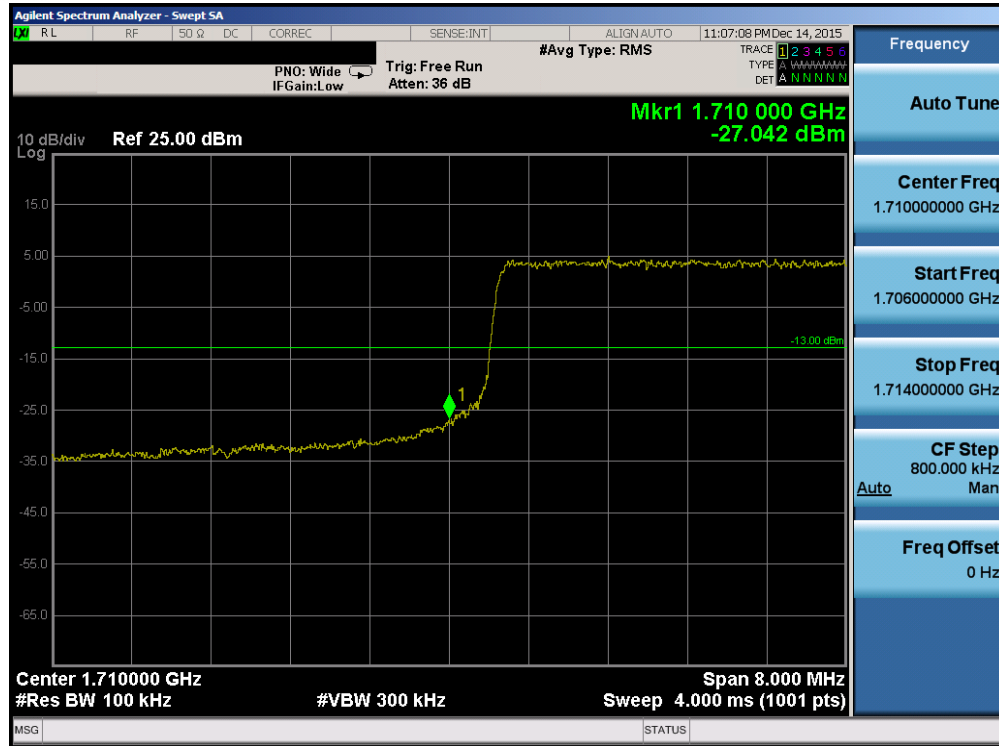
Plot 7-76. Lower Band Edge Plot (Band 4 – 10.0MHz QPSK – RB Size 50)
