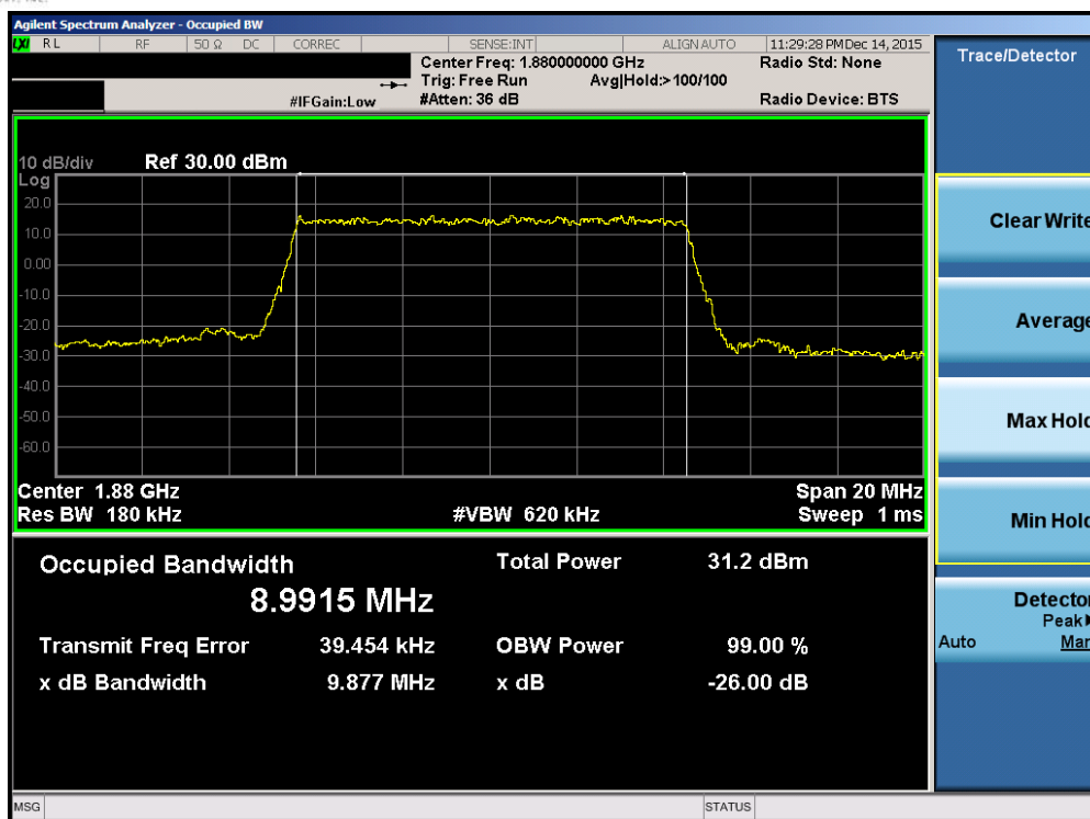
Plot 7-23. Occupied Bandwidth Plot (Band 2 – 10.0MHz QPSK – RB Size 50)
