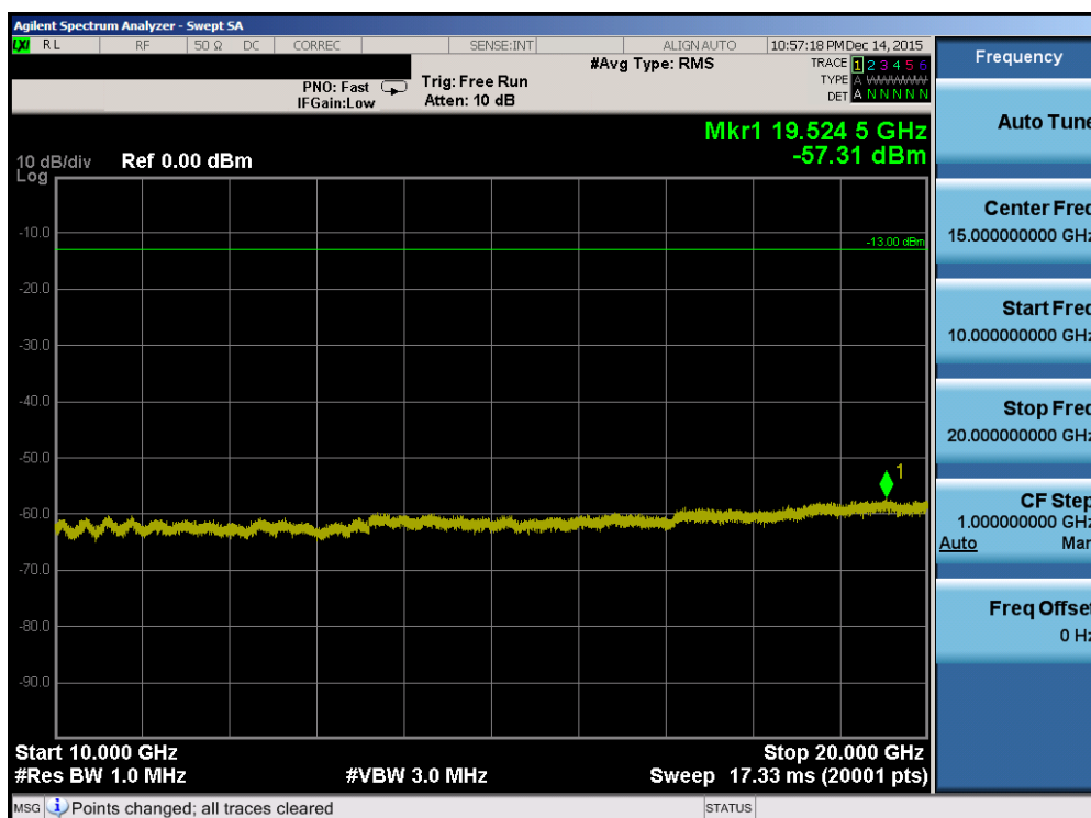
Plot 7-40. Conducted Spurious Plot (Band 4 – 3.0MHz QPSK – RB Size 1, RB Offset 0 – Low Channel)
