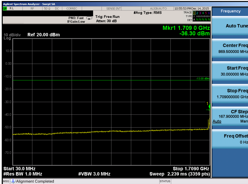
Plot 7-38. Conducted Spurious Plot (Band 4 – 3.0MHz QPSK – RB Size 1, RB Offset 0 – Low Channel)
