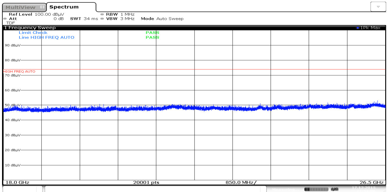
Plot 7-8. Radiated Spurious Plot above 18GHz (Pol. V)
