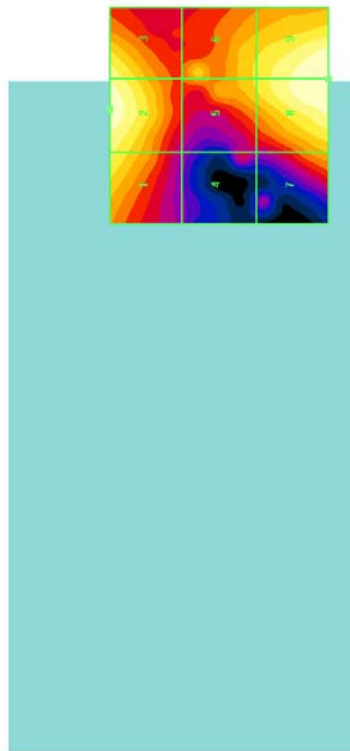
Figure 10-1 Sample E-field Scan Overlay (T-Coil Centered Scan area pictured. See Test Setup Photographs for actual WD overlay and Acoustic Centered Scan Area.)
