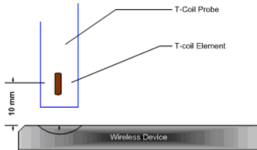
Figure 4-11 Measurement Distance
