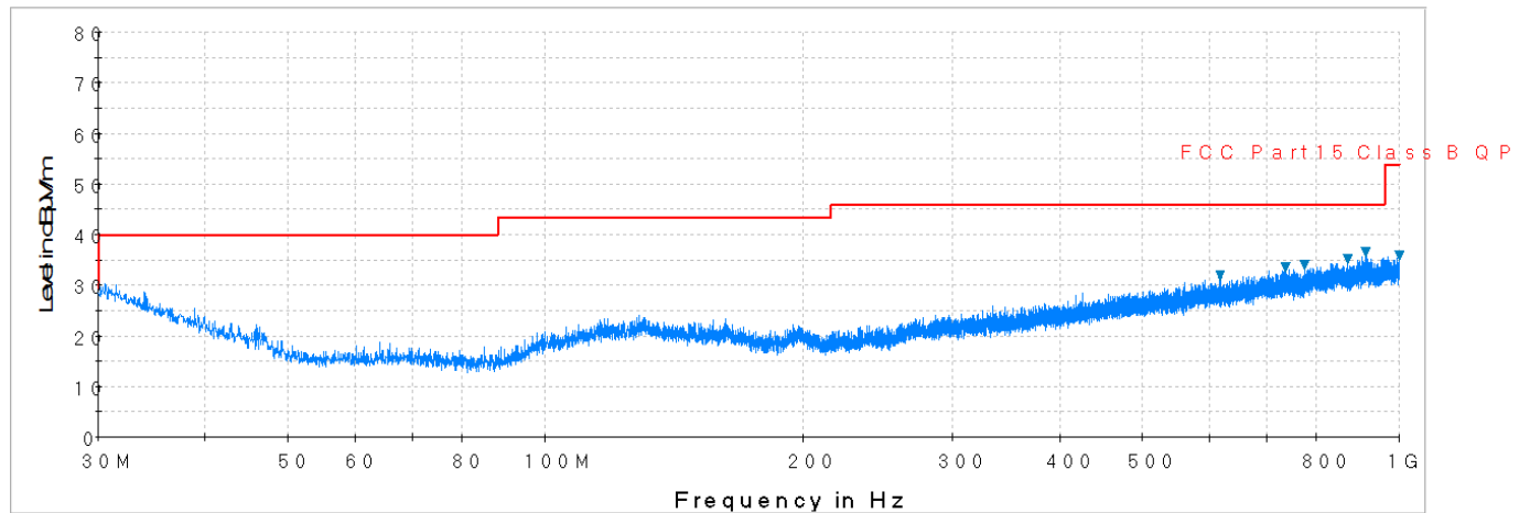
Plot 7-12. Radiated Spurious Plot below 1GHz (Pol. V)
