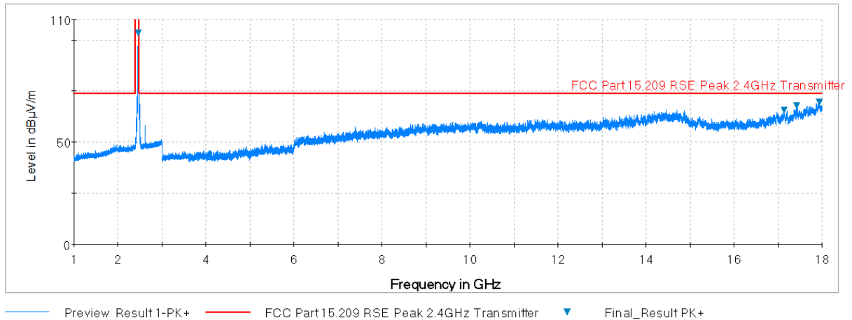
Plot 7-35. Radiated Spurious Plot above 1GHz (802.11b – Ch. 11, Ant. Pol. H)
