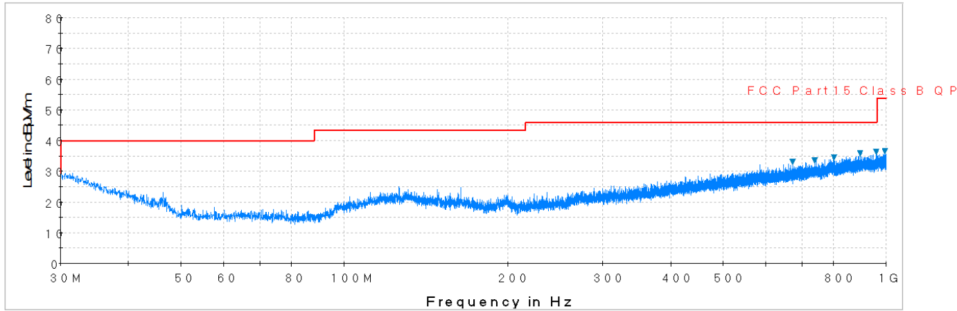
Plot 7-13. Radiated Spurious Plot below 1GHz (Pol. H)
