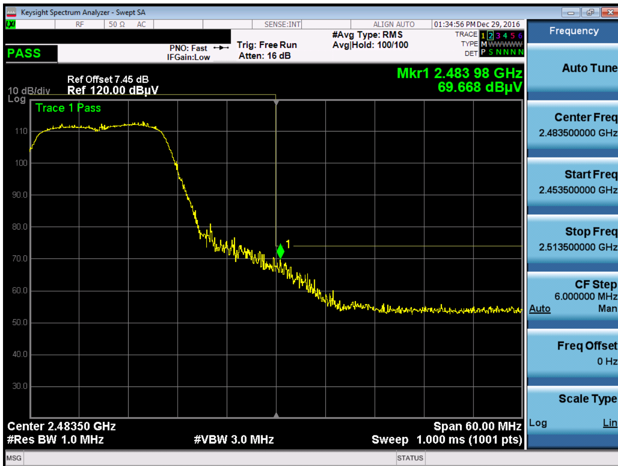
Plot 7-12. Radiated Restricted Upper Band Edge Measurement (Peak)
