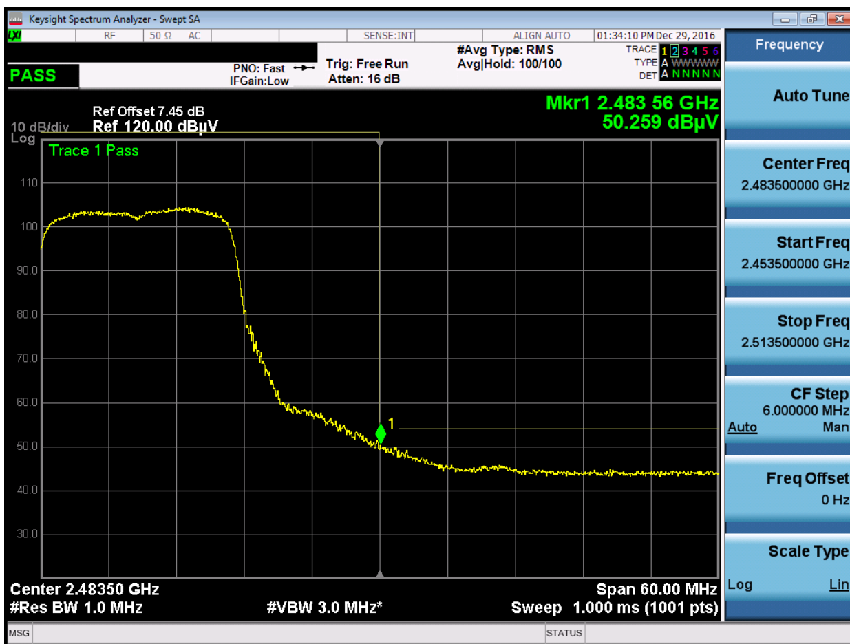
Plot 7-11. Radiated Restricted Upper Band Edge Measurement (Average)
