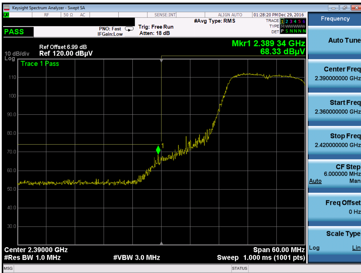
Plot 7-10. Radiated Restricted Lower Band Edge Measurement (Peak)
