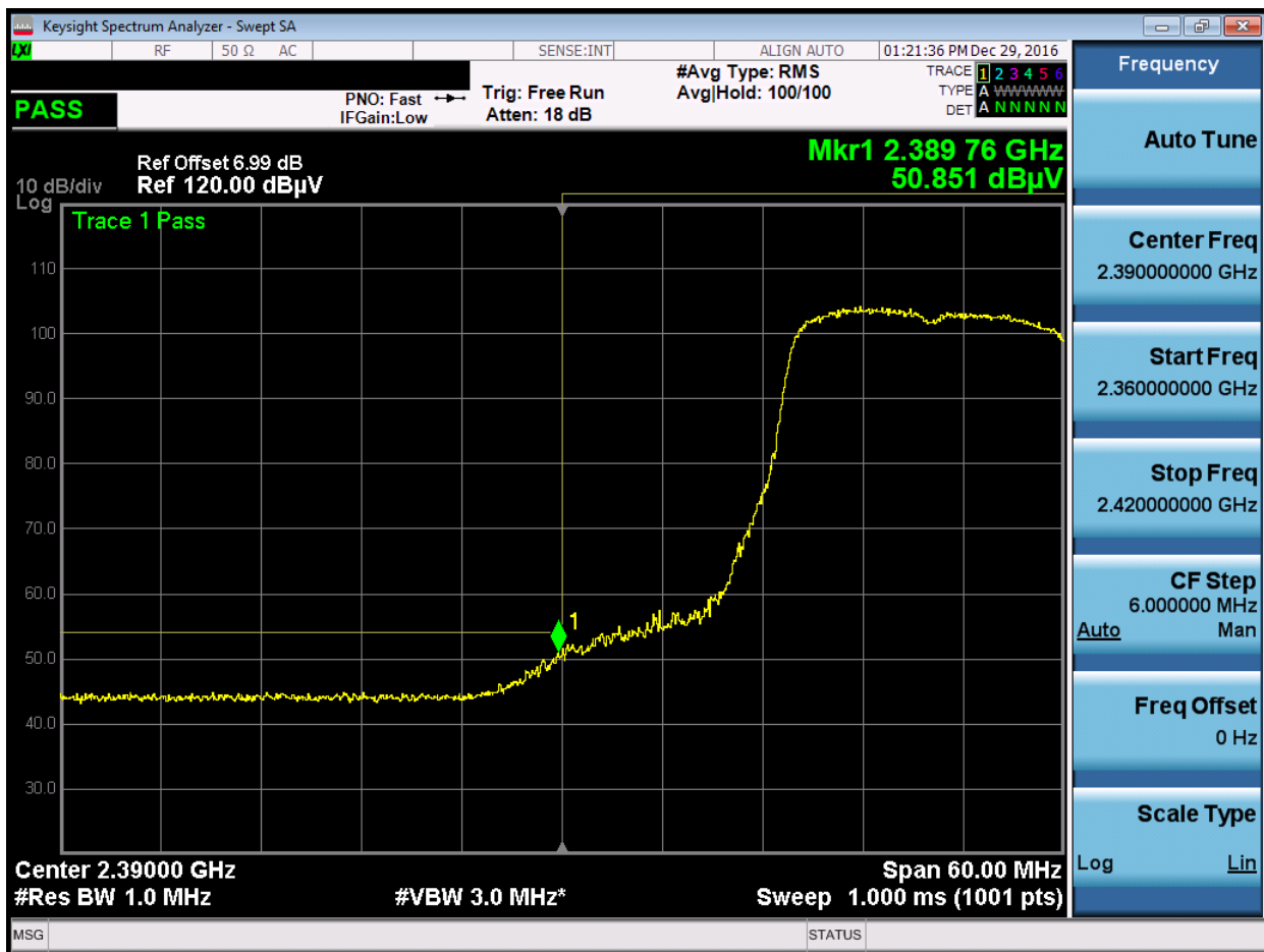
Plot 7-9. Radiated Restricted Lower Band Edge Measurement (Average)
