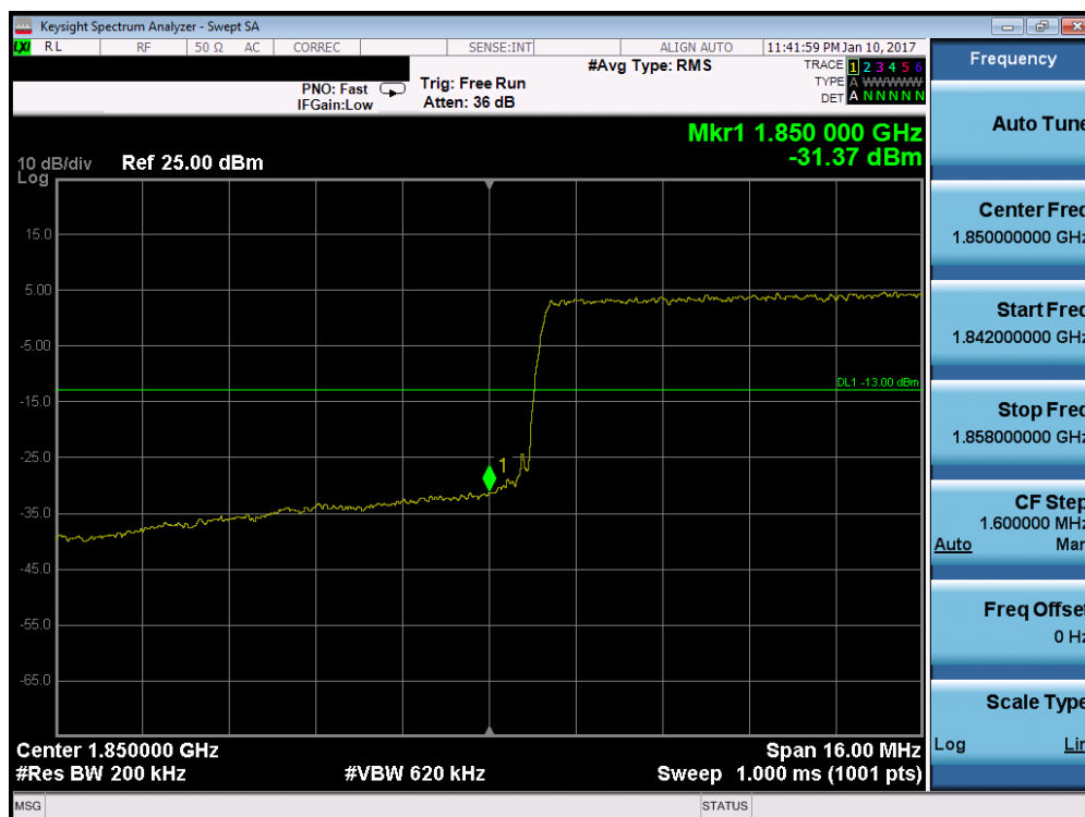
Plot 7-102. Lower Band Edge Plot (Band 2 – 20.0MHz QPSK – RB Size 100)
