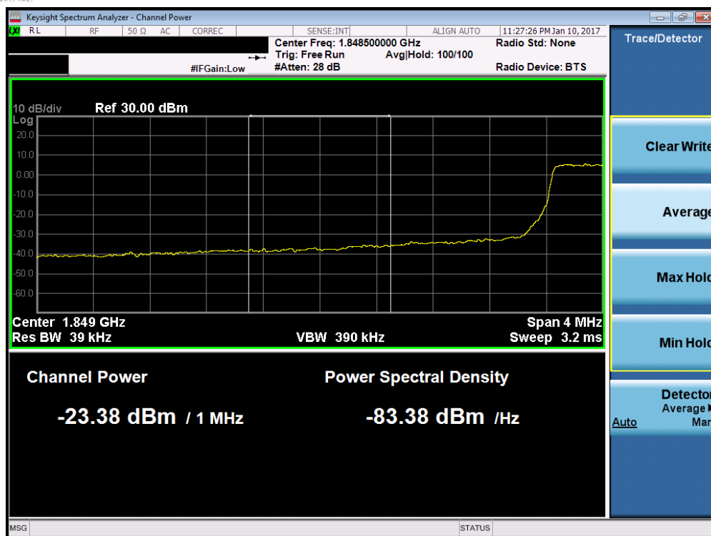
Plot 7-87. Lower Extended Band Edge Plot (Band 2 – 3.0MHz QPSK – RB Size 15)
