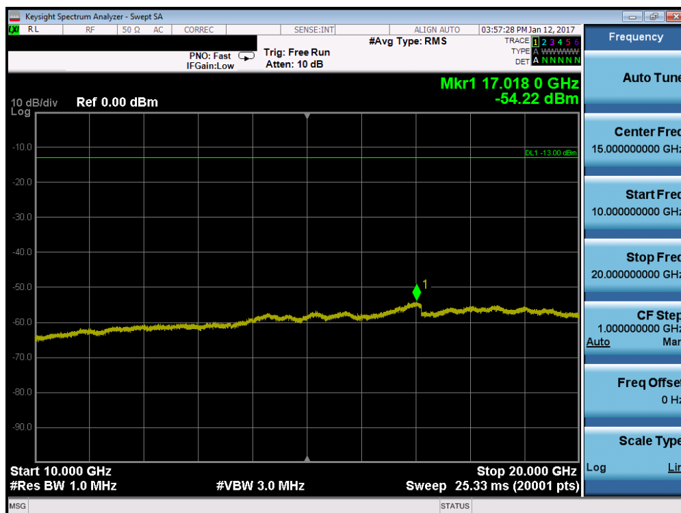
Plot 7-34. Conducted Spurious Plot (Band 4 – 15.0MHz QPSK – RB Size 1, RB Offset 0 – Low Channel)
