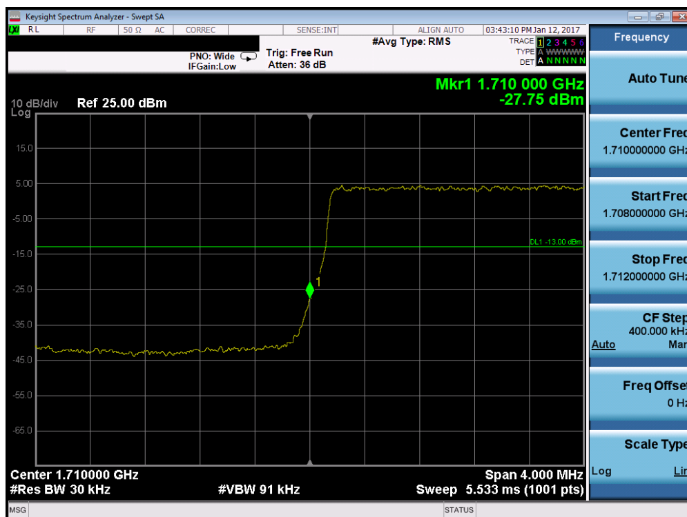
Plot 7-62. Lower Band Edge Plot (Band 4 – 3.0MHz QPSK – RB Size 15)
