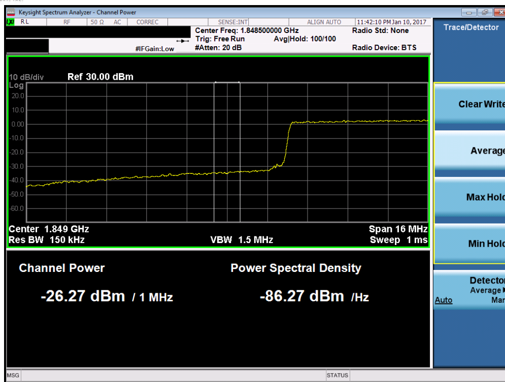
Plot 7-103. Lower Extended Band Edge Plot (Band 2 – 20.0MHz QPSK – RB Size 100)
