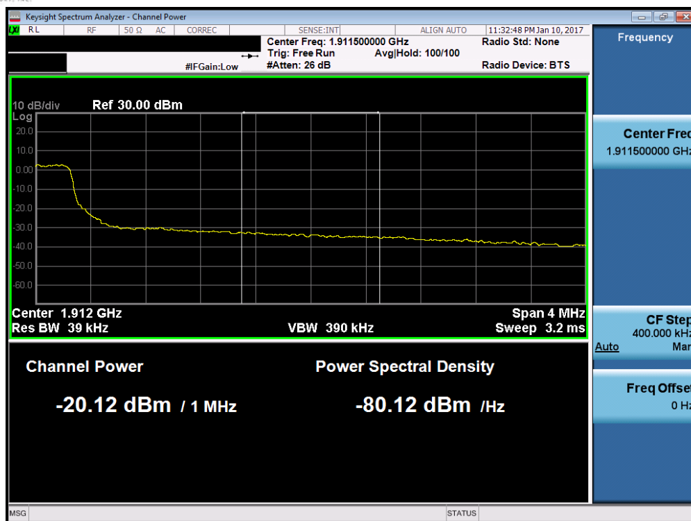
Plot 7-93. Upper Extended Band Edge Plot (Band 2 – 5.0MHz QPSK – RB Size 25)
