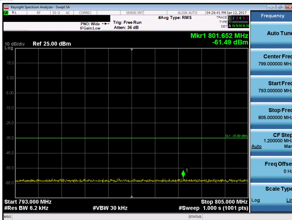
Plot 7-57. Upper Emission Mask Edge Plot (Band 13 – 10.0MHz QPSK – RB Size 50)
