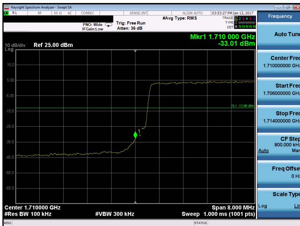
Plot 7-70. Lower Band Edge Plot (Band 4 – 10.0MHz QPSK – RB Size 50)
