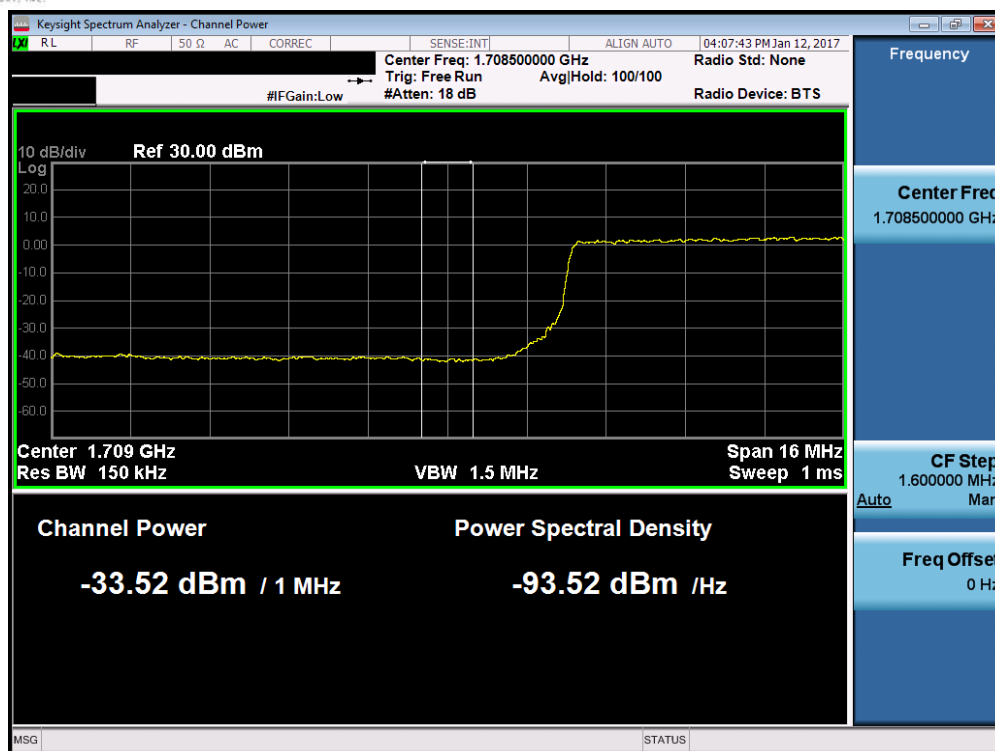
Plot 7-79. Lower Extended Band Edge Plot (Band 4 – 20.0MHz QPSK – RB Size 100)
