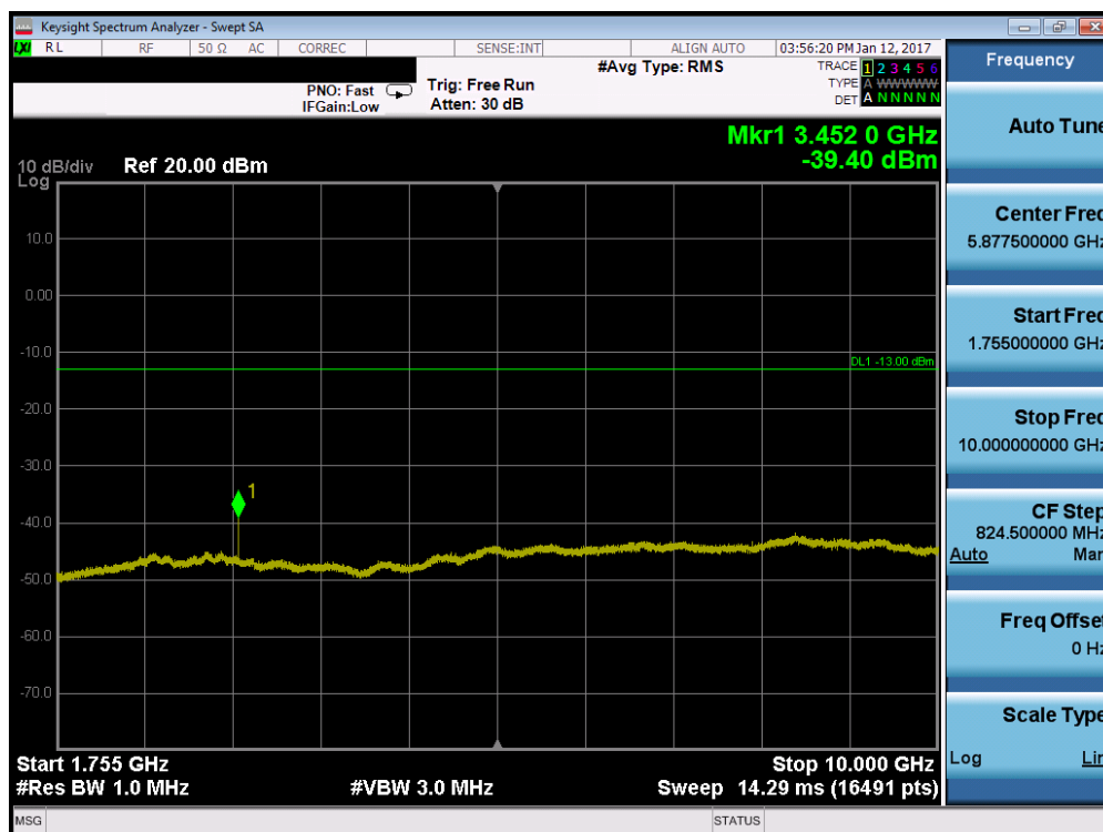
Plot 7-36. Conducted Spurious Plot (Band 4 – 15.0MHz QPSK – RB Size 1, RB Offset 0 – Mid Channel)
