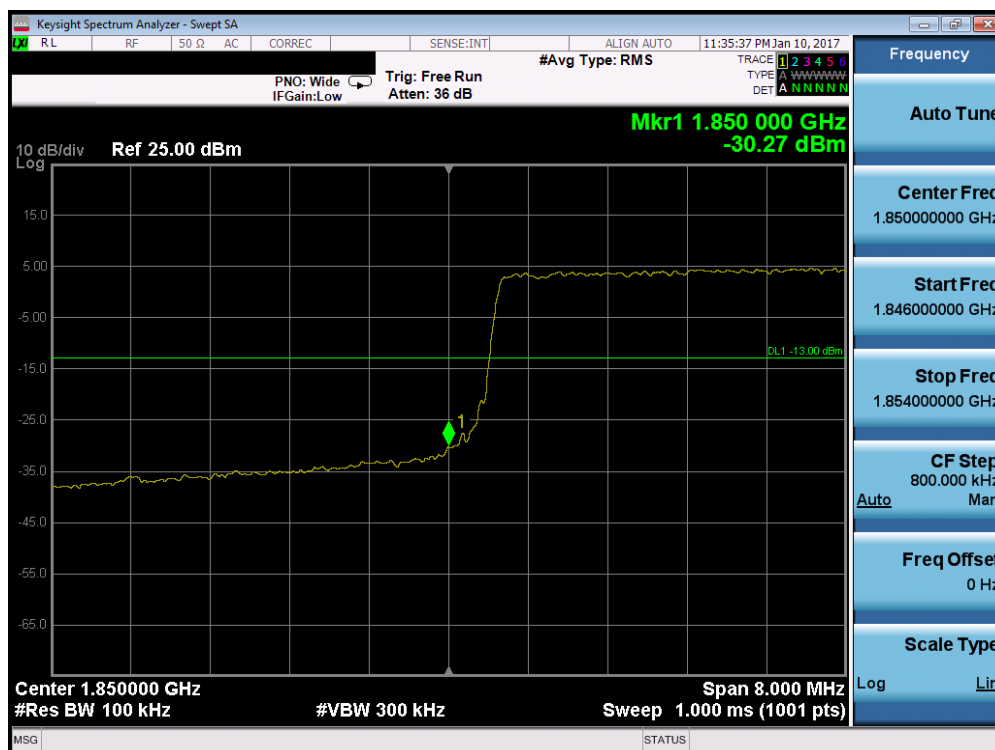
Plot 7-94. Lower Band Edge Plot (Band 2 – 10.0MHz QPSK – RB Size 50)
