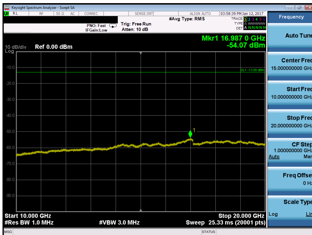
Plot 7-40. Conducted Spurious Plot (Band 4 – 15.0MHz QPSK – RB Size 1, RB Offset 0 – High Channel)
