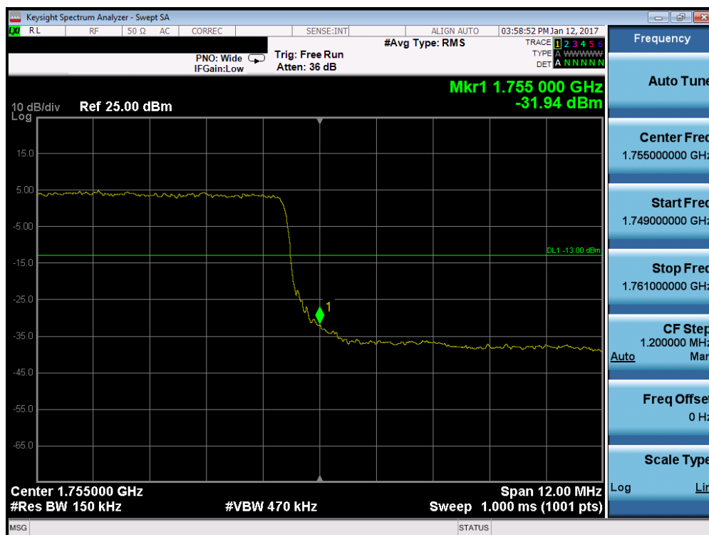
Plot 7-76. Upper Band Edge Plot (Band 4 – 15.0MHz QPSK – RB Size 75)
