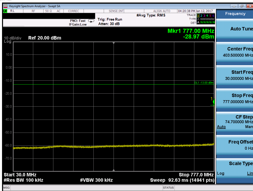
Plot 7-29. Conducted Spurious Plot (Band 13 – 10.0MHz QPSK – RB Size 1, RB Offset 0)
