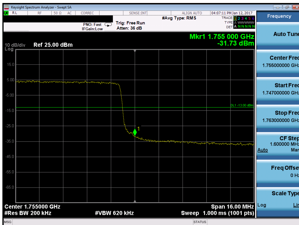
Plot 7-80. Upper Band Edge Plot (Band 4 – 20.0MHz QPSK – RB Size 100)
