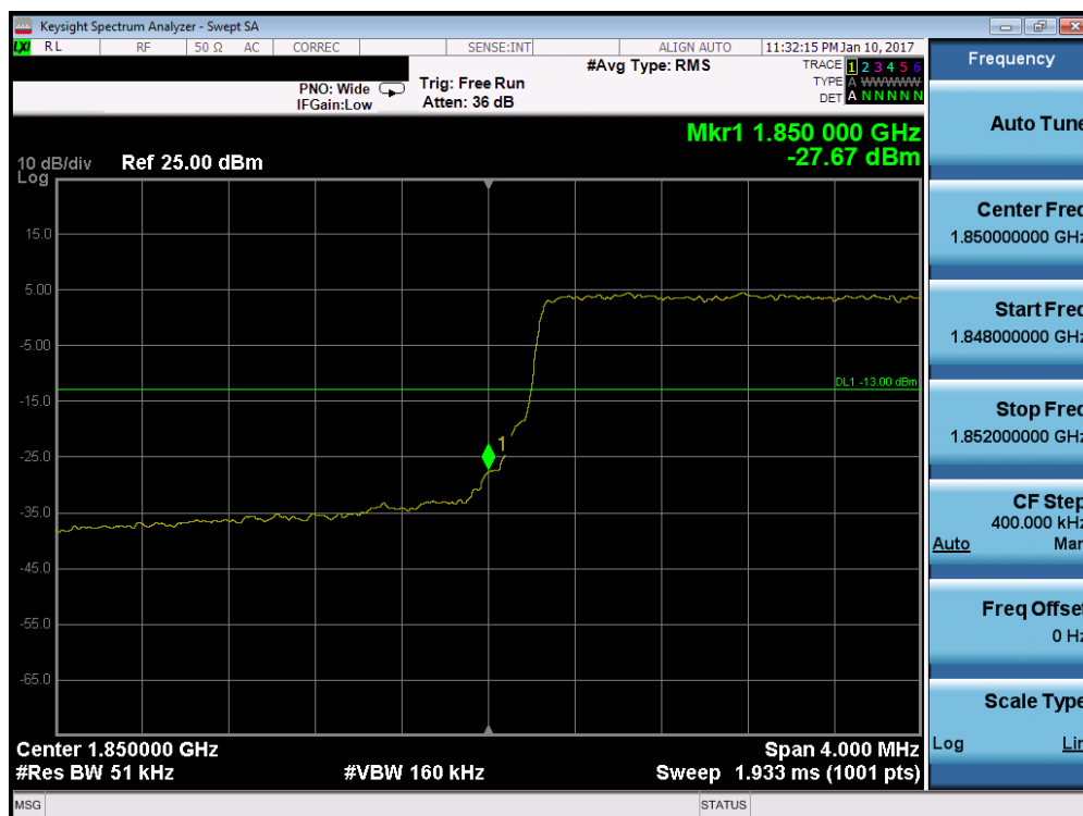
Plot 7-90. Lower Band Edge Plot (Band 2 – 5.0MHz QPSK – RB Size 25)
