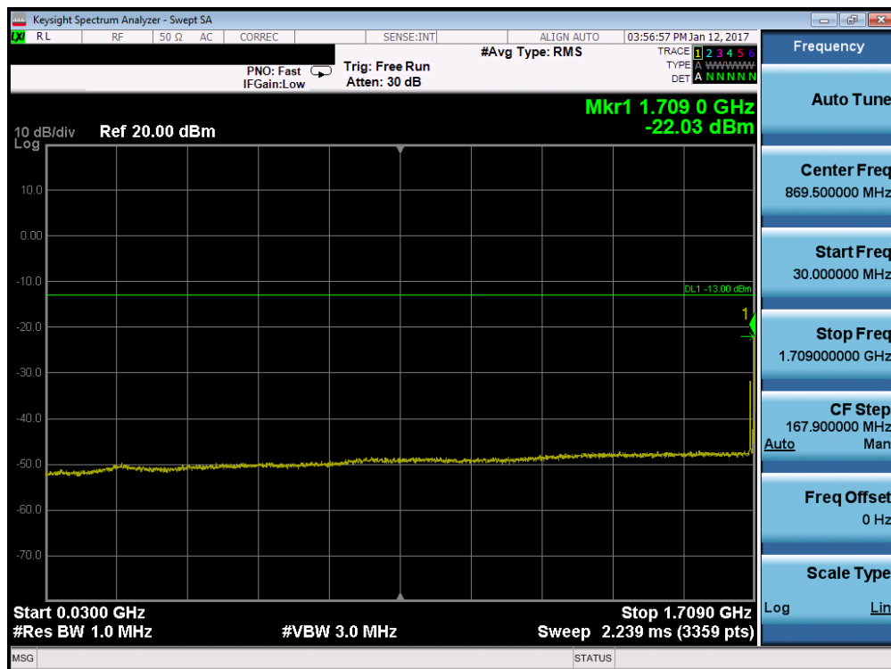
Plot 7-32. Conducted Spurious Plot (Band 4 – 15.0MHz QPSK – RB Size 1, RB Offset 0 – Low Channel)
