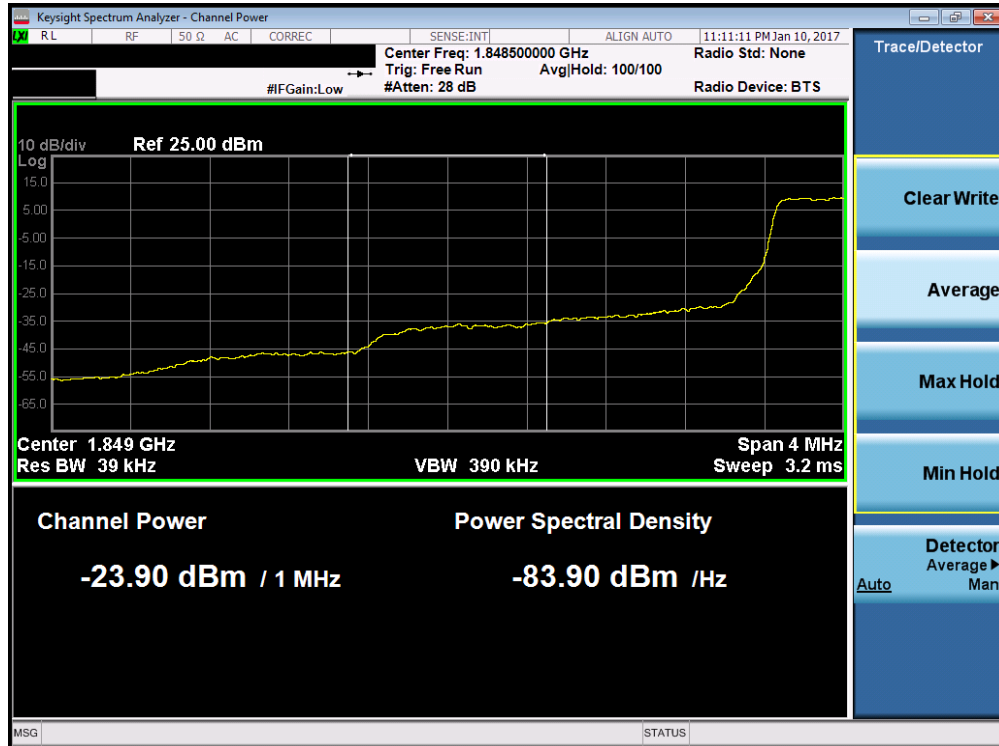
Plot 7-83. Lower Extended Band Edge Plot (Band 2 – 1.4MHz QPSK – RB Size 6)
