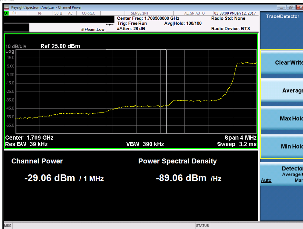
Plot 7-59. Lower Extended Band Edge Plot (Band 4 – 1.4MHz QPSK – RB Size 6)
