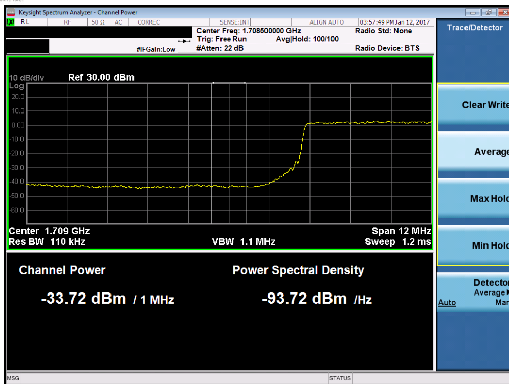
Plot 7-75. Lower Extended Band Edge Plot (Band 4 – 15.0MHz QPSK – RB Size 75)
