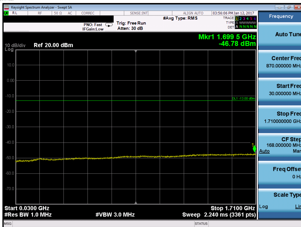
Plot 7-35. Conducted Spurious Plot (Band 4 – 15.0MHz QPSK – RB Size 1, RB Offset 0 – Mid Channel)
