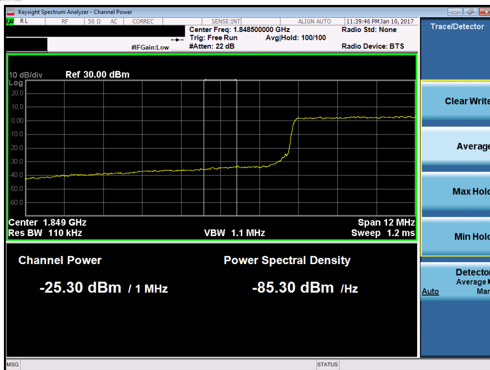
Plot 7-99. Lower Extended Band Edge Plot (Band 2 – 15.0MHz QPSK – RB Size 75)
