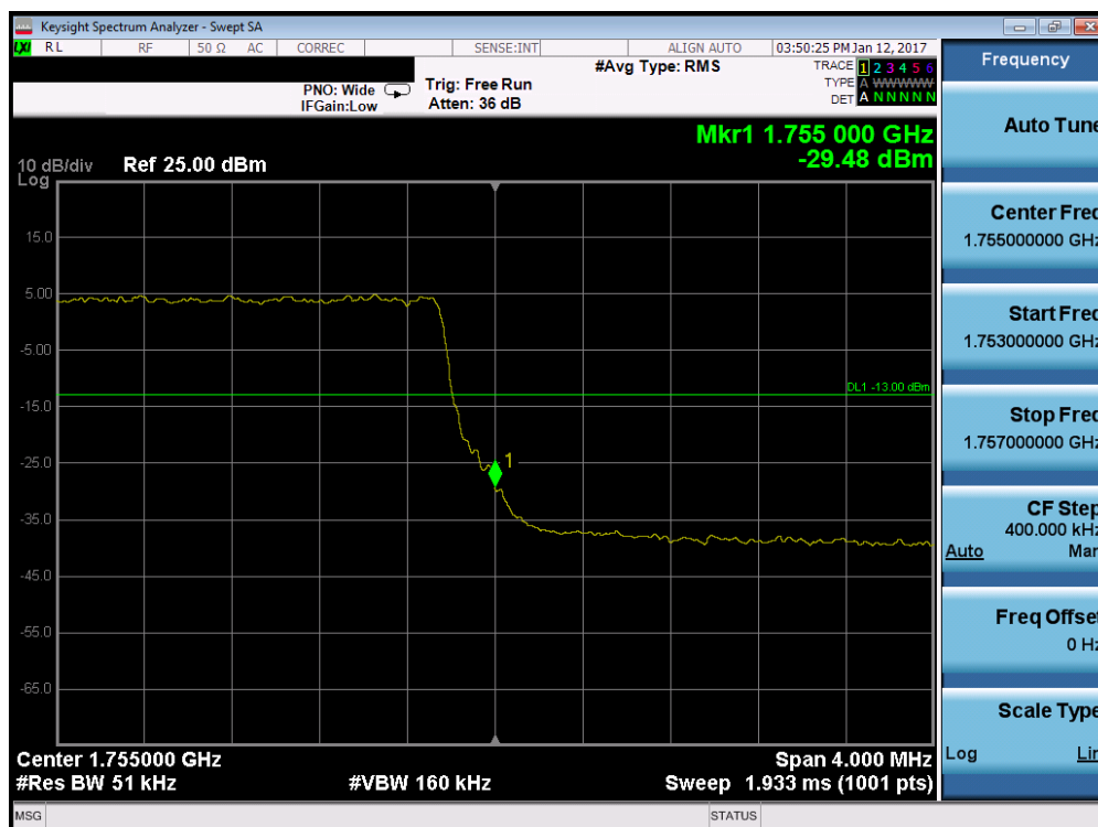
Plot 7-68. Upper Band Edge Plot (Band 4 – 5.0MHz QPSK – RB Size 25)
