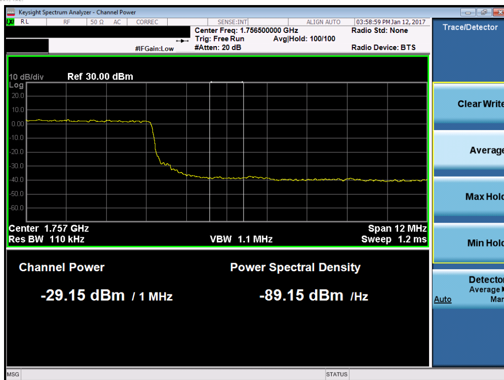
Plot 7-77. Upper Extended Band Edge Plot (Band 4 – 15.0MHz QPSK – RB Size 75)
