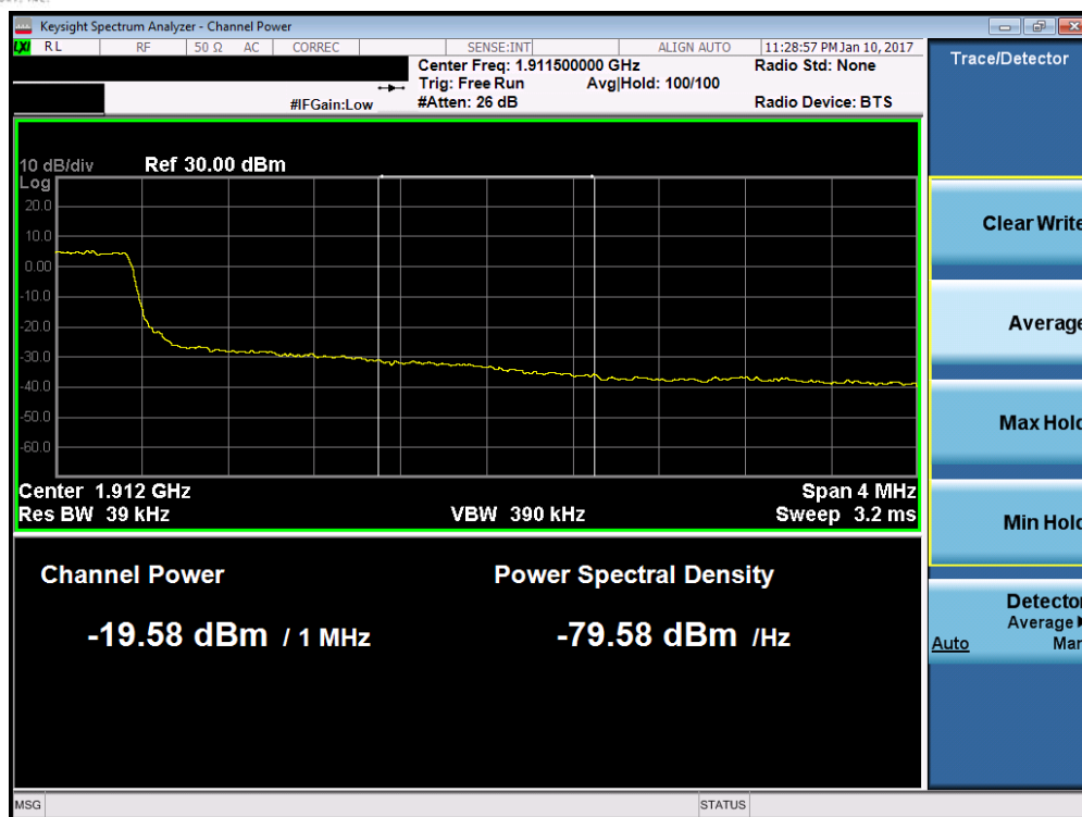
Plot 7-89. Upper Extended Band Edge Plot (Band 2 – 3.0MHz QPSK – RB Size 15)
