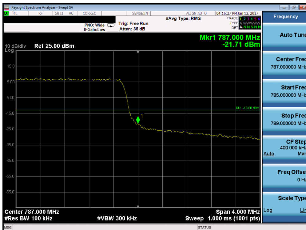
Plot 7-52. Upper Band Edge Plot (Band 13 – 5.0MHz QPSK – RB Size 25)
