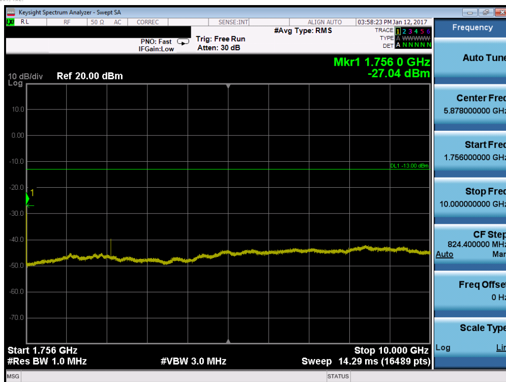
Plot 7-39. Conducted Spurious Plot (Band 4 – 15.0MHz QPSK – RB Size 1, RB Offset 0 – High Channel)
