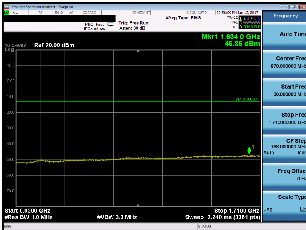
Plot 7-38. Conducted Spurious Plot (Band 4 – 15.0MHz QPSK – RB Size 1, RB Offset 0 – High Channel)
