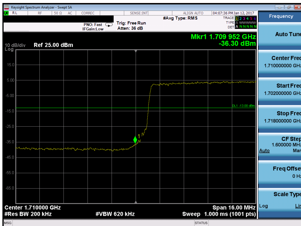
Plot 7-78. Lower Band Edge Plot (Band 4 – 20.0MHz QPSK – RB Size 100)
