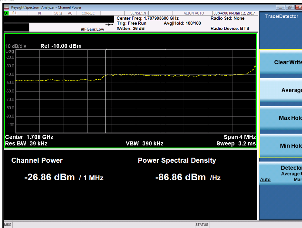
Plot 7-63. Lower Extended Band Edge Plot (Band 4 – 3.0MHz QPSK – RB Size 15)
