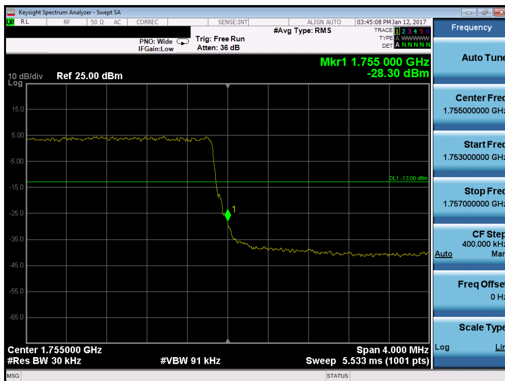
Plot 7-64. Upper Band Edge Plot (Band 4 – 3.0MHz QPSK – RB Size 15)
