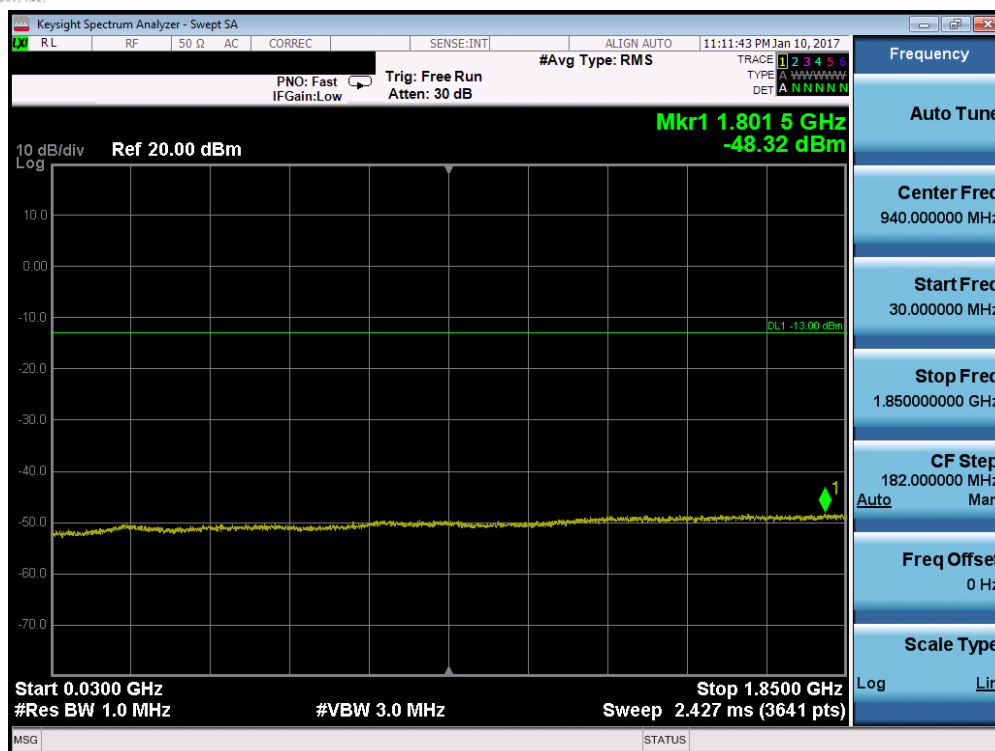
Plot 7-47. Conducted Spurious Plot (Band 2 – 1.4MHz QPSK – RB Size 1, RB Offset 0 – High Channel)
