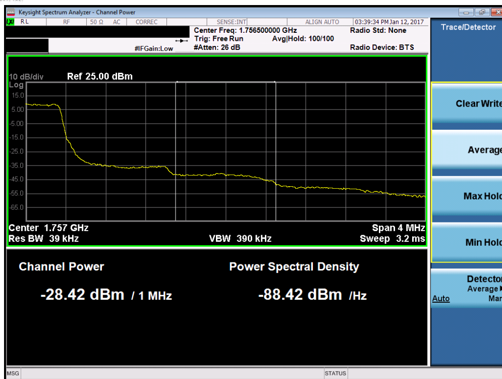
Plot 7-61. Upper Extended Band Edge Plot (Band 4 – 1.4MHz QPSK – RB Size 6)
