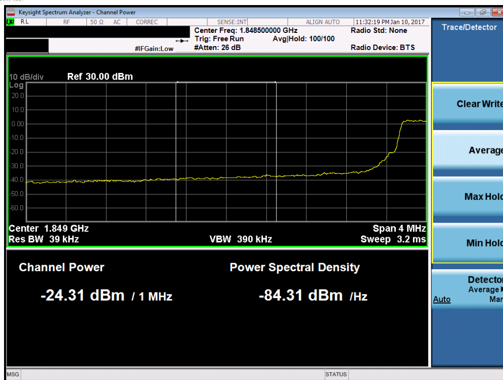
Plot 7-91. Lower Extended Band Edge Plot (Band 2 – 5.0MHz QPSK – RB Size 25)
