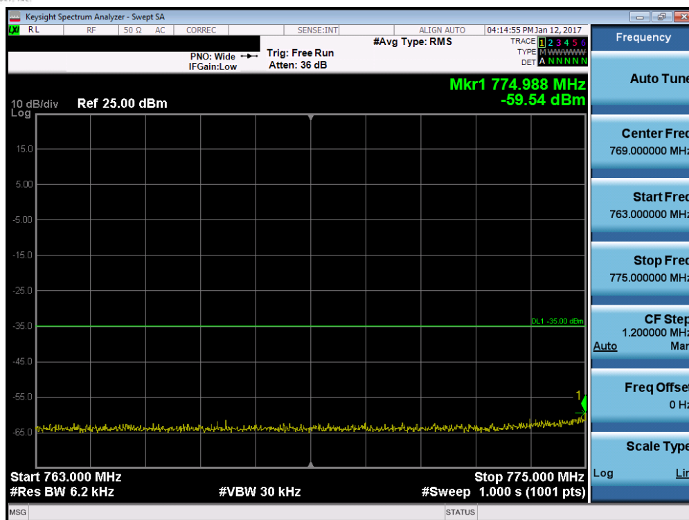
Plot 7-51. Lower Emission Mask Edge Plot (Band 13 – 5.0MHz QPSK – RB Size 25)
