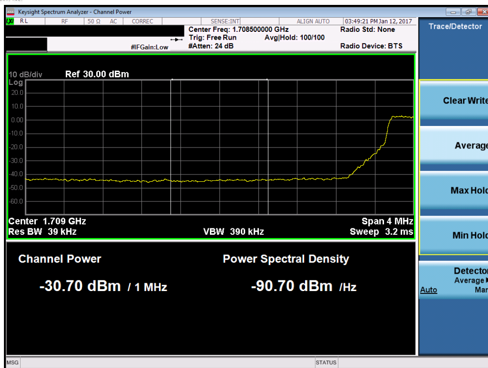
Plot 7-67. Lower Extended Band Edge Plot (Band 4 – 5.0MHz QPSK – RB Size 25)
