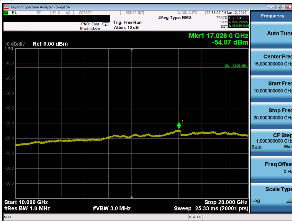
Plot 7-37. Conducted Spurious Plot (Band 4 – 15.0MHz QPSK – RB Size 1, RB Offset 0 – Mid Channel)
