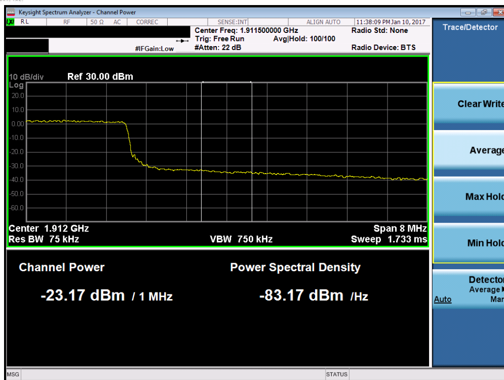
Plot 7-97. Upper Extended Band Edge Plot (Band 2 – 10.0MHz QPSK – RB Size 50)
