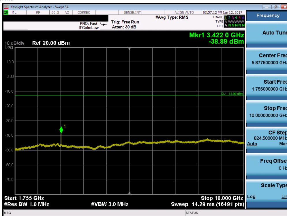
Plot 7-33. Conducted Spurious Plot (Band 4 – 15.0MHz QPSK – RB Size 1, RB Offset 0 – Low Channel)
