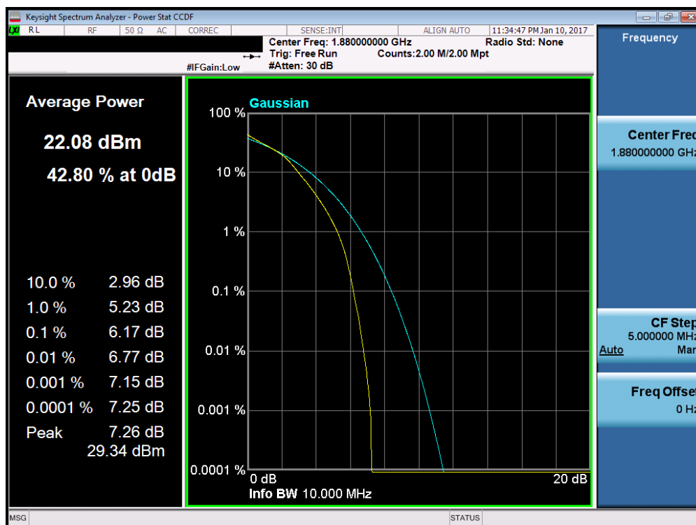
Plot 7-113. PAR Plot (Band 2 – 10.0MHz 16-QAM – RB Size 50)
