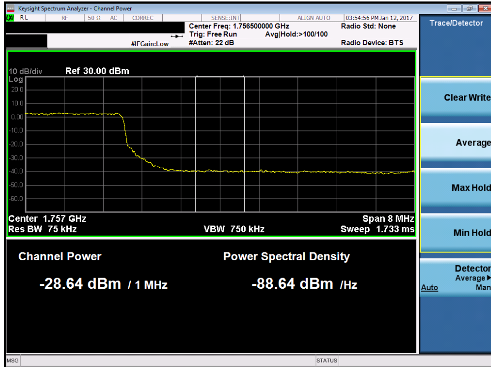
Plot 7-73. Upper Extended Band Edge Plot (Band 4 – 10.0MHz QPSK – RB Size 50)
