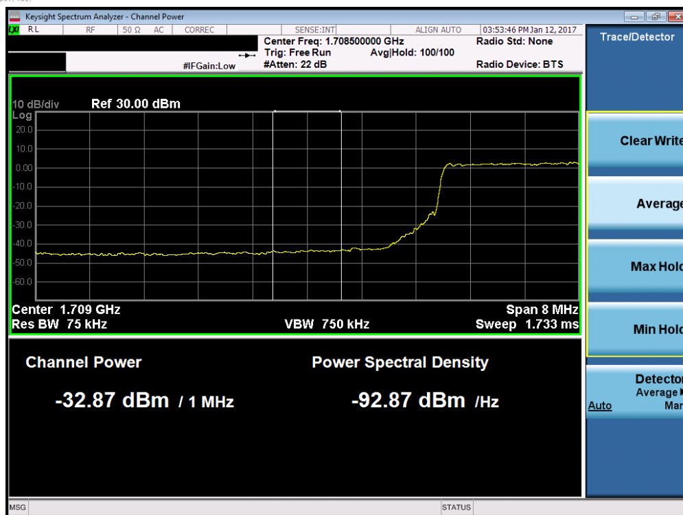
Plot 7-71. Lower Extended Band Edge Plot (Band 4 – 10.0MHz QPSK – RB Size 50)
