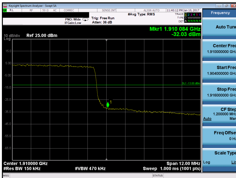
Plot 7-100. Upper Band Edge Plot (Band 2 – 15.0MHz QPSK – RB Size 75)
