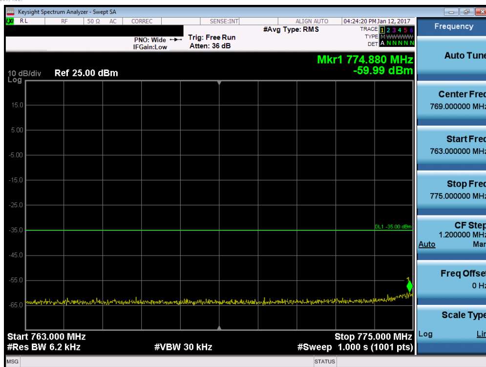
Plot 7-55. Lower Emission Mask Edge Plot (Band 13 – 10.0MHz QPSK – RB Size 50)
