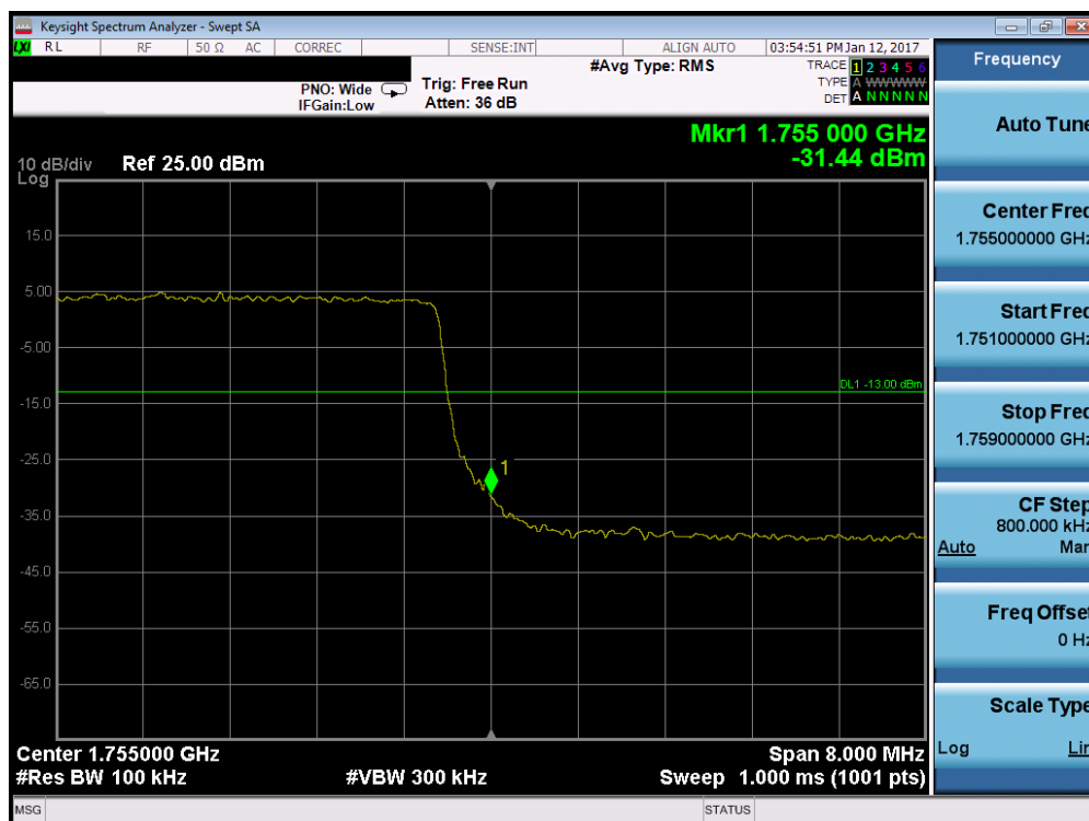
Plot 7-72. Upper Band Edge Plot (Band 4 – 10.0MHz QPSK – RB Size 50)
