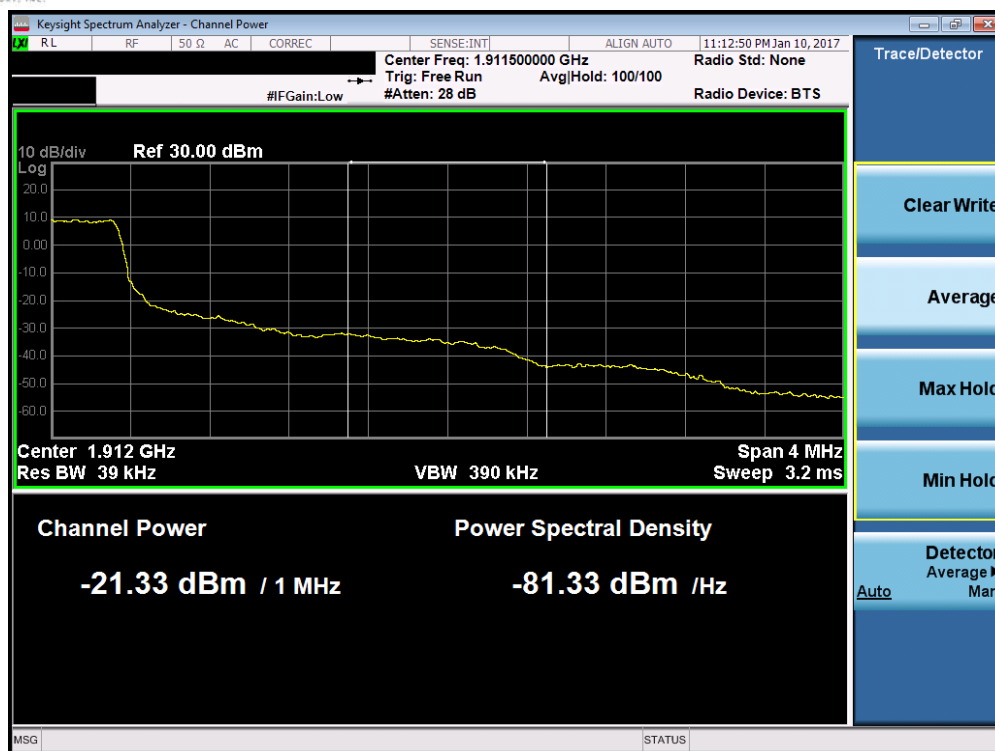
Plot 7-85. Upper Extended Band Edge Plot (Band 2 – 1.4MHz QPSK – RB Size 6)
