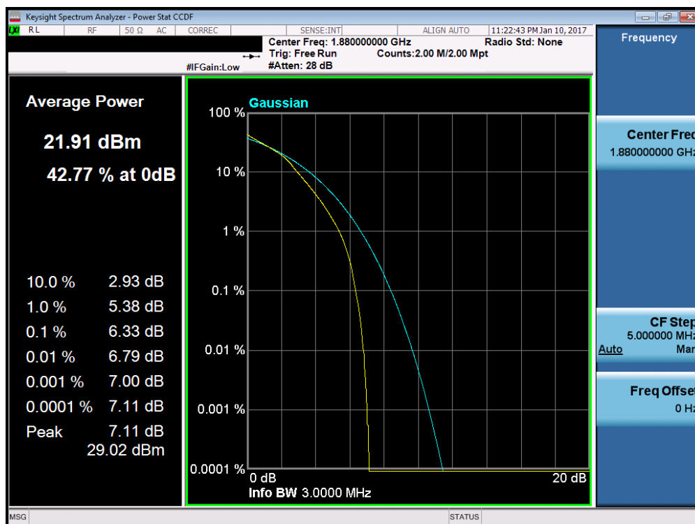
Plot 7-109. PAR Plot (Band 2 – 3.0MHz 16-QAM – RB Size 15)
