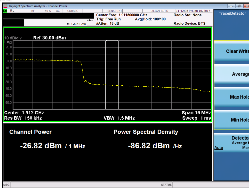
Plot 7-105. Upper Extended Band Edge Plot (Band 2 – 20.0MHz QPSK – RB Size 100)
