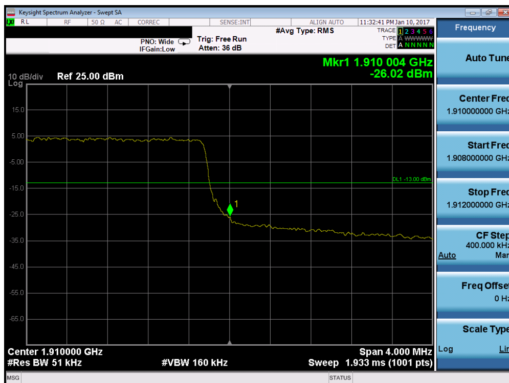
Plot 7-92. Upper Band Edge Plot (Band 2 – 5.0MHz QPSK – RB Size 25)
