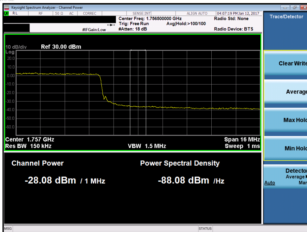
Plot 7-81. Upper Extended Band Edge Plot (Band 4 – 20.0MHz QPSK – RB Size 100)
