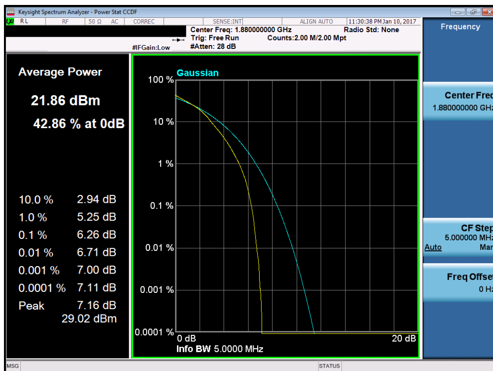
Plot 7-111. PAR Plot (Band 2 – 5.0MHz 16-QAM – RB Size 25)
