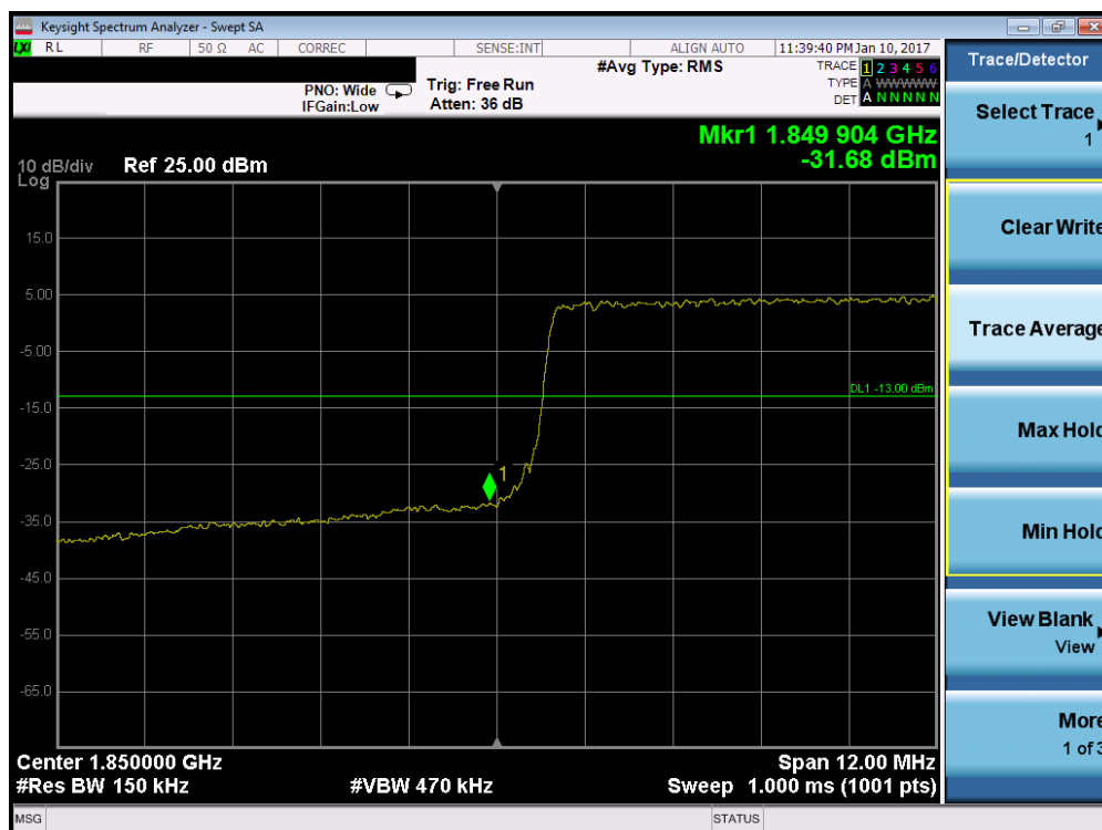
Plot 7-98. Lower Band Edge Plot (Band 2 – 15.0MHz QPSK – RB Size 75)
