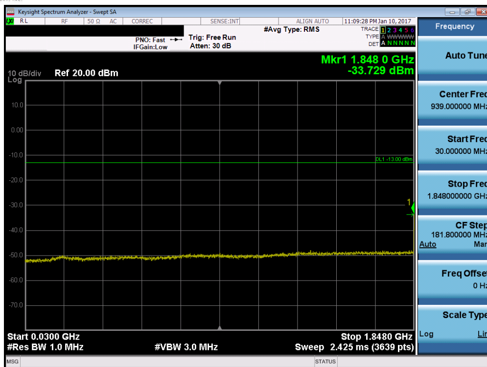
Plot 7-41. Conducted Spurious Plot (Band 2 – 1.4MHz QPSK – RB Size 1, RB Offset 0 – Low Channel)
