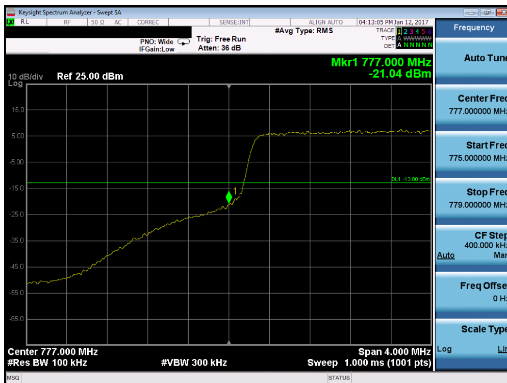
Plot 7-50. Lower Band Edge Plot (Band 13 – 5.0MHz QPSK – RB Size 25)
