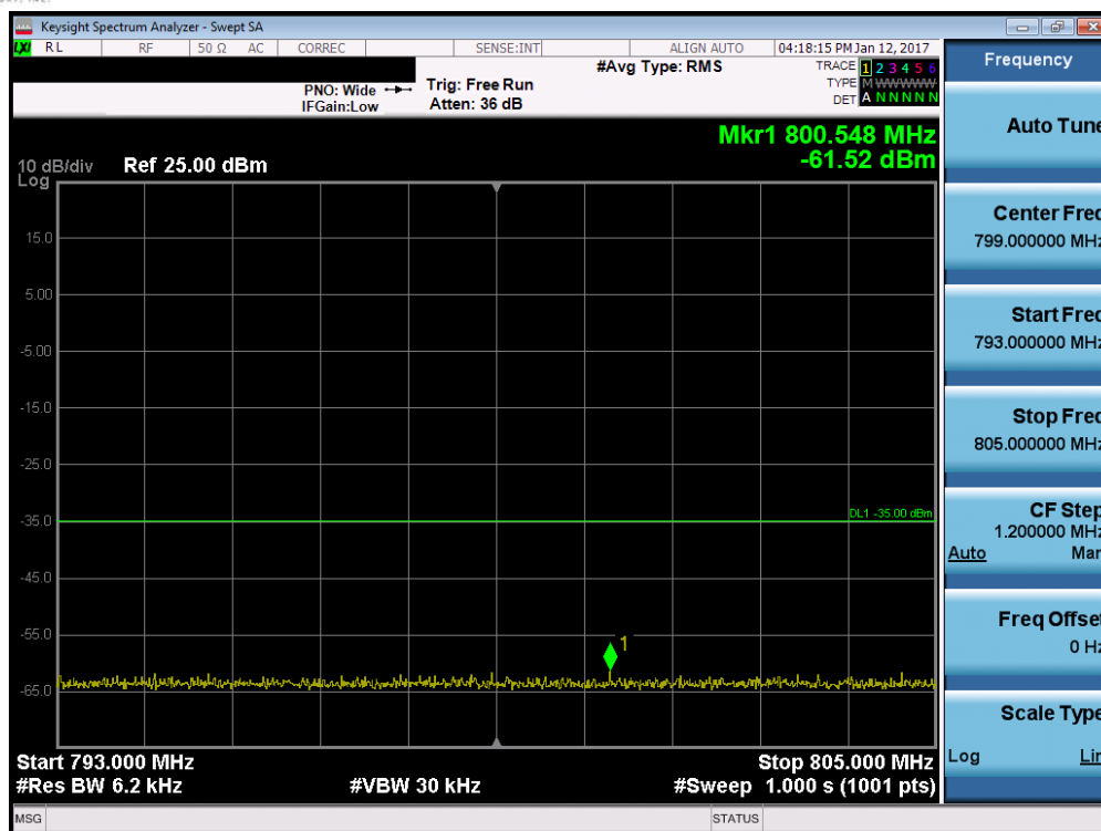
Plot 7-53. Upper Emission Mask Edge Plot (Band 13 – 5.0MHz QPSK – RB Size 25)
