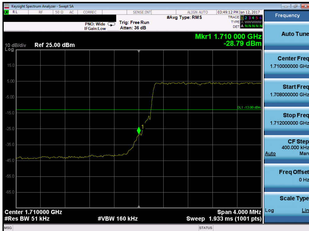
Plot 7-66. Lower Band Edge Plot (Band 4 – 5.0MHz QPSK – RB Size 25)
