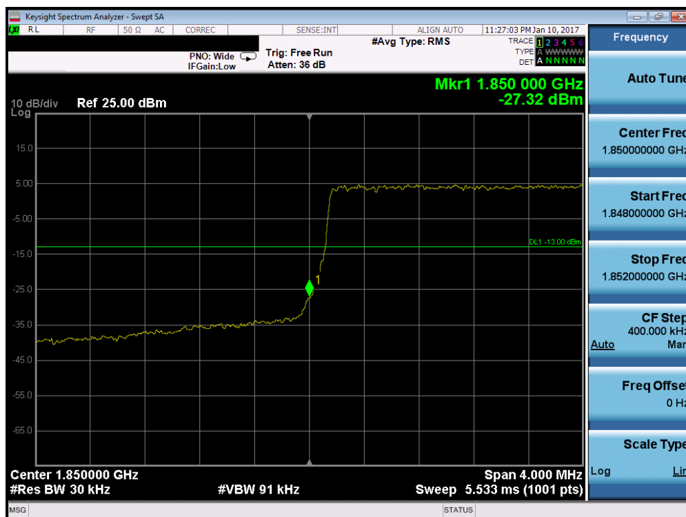
Plot 7-86. Lower Band Edge Plot (Band 2 – 3.0MHz QPSK – RB Size 15)
