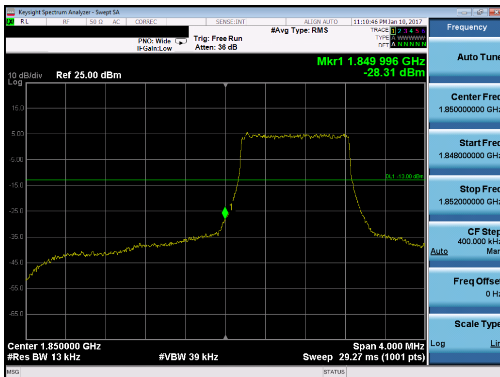
Plot 7-82. Lower Band Edge Plot (Band 2 – 1.4MHz QPSK – RB Size 6)
