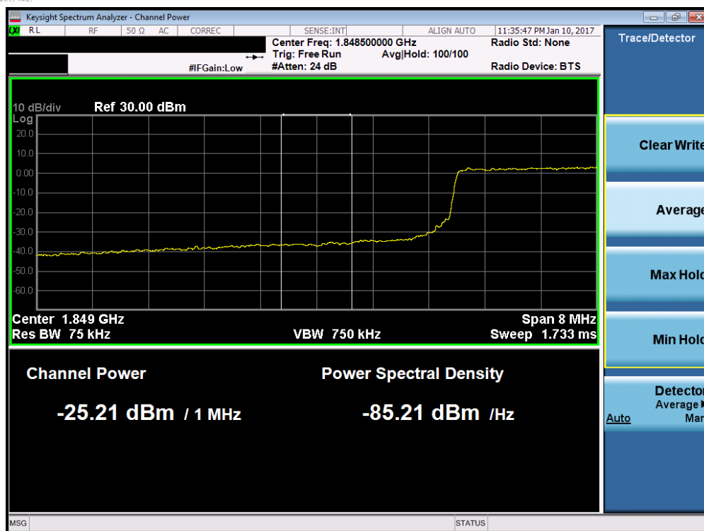
Plot 7-95. Lower Extended Band Edge Plot (Band 2 – 10.0MHz QPSK – RB Size 50)
