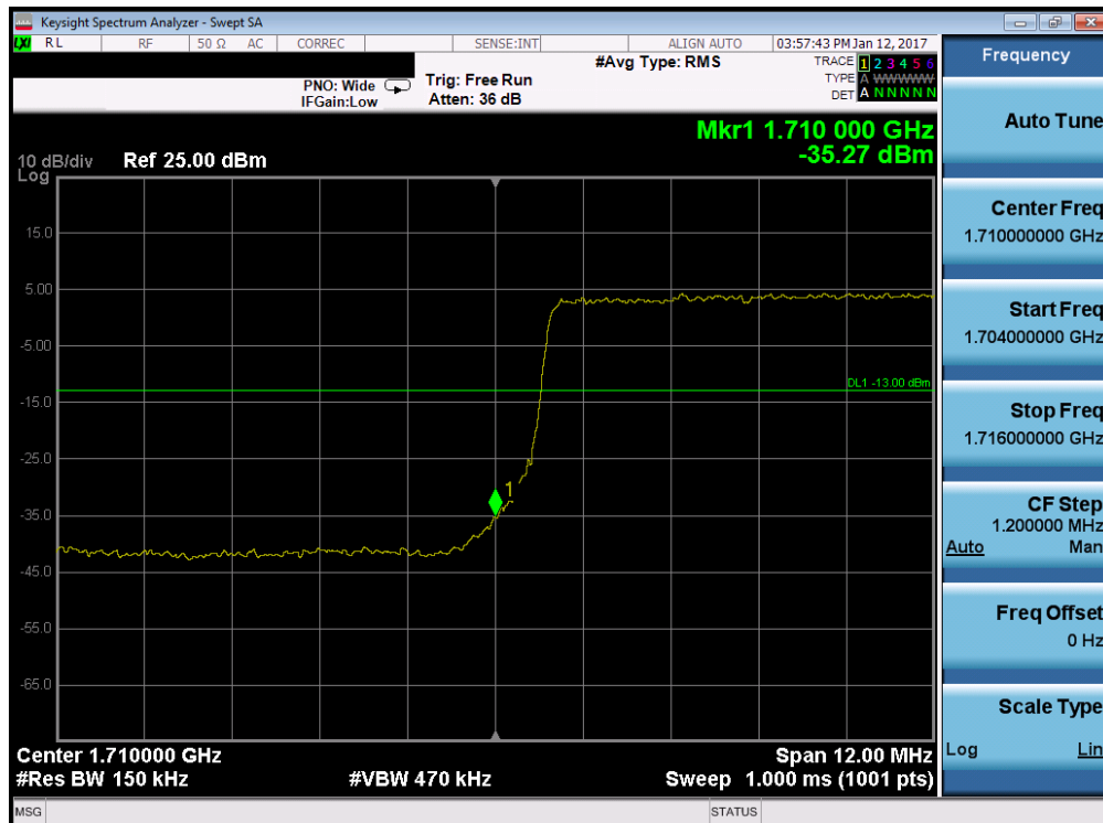
Plot 7-74. Lower Band Edge Plot (Band 4 – 15.0MHz QPSK – RB Size 75)
