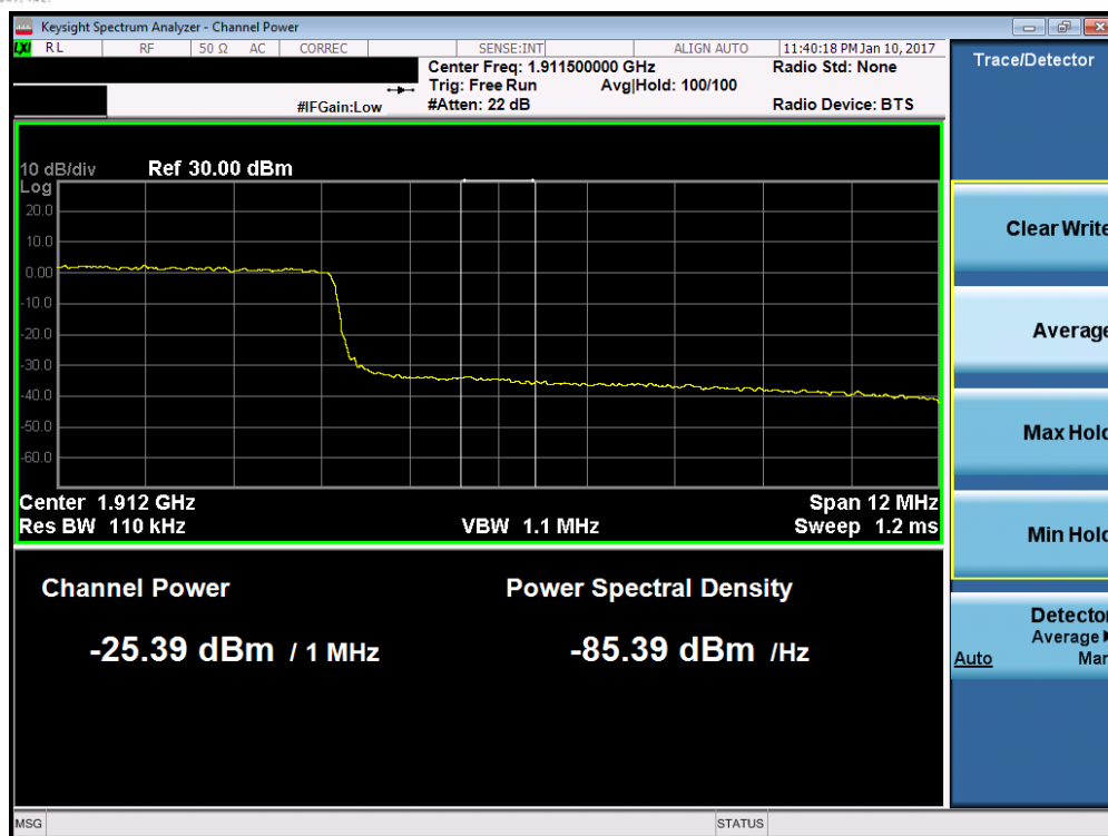
Plot 7-101. Upper Extended Band Edge Plot (Band 2 – 15.0MHz QPSK – RB Size 75)
