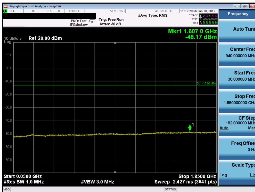
Plot 7-44. Conducted Spurious Plot (Band 2 – 1.4MHz QPSK – RB Size 1, RB Offset 0 – Mid Channel)
