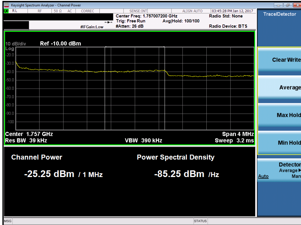
Plot 7-65. Upper Extended Band Edge Plot (Band 4 – 3.0MHz QPSK – RB Size 15)
