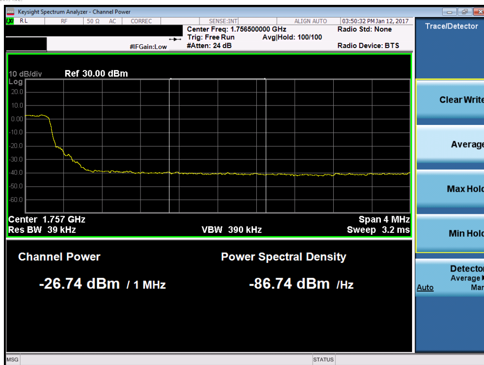
Plot 7-69. Upper Extended Band Edge Plot (Band 4 – 5.0MHz QPSK – RB Size 25)
