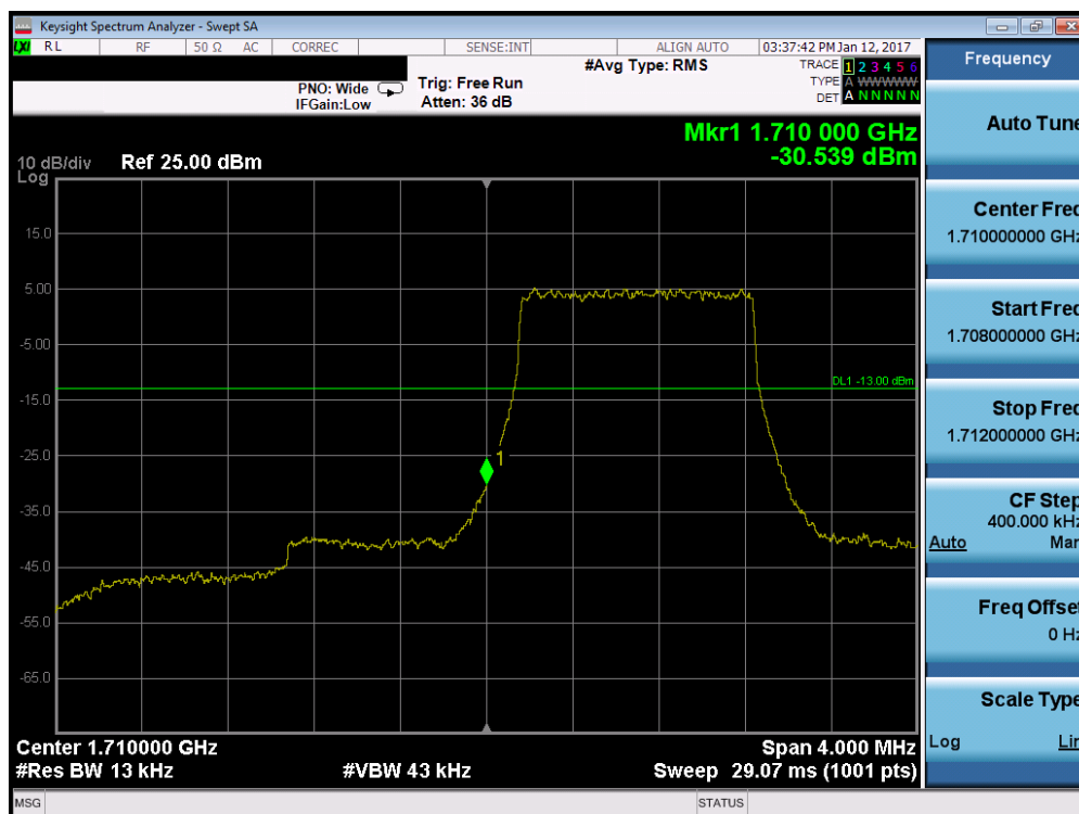
Plot 7-58. Lower Band Edge Plot (Band 4 – 1.4MHz QPSK – RB Size 6)
