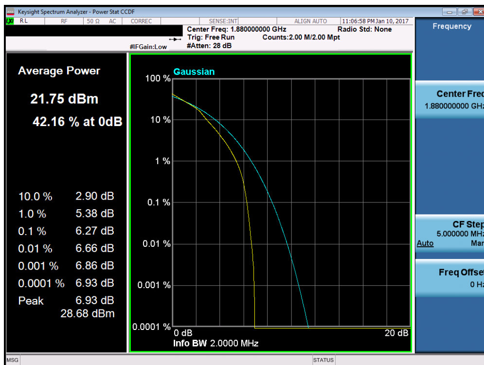
Plot 7-107. PAR Plot (Band 2 – 1.4MHz 16-QAM – RB Size 6)
