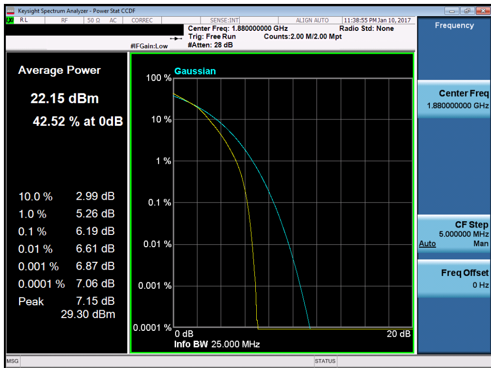
Plot 7-115. PAR Plot (Band 2 – 15.0MHz 16-QAM – RB Size 75)
