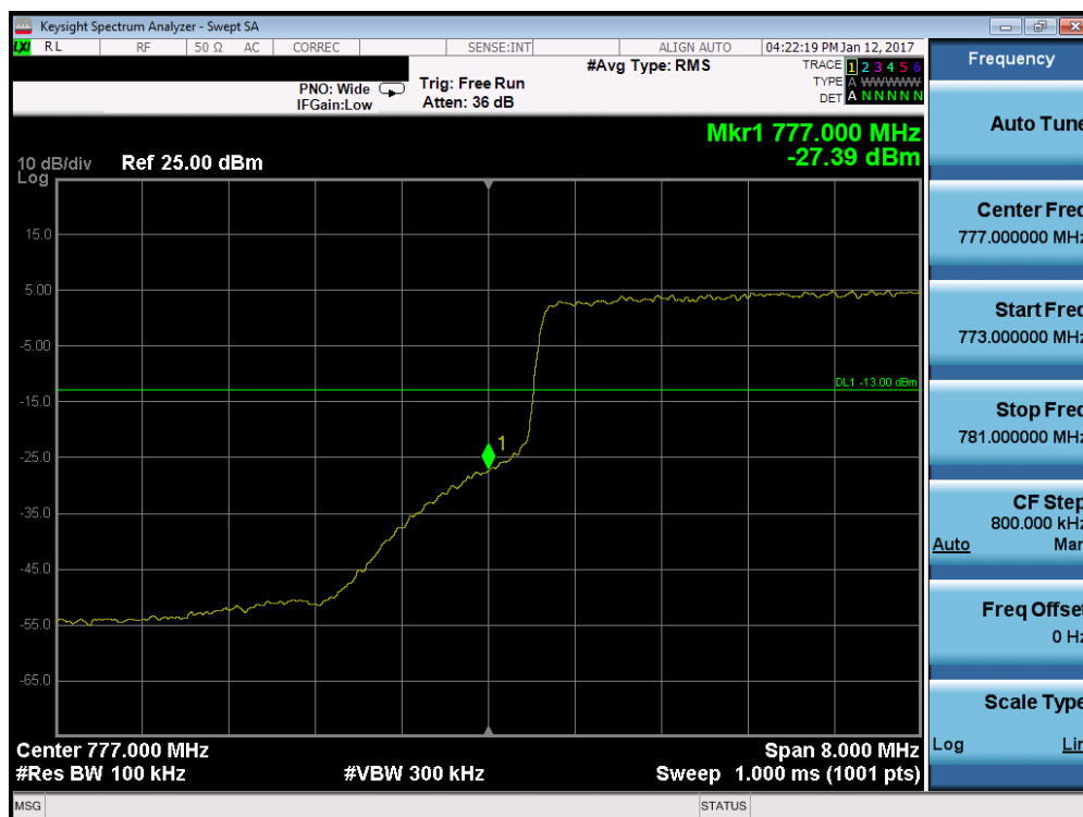
Plot 7-54. Lower Band Edge Plot (Band 13 – 10.0MHz QPSK – RB Size 50)
