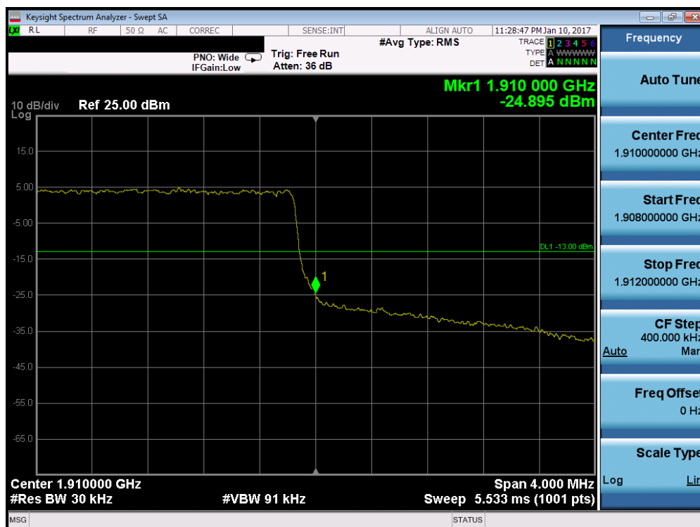
Plot 7-88. Upper Band Edge Plot (Band 2 – 3.0MHz QPSK – RB Size 15)
