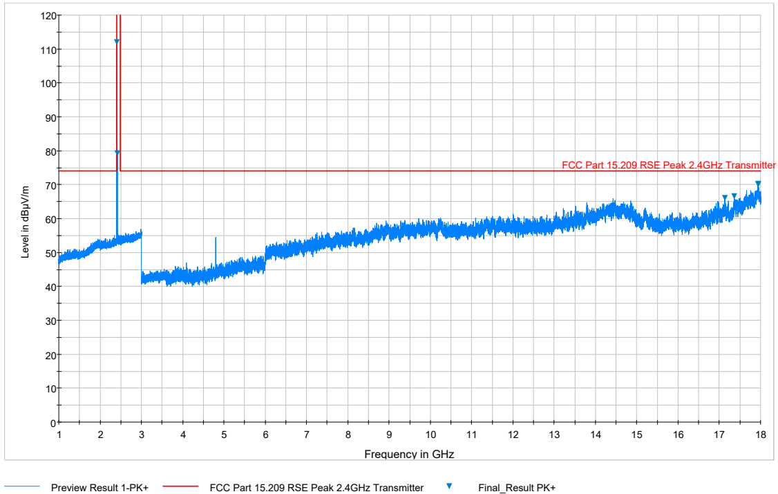
Plot 7-42. Radiated Spurious Plot above 1GHz (BT – Ch. 0, Ant. Pol. H)
