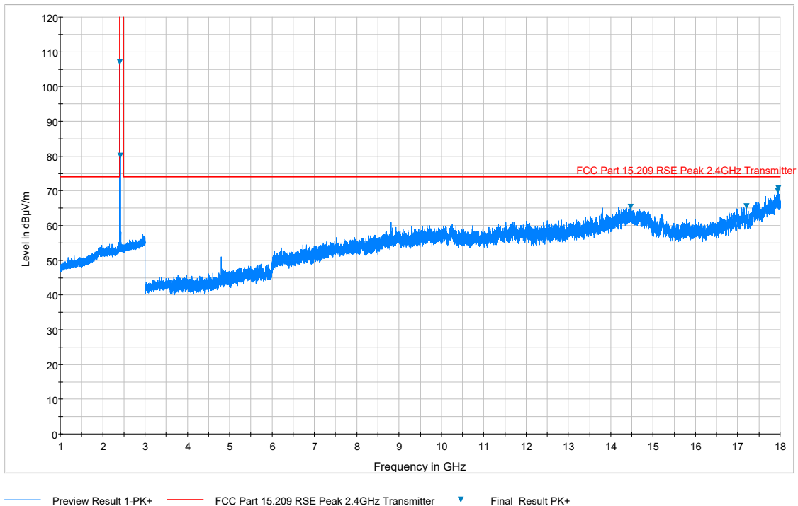
Plot 7-43. Radiated Spurious Plot above 1GHz (BT – Ch. 0, Ant. Pol. V)
