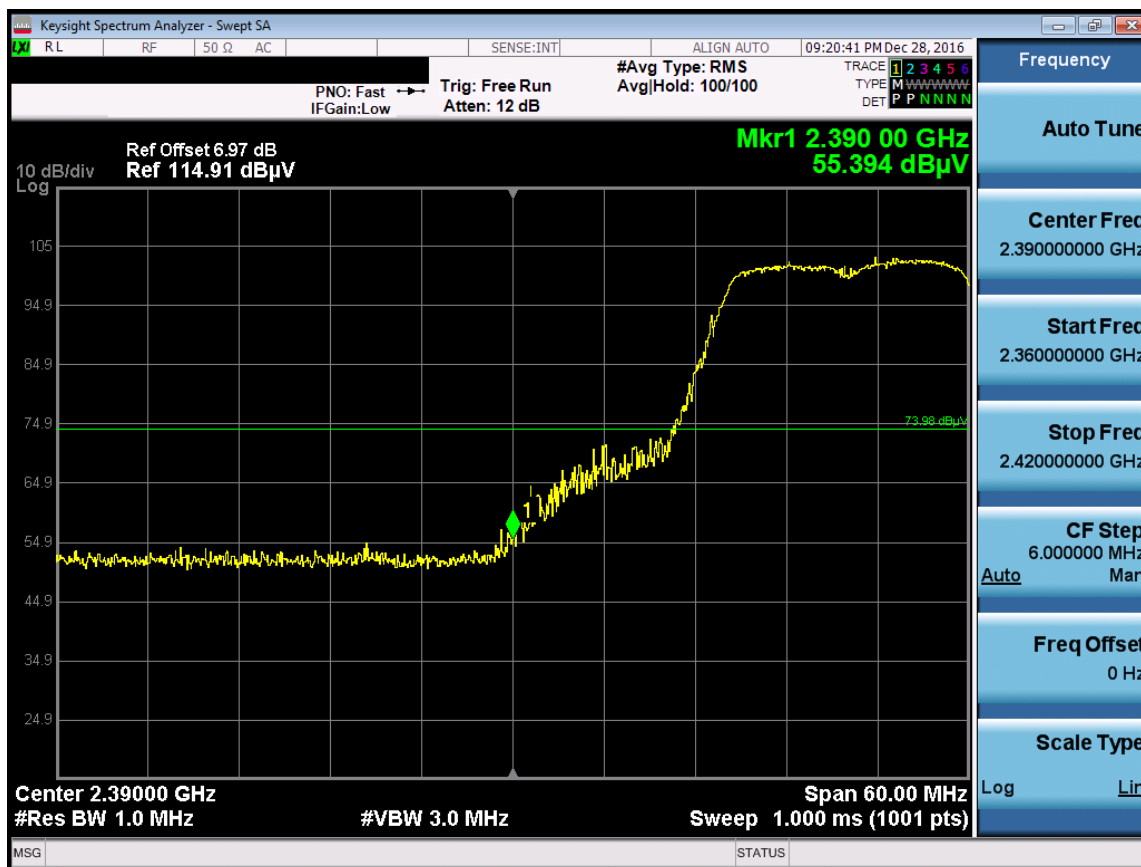
Plot 7-40. Radiated Restricted Lower Band Edge Measurement (Peak)
