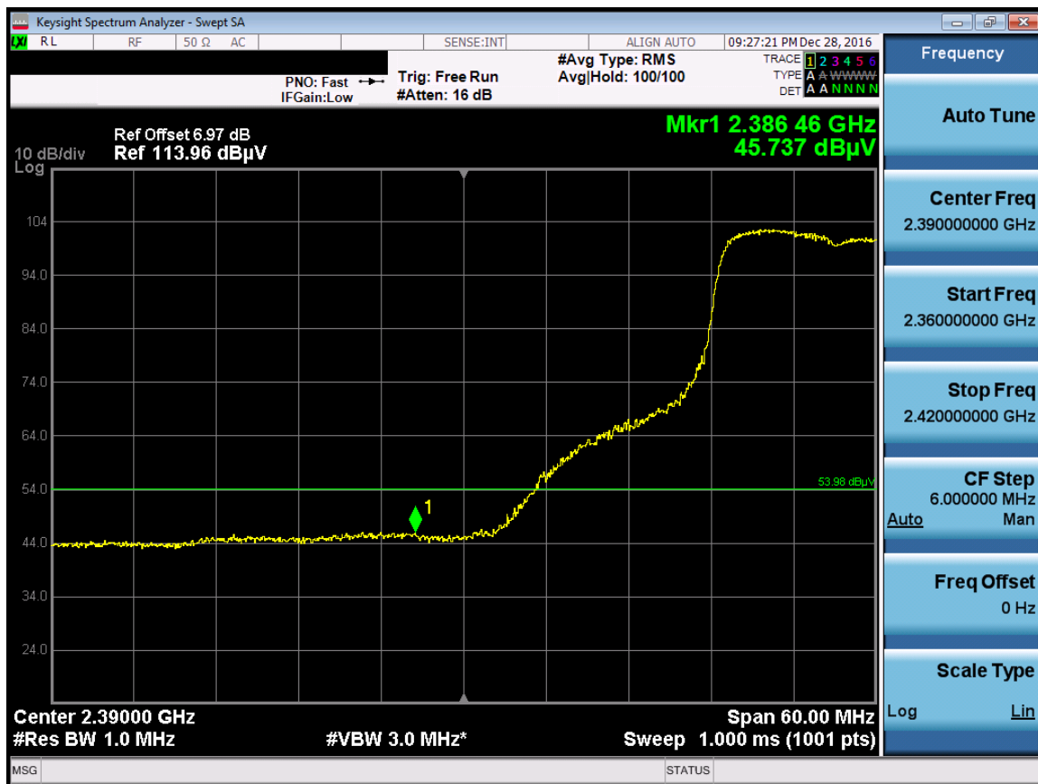
Plot 7-41. Radiated Restricted Lower Band Edge Measurement (Average)
