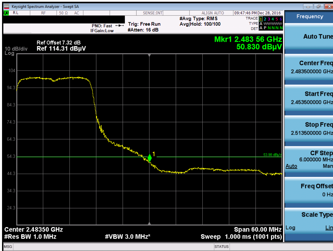
Plot 7-45. Radiated Restricted Upper Band Edge Measurement (Average)
