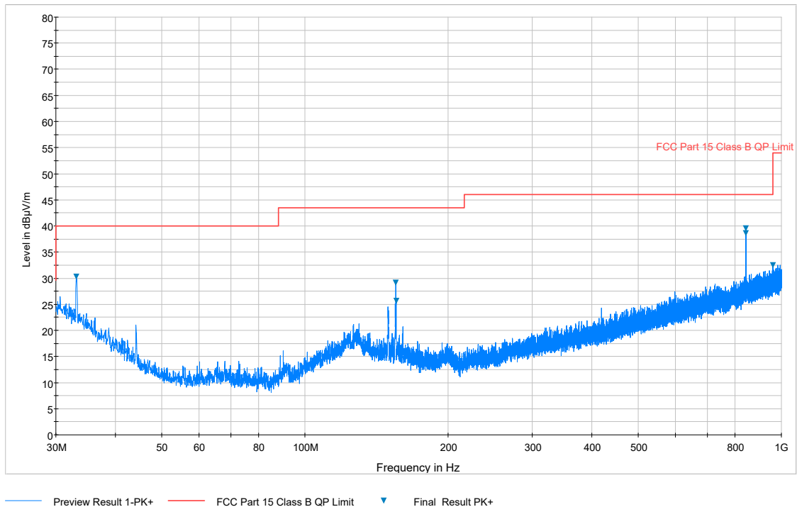
Plot 7-48. Radiated Spurious Plot below 1GHz (Pol. V)
