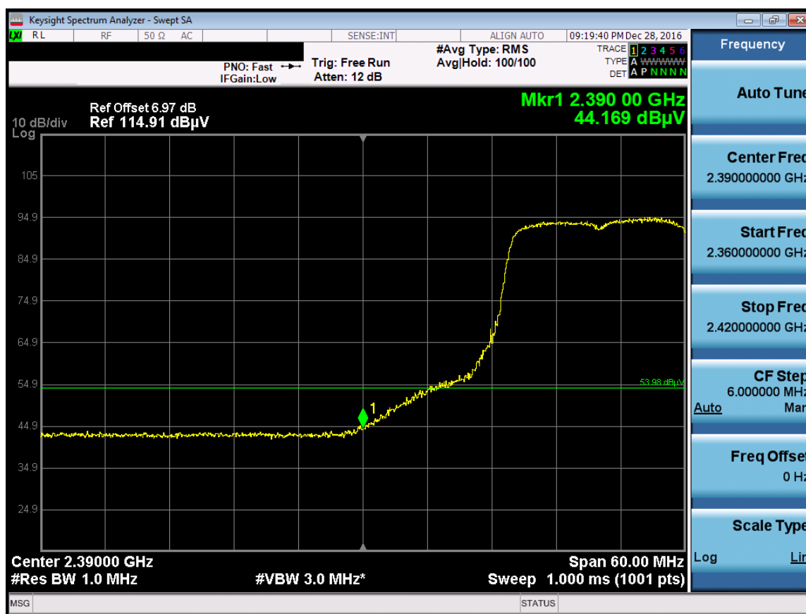
Plot 7-39. Radiated Restricted Lower Band Edge Measurement (Average)
