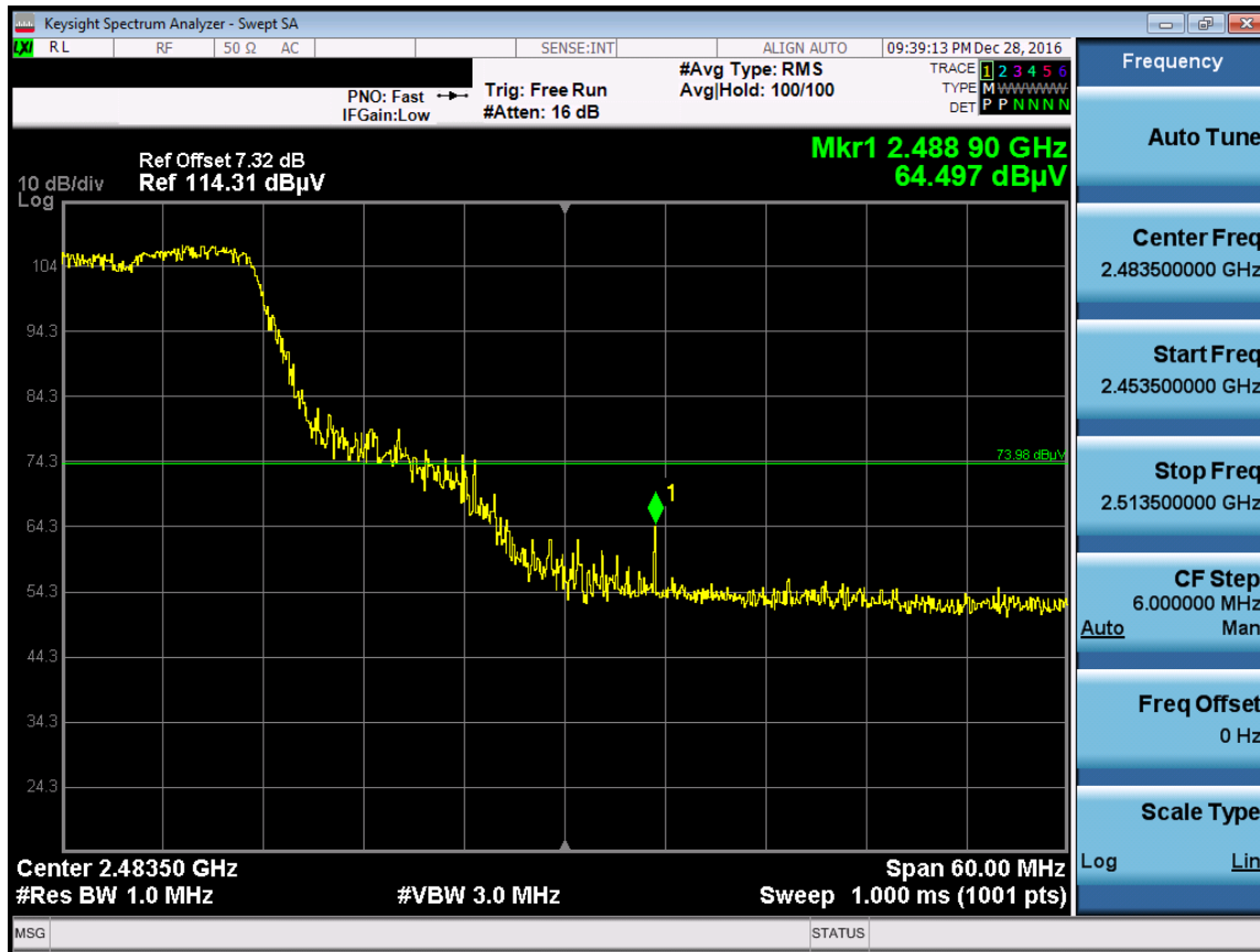
Plot 7-44. Radiated Restricted Upper Band Edge Measurement (Peak)
