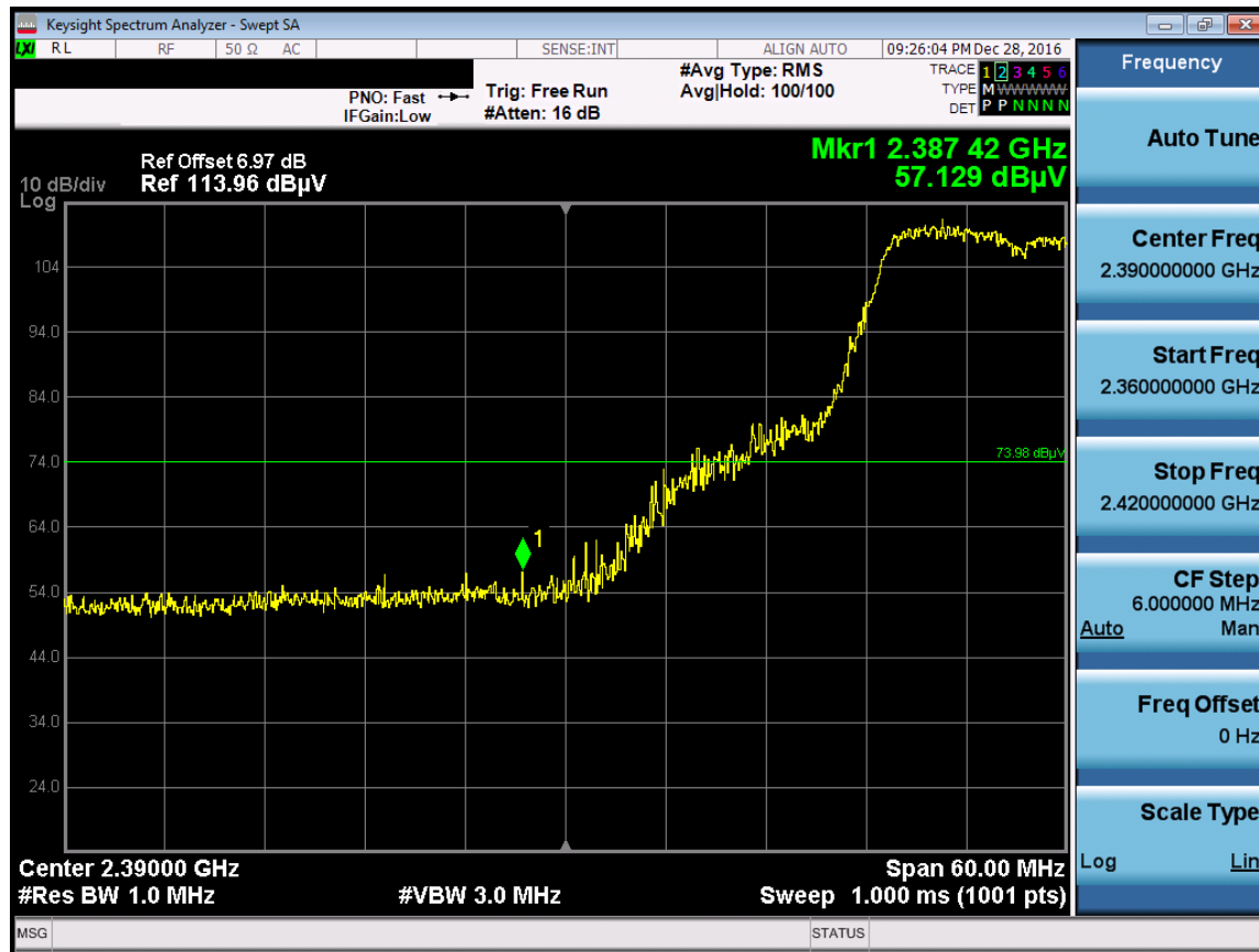
Plot 7-42. Radiated Restricted Lower Band Edge Measurement (Peak)
