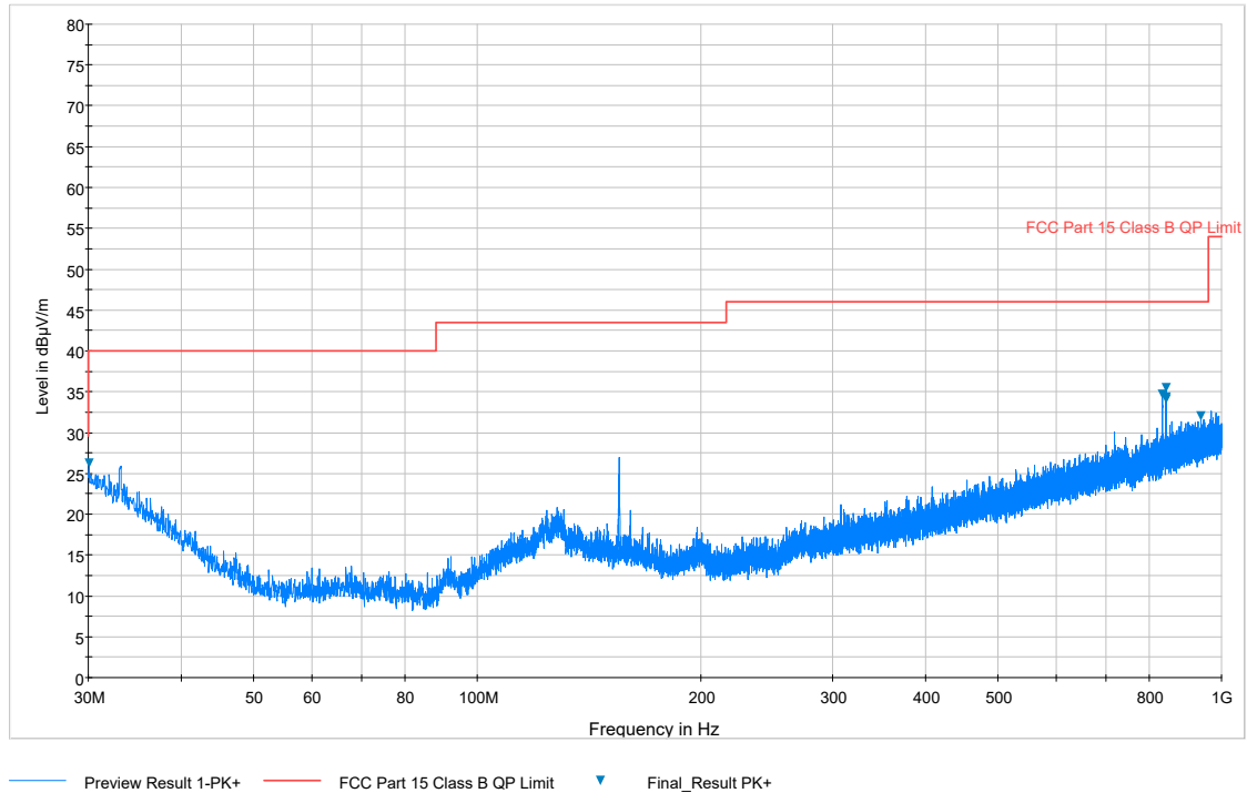
Plot 7-47. Radiated Spurious Plot below 1GHz (Pol. H)
