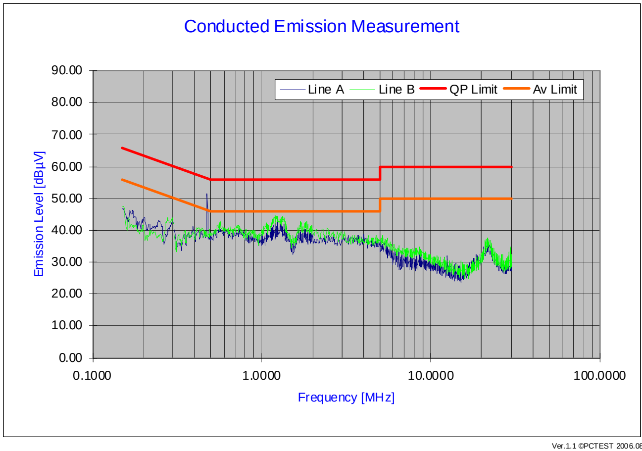
Plot 6-32. Line Conducted Plot with 802.11g
