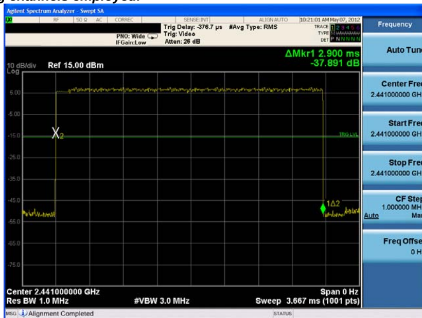
Plot 6-15. Time of Occupancy Plot (Bluetooth)
