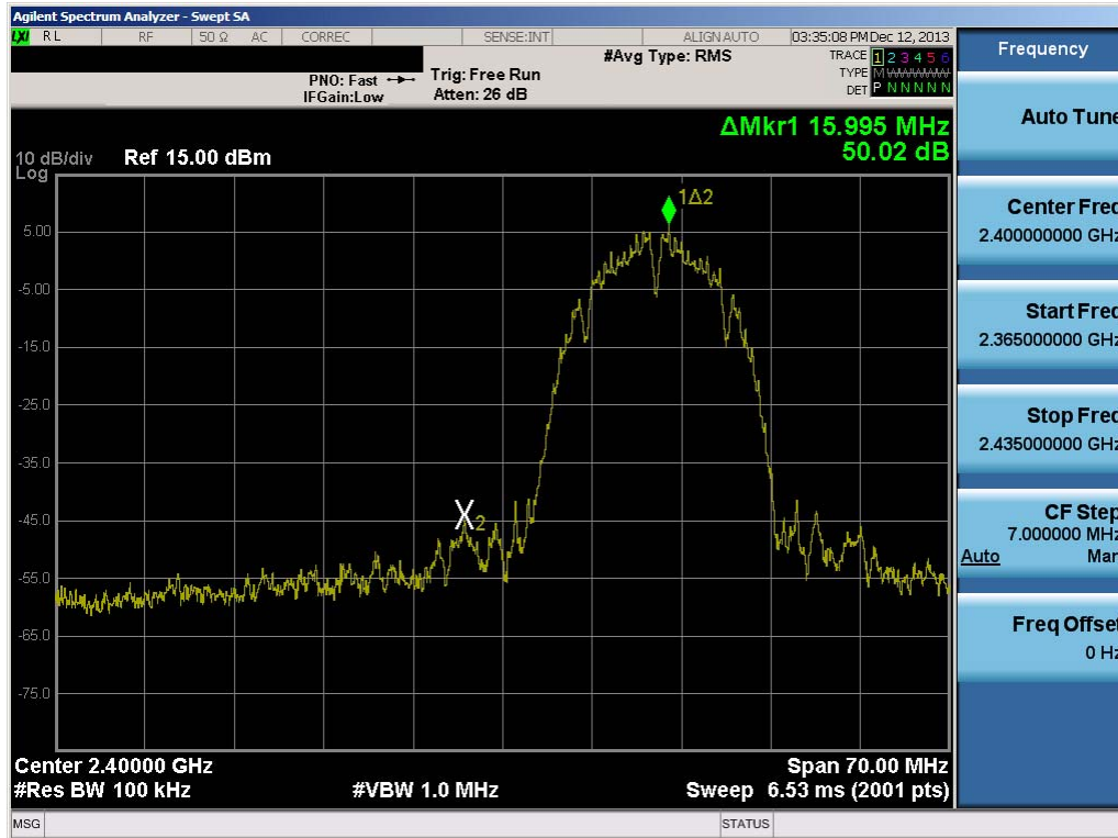
Plot 6-13. Band Edge Plot (802.11b – Ch. 1)
