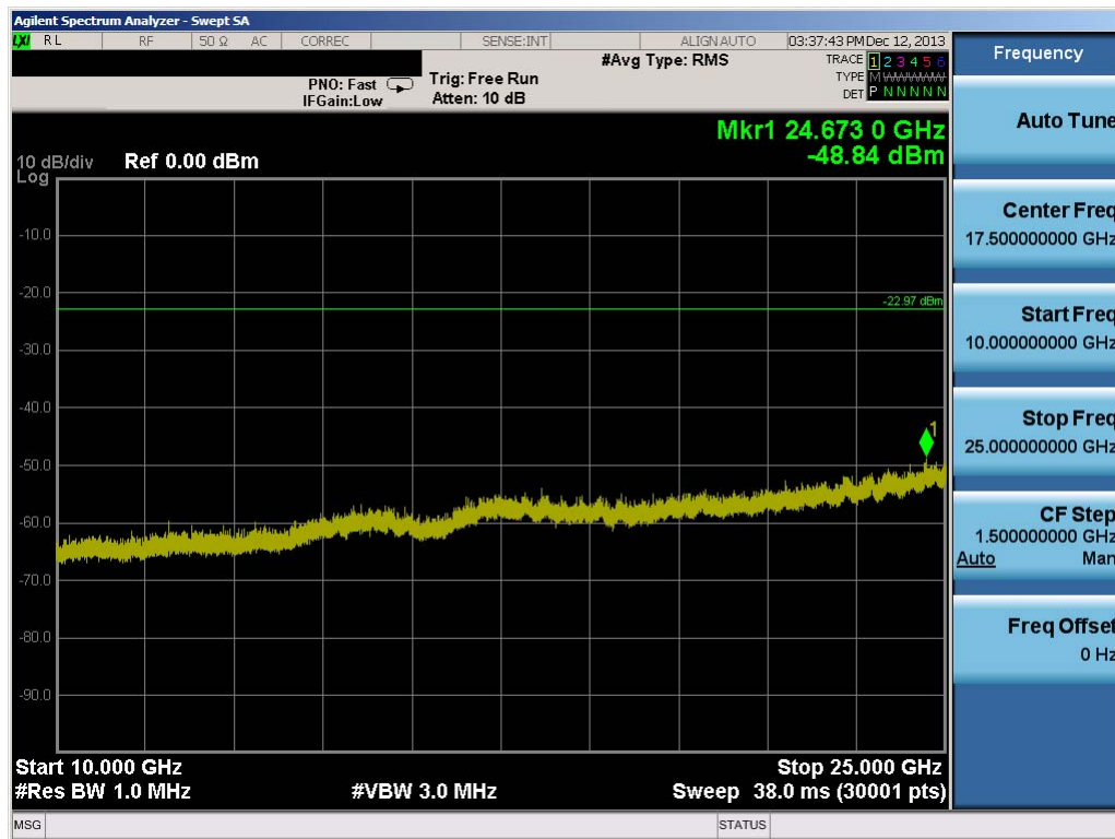
Plot 6-20. Conducted Spurious Plot (802.11b – Ch. 6)
