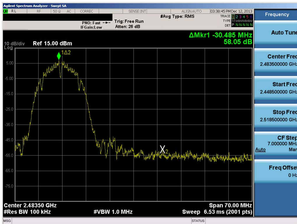
Plot 6-14. Band Edge Plot (802.11b – Ch. 11)
