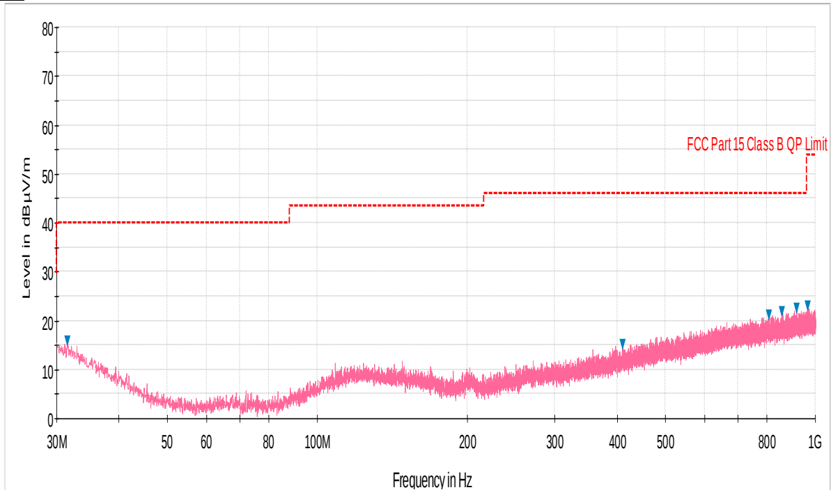
Plot 6-9. Radiated Spurious Plot below 1GHz (Pol. H)
