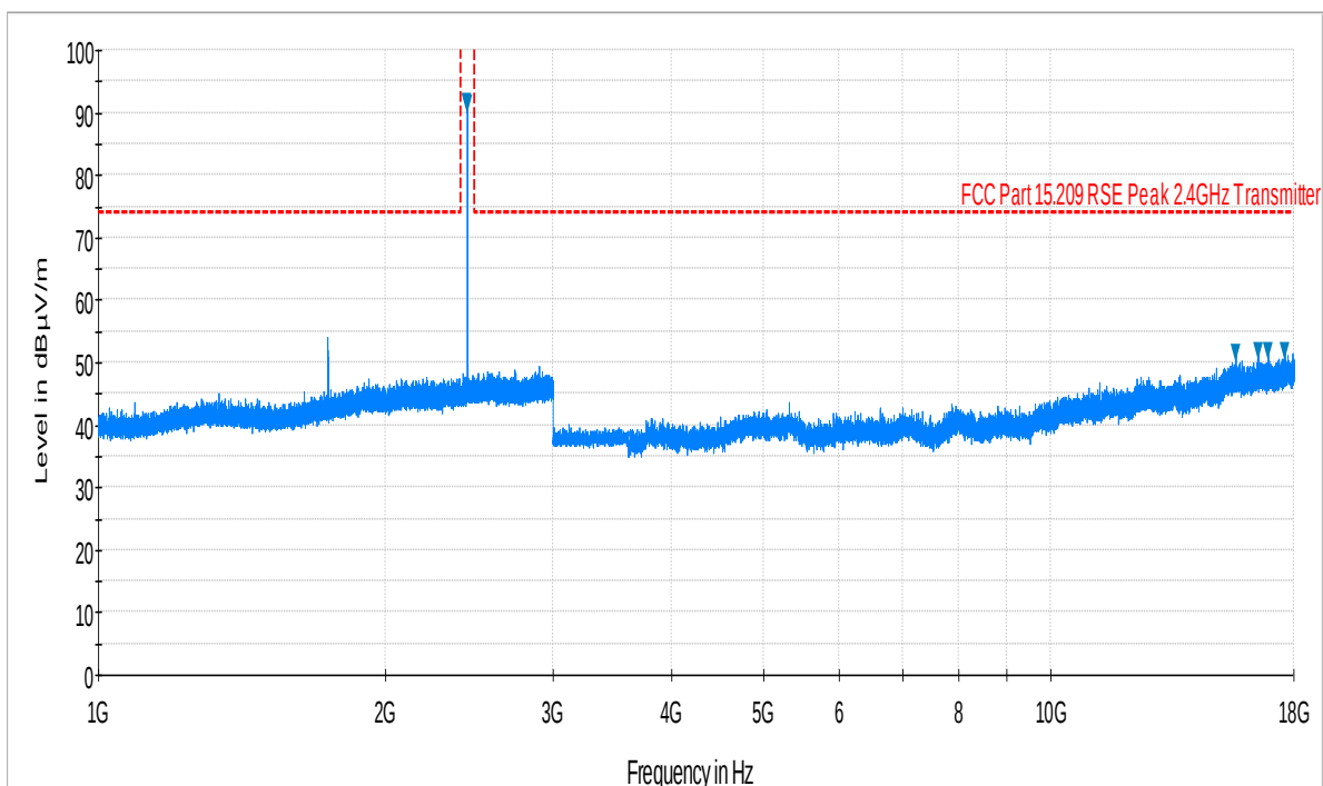
Plot 6-4. Radiated Spurious Plot above 1GHz (Bluetooth LE – Ch. 19, Ant. Pol. V)
