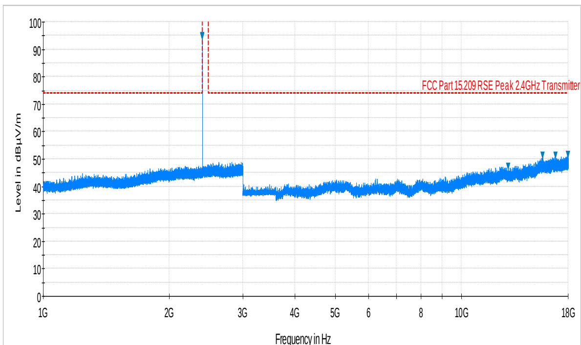
Plot 6-1. Radiated Spurious Plot above 1GHz (Bluetooth LE – Ch. 0, Ant. Pol. H)
