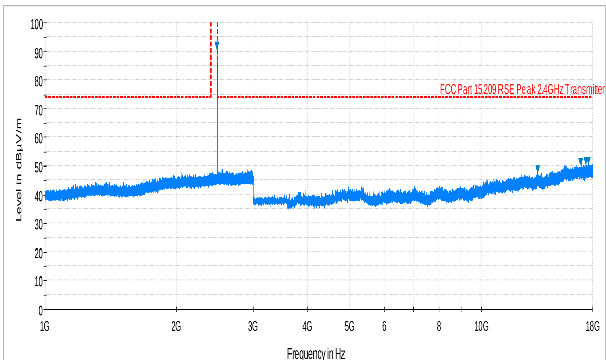
Plot 6-5. Radiated Spurious Plot above 1GHz (Bluetooth LE – Ch. 39, Ant. Pol. H)
