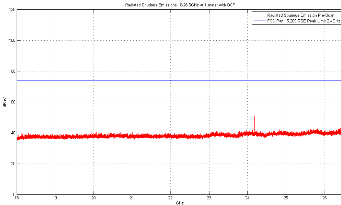
Plot 6-7. Radiated Spurious Plot above 1GHz (Bluetooth LE – Ch. 39, Ant. Pol. V)
