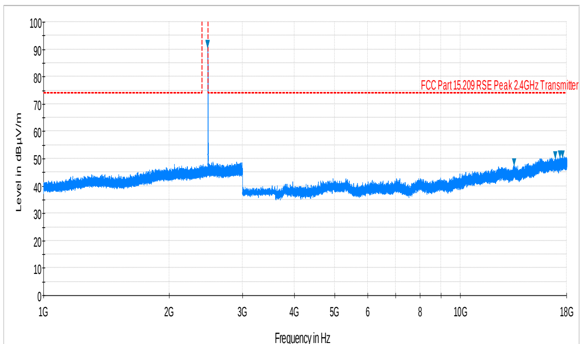
Plot 6-6. Radiated Spurious Plot above 1GHz (Bluetooth LE – Ch. 39, Ant. Pol. V)
