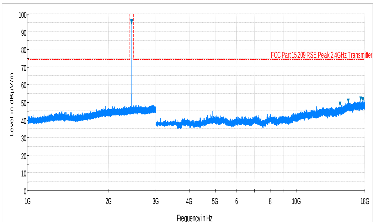
Plot 6-3. Radiated Spurious Plot above 1GHz (Bluetooth LE – Ch. 19, Ant. Pol. H)
