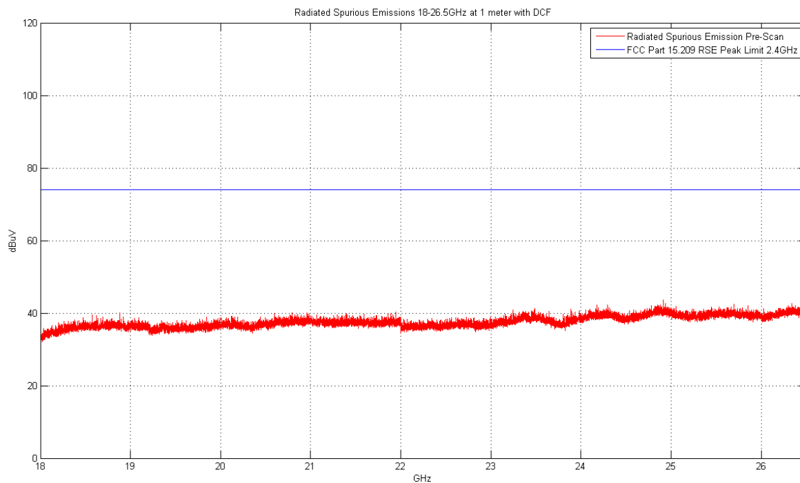
Plot 6-8. Radiated Spurious Plot above 1GHz (Bluetooth LE – Ch. 39, Ant. Pol. V)
