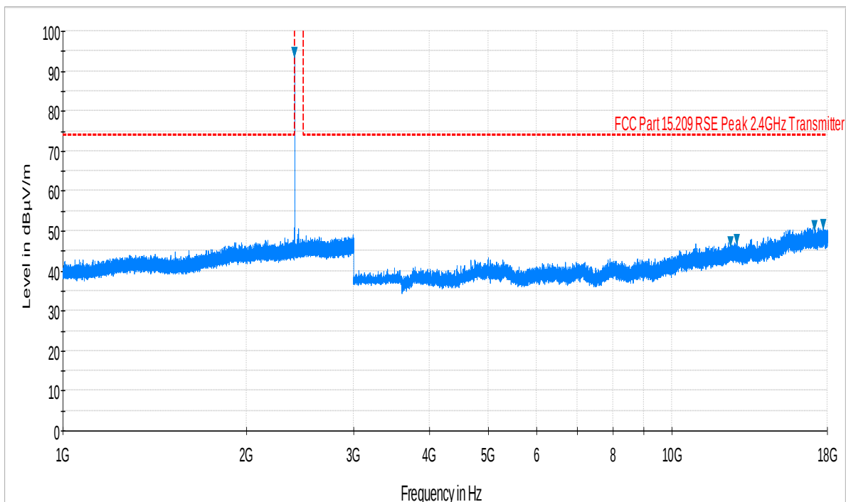
Plot 6-2. Radiated Spurious Plot above 1GHz (Bluetooth LE – Ch. 0, Ant. Pol. V)
