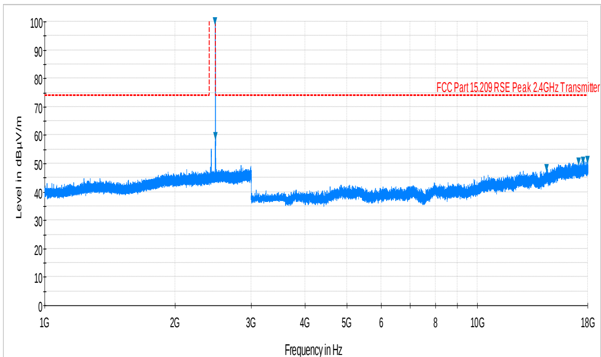
Plot 6-5. Radiated Spurious Plot above 1GHz (Bluetooth – Ch. 78, Ant. Pol. H)
