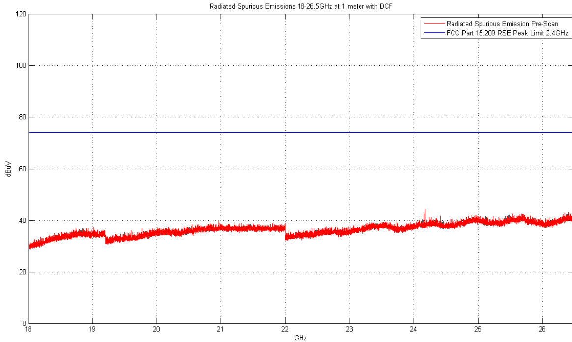
Plot 6-7. Radiated Spurious Plot above 18GHz (Bluetooth – Ch. 78, Ant. Pol. V)
