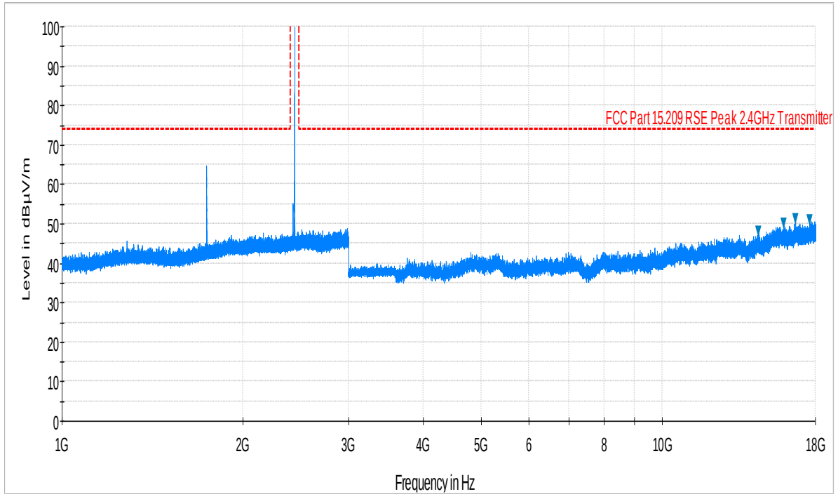
Plot 6-3. Radiated Spurious Plot above 1GHz (Bluetooth – Ch. 39, Ant. Pol. H)
