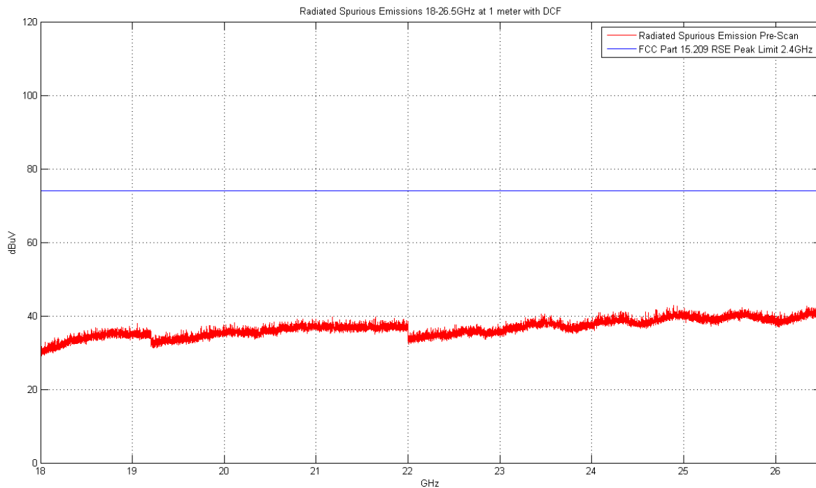
Plot 6-8. Radiated Spurious Plot above 18GHz (Bluetooth – Ch. 78, Ant. Pol. V)
