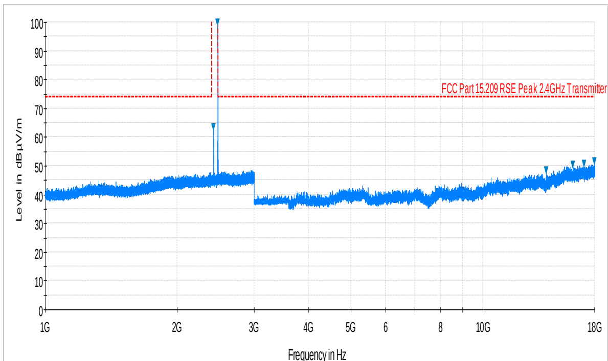
Plot 6-6. Radiated Spurious Plot above 1GHz (Bluetooth – Ch. 78, Ant. Pol. V)
