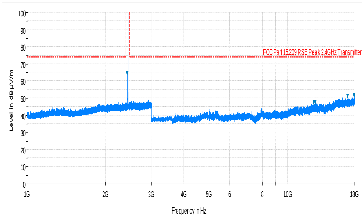
Plot 6-4. Radiated Spurious Plot above 1GHz (Bluetooth – Ch. 39, Ant. Pol. V)
