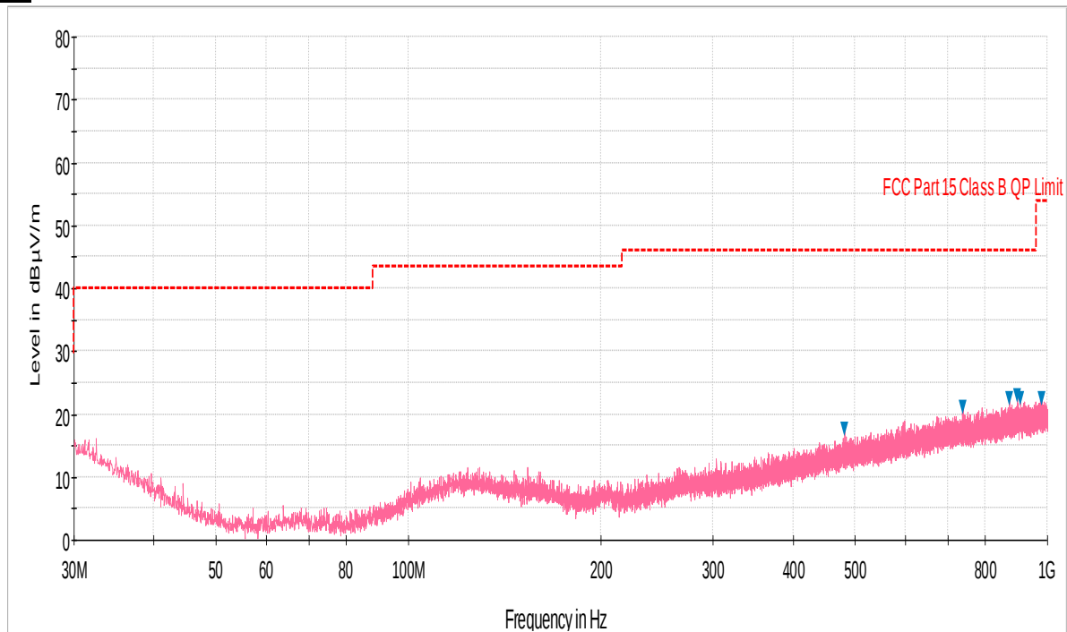
Plot 6-9. Radiated Spurious Plot below 1GHz (Pol. H)
