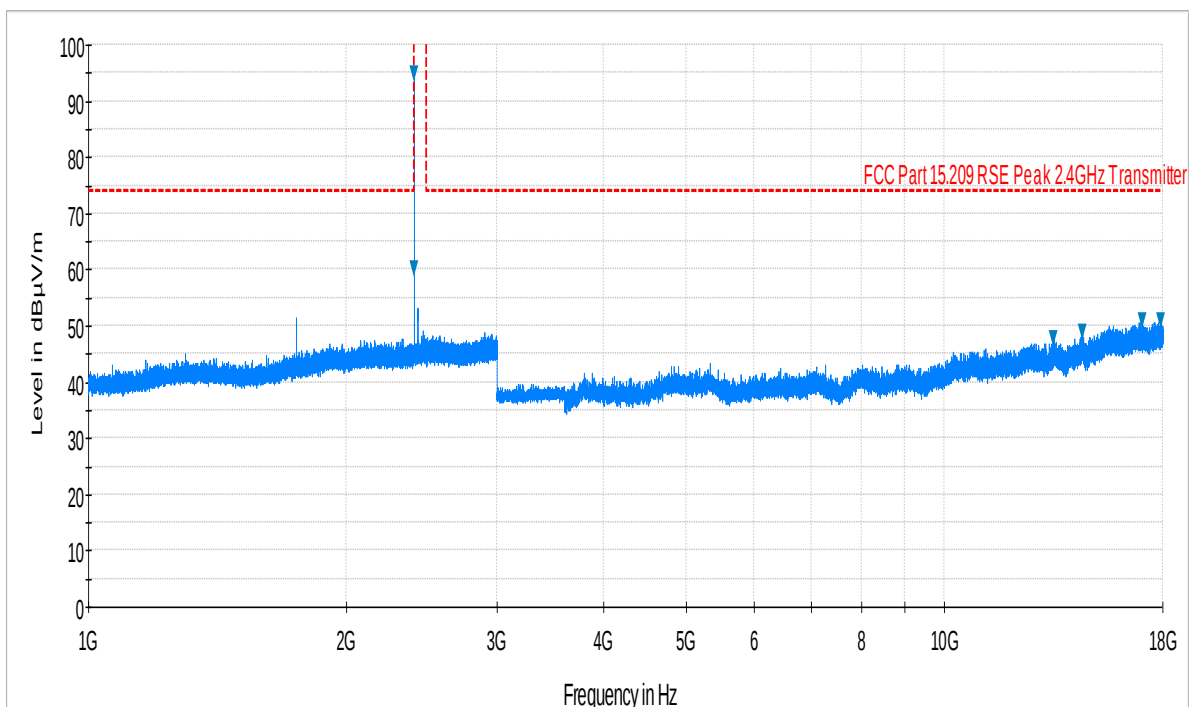
Plot 6-1. Radiated Spurious Plot above 1GHz (Bluetooth – Ch. 0, Ant. Pol. H)
