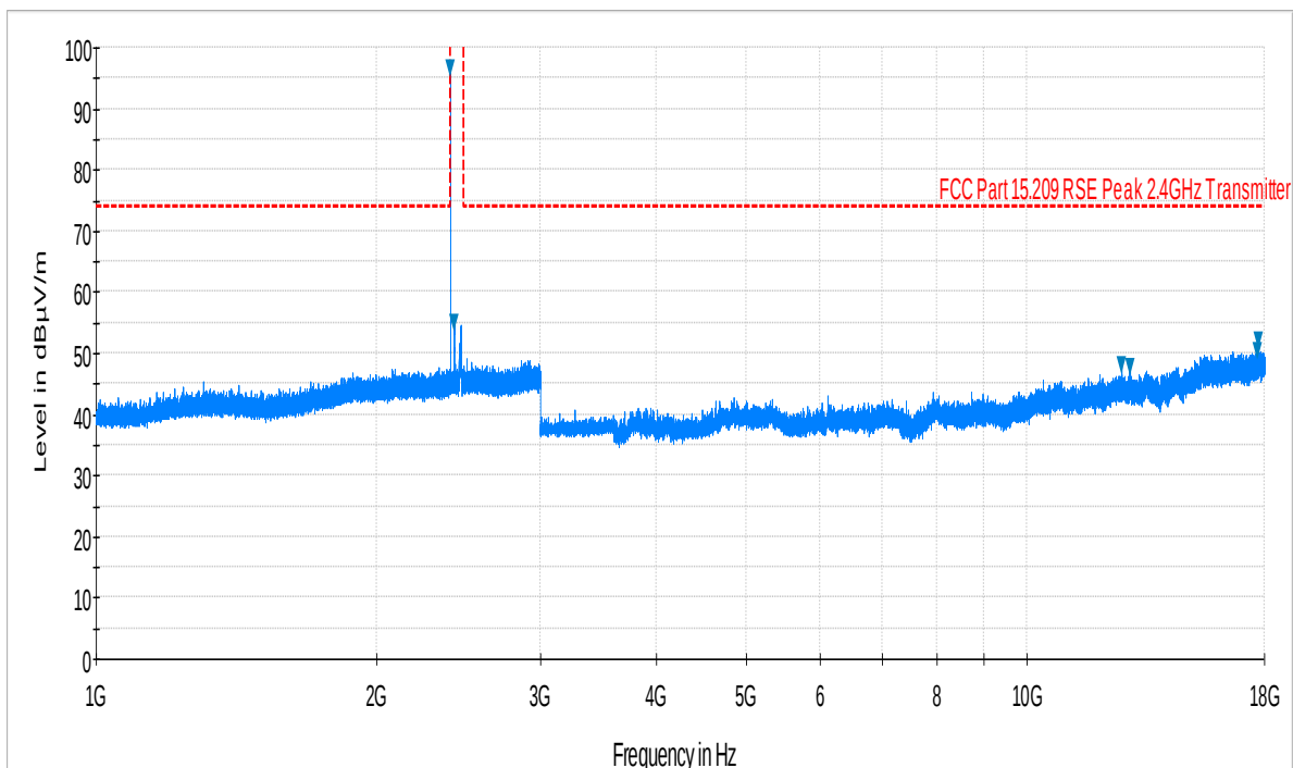
Plot 6-2. Radiated Spurious Plot above 1GHz (Bluetooth – Ch. 0, Ant. Pol. V)
