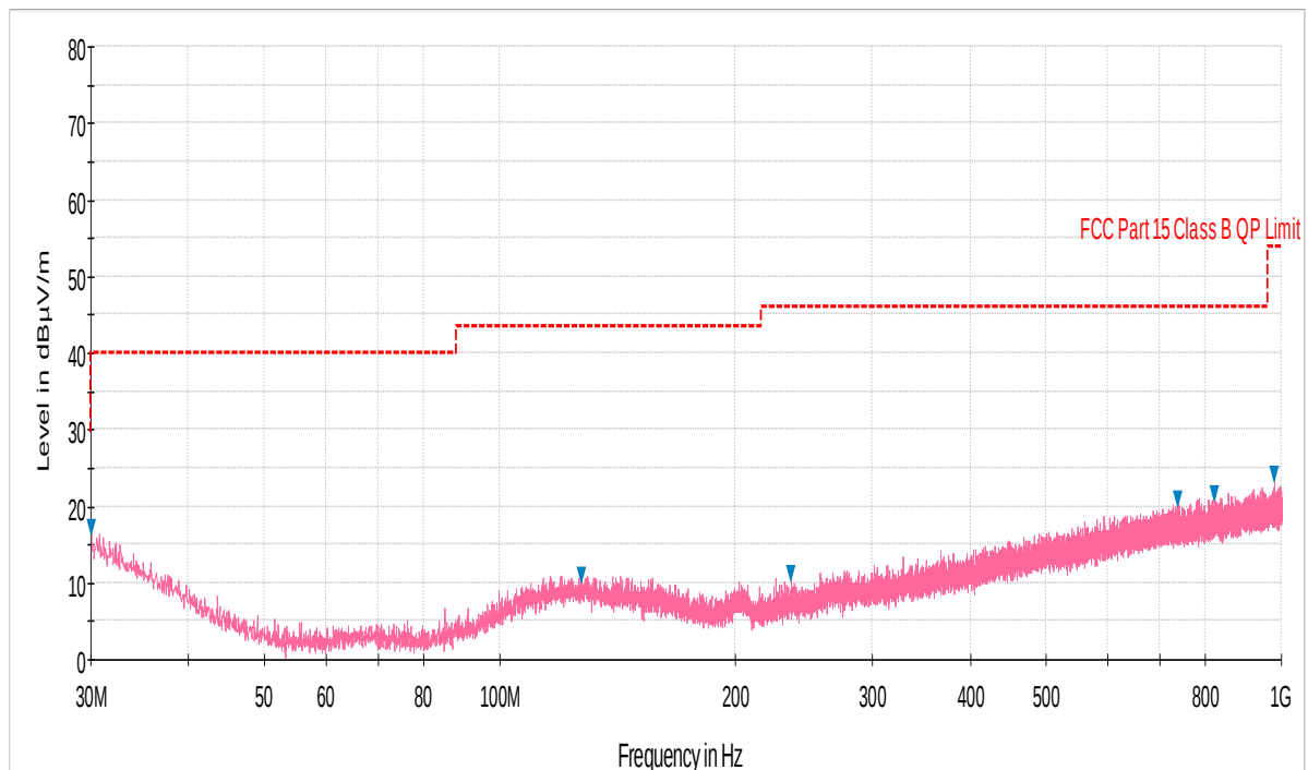
Plot 6-10. Radiated Spurious Plot below 1GHz (Pol. V)
