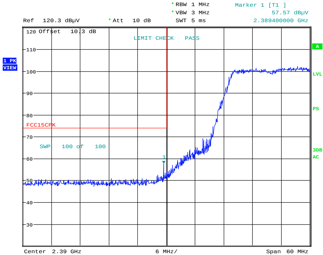
Plot 6-10. Radiated Restricted Lower Band Edge Measurement (Peak)
