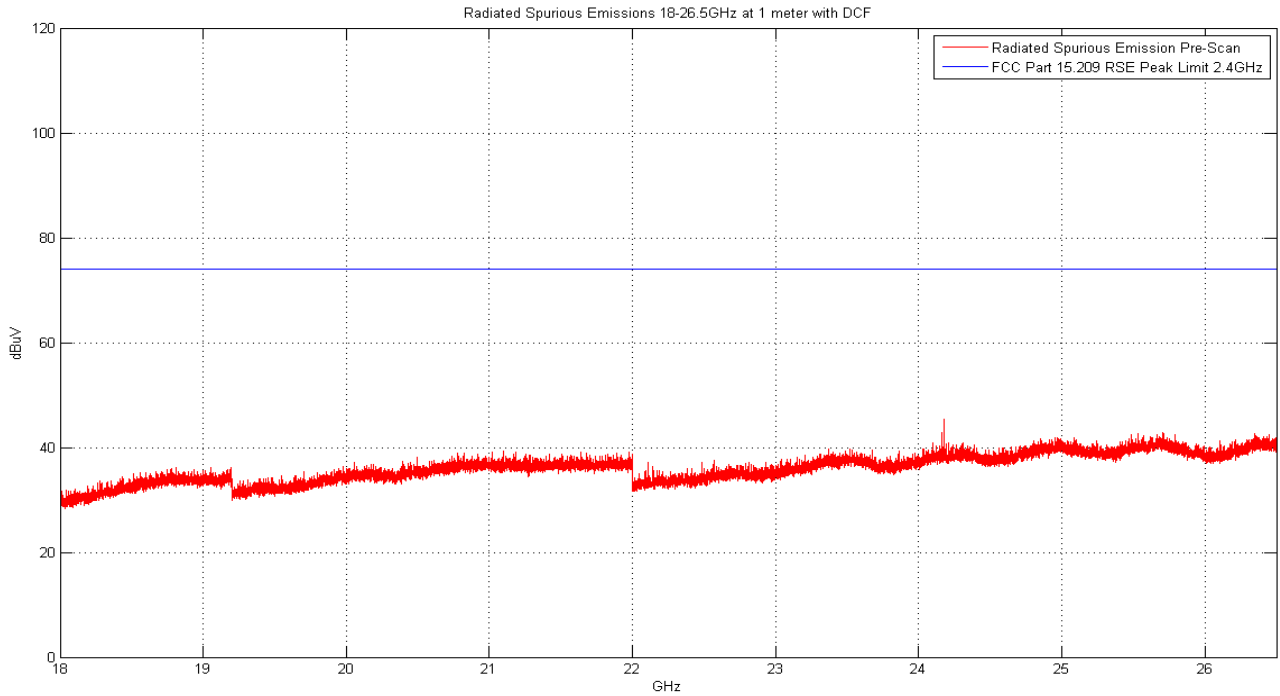
Plot 6-7. Radiated Spurious Plot above 18GHz (802.11b – Ch. 11, Ant. Pol. V)
