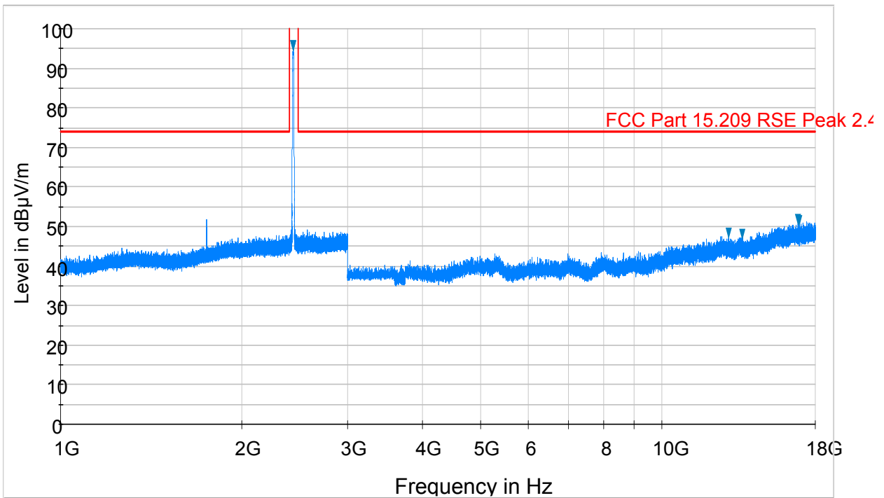
Plot 6-4. Radiated Spurious Plot above 1GHz (802.11b – Ch. 6, Ant. Pol. V)
