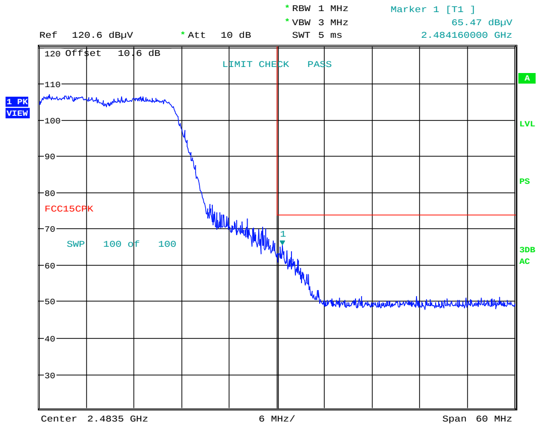
Plot 6-12. Radiated Restricted Upper Band Edge Measurement (Peak)
