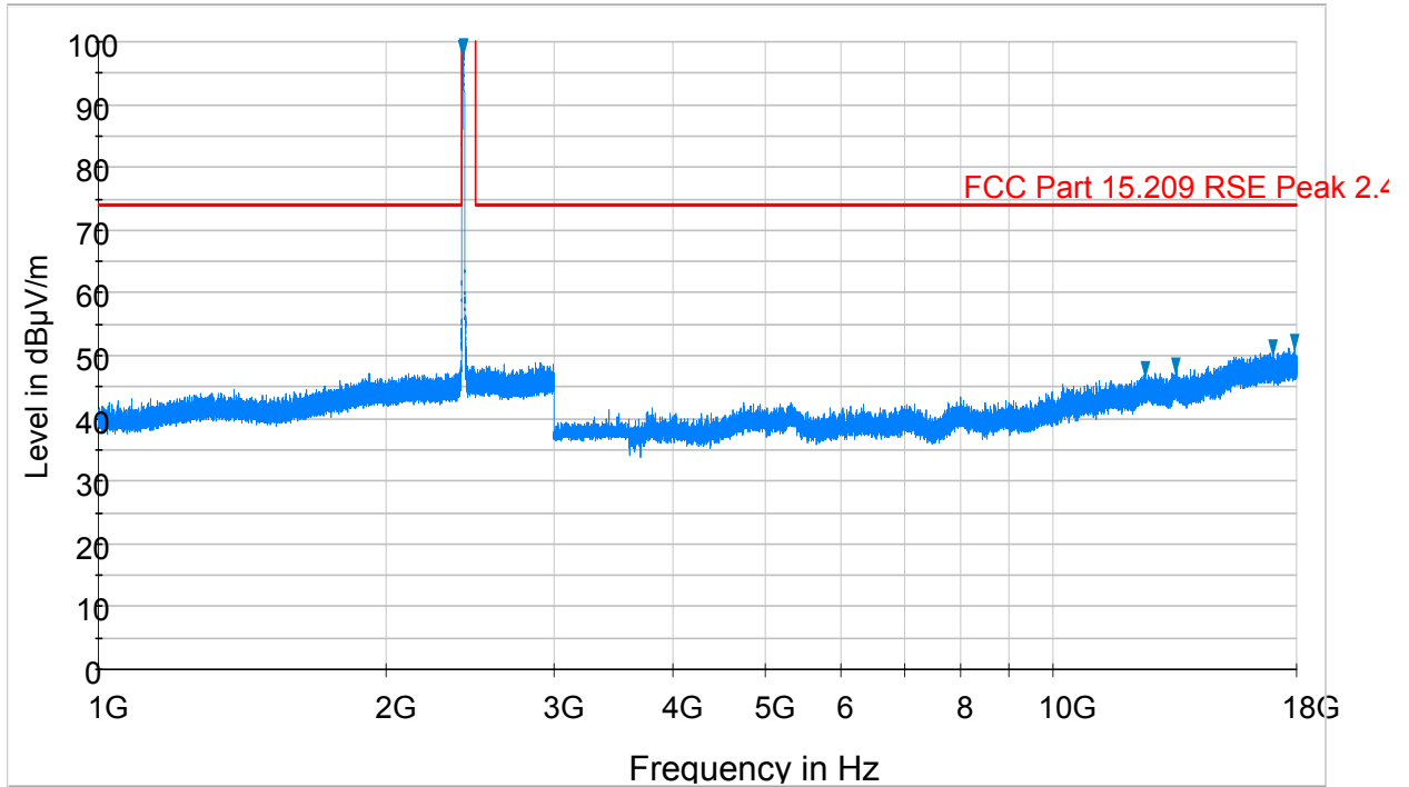
Plot 6-1. Radiated Spurious Plot above 1GHz (802.11b – Ch. 1, Ant. Pol. H)
