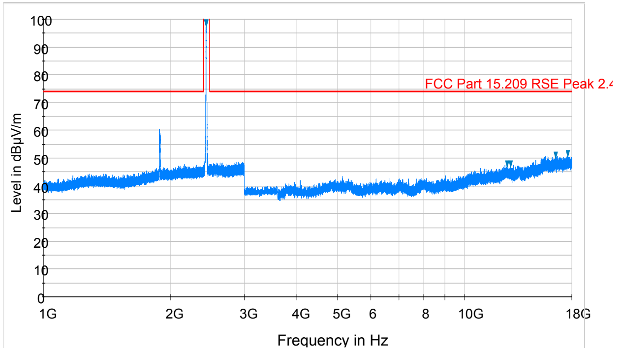
Plot 6-3. Radiated Spurious Plot above 1GHz (802.11b – Ch. 6, Ant. Pol. H)
