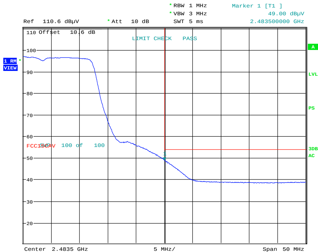
Plot 6-11. Radiated Restricted Upper Band Edge Measurement (Average)
