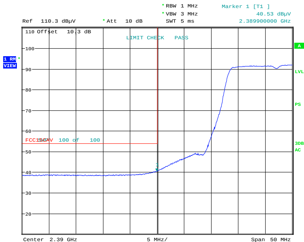
Plot 6-9. Radiated Restricted Lower Band Edge Measurement (Average)
