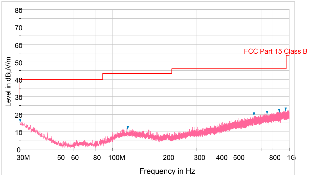
Plot 6-13. Radiated Spurious Plot below 1GHz (Pol. H)
