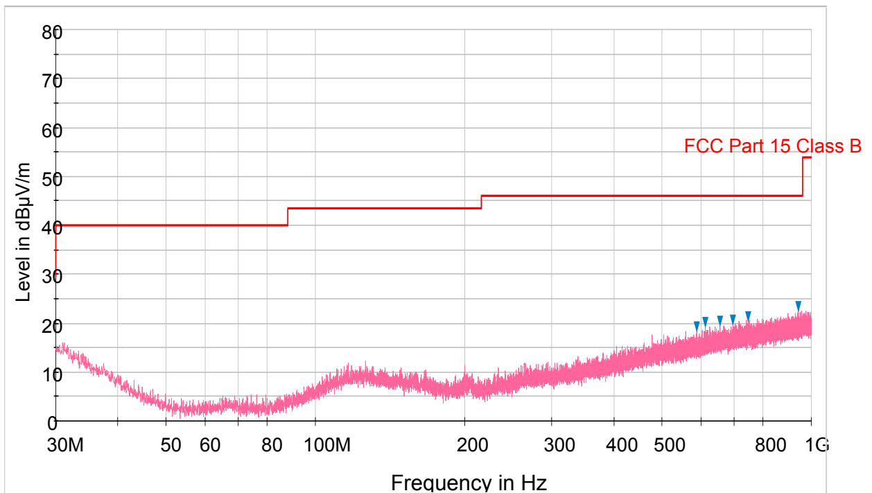
Plot 6-14. Radiated Spurious Plot below 1GHz (Pol. V)
