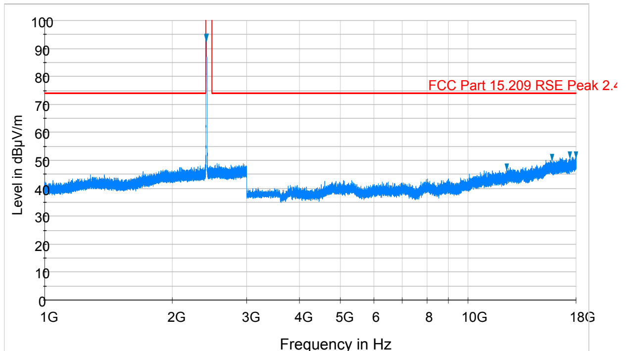
Plot 6-2. Radiated Spurious Plot above 1GHz (802.11b – Ch. 1, Ant. Pol. V)
