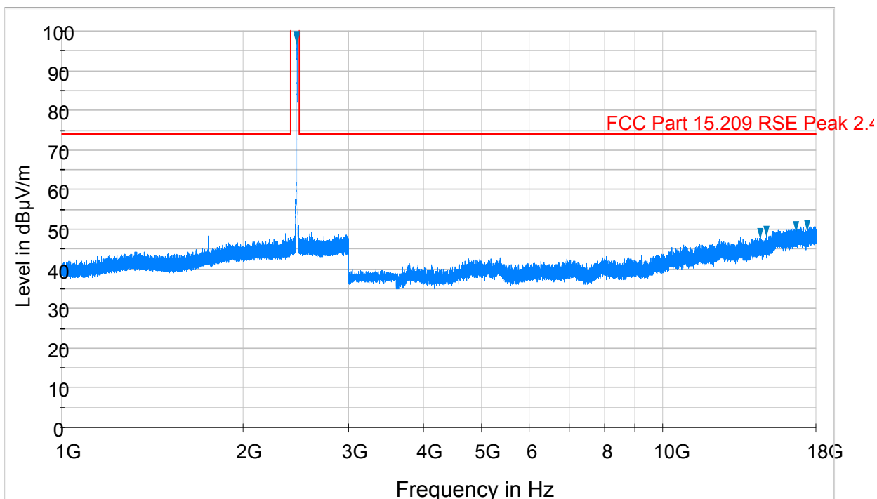
Plot 6-5. Radiated Spurious Plot above 1GHz (802.11b – Ch. 11, Ant. Pol. H)
