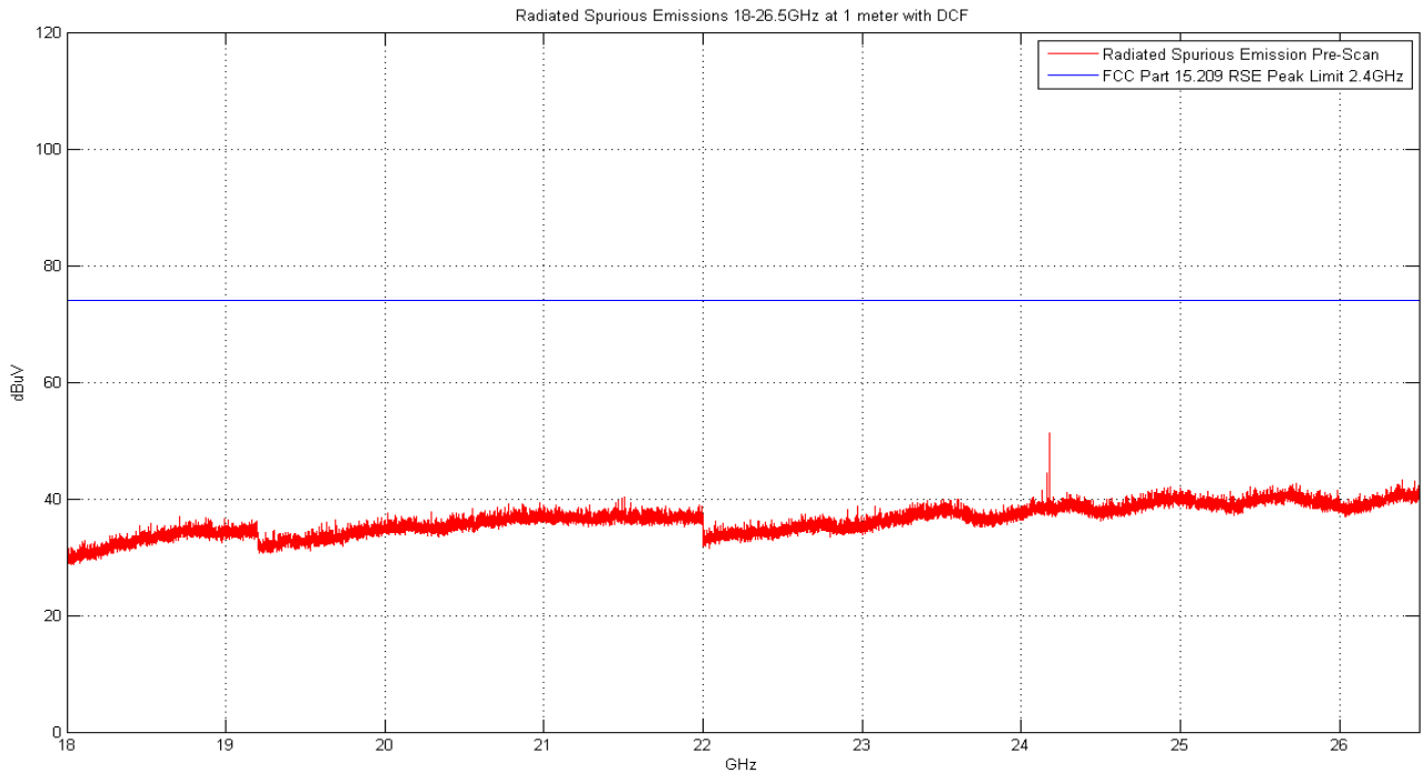
Plot 6-8. Radiated Spurious Plot above 18GHz (802.11b – Ch. 11, Ant. Pol. V)
