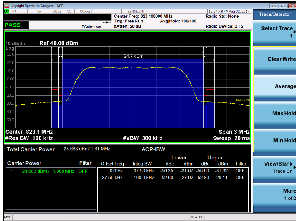
Plot 7-22. CDMA800 (BC10) Channel Edge Plot (Ch. 684)
