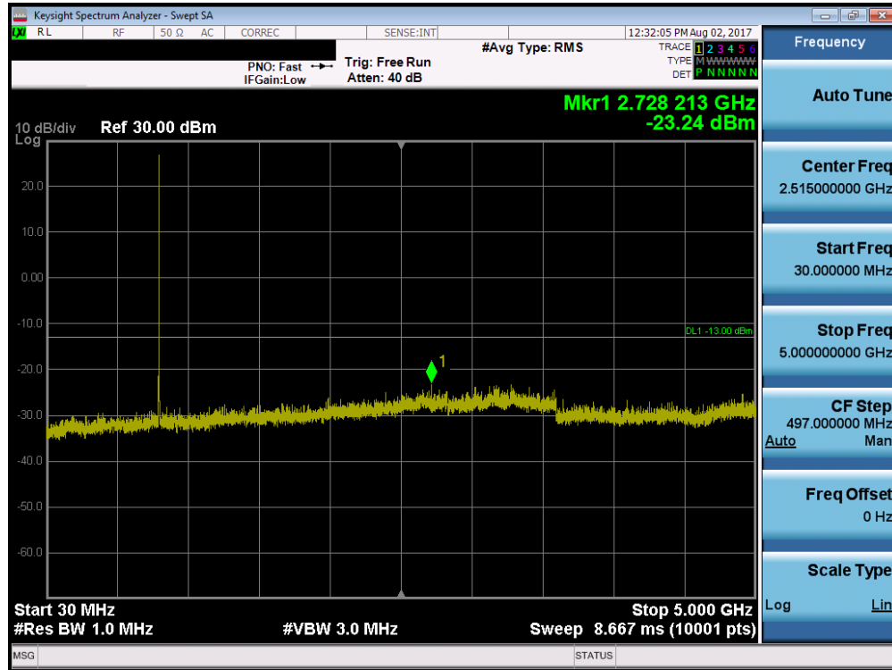
Plot 7-13. CDMA800 (BC10) Conducted Spurious Plot (Ch. 476)
