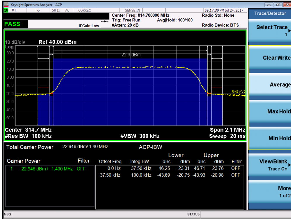
Plot 7-23. LTE Band 26 Channel Edge Plot (1.4MHz QPSK – RB Size 6– Low Channel)
