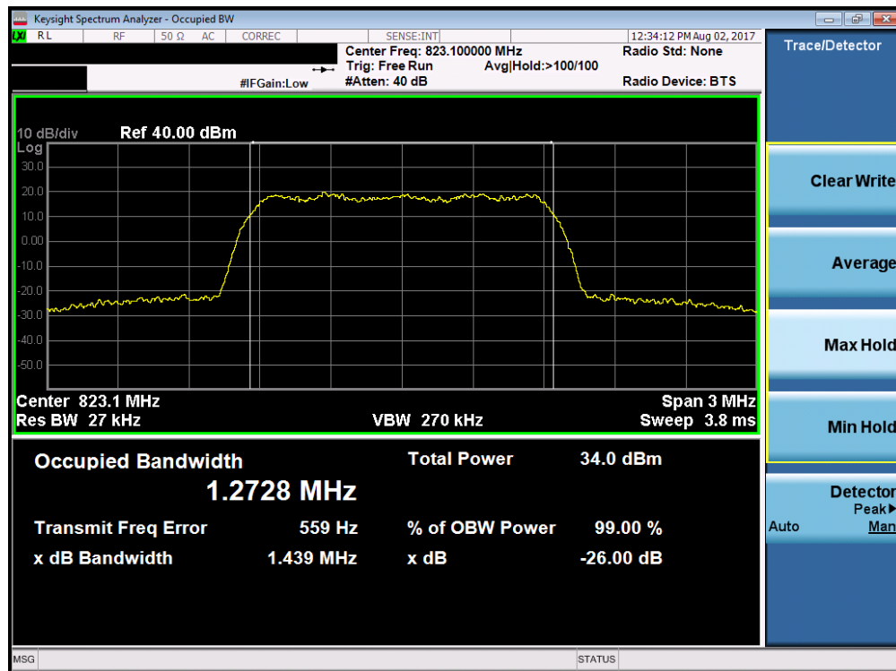
Plot 7-2. CDMA800 (BC10) Occupied Bandwidth Plot (Ch. 684)
