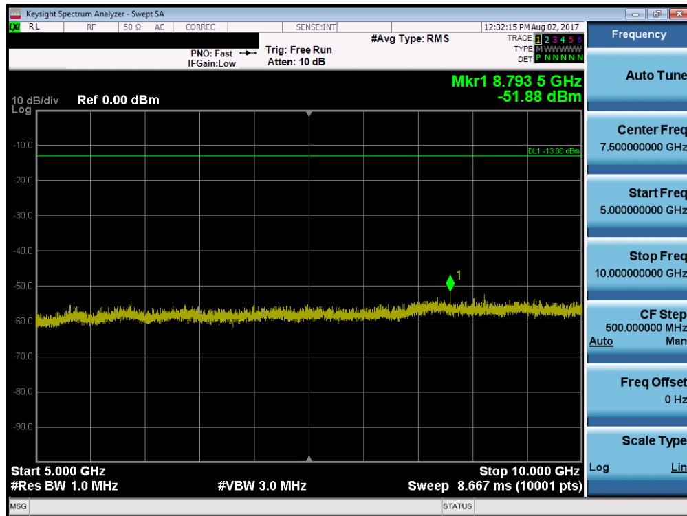
Plot 7-14. CDMA800 (BC10) Conducted Spurious Plot (Ch. 476)
