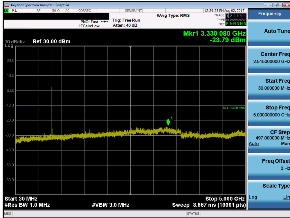
Plot 7-15. CDMA800 (BC10) Conducted Spurious Plot (Ch. 684)
