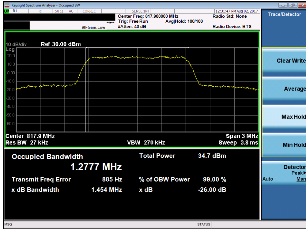
Plot 7-1. CDMA800 (BC10) Occupied Bandwidth Plot (Ch. 476)
