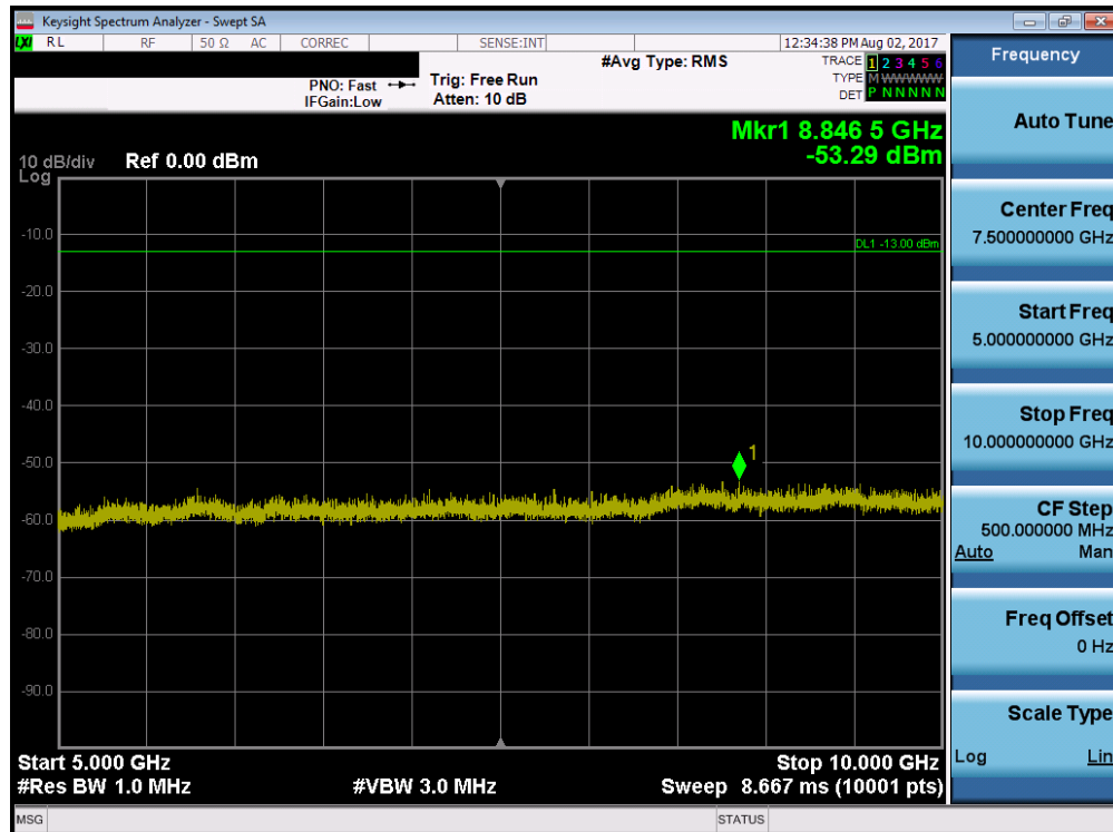
Plot 7-16. CDMA800 (BC10) Conducted Spurious Plot (Ch. 684)
