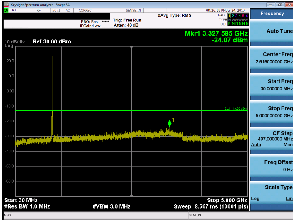
Plot 7-19. LTE Band 26 Conducted Spurious Plot (5MHz QPSK – RB Size 1, RB Offset 0 – High Channel)
