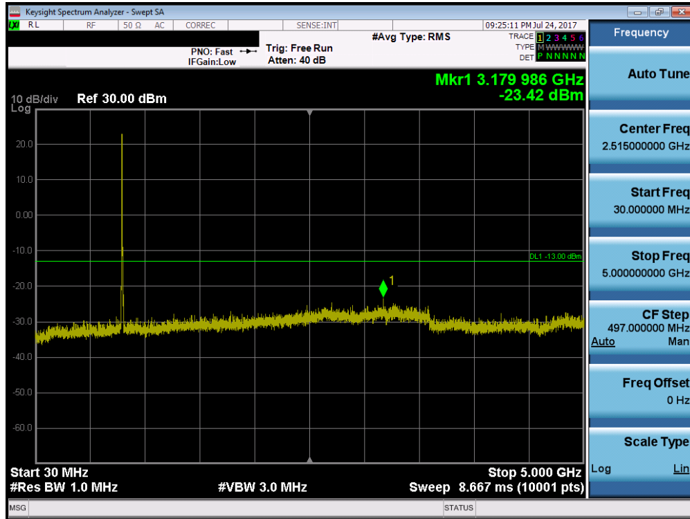
Plot 7-17. LTE Band 26 Conducted Spurious Plot (5MHz QPSK – RB Size 1, RB Offset 0 – Low Channel)
