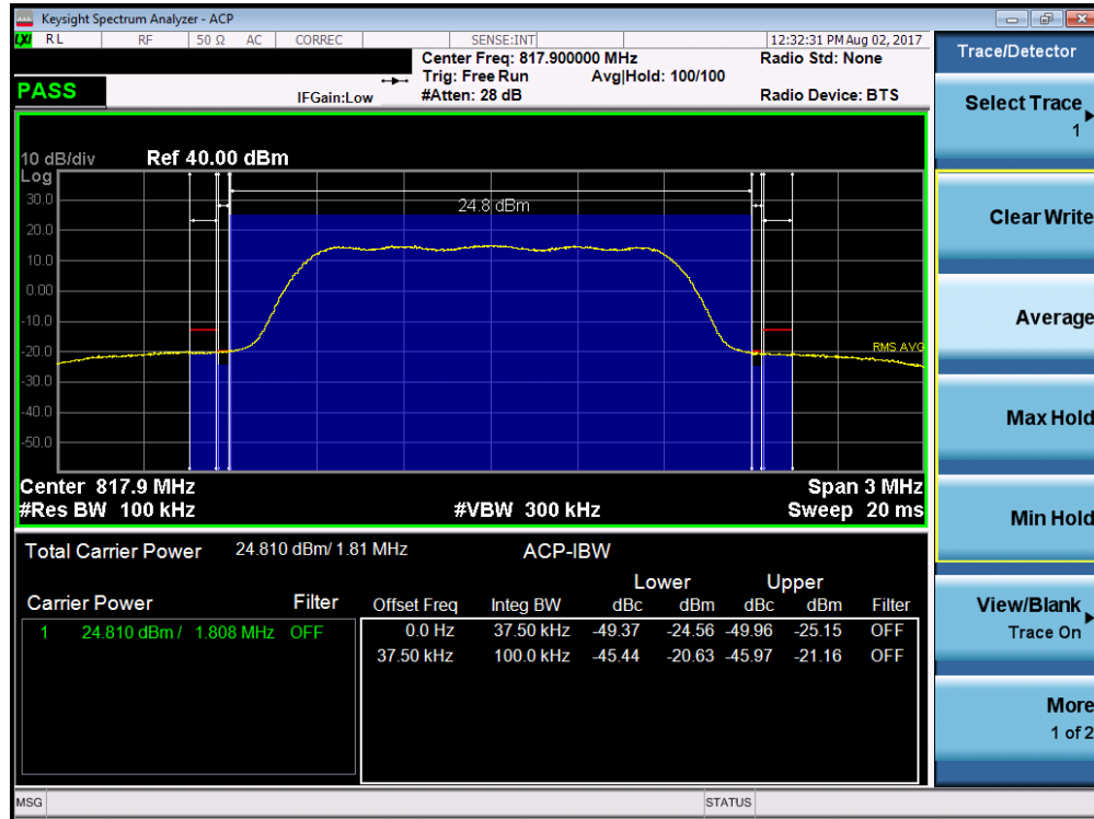
Plot 7-21. CDMA800 (BC10) Channel Edge Plot (Ch. 476)
