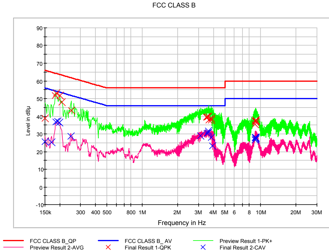
Figure 4: Conducted Emission, AC Main Port, Data Communication Mode(with sound pack), Line (N)
