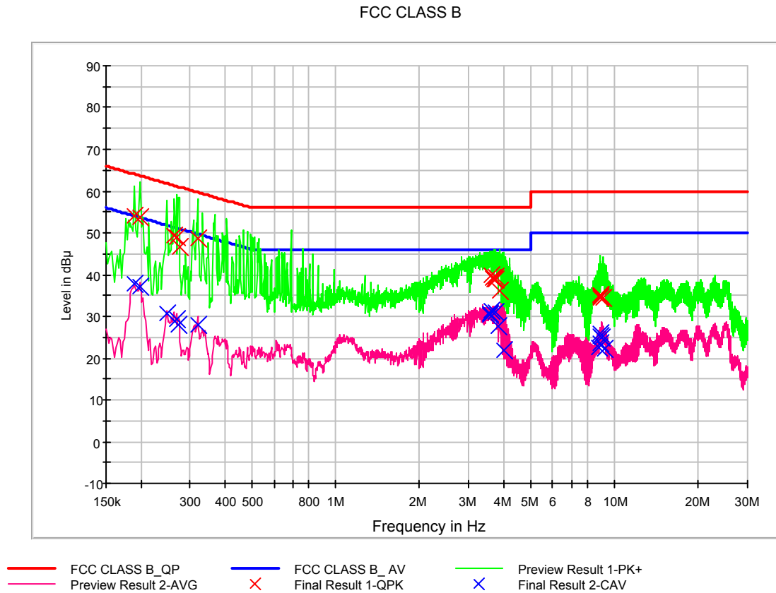
Figure 3: Conducted Emission, AC Main Port, Data Communication Mode(with sound pack), Line (L1)
