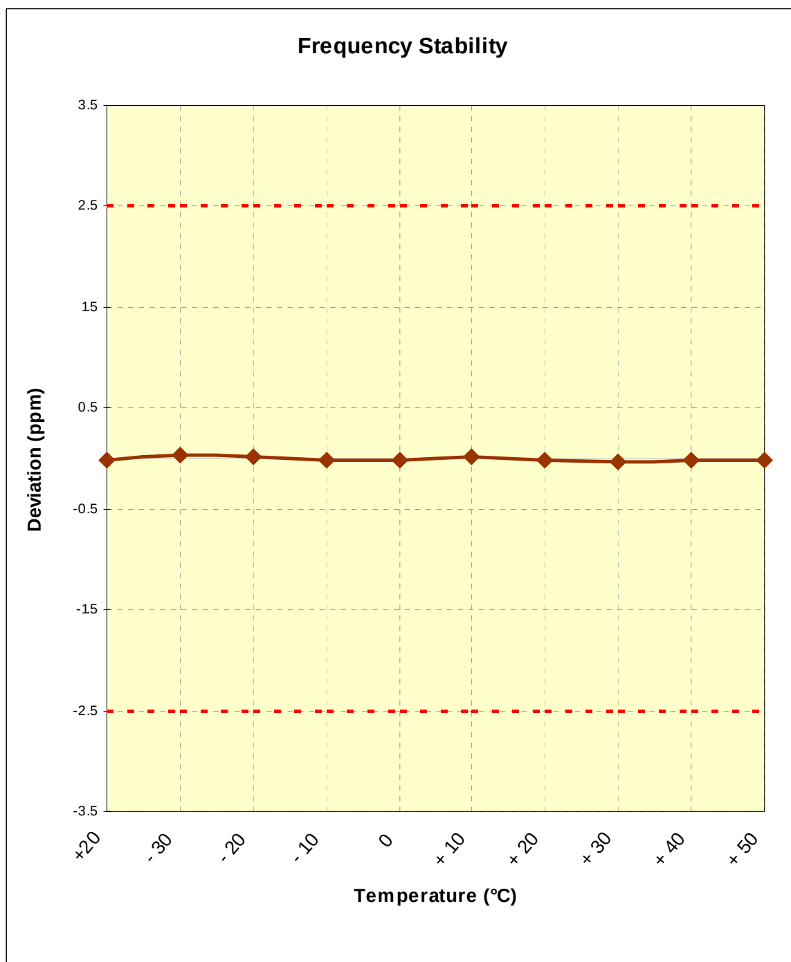
Figure 6-1. Frequency Stability Graph (Cellular CDMA Mode – Ch. 684)
