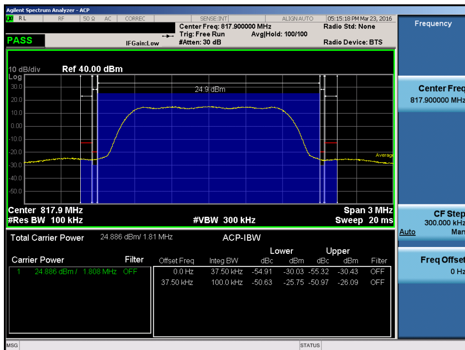
Plot 7-23. Channel Edge Plot (Ch. 476)
