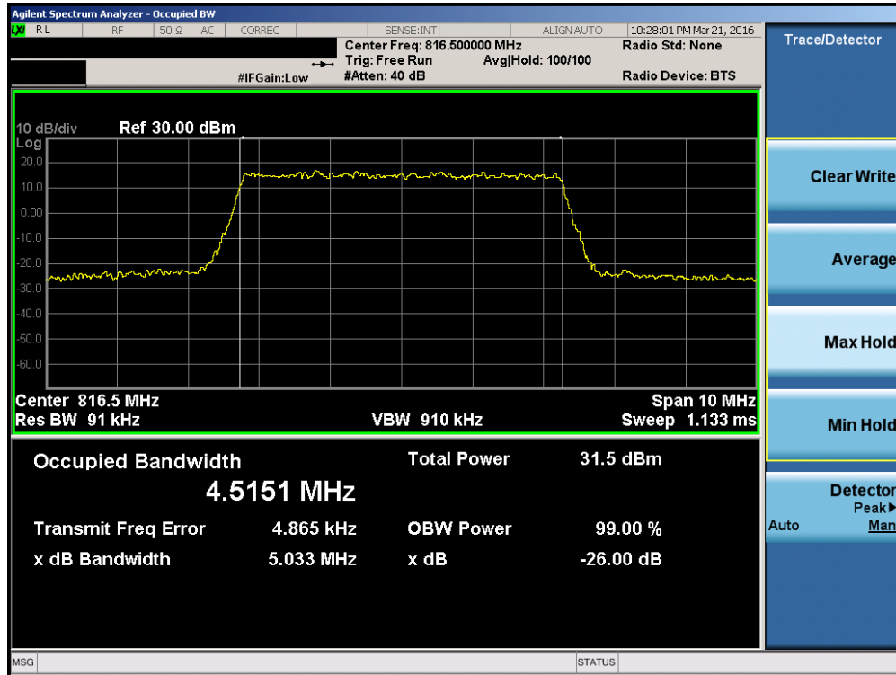
Plot 7-11. Occupied Bandwidth Plot (5MHz QPSK – RB Size 25– Low Channel)
