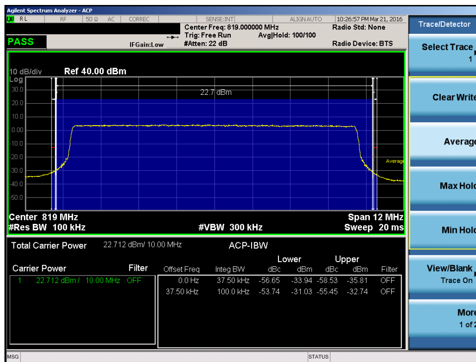
Plot 7-31. Channel Edge Plot (10MHz QPSK – RB Size 50)
