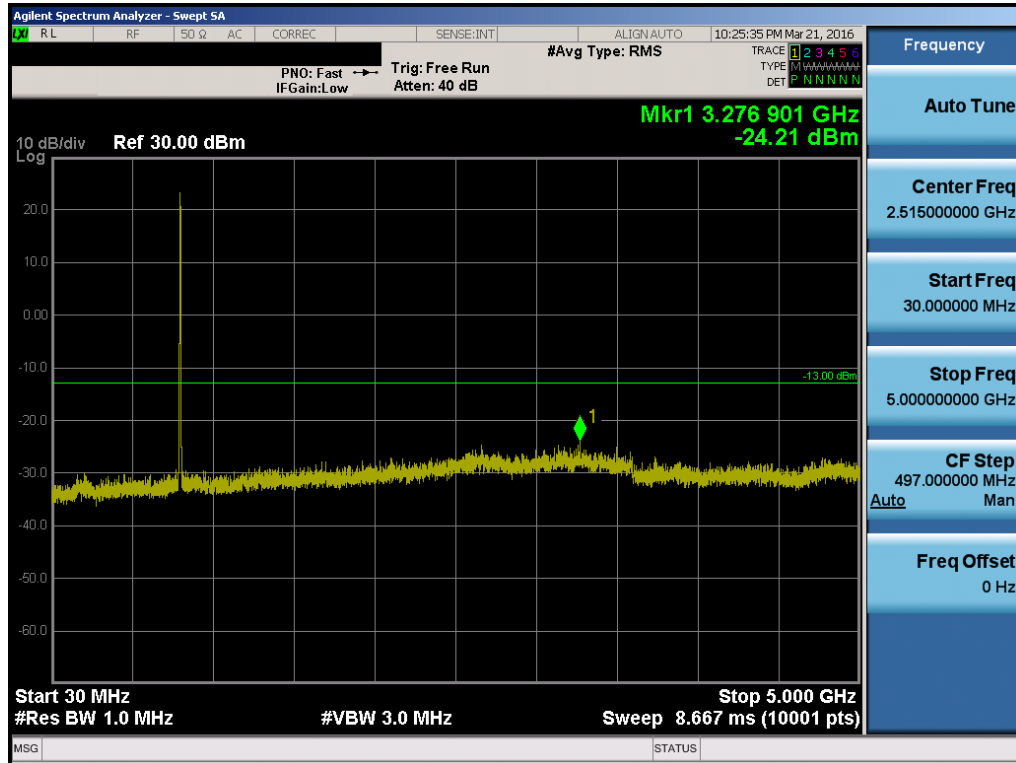
Plot 7-21. Conducted Spurious Plot ( 10MHz QPSK – RB Size 1, RB Offset 0 – Mid Channel)
