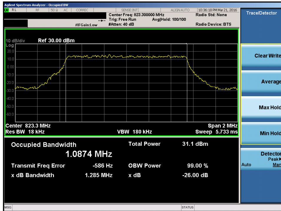
Plot 7-6. Occupied Bandwidth Plot (1.4MHz 16-QAM – RB Size 6– High Channel)
