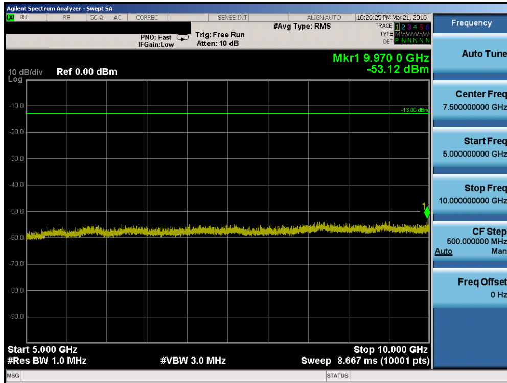
Plot 7-22. Conducted Spurious Plot ( 10MHz QPSK – RB Size 1, RB Offset 0 – Mid Channel)
