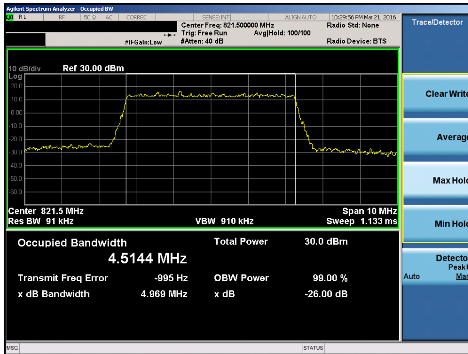
Plot 7-14. Occupied Bandwidth Plot (5MHz 16-QAM – RB Size 25– High Channel)
