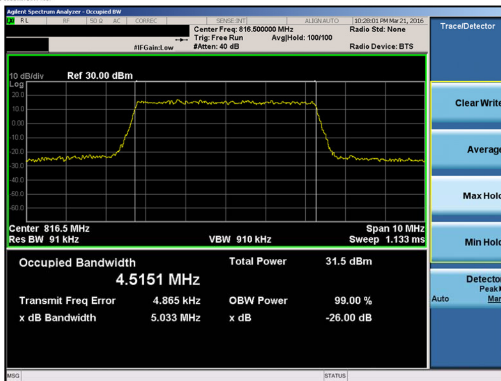
Plot 7-11. Occupied Bandwidth Plot (5MHz QPSK – RB Size 25– Low Channel)
