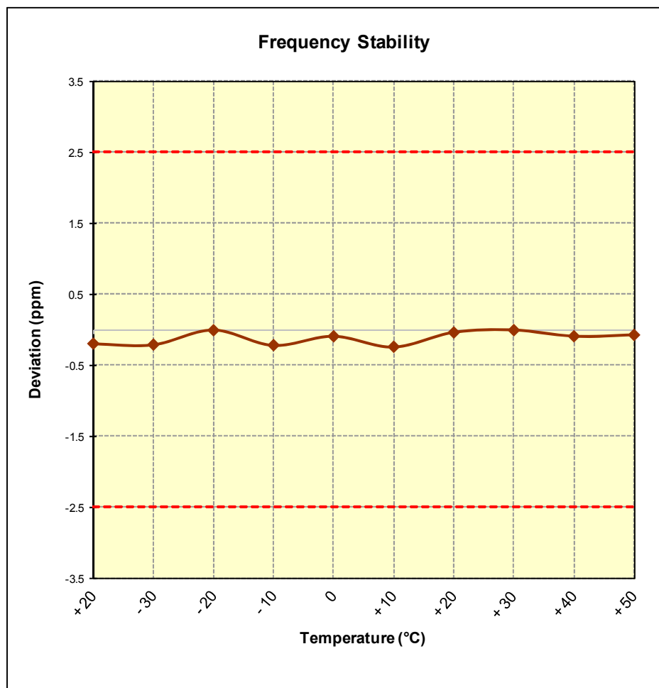
Figure 7-5. CDMA BC10 Frequency Stability Graph (Ch. 476)
