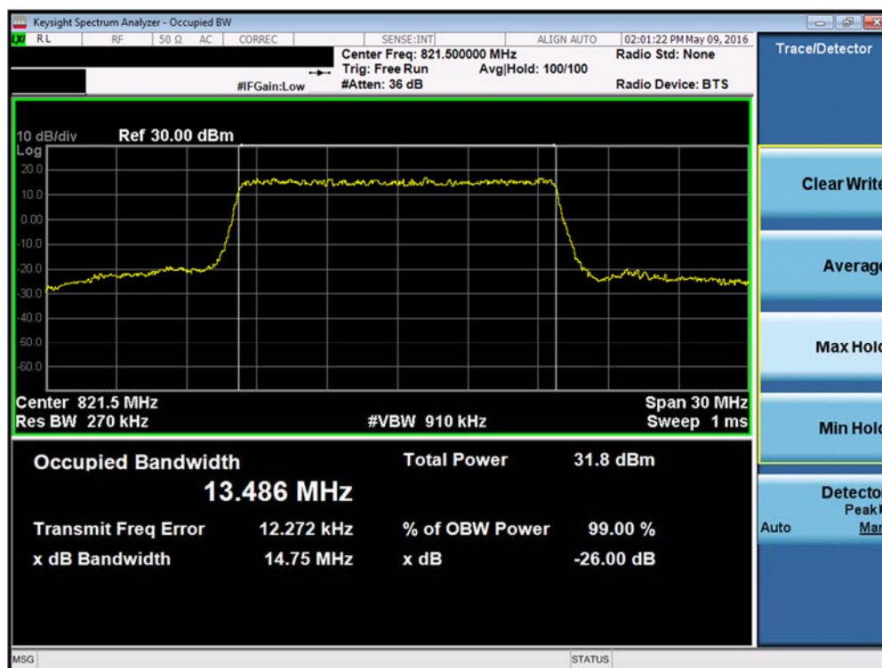
Plot 7-17. Occupied Bandwidth Plot (15MHz QPSK – RB Size 75)
