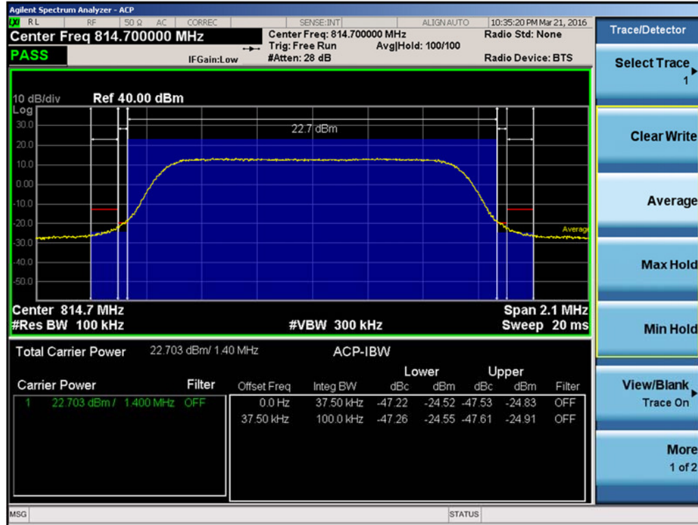
Plot 7-27. Channel Edge Plot (1.4MHz QPSK – RB Size 6– Low Channel)
