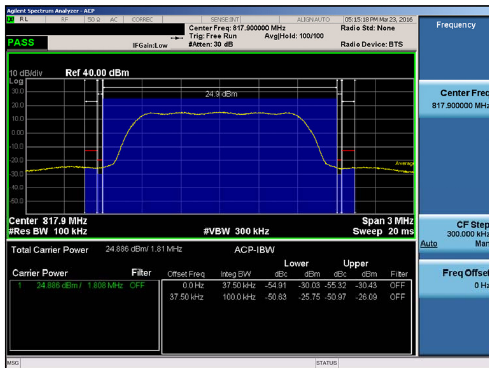
Plot 7-25. Channel Edge Plot (Ch. 476)
