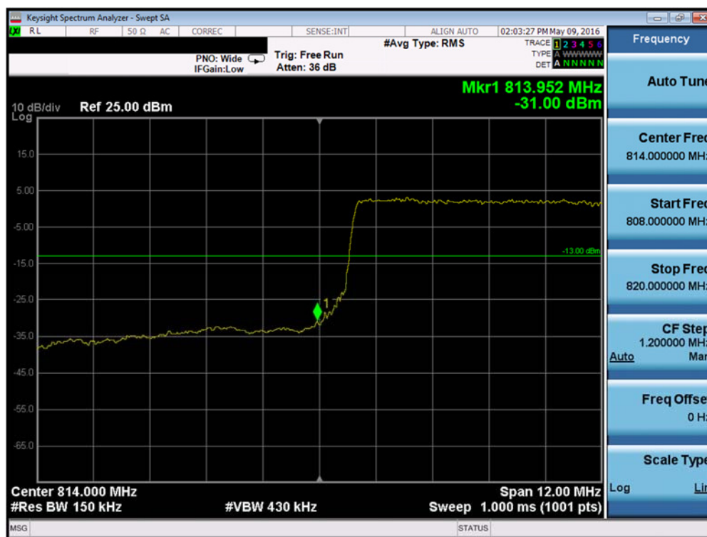
Plot 7-34. Lower Band Edge Plot (15MHz QPSK – RB Size 75)
