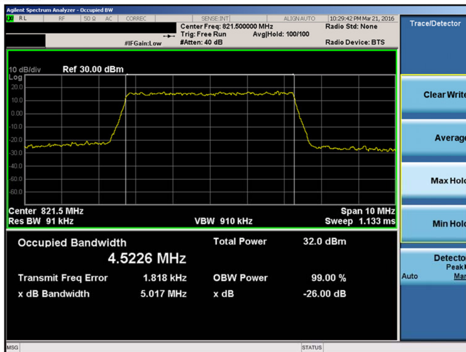
Plot 7-13. Occupied Bandwidth Plot (5MHz QPSK – RB Size 25– High Channel)
