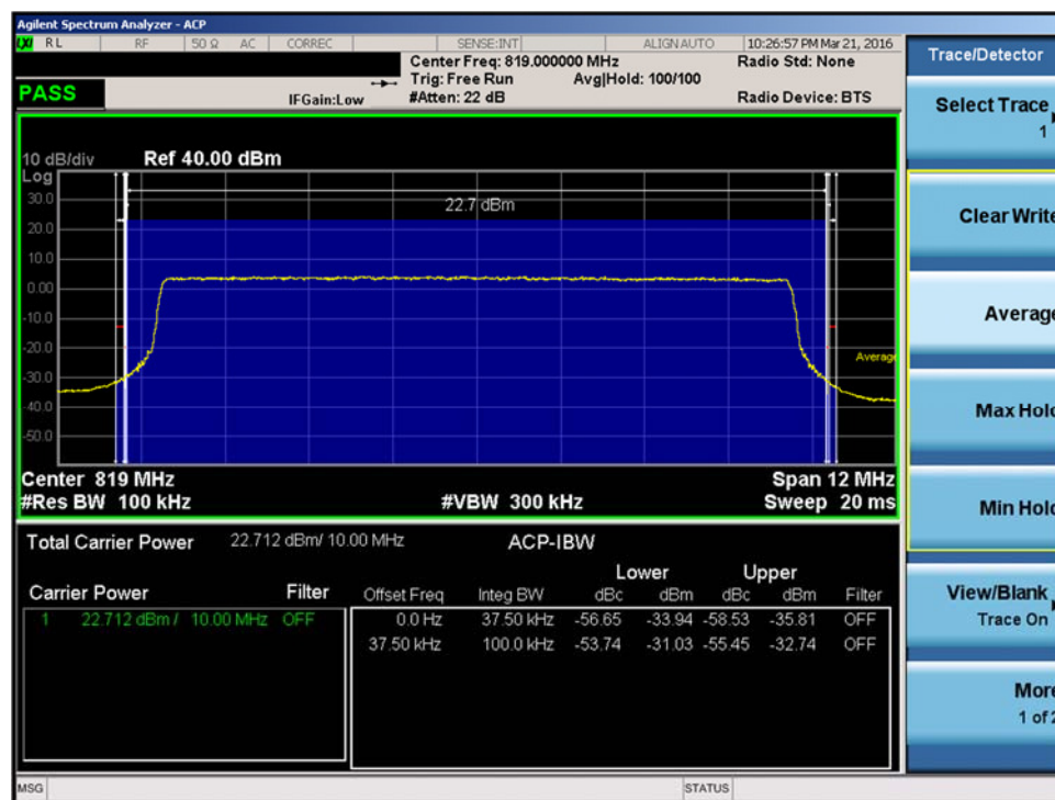
Plot 7-33. Channel Edge Plot (10MHz QPSK – RB Size 50)
