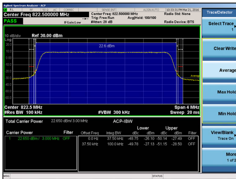
Plot 7-30. Channel Edge Plot (3MHz QPSK – RB Size 15 – High Channel)
