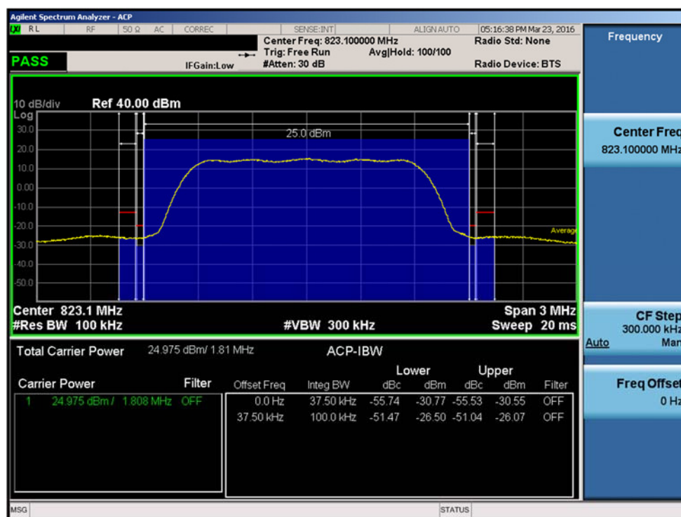
Plot 7-26. Channel Edge Plot (Ch. 684)
