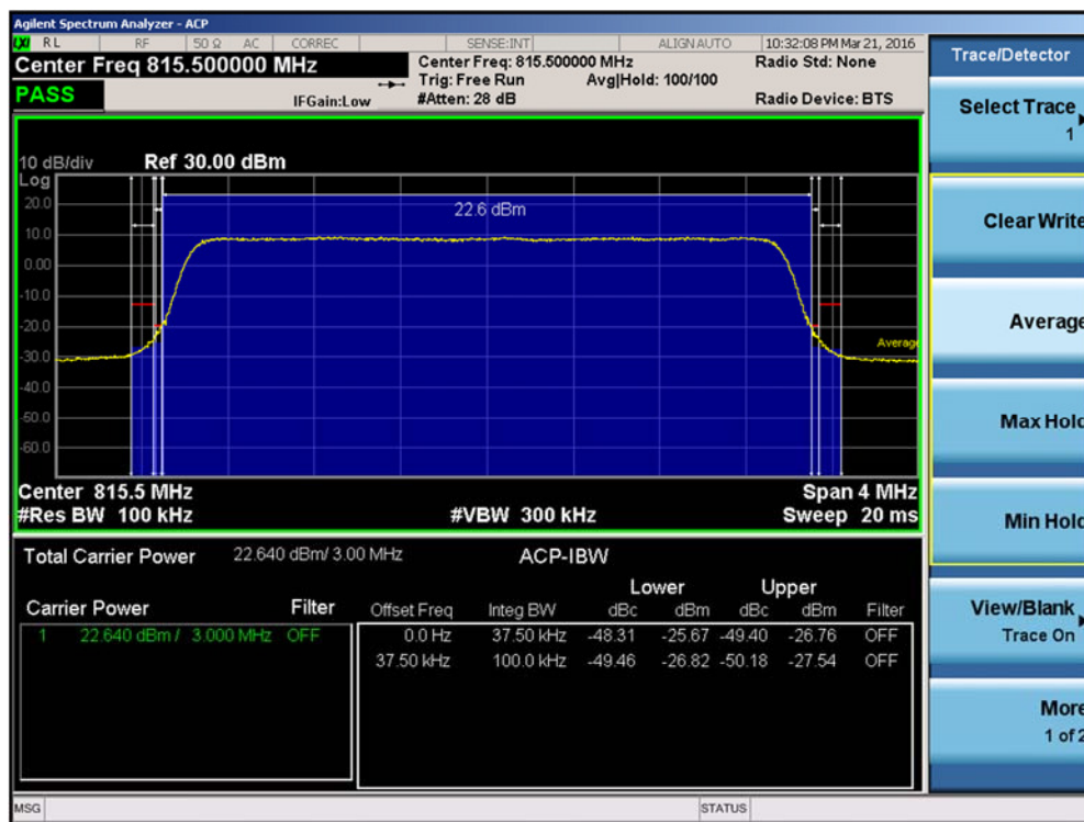
Plot 7-29. Channel Edge Plot (3MHz QPSK – RB Size 15– Low Channel)
