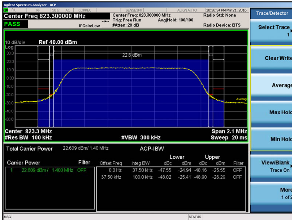
Plot 7-28. Channel Edge Plot (1.4MHz QPSK – RB Size 6 – High Channel)
