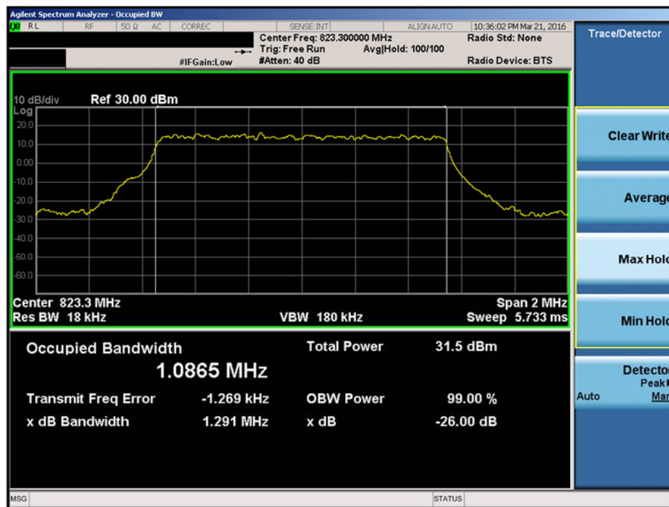
Plot 7-5. Occupied Bandwidth Plot (1.4MHz QPSK – RB Size 6– High Channel)
