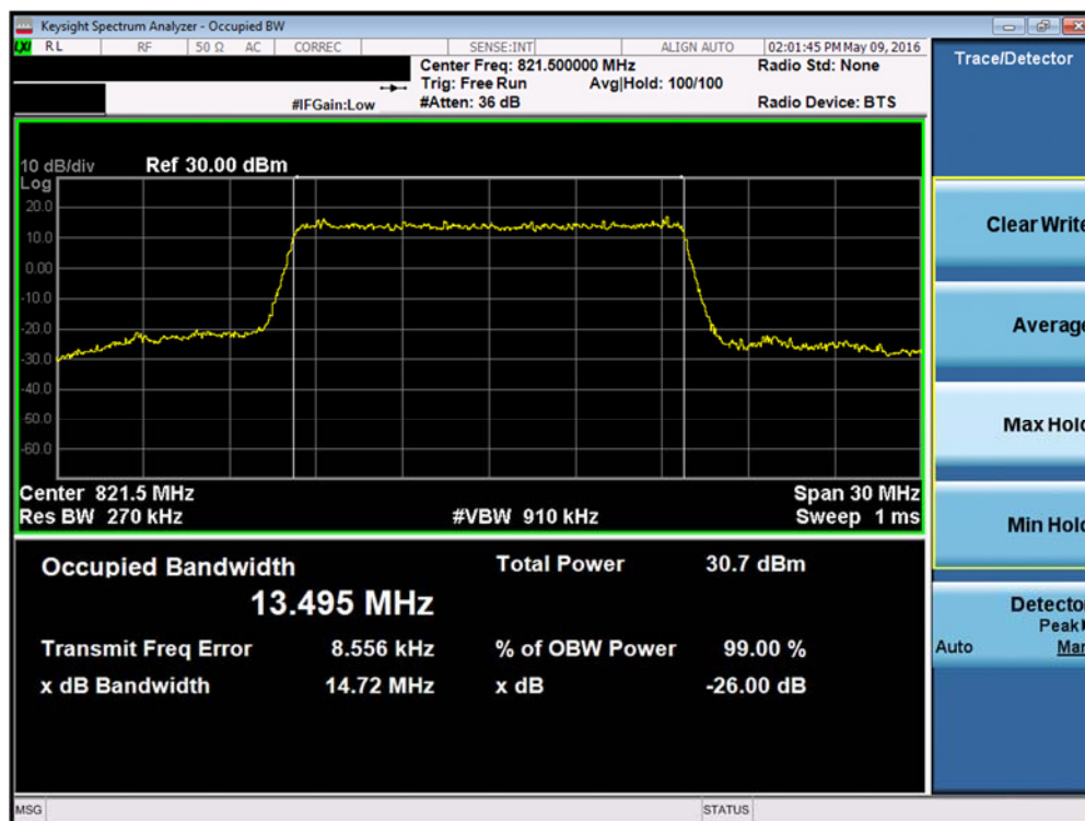
Plot 7-18. Occupied Bandwidth Plot (15MHz 16-QAM – RB Size 75)
