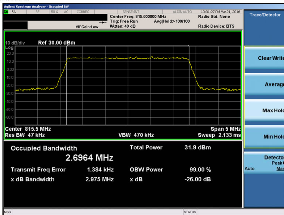
Plot 7-7. Occupied Bandwidth Plot (3MHz QPSK – RB Size 15– Low Channel)
