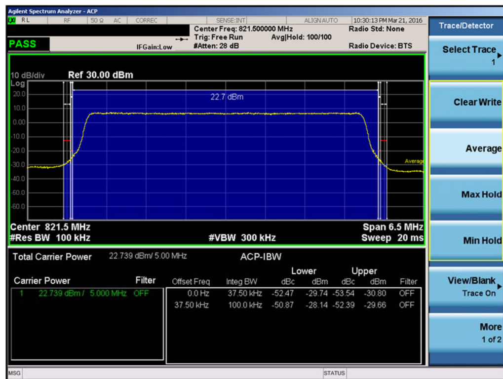
Plot 7-32. Channel Edge Plot (5MHz QPSK – RB Size 25 – High Channel)
