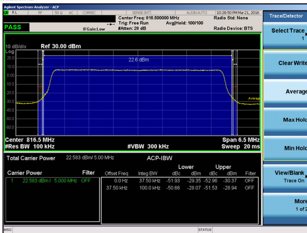
Plot 7-31. Channel Edge Plot (5MHz QPSK – RB Size 25– Low Channel)
