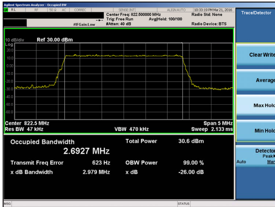
Plot 7-10. Occupied Bandwidth Plot (3MHz 16-QAM – RB Size 15– High Channel)
