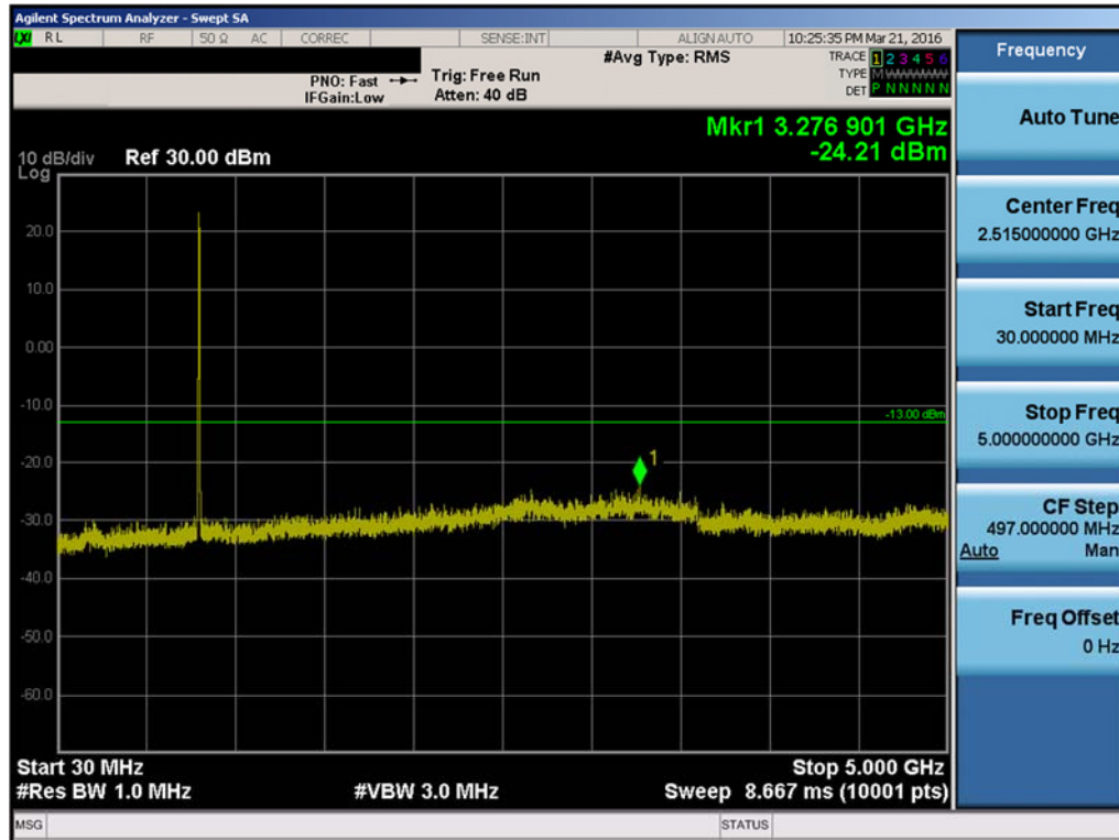
Plot 7-23. Conducted Spurious Plot ( 10MHz QPSK – RB Size 1, RB Offset 0 – Mid Channel)
