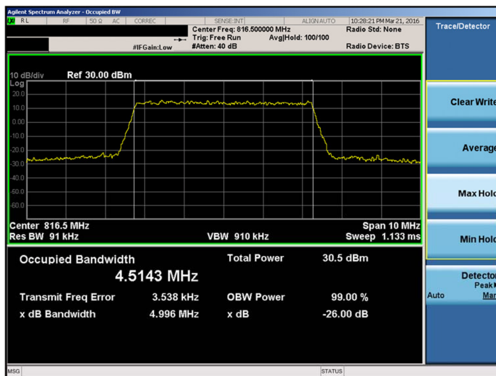
Plot 7-12. Occupied Bandwidth Plot (5MHz 16-QAM – RB Size 25– Low Channel)
