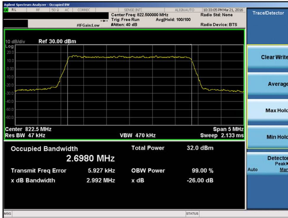
Plot 7-9. Occupied Bandwidth Plot (3MHz QPSK – RB Size 15– High Channel)
