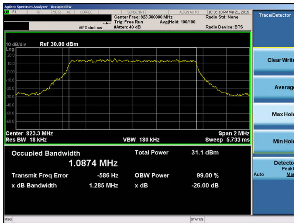
Plot 7-6. Occupied Bandwidth Plot (1.4MHz 16-QAM – RB Size 6– High Channel)
