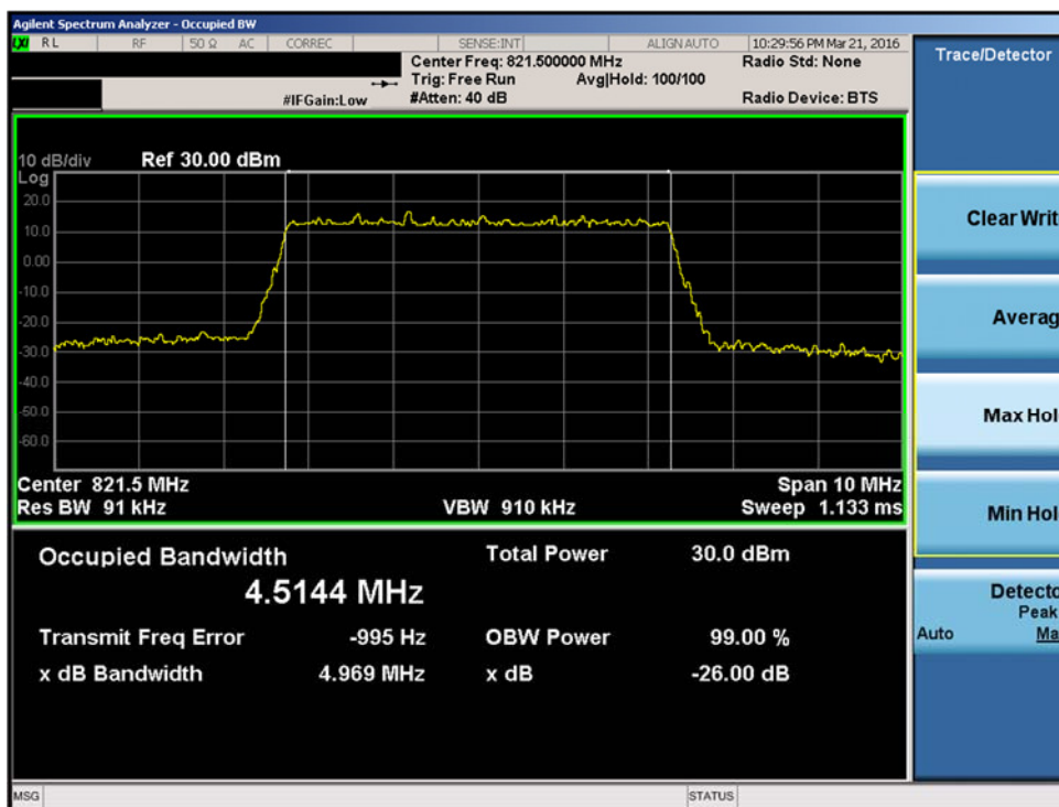
Plot 7-14. Occupied Bandwidth Plot (5MHz 16-QAM – RB Size 25– High Channel)
