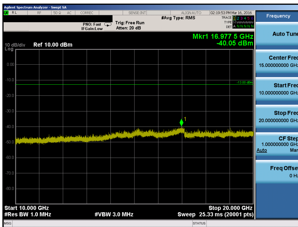
Plot 7-27. Conducted Spurious Plot (PCS GSM Mode – Ch. 810)
