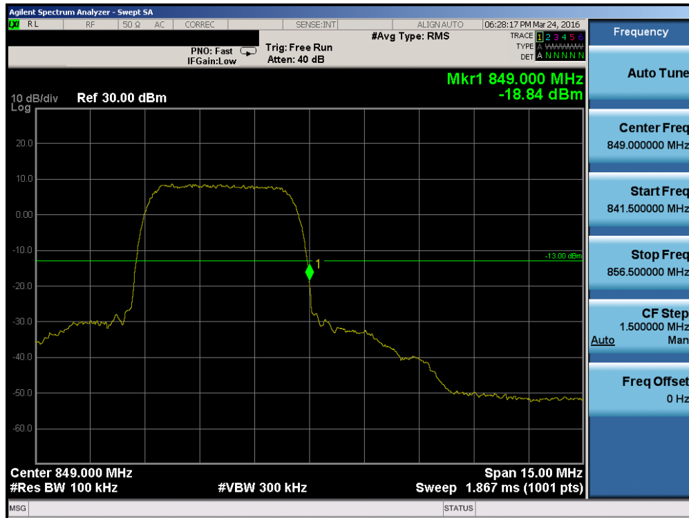
Plot 7-88. Band Edge Plot (Cellular WCDMA Mode – Ch. 4233)
