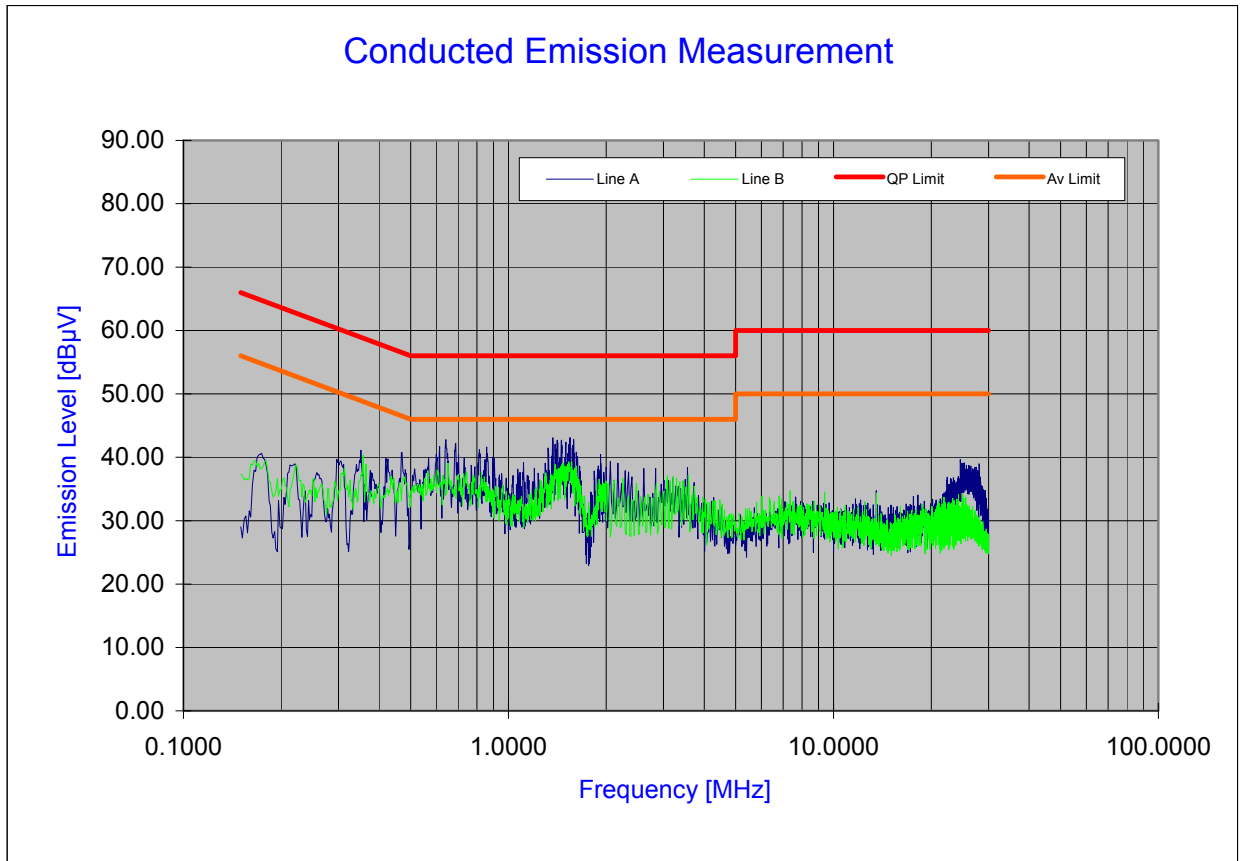
Plot 6-33. Line Conducted Plot with 802.11b
