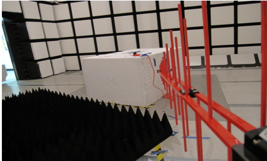
RADIATED FRONT PHOTO (BELOW 1 GHz)
