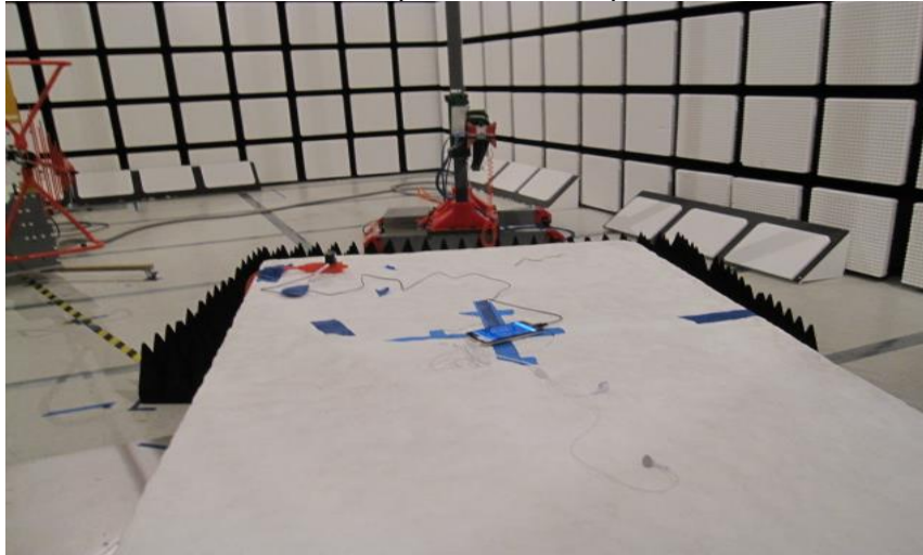
RADIATED BACK PHOTO (ABOVE 1 GHz)
