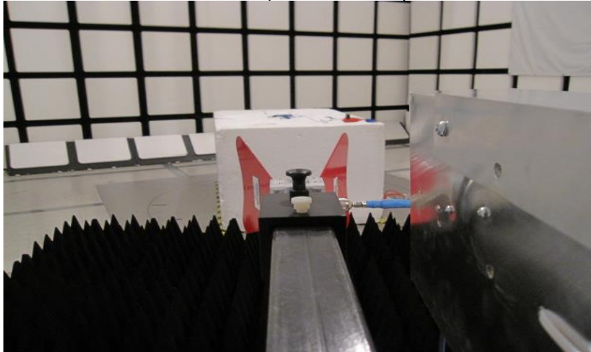
RADIATED FRONT PHOTO (ABOVE 1 GHz)
