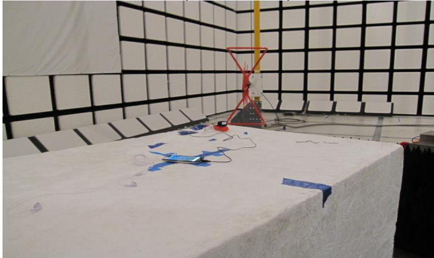
RADIATED BACK PHOTO (BELOW 1 GHz)
