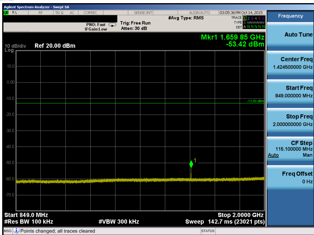
Plot 7-35. Conducted Spurious Plot (Band 26 – 15.0MHz QPSK – RB Size 1, RB Offset 0 – Mid Channel)
