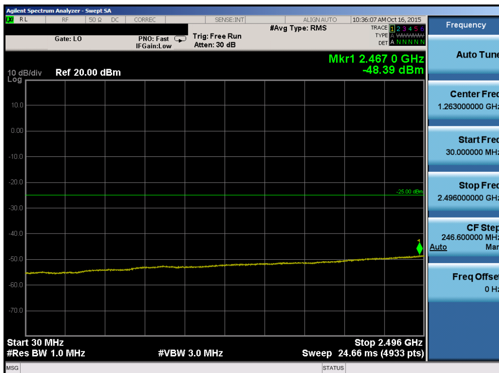
Plot 7-82. Conducted Spurious Plot (Band 41 – 20.0MHz QPSK – RB Size 1, RB Offset 0 – High Channel)
