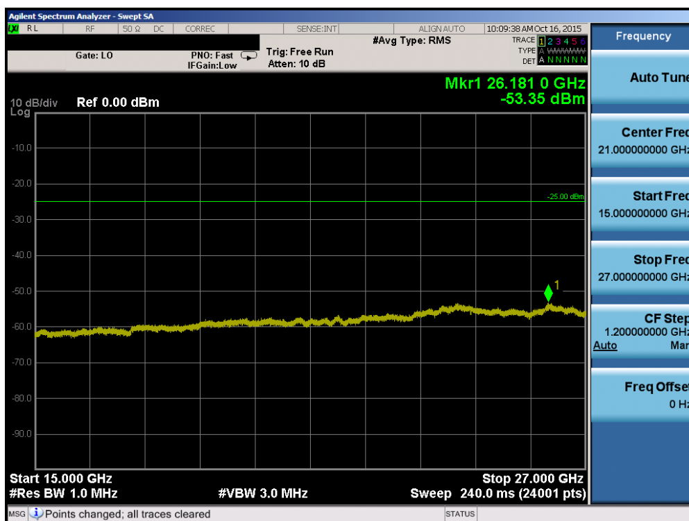
Plot 7-72. Conducted Spurious Plot (Band 41 – 15.0MHz QPSK – RB Size 1, RB Offset 0 – Mid Channel)
