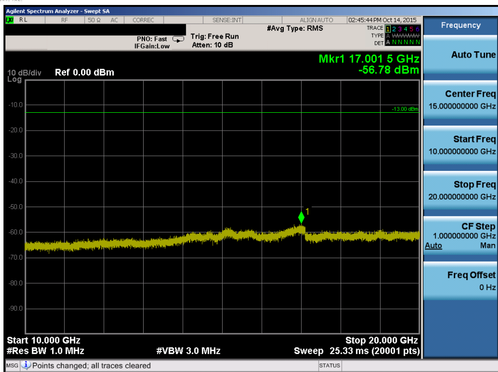
Plot 7-45. Conducted Spurious Plot (Band 25 – 20.0MHz QPSK – RB Size 1, RB Offset 0 – Mid Channel)
