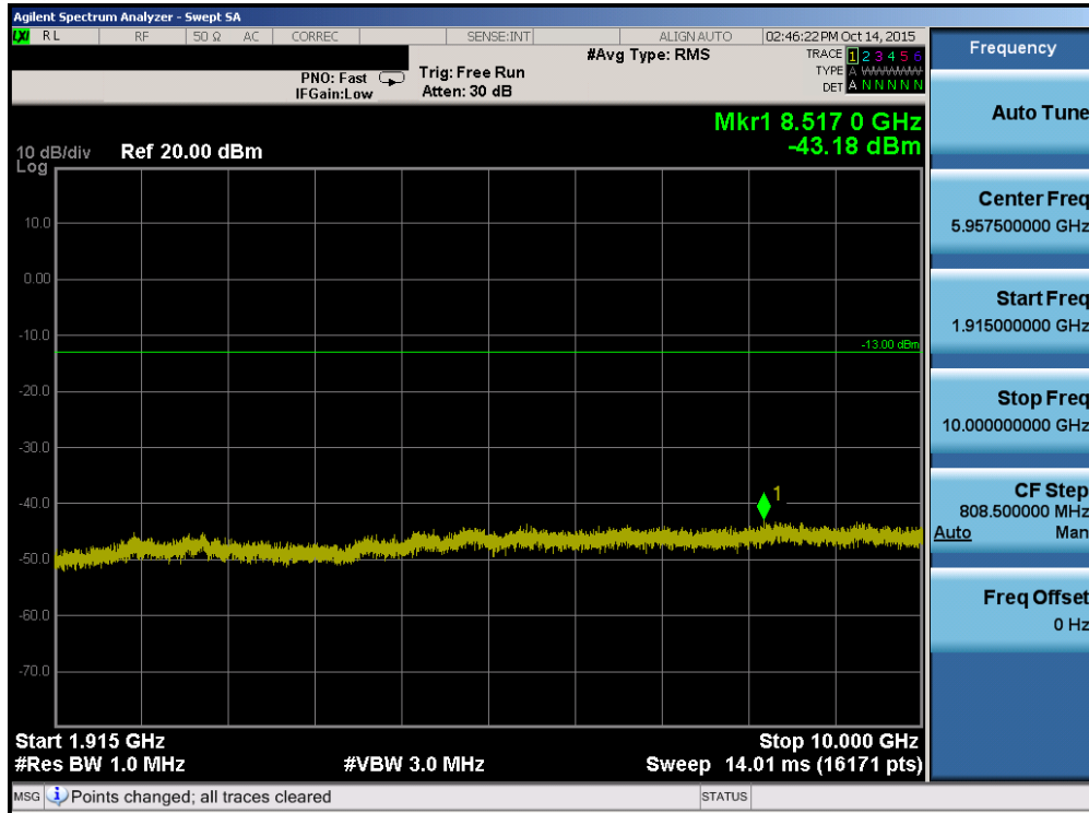
Plot 7-41. Conducted Spurious Plot (Band 25 – 20.0MHz QPSK – RB Size 1, RB Offset 0 – Low Channel)
