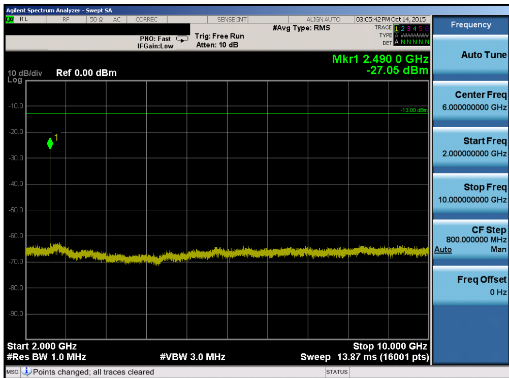
Plot 7-36. Conducted Spurious Plot (Band 26 – 15.0MHz QPSK – RB Size 1, RB Offset 0 – Mid Channel)
