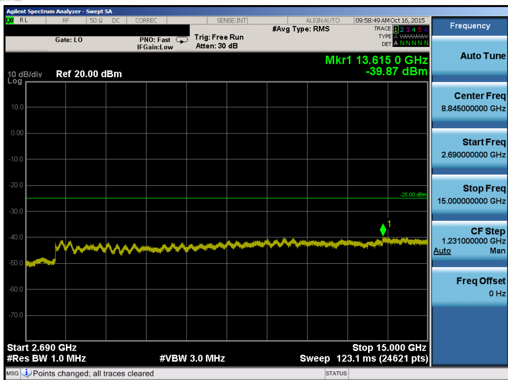
Plot 7-59. Conducted Spurious Plot (Band 41 – 10.0MHz QPSK – RB Size 1, RB Offset 0 – Low Channel)
