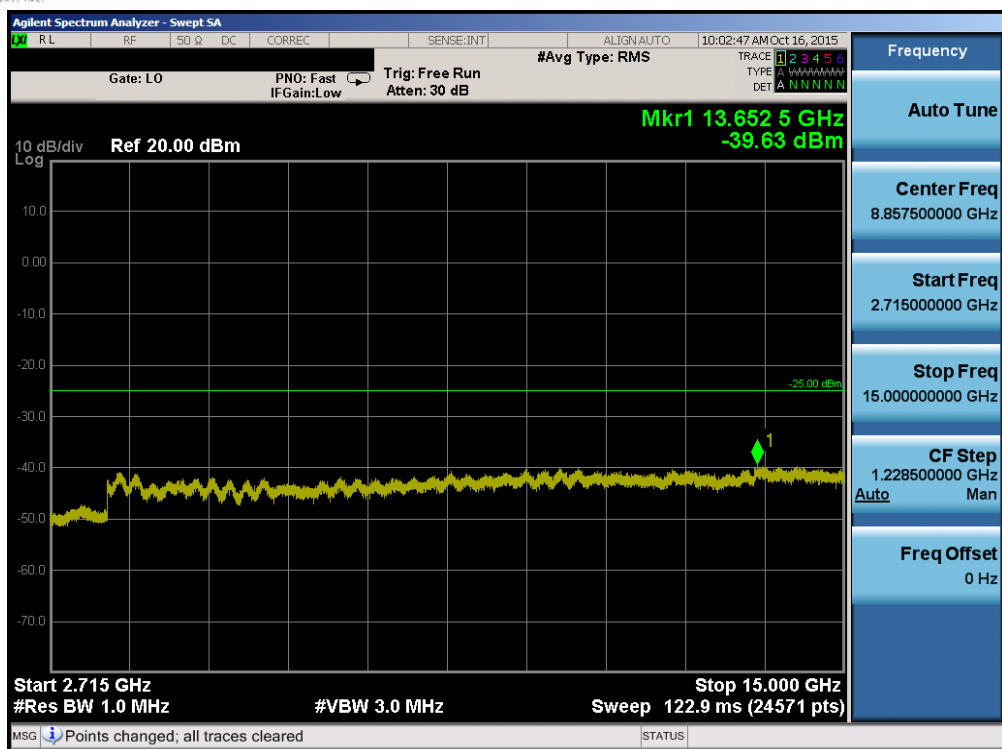
Plot 7-65. Conducted Spurious Plot (Band 41 – 10.0MHz QPSK – RB Size 1, RB Offset 0 – High Channel)
