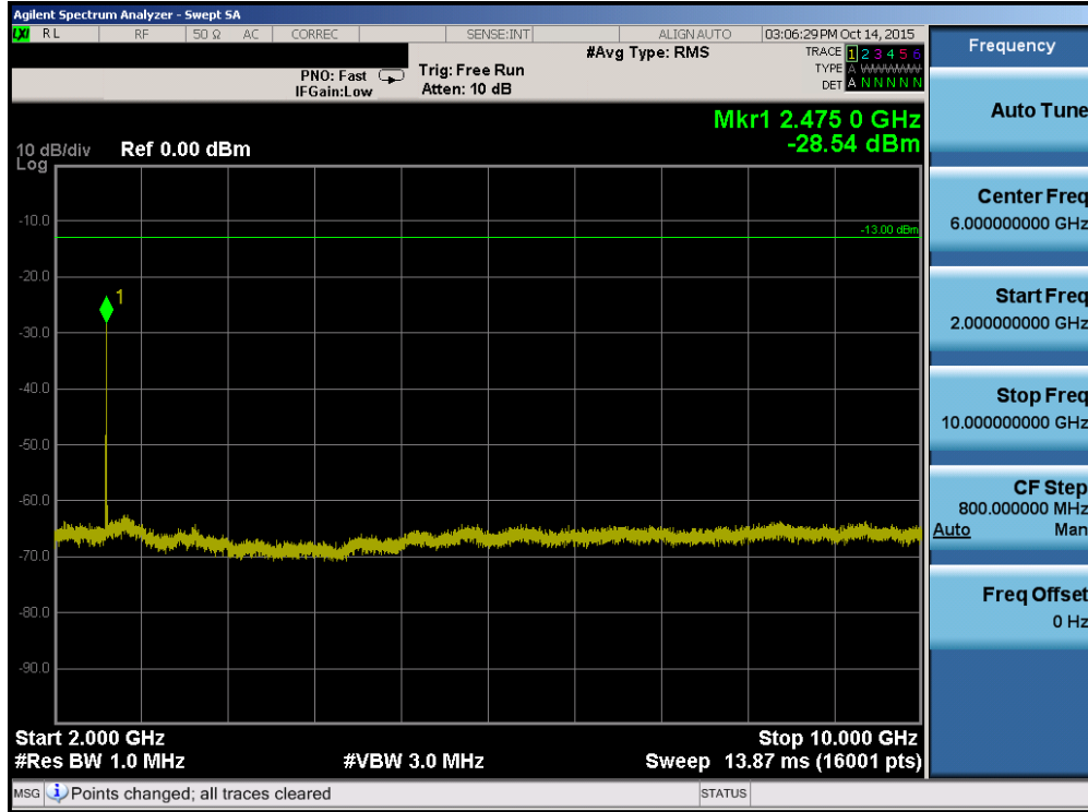
Plot 7-33. Conducted Spurious Plot (Band 26 – 15.0MHz QPSK – RB Size 1, RB Offset 0 – Low Channel)
