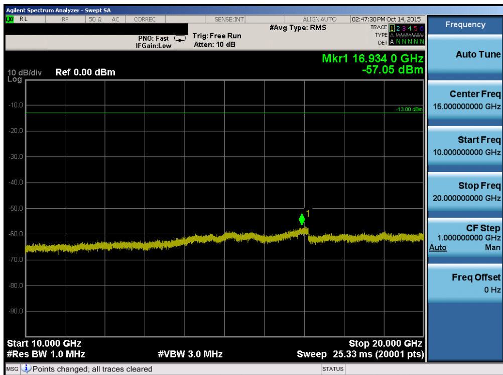
Plot 7-48. Conducted Spurious Plot (Band 25 – 20.0MHz QPSK – RB Size 1, RB Offset 0 – High Channel)
