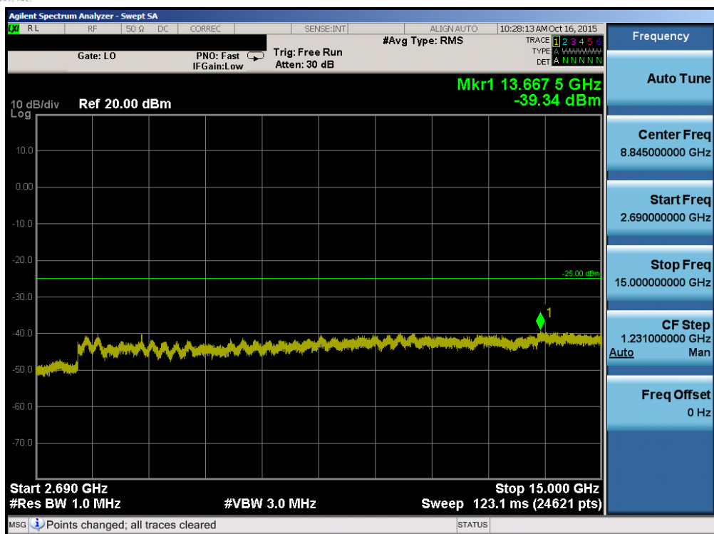
Plot 7-77. Conducted Spurious Plot (Band 41 – 20.0MHz QPSK – RB Size 1, RB Offset 0 – Low Channel)
