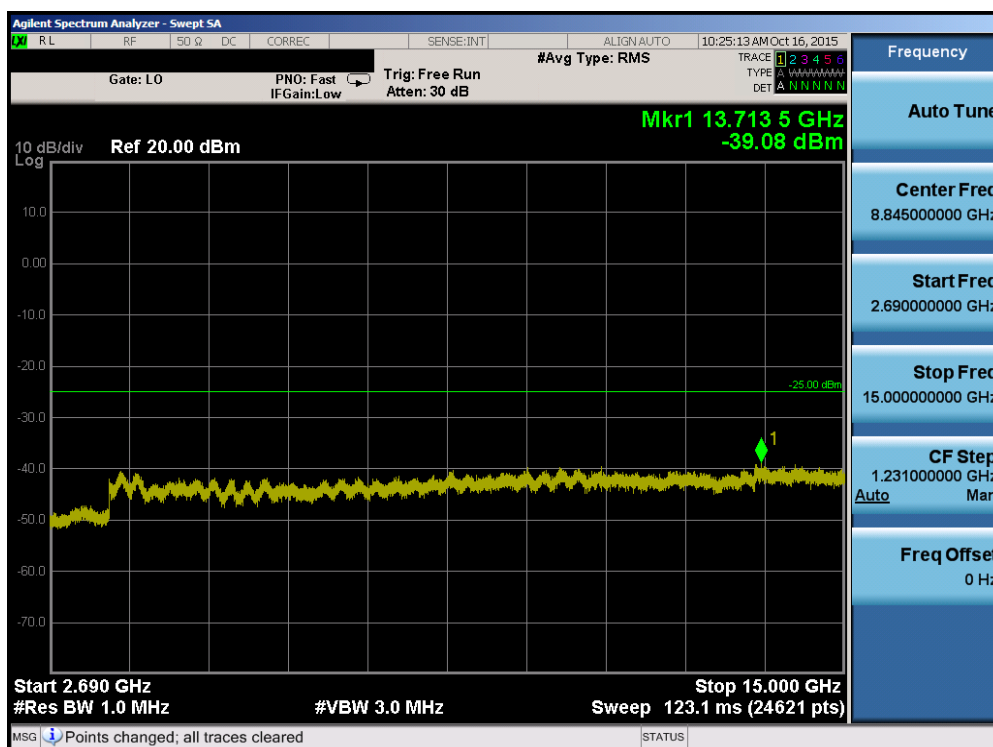
Plot 7-80. Conducted Spurious Plot (Band 41 – 20.0MHz QPSK – RB Size 1, RB Offset 0 – Mid Channel)
