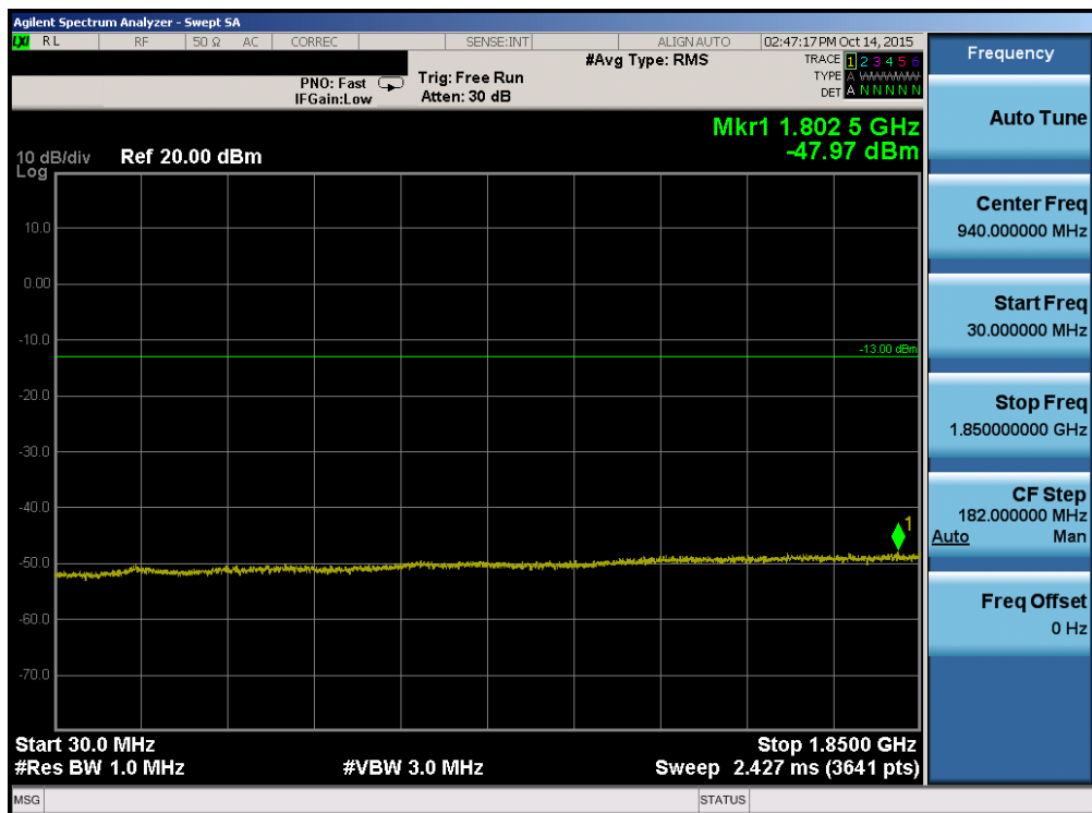
Plot 7-46. Conducted Spurious Plot (Band 25 – 20.0MHz QPSK – RB Size 1, RB Offset 0 – High Channel)
