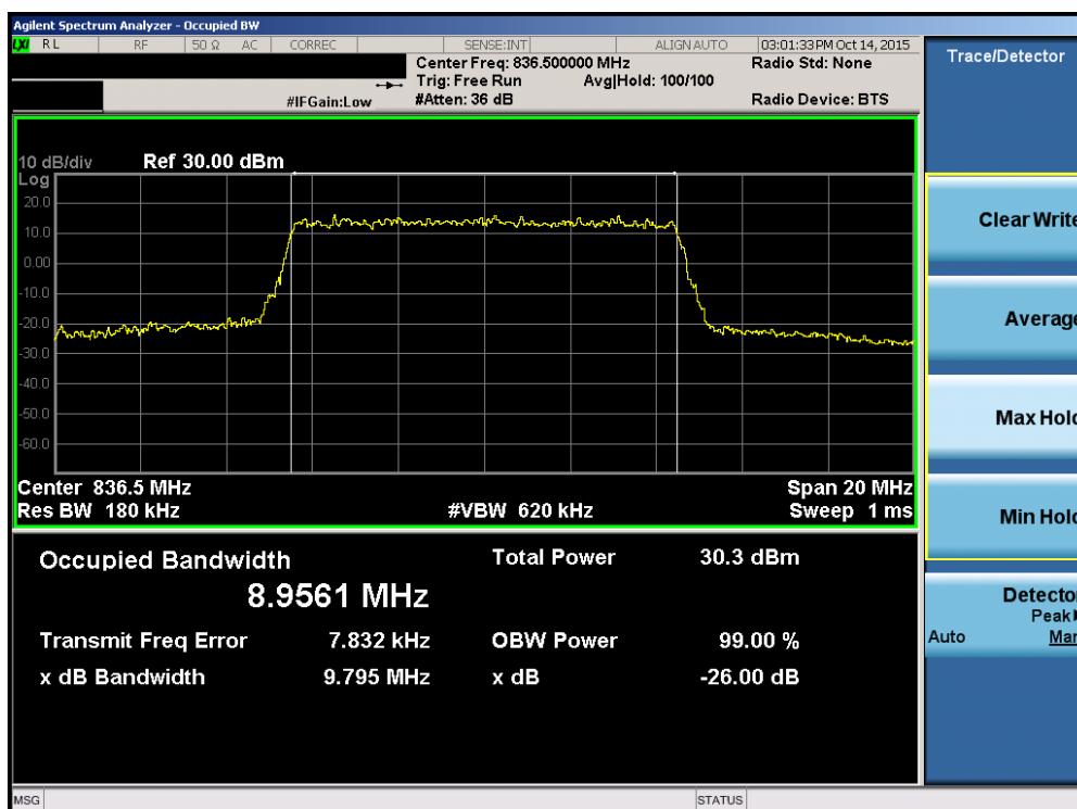
Plot 7-8. Occupied Bandwidth Plot (Band 26 – 10.0MHz 16-QAM – RB Size 50)
