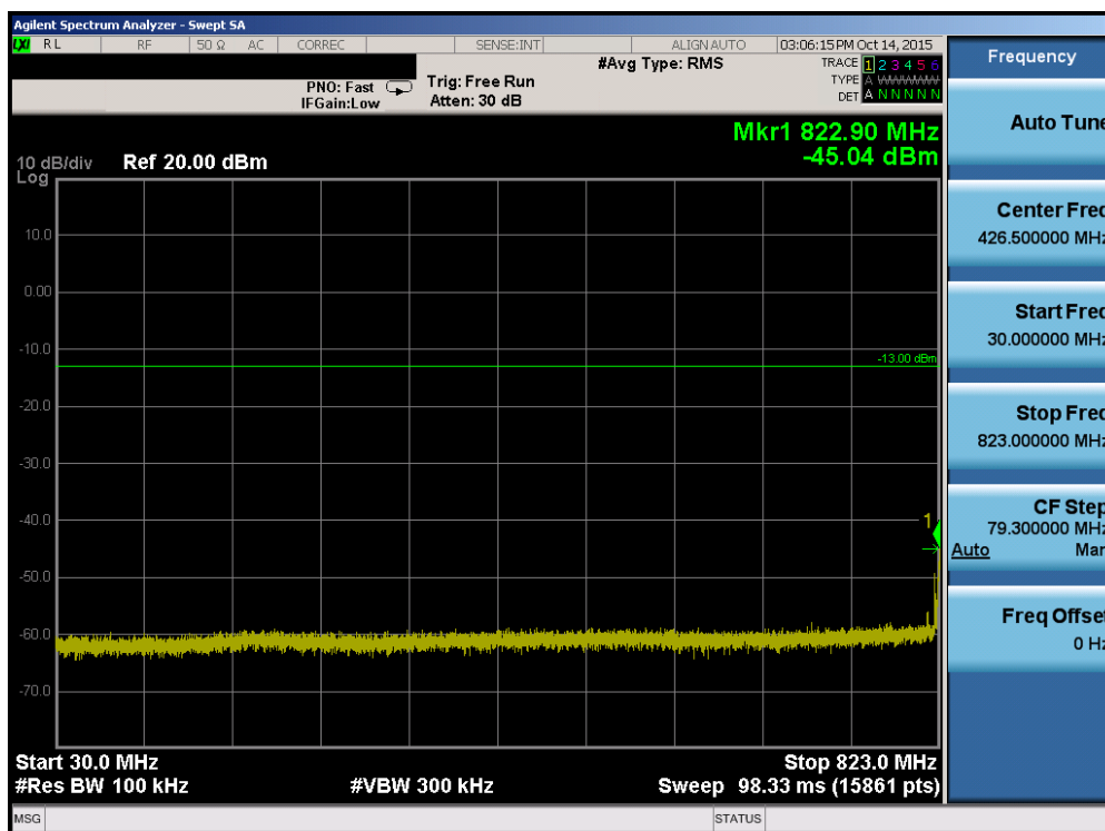
Plot 7-31. Conducted Spurious Plot (Band 26 – 15.0MHz QPSK – RB Size 1, RB Offset 0 – Low Channel)
