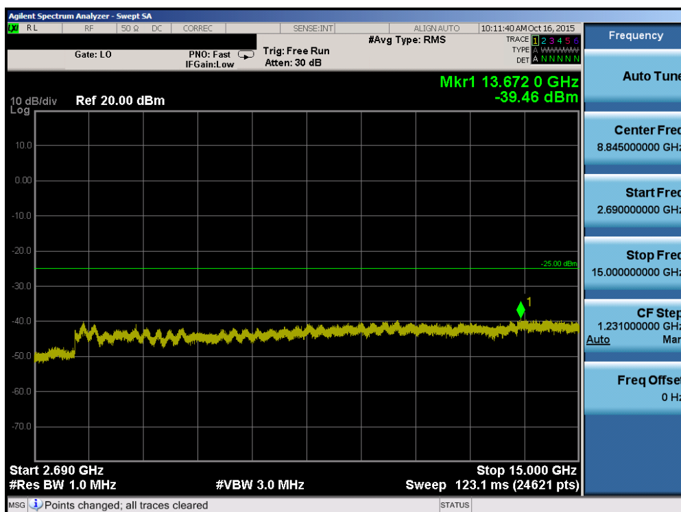
Plot 7-68. Conducted Spurious Plot (Band 41 – 15.0MHz QPSK – RB Size 1, RB Offset 0 – Low Channel)
