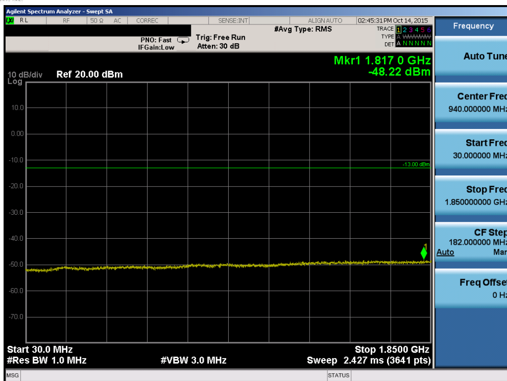
Plot 7-43. Conducted Spurious Plot (Band 25 – 20.0MHz QPSK – RB Size 1, RB Offset 0 – Mid Channel)
