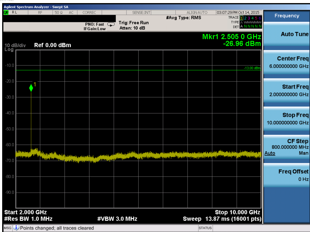
Plot 7-39. Conducted Spurious Plot (Band 26 – 15.0MHz QPSK – RB Size 1, RB Offset 0 – High Channel)
