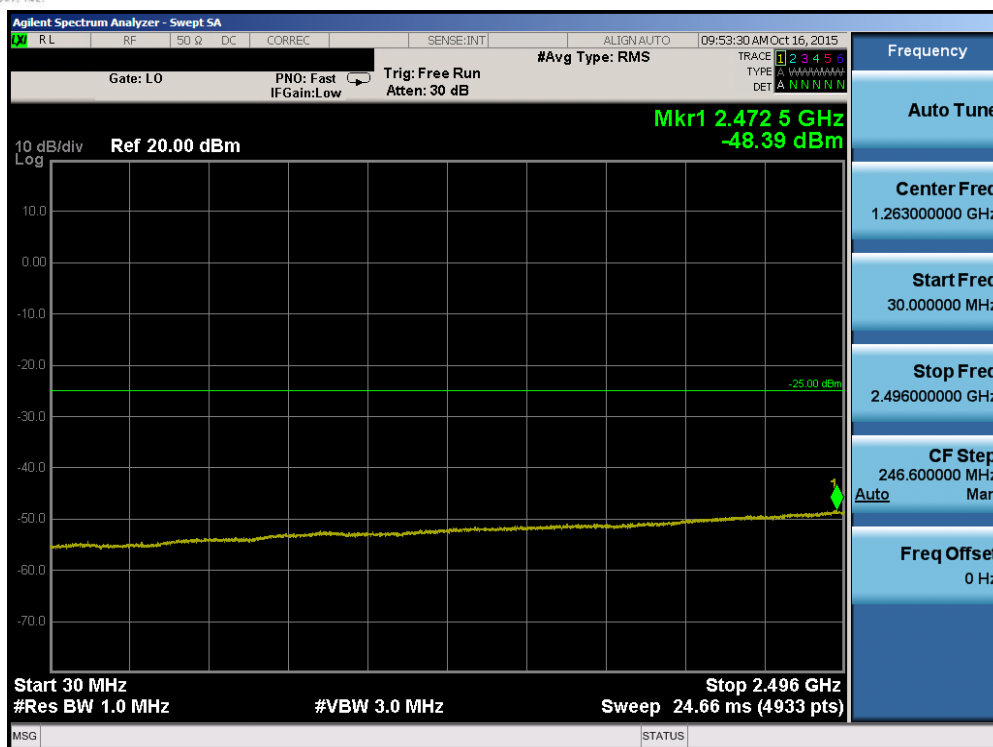
Plot 7-61. Conducted Spurious Plot (Band 41 – 10.0MHz QPSK – RB Size 1, RB Offset 0 – Mid Channel)
