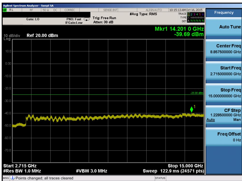
Plot 7-74. Conducted Spurious Plot (Band 41 – 15.0MHz QPSK – RB Size 1, RB Offset 0 – High Channel)
