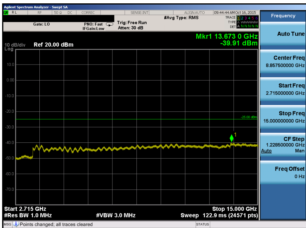
Plot 7-56. Conducted Spurious Plot (Band 41 – 5.0MHz QPSK – RB Size 1, RB Offset 0 – High Channel)
