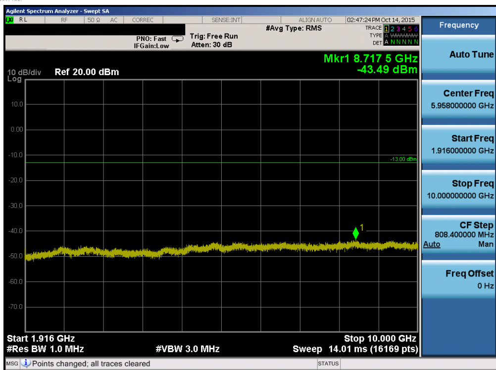
Plot 7-47. Conducted Spurious Plot (Band 25 – 20.0MHz QPSK – RB Size 1, RB Offset 0 – High Channel)
