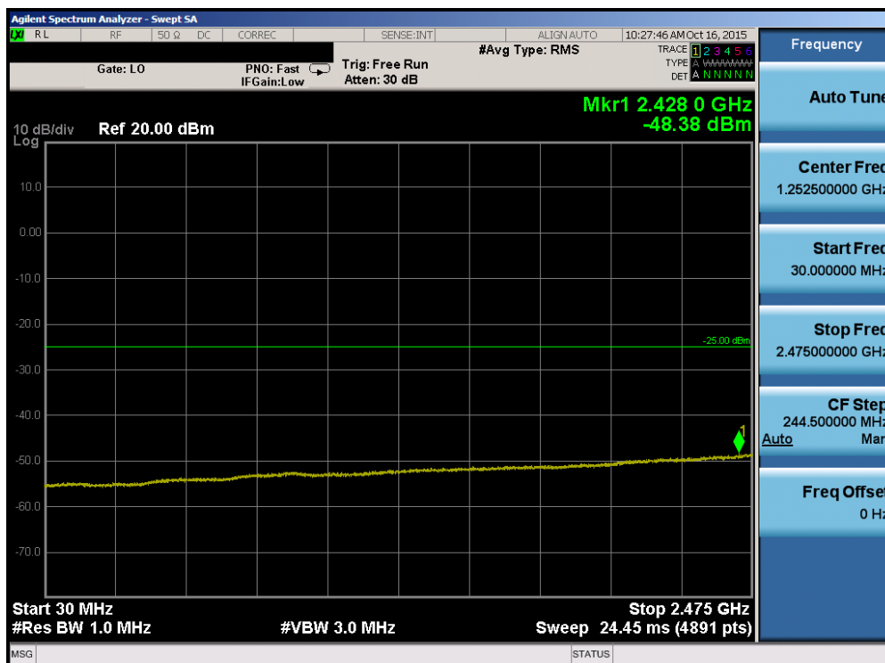
Plot 7-76. Conducted Spurious Plot (Band 41 – 20.0MHz QPSK – RB Size 1, RB Offset 0– Low Channel)
