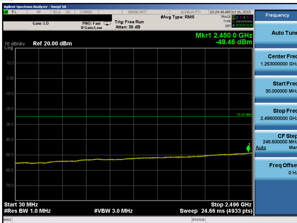
Plot 7-79. Conducted Spurious Plot (Band 41 – 20.0MHz QPSK – RB Size 1, RB Offset 0 – Mid Channel)
