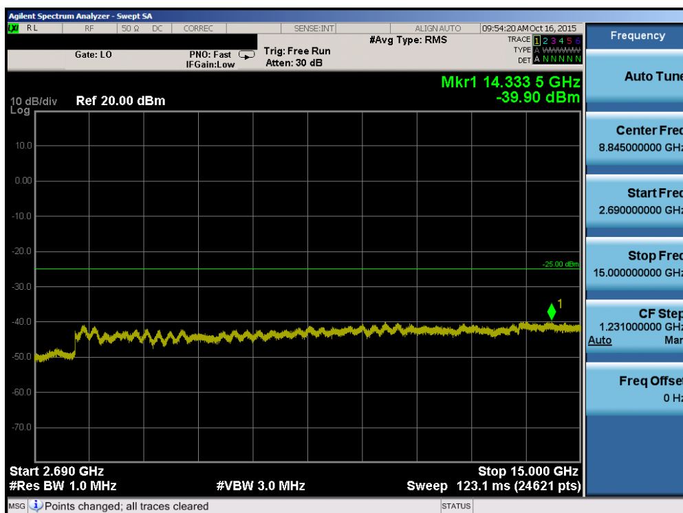
Plot 7-62. Conducted Spurious Plot (Band 41 – 10.0MHz QPSK – RB Size 1, RB Offset 0 – Mid Channel)
