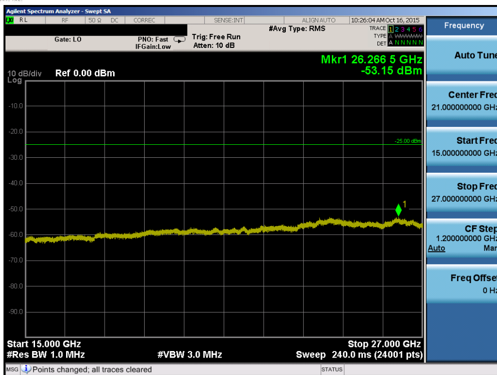
Plot 7-81. Conducted Spurious Plot (Band 41 – 20.0MHz QPSK – RB Size 1, RB Offset 0 – Mid Channel)
