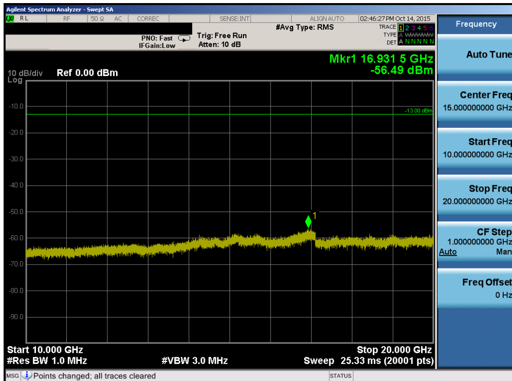
Plot 7-42. Conducted Spurious Plot (Band 25 – 20.0MHz QPSK – RB Size 1, RB Offset 0 – Low Channel)
