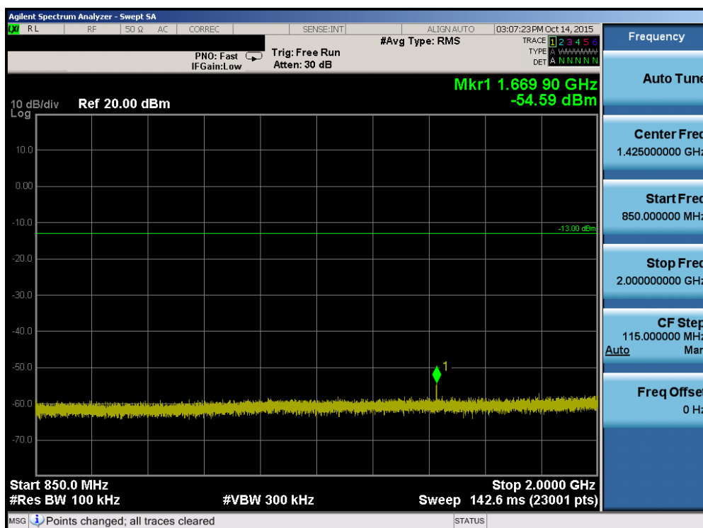
Plot 7-38. Conducted Spurious Plot (Band 26 – 15.0MHz QPSK – RB Size 1, RB Offset 0 – High Channel)
