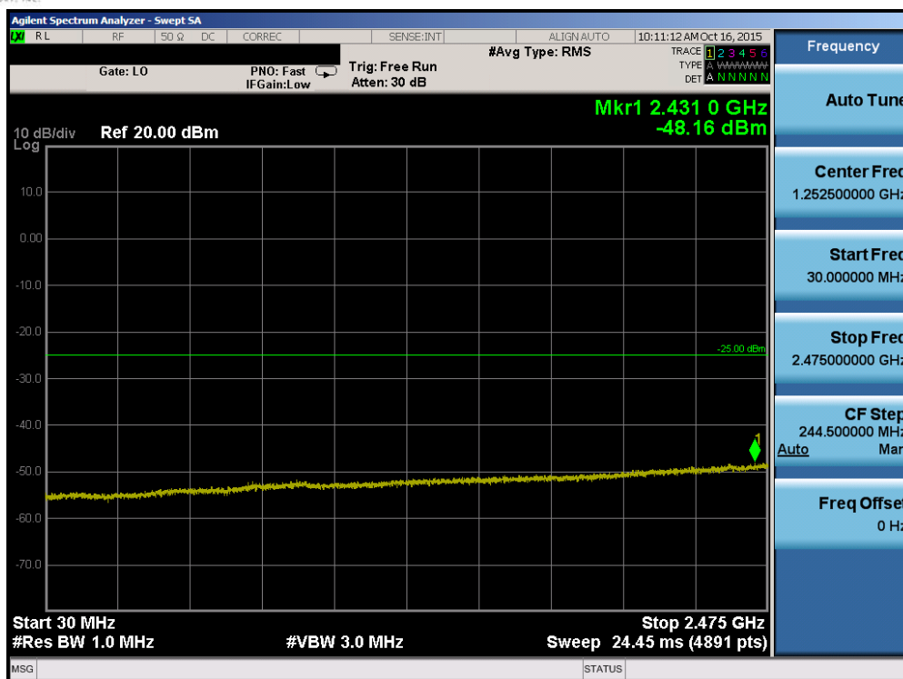
Plot 7-67. Conducted Spurious Plot (Band 41 – 15.0MHz QPSK – RB Size 1, RB Offset 0 – Low Channel)
