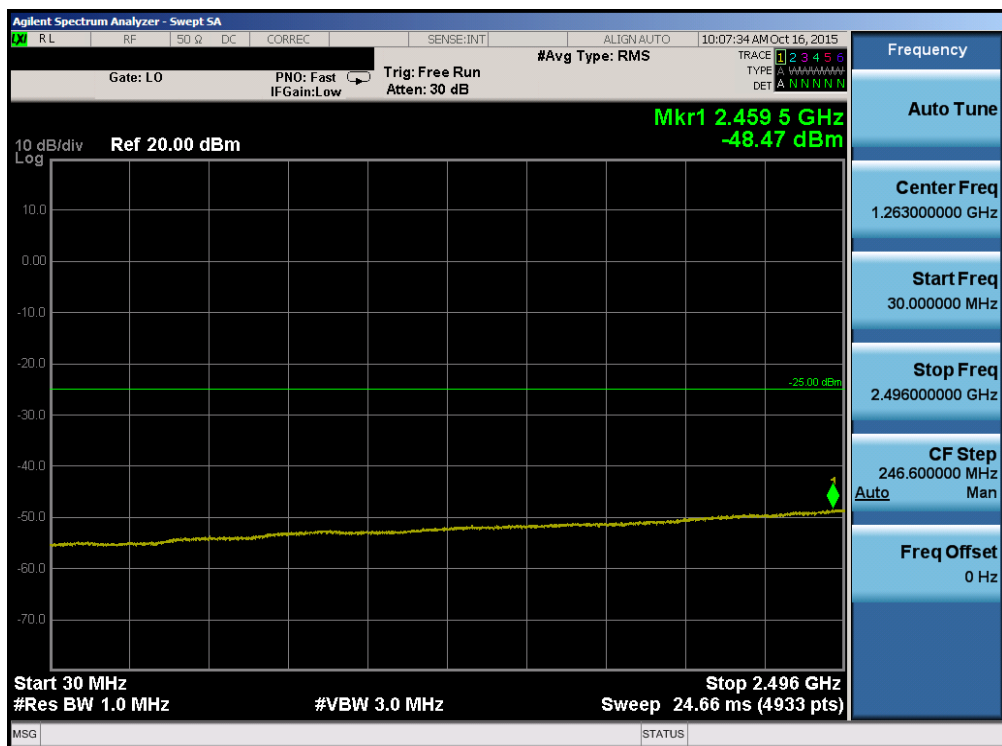
Plot 7-70. Conducted Spurious Plot (Band 41 – 15.0MHz QPSK – RB Size 1, RB Offset 0 – Mid Channel)
