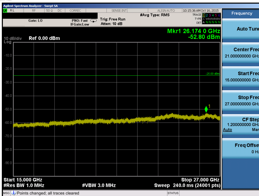
Plot 7-75. Conducted Spurious Plot (Band 41 – 15.0MHz QPSK – RB Size 1, RB Offset 0 – High Channel)
