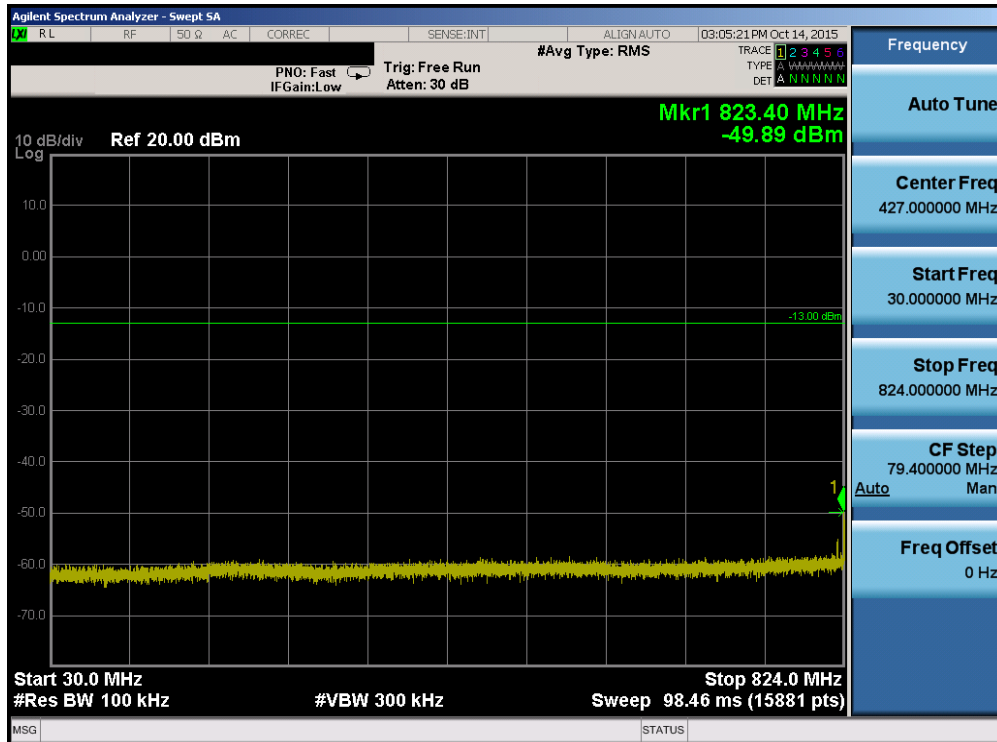
Plot 7-34. Conducted Spurious Plot (Band 26 – 15.0MHz QPSK – RB Size 1, RB Offset 0 – Mid Channel)
