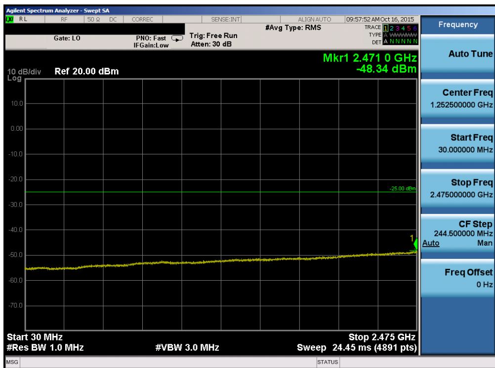
Plot 7-58. Conducted Spurious Plot (Band 41 – 10.0MHz QPSK – RB Size 1, RB Offset 0– Low Channel)
