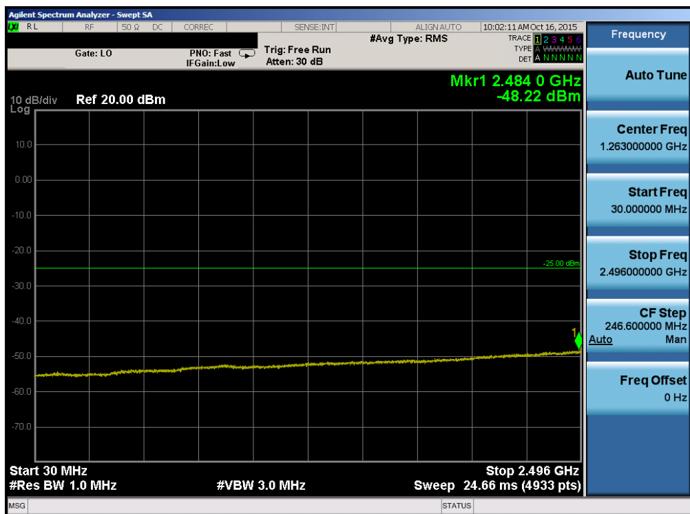
Plot 7-64. Conducted Spurious Plot (Band 41 – 10.0MHz QPSK – RB Size 1, RB Offset 0 – High Channel)
