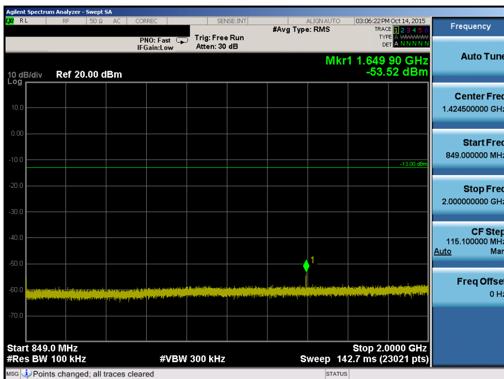
Plot 7-32. Conducted Spurious Plot (Band 26 – 15.0MHz QPSK – RB Size 1, RB Offset 0 – Low Channel)
