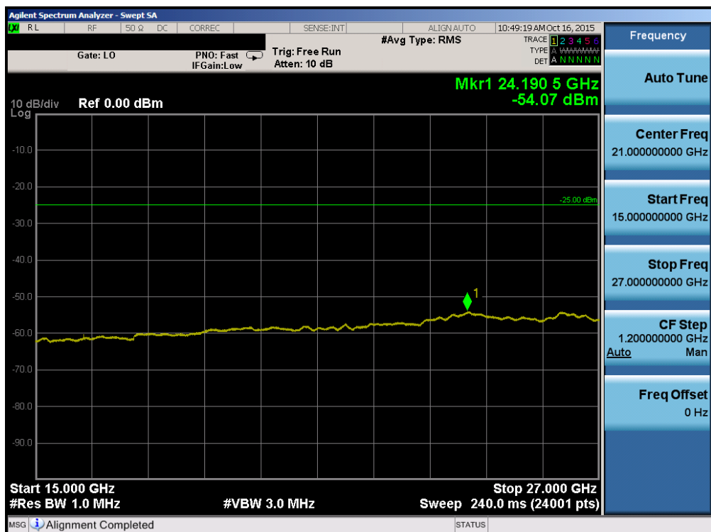
Plot 7-84. Conducted Spurious Plot (Band 41 – 20.0MHz QPSK – RB Size 1, RB Offset 0 – High Channel)
