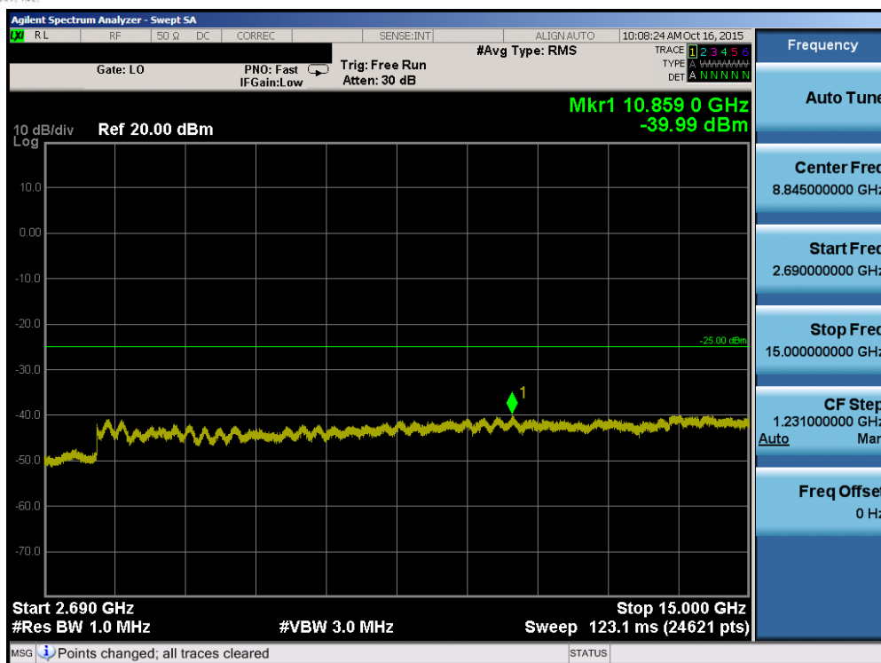
Plot 7-71. Conducted Spurious Plot (Band 41 – 15.0MHz QPSK – RB Size 1, RB Offset 0 – Mid Channel)
