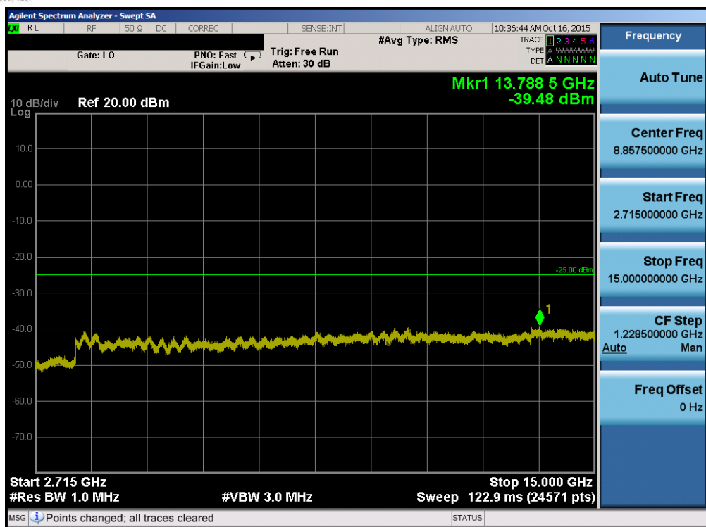
Plot 7-83. Conducted Spurious Plot (Band 41 – 20.0MHz QPSK – RB Size 1, RB Offset 0 – High Channel)
