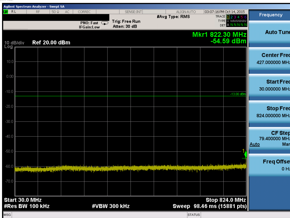
Plot 7-37. Conducted Spurious Plot (Band 26 – 15.0MHz QPSK – RB Size 1, RB Offset 0 – High Channel)
