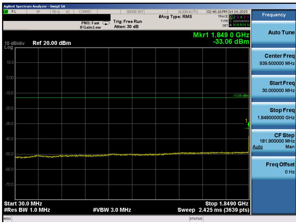
Plot 7-40. Conducted Spurious Plot (Band 25 – 20.0MHz QPSK – RB Size 1, RB Offset 0– Low Channel)
