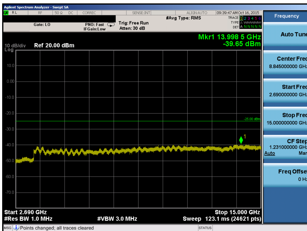
Plot 7-50. Conducted Spurious Plot (Band 41 – 5.0MHz QPSK – RB Size 1, RB Offset 0 – Low Channel)
