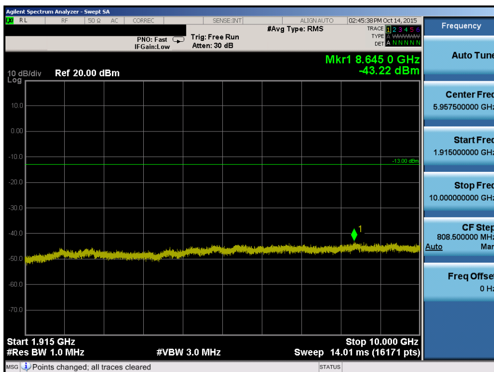
Plot 7-44. Conducted Spurious Plot (Band 25 – 20.0MHz QPSK – RB Size 1, RB Offset 0 – Mid Channel)
