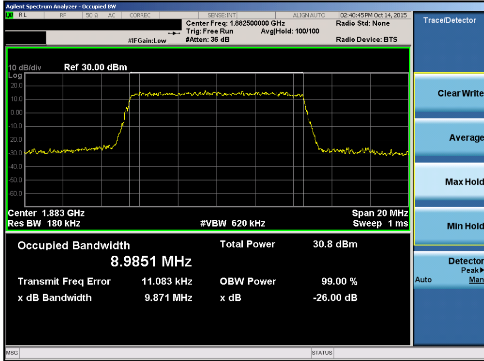
Plot 7-17. Occupied Bandwidth Plot (Band 25 – 10.0MHz QPSK – RB Size 50)
