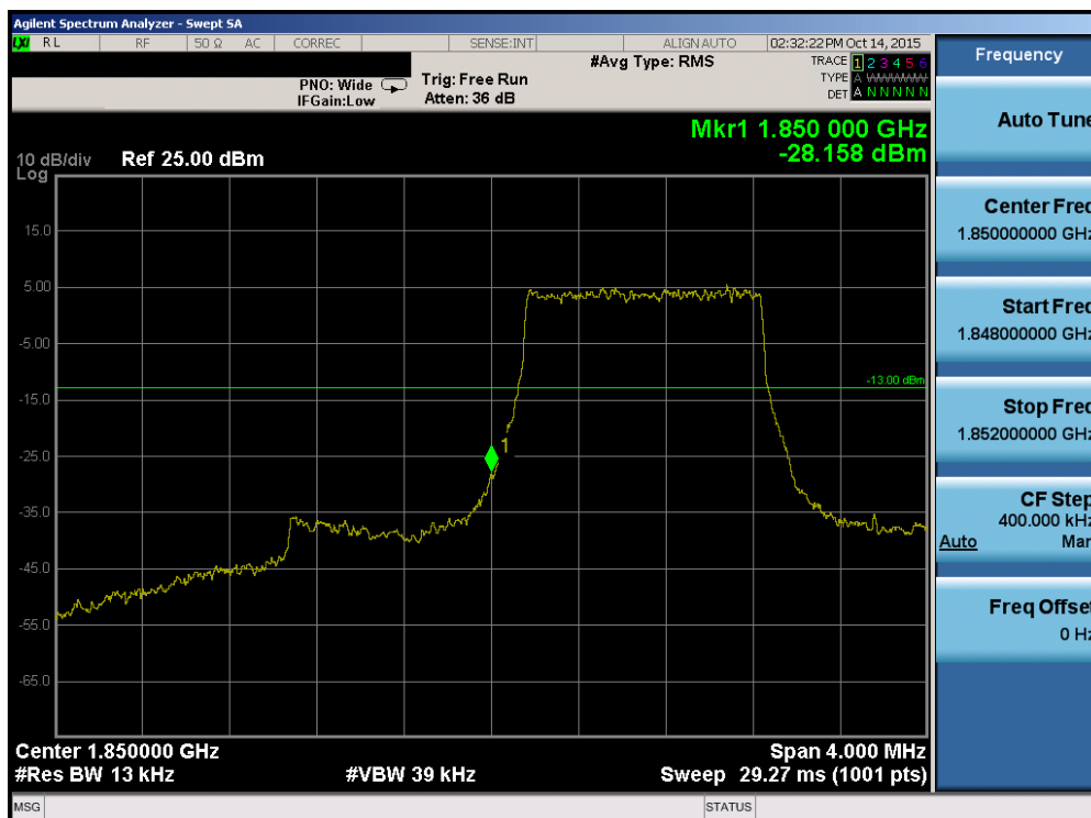
Plot 7-101. Lower Band Edge Plot (Band 25 – 1.4MHz QPSK – RB Size 6)
