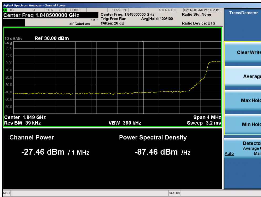
Plot 7-110. Lower Extended Band Edge Plot (Band 25 – 5.0MHz QPSK – RB Size 25)
