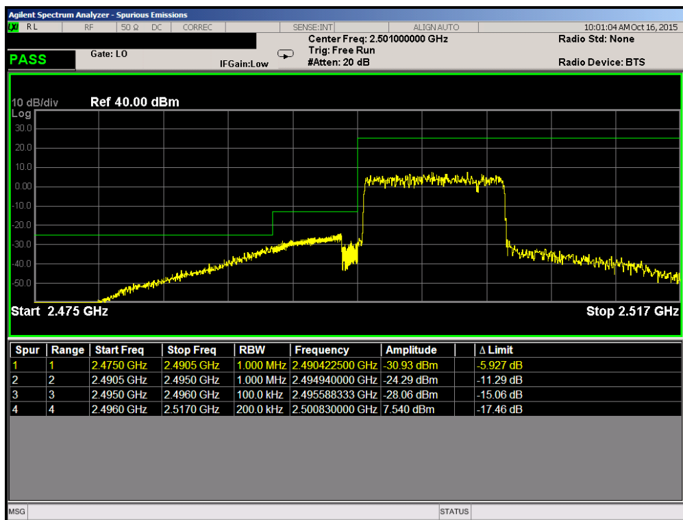
Plot 7-127. Lower ACP Plot (Band 41 – 10.0MHz QPSK – RB Size 50)
