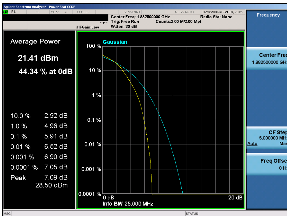
Plot 7-144. PAR Plot (Band 25 – 20.0MHz 16-QAM – RB Size 100)
