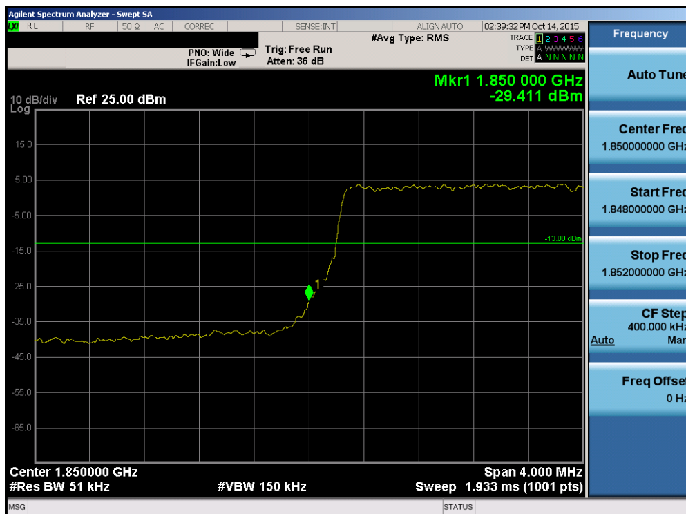
Plot 7-109. Lower Band Edge Plot (Band 25 – 5.0MHz QPSK – RB Size 25)
