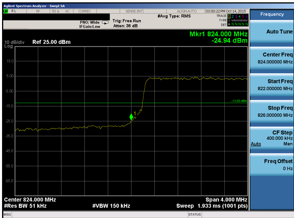
Plot 7-93. Lower Band Edge Plot (Band 26 – 5.0MHz QPSK – RB Size 25)
