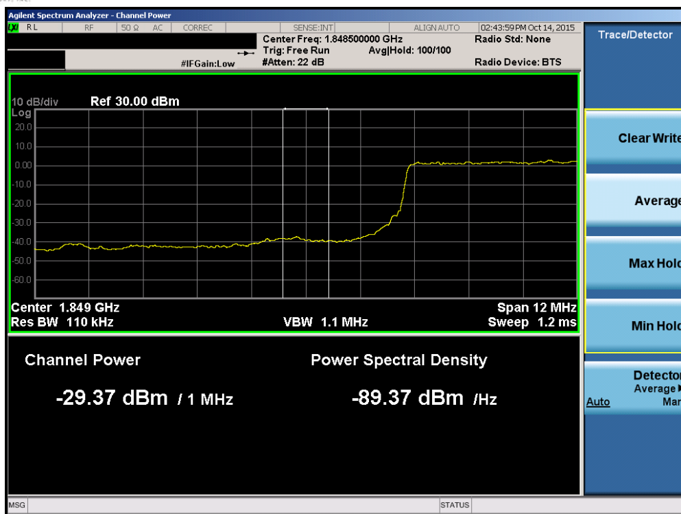
Plot 7-118. Lower Extended Band Edge Plot (Band 25 – 15.0MHz QPSK – RB Size 75)
