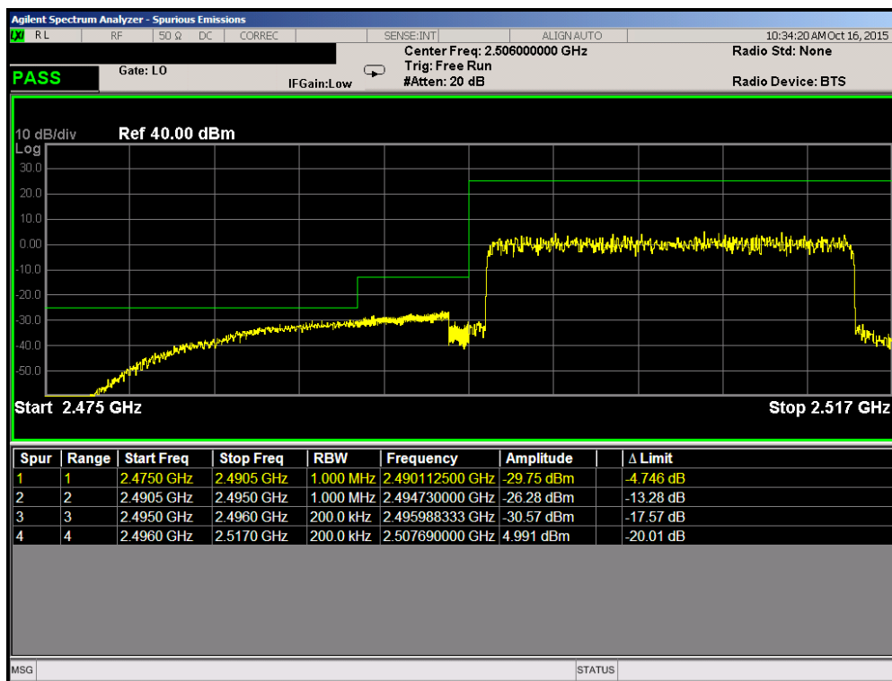
Plot 7-131. Lower ACP Plot (Band 41 – 20.0MHz QPSK – RB Size 100)
