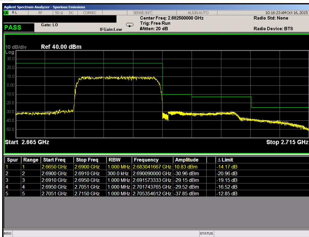
Plot 7-130. Upper ACP Plot (Band 41 – 15.0MHz QPSK – RB Size 75)
