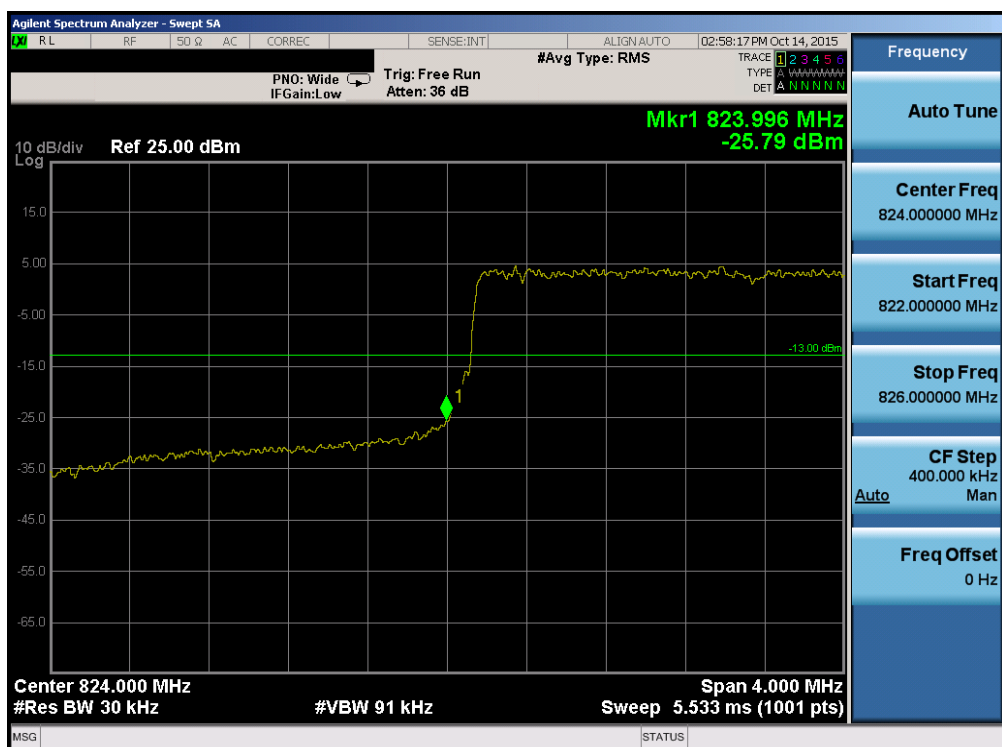
Plot 7-89. Lower Band Edge Plot (Band 26 – 3.0MHz QPSK – RB Size 15)
