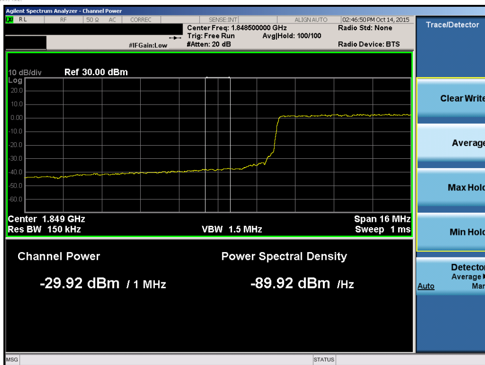
Plot 7-122. Lower Extended Band Edge Plot (Band 25 – 20.0MHz QPSK – RB Size 100)
