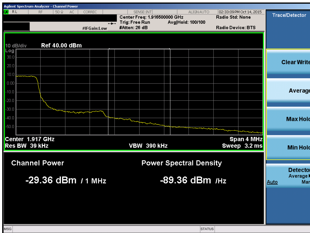
Plot 7-104. Upper Extended Band Edge Plot (Band 25 – 1.4MHz QPSK – RB Size 6)
