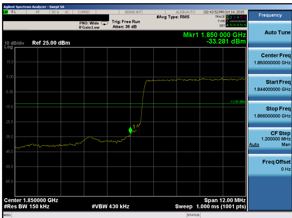
Plot 7-117. Lower Band Edge Plot (Band 25 – 15.0MHz QPSK – RB Size 75)
