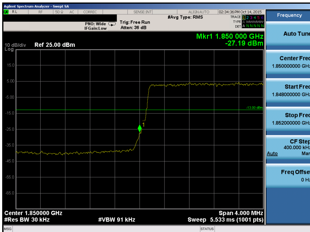
Plot 7-105. Lower Band Edge Plot (Band 25 – 3.0MHz QPSK – RB Size 15)
