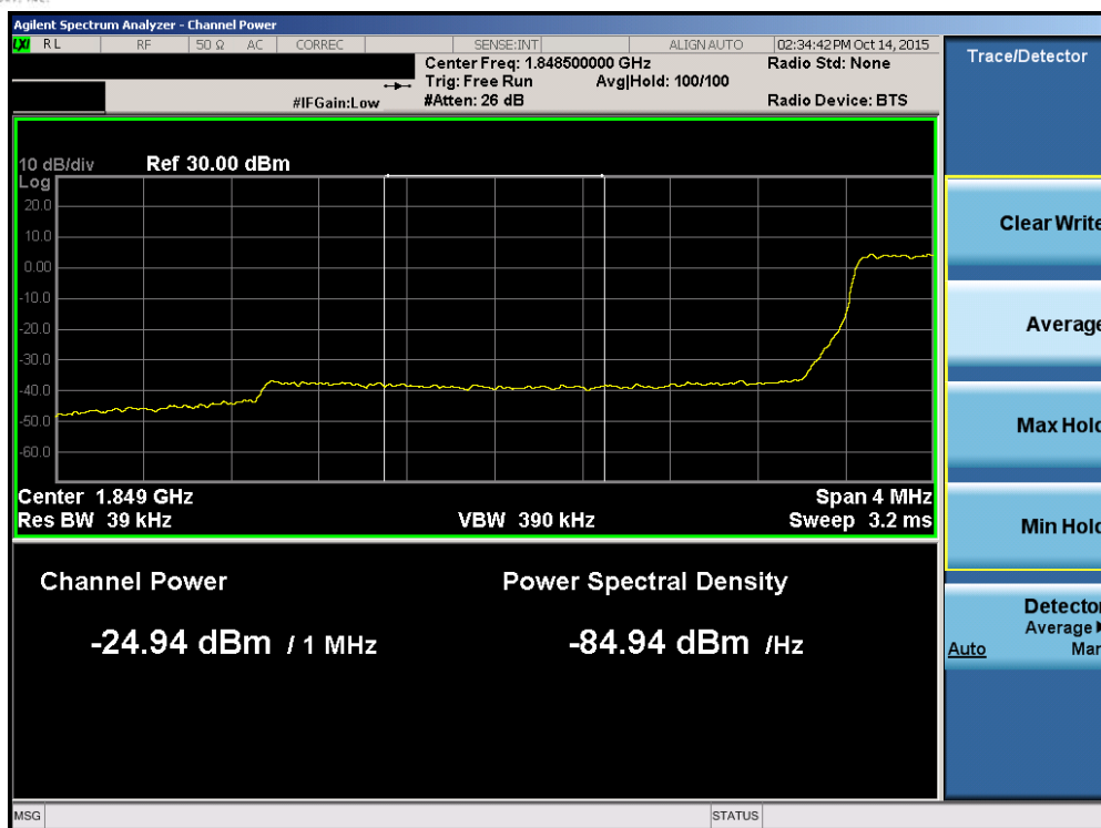
Plot 7-106. Lower Extended Band Edge Plot (Band 25 – 3.0MHz QPSK – RB Size 15)
