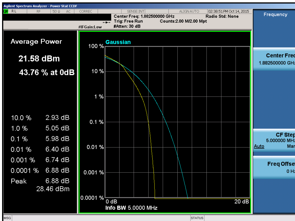
Plot 7-138. PAR Plot (Band 25 – 5.0MHz 16-QAM – RB Size 25)
