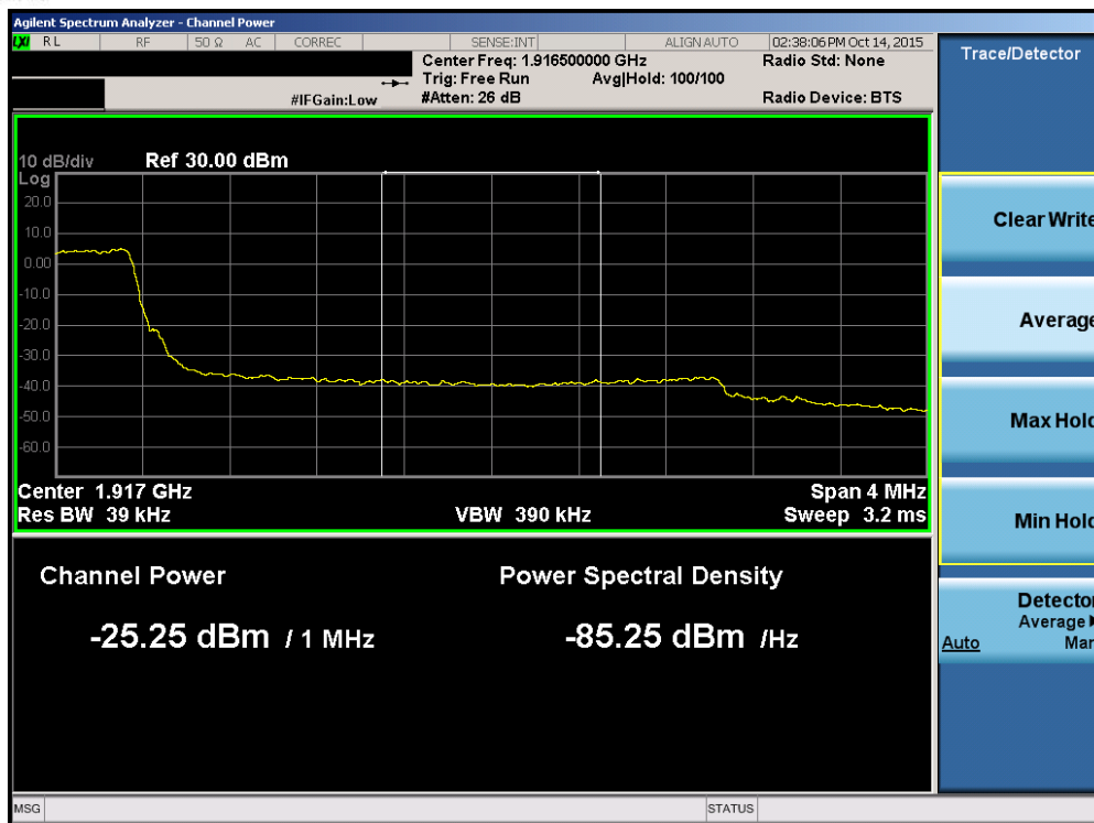
Plot 7-108. Upper Extended Band Edge Plot (Band 25 – 3.0MHz QPSK – RB Size 15)
