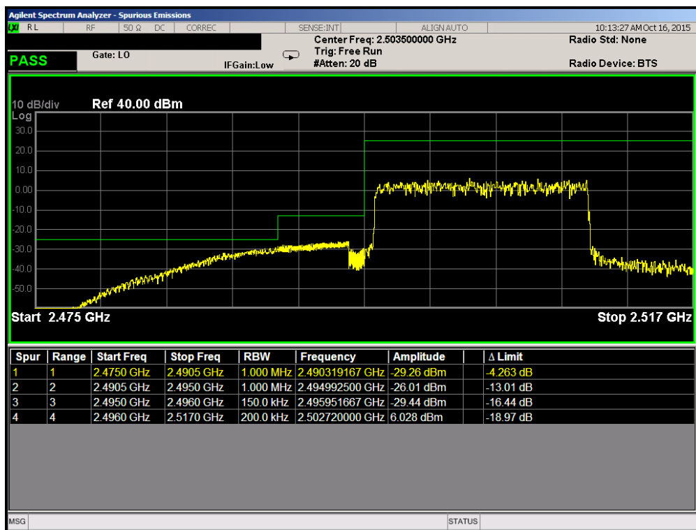
Plot 7-129. Lower ACP Plot (Band 41 – 15.0MHz QPSK – RB Size 75)
