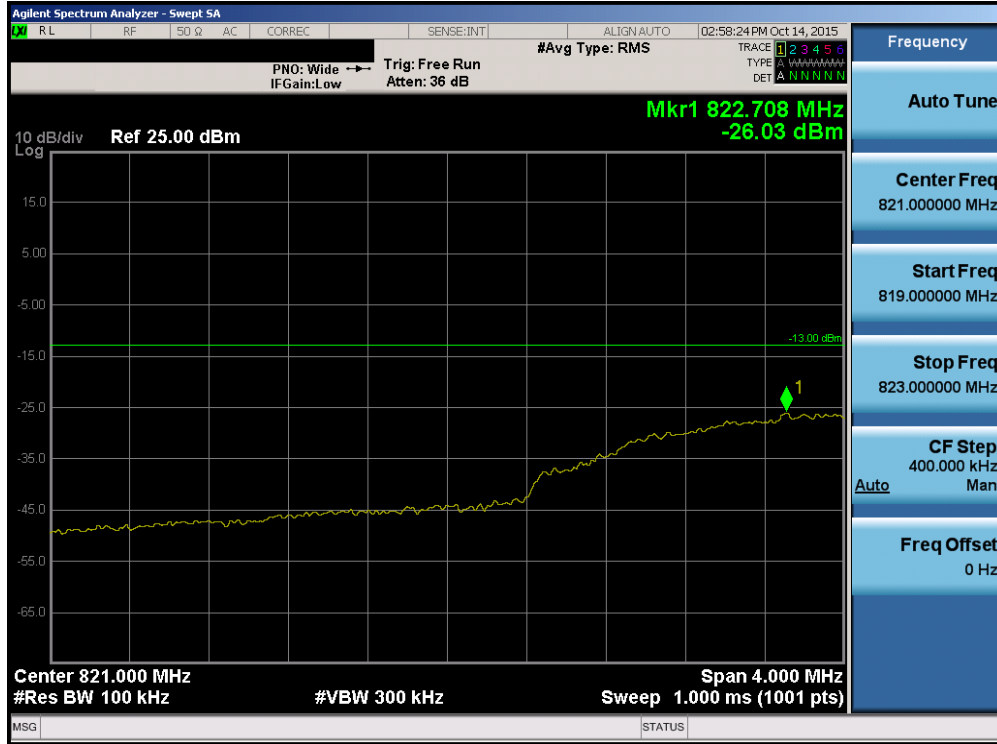
Plot 7-90. Lower Extended Band Edge Plot (Band 26 – 3.0MHz QPSK – RB Size 15)
