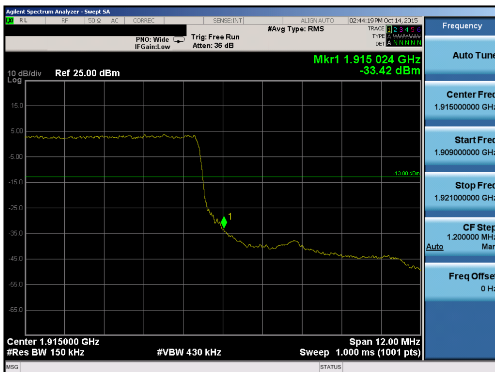
Plot 7-119. Upper Band Edge Plot (Band 25 – 15.0MHz QPSK – RB Size 75)
