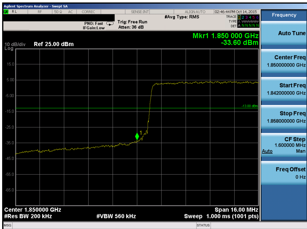
Plot 7-121. Lower Band Edge Plot (Band 25 – 20.0MHz QPSK – RB Size 100)
