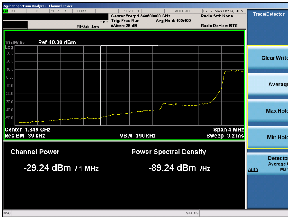
Plot 7-102. Lower Extended Band Edge Plot (Band 25 – 1.4MHz QPSK – RB Size 6)
