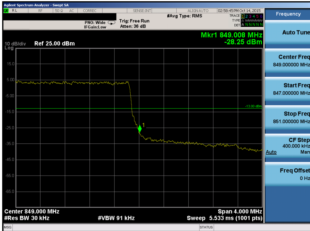
Plot 7-91. Upper Band Edge Plot (Band 26 – 3.0MHz QPSK – RB Size 15)
