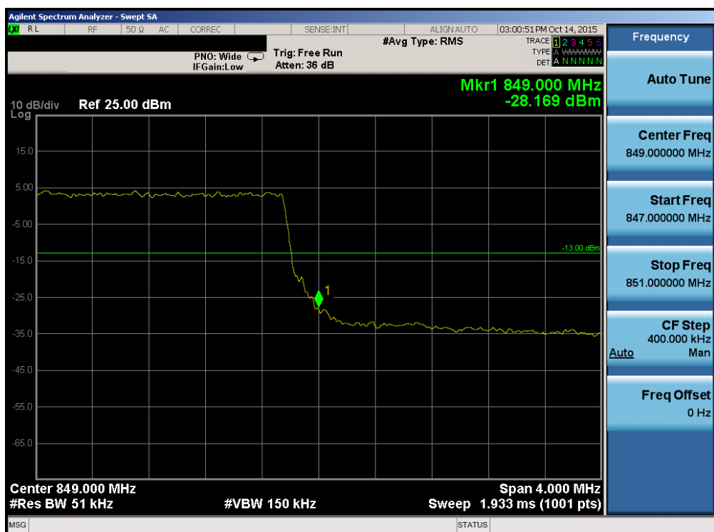
Plot 7-95. Upper Band Edge Plot (Band 26 - 5.0MHz QPSK - RB Size 25)
