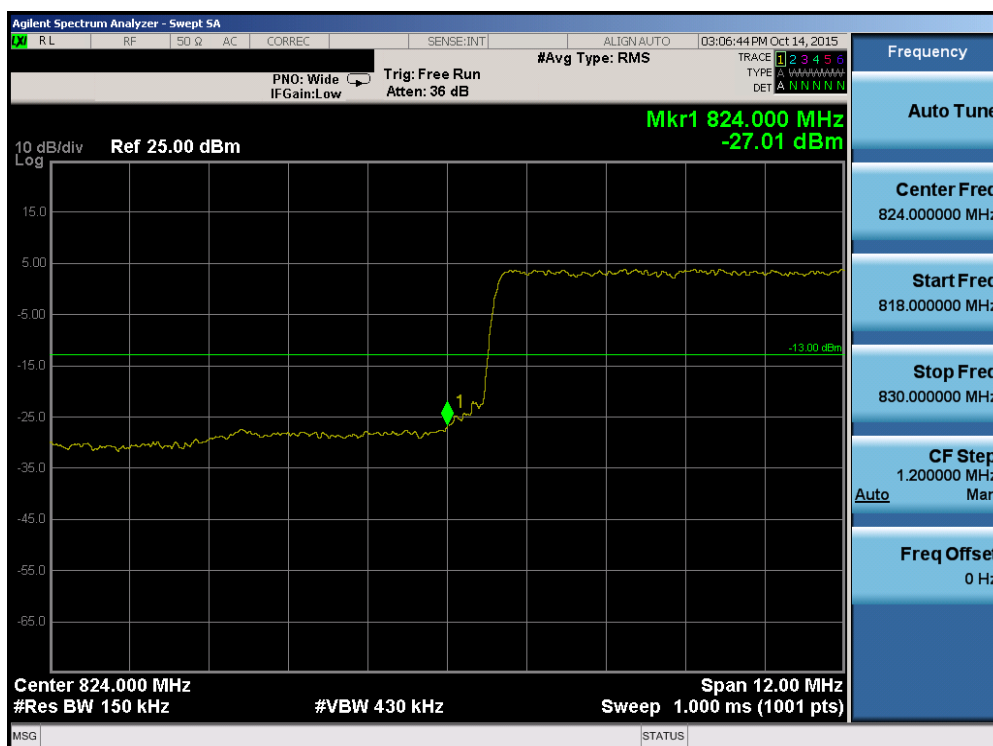
Plot 7-99. Lower Band Edge Plot (Band 26 – 15.0MHz QPSK – RB Size 75)
