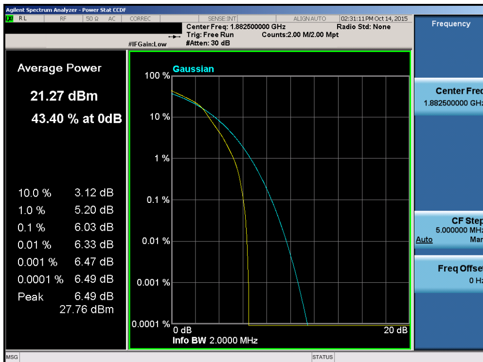
Plot 7-134. PAR Plot (Band 25 – 1.4MHz 16-QAM – RB Size 6)
