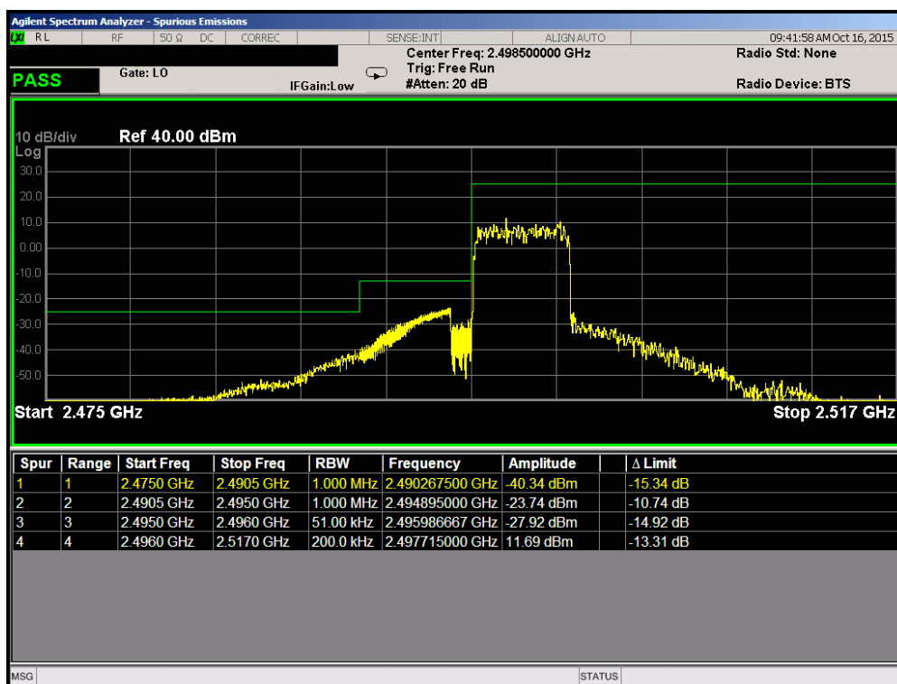
Plot 7-125. Lower ACP Plot (Band 41 – 5.0MHz QPSK – RB Size 25)
