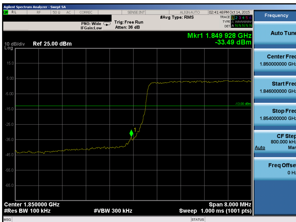
Plot 7-113. Lower Band Edge Plot (Band 25 – 10.0MHz QPSK – RB Size 50)
