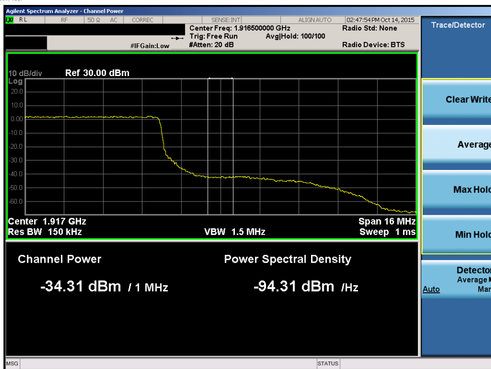
Plot 7-124. Upper Extended Band Edge Plot (Band 25 – 20.0MHz QPSK – RB Size 100)
