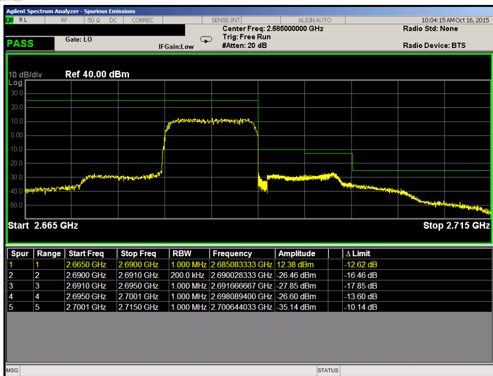
Plot 7-128. Upper ACP Plot (Band 41 – 10.0MHz QPSK – RB Size 50)
