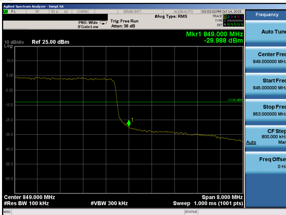
Plot 7-98. Upper Band Edge Plot (Band 26 – 10.0MHz QPSK – RB Size 50)
