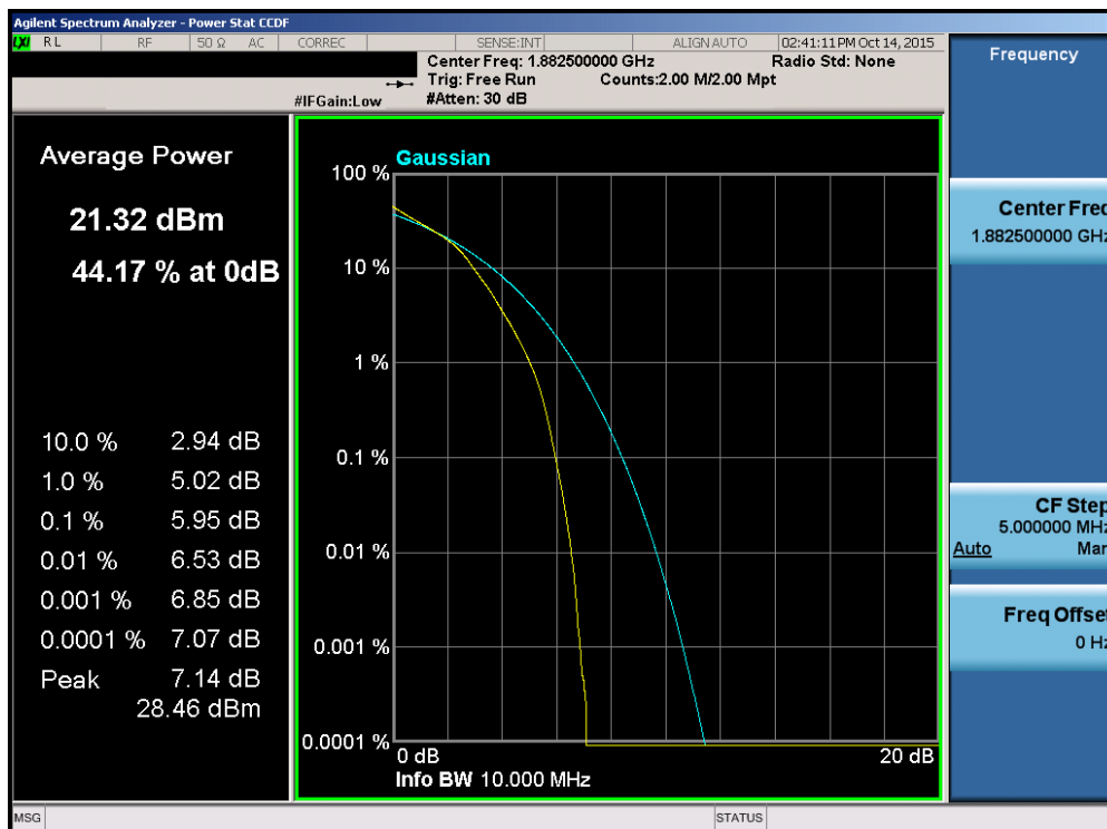
Plot 7-140. PAR Plot (Band 25 – 10.0MHz 16-QAM – RB Size 50)
