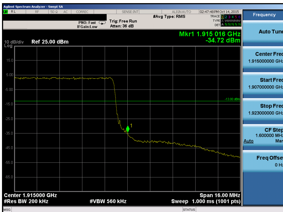
Plot 7-123. Upper Band Edge Plot (Band 25 – 20.0MHz QPSK – RB Size 100)
