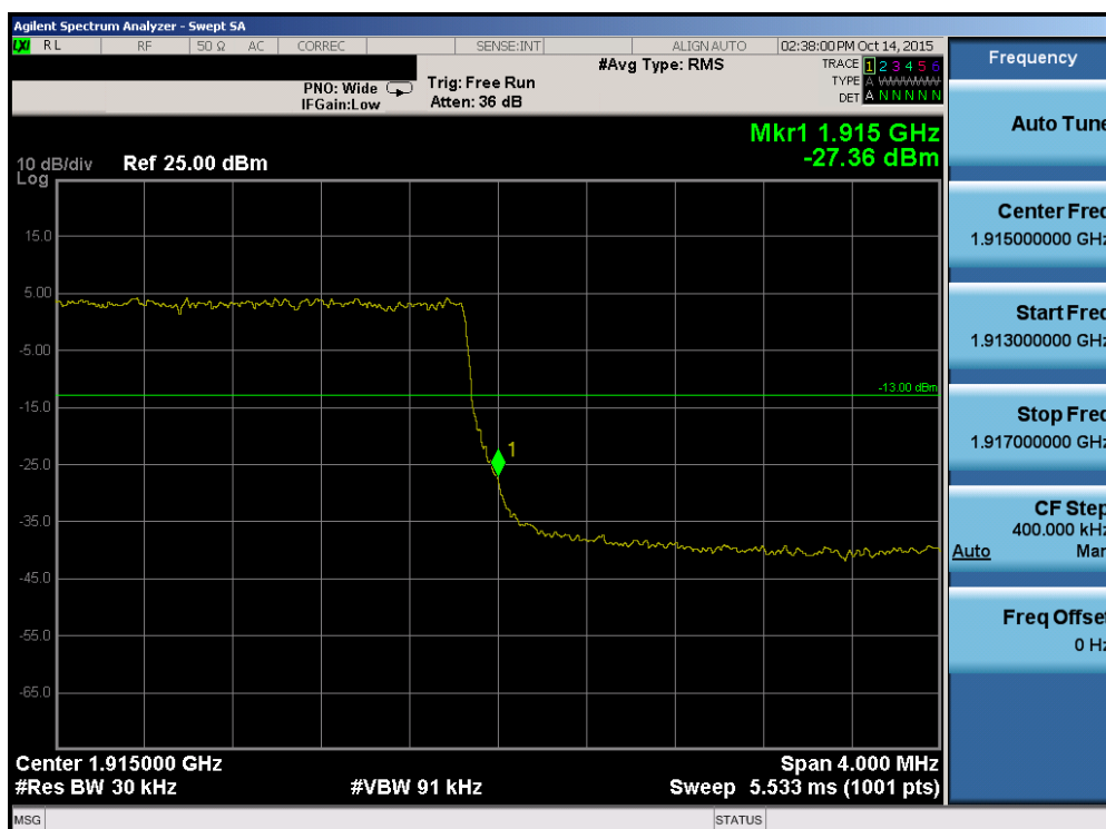
Plot 7-107. Upper Band Edge Plot (Band 25 – 3.0MHz QPSK – RB Size 15)
