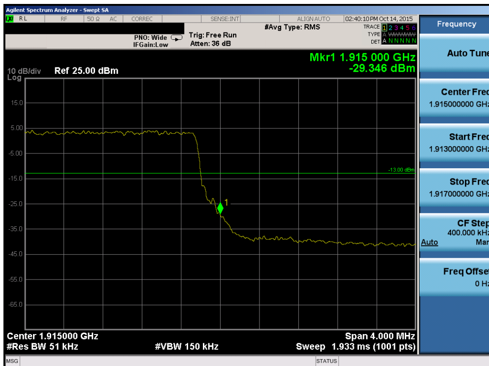
Plot 7-111. Upper Band Edge Plot (Band 25 – 5.0MHz QPSK – RB Size 25)
