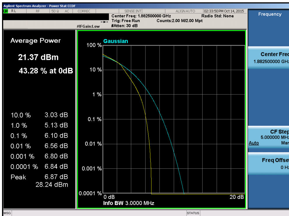
Plot 7-136. PAR Plot (Band 25 – 3.0MHz 16-QAM – RB Size 15)
