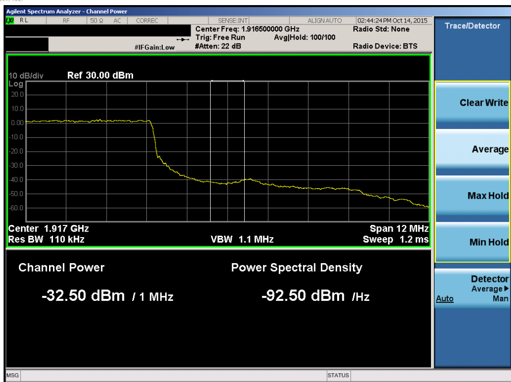
Plot 7-120. Upper Extended Band Edge Plot (Band 25 – 15.0MHz QPSK – RB Size 75)
