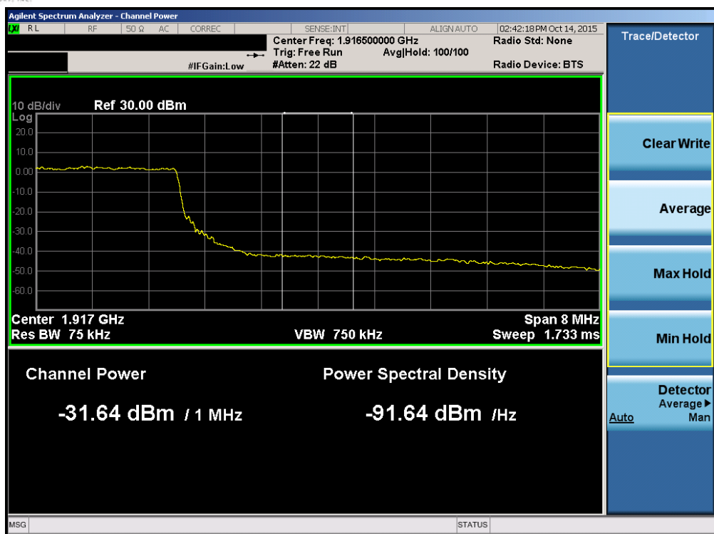
Plot 7-116. Upper Extended Band Edge Plot (Band 25 – 10.0MHz QPSK – RB Size 50)
