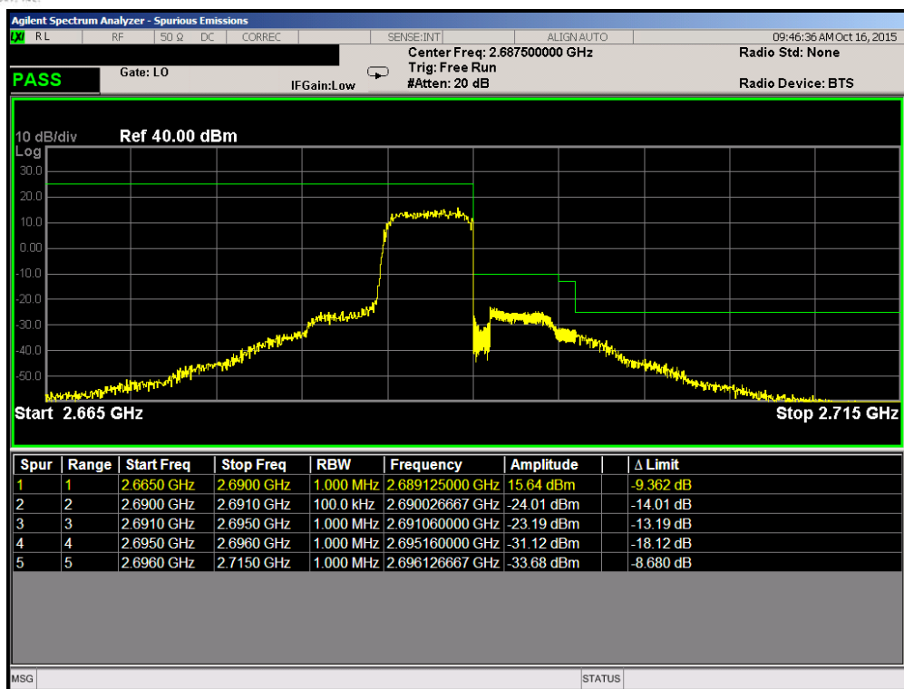
Plot 7-126. Upper ACP Plot (Band 41 – 5.0MHz QPSK – RB Size 25)
