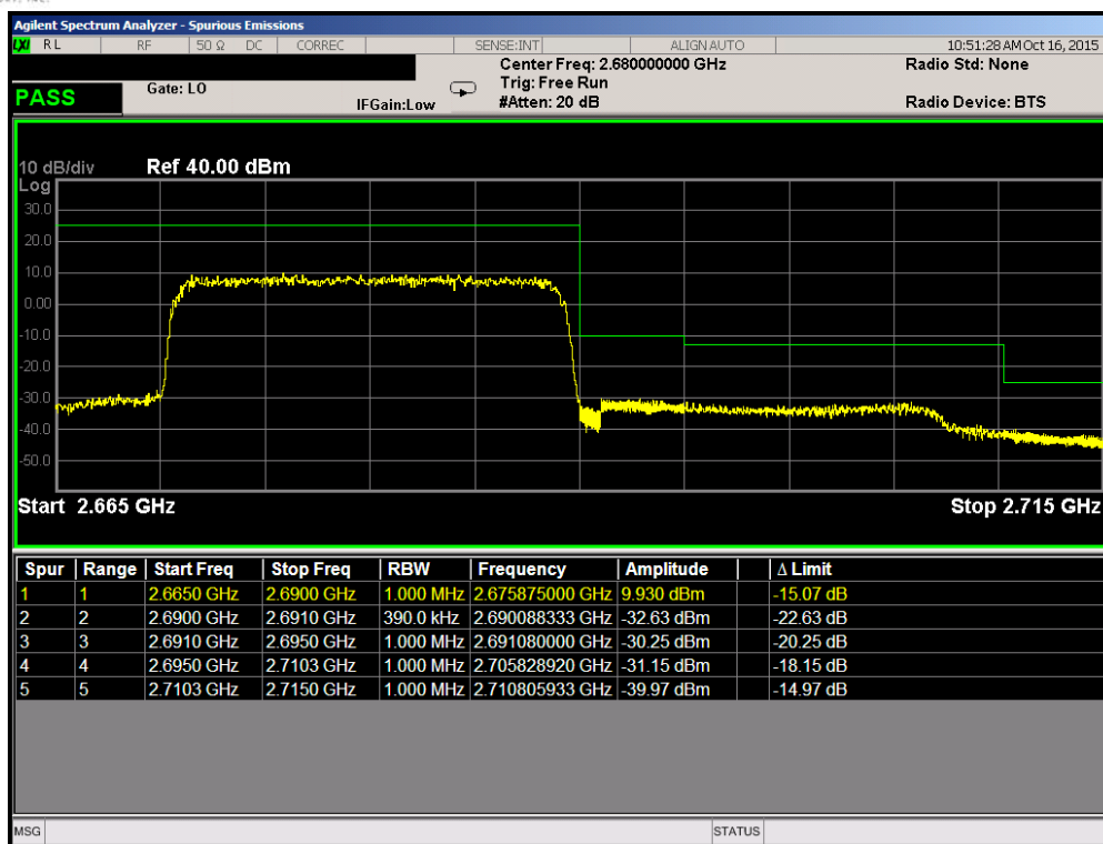
Plot 7-132. Upper ACP Plot (Band 41 – 20.0MHz QPSK – RB Size 100)
