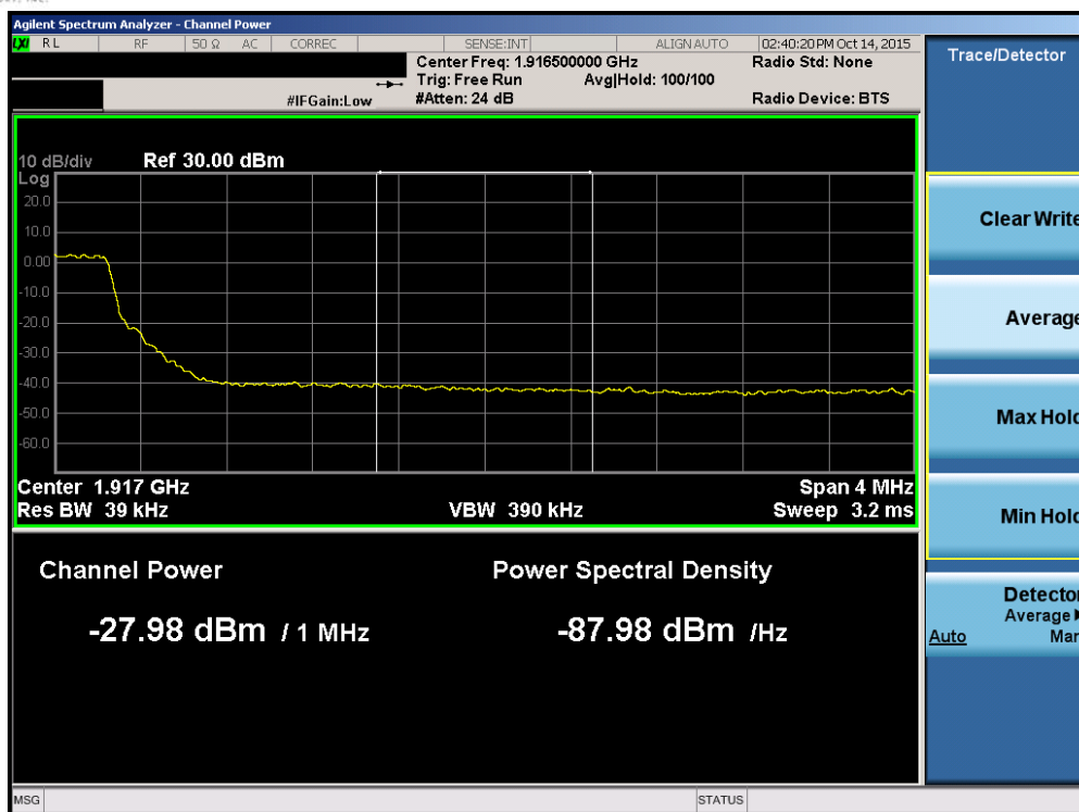
Plot 7-112. Upper Extended Band Edge Plot (Band 25 – 5.0MHz QPSK – RB Size 25)
