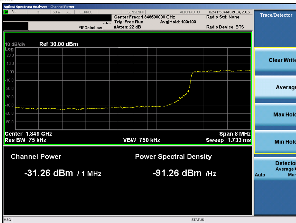
Plot 7-114. Lower Extended Band Edge Plot (Band 25 – 10.0MHz QPSK – RB Size 50)
