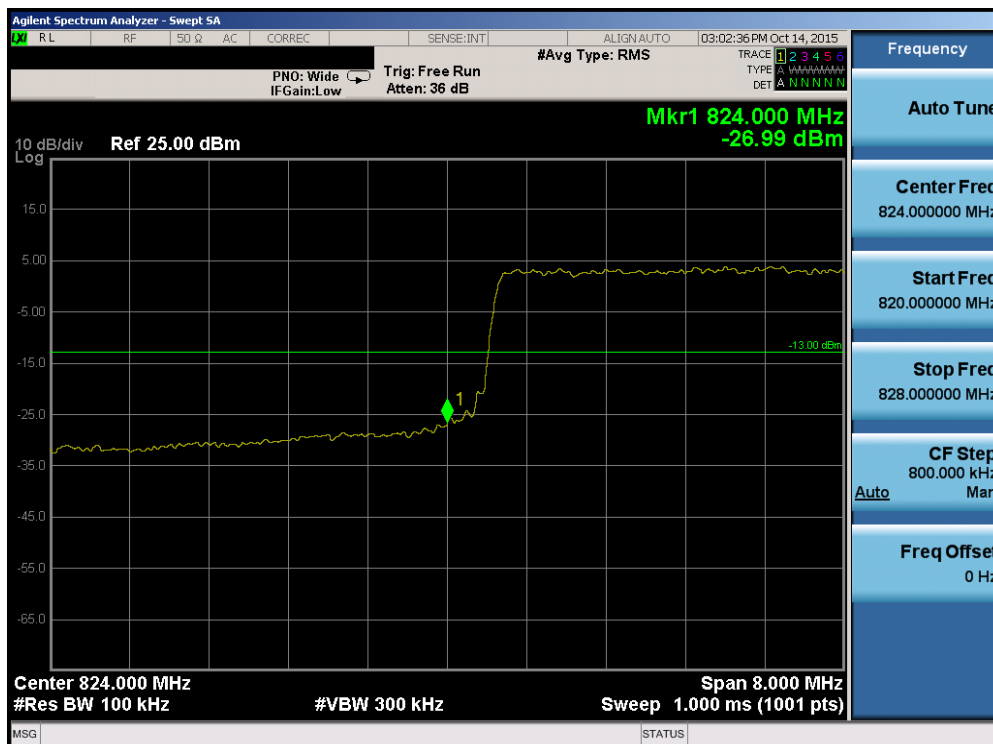
Plot 7-97. Lower Band Edge Plot (Band 26 – 10.0MHz QPSK – RB Size 50)
